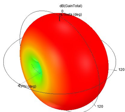
Gain Plot 1
