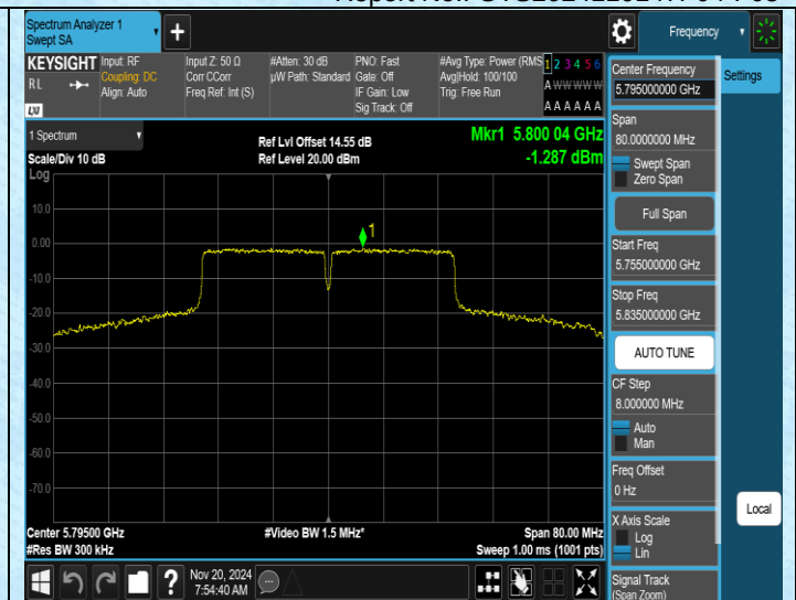
11AC40SISO-Ant1-5795-PASS
