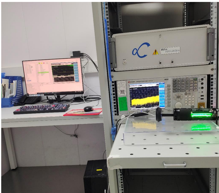
Conducted Test-BT/WIFI/2.4G ISM Band
