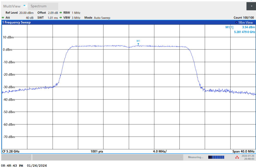
11AX20-5280-PASS
