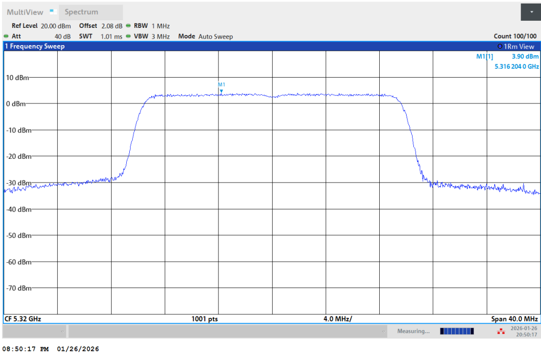
11AX20-5320-PASS
