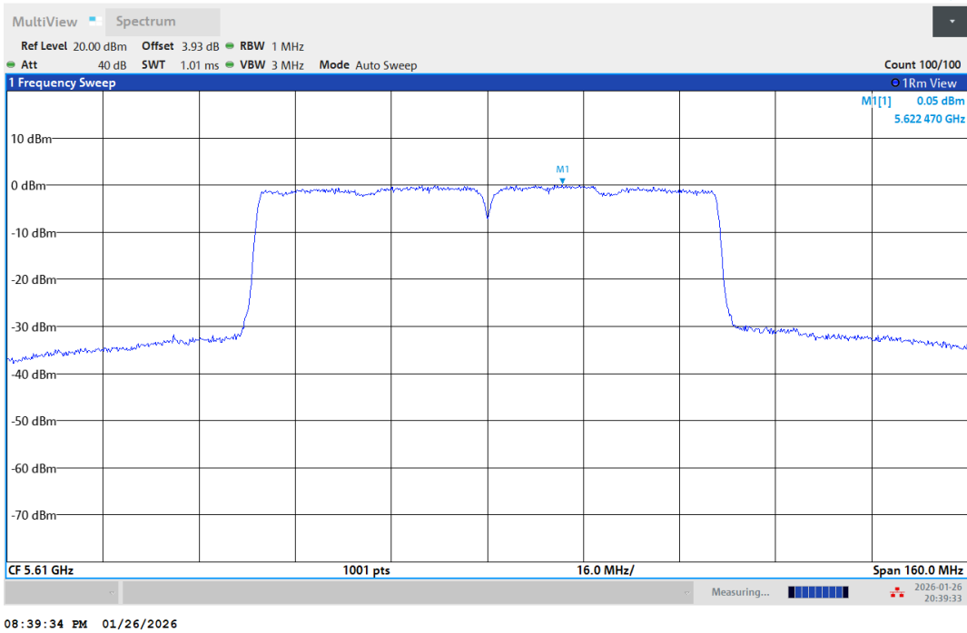
11AC80-5610-PASS
