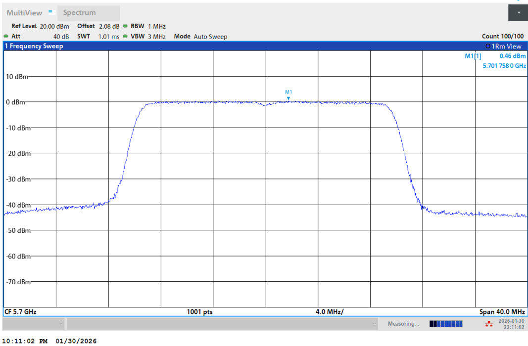
11AX20-5700-PASS
