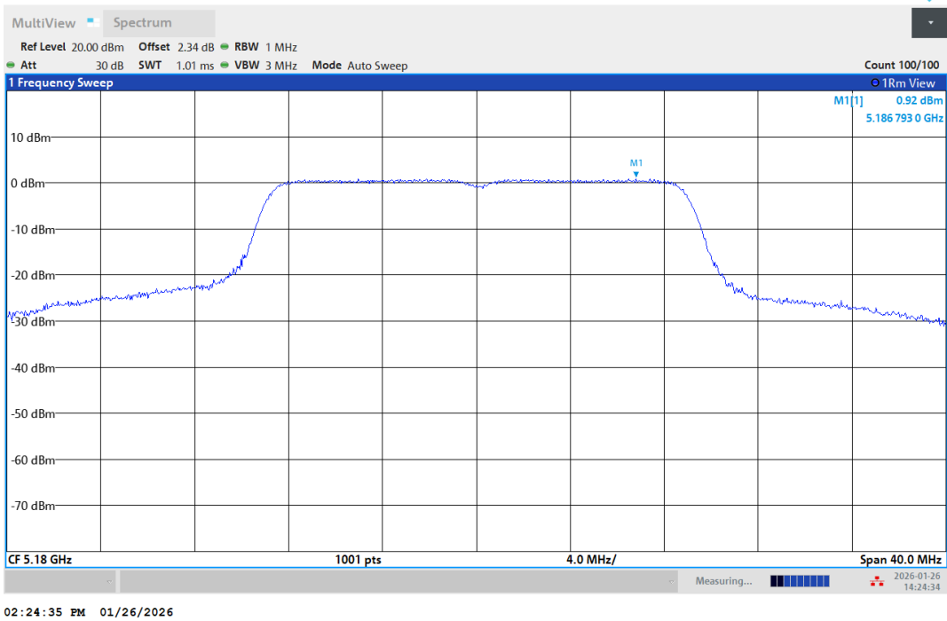
11AC20SISO-Ant1-5180-PASS
