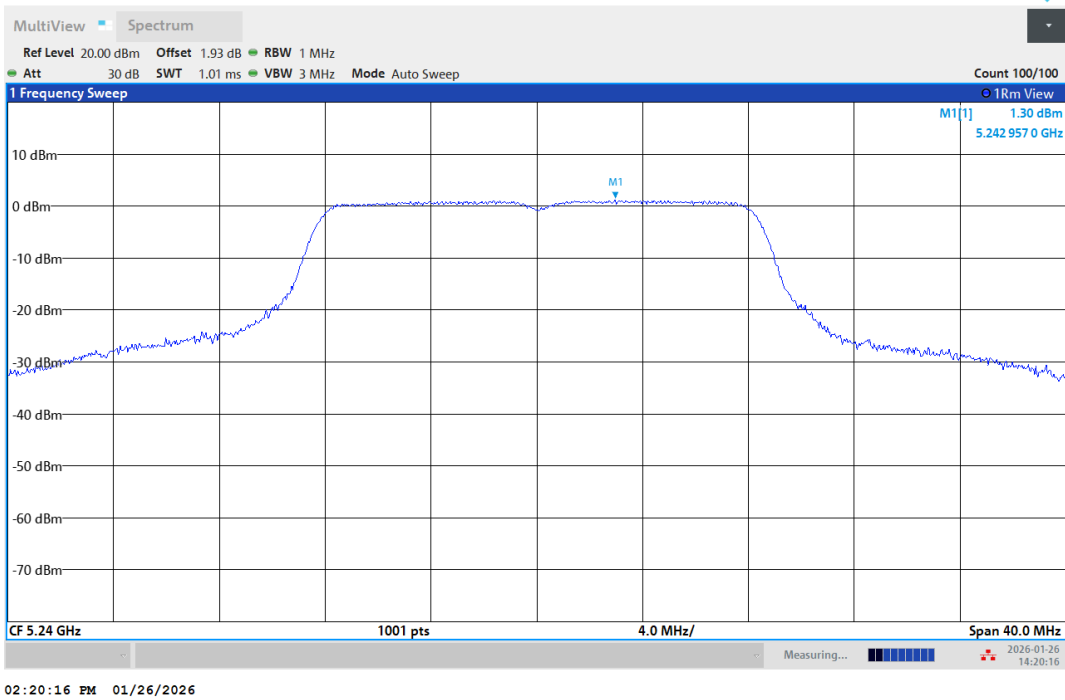
11A-Ant1-5240-PASS
