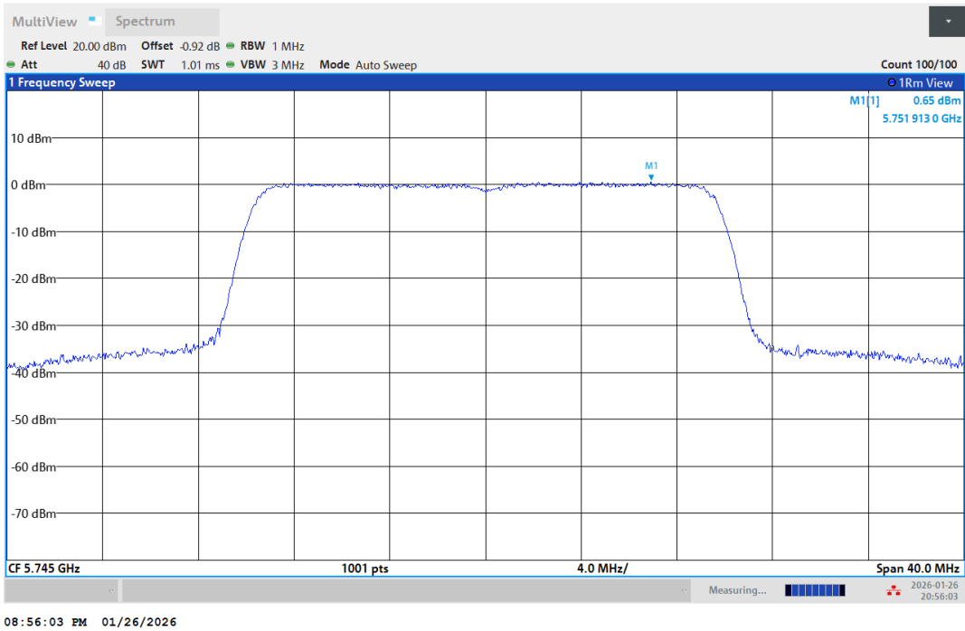
11AX20-5745-PASS
