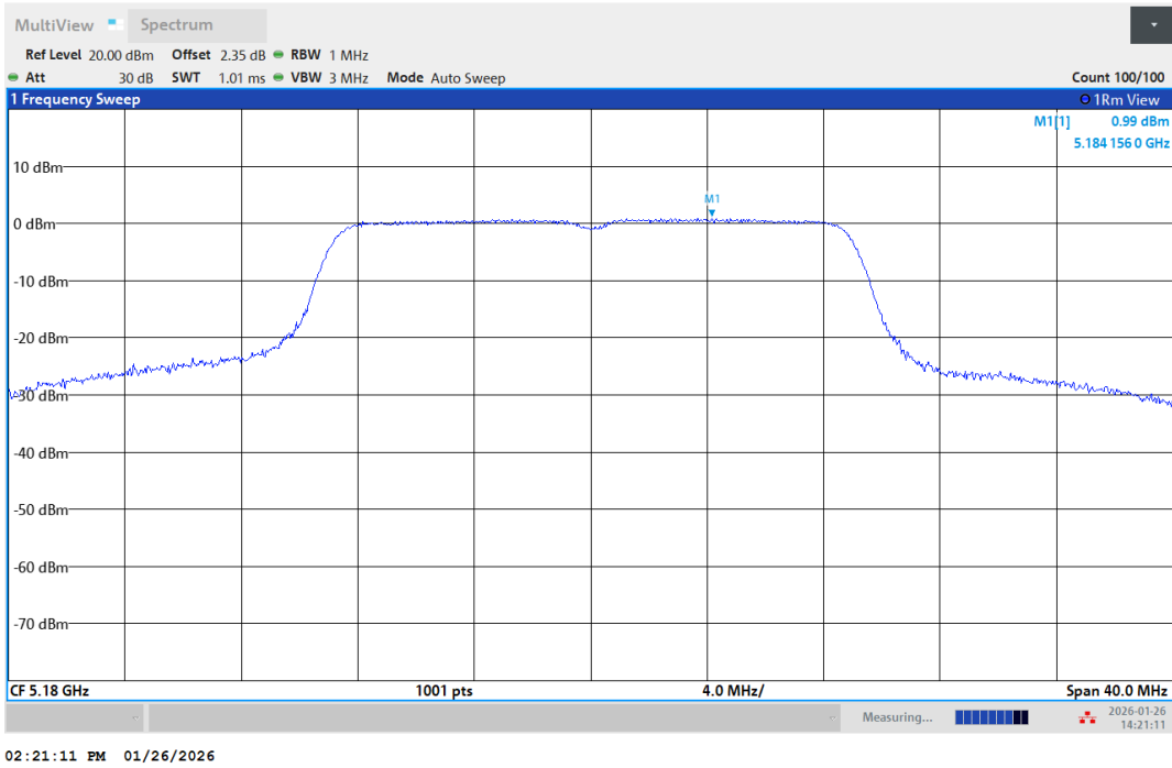
11N20SISO-Ant1-5180-PASS
