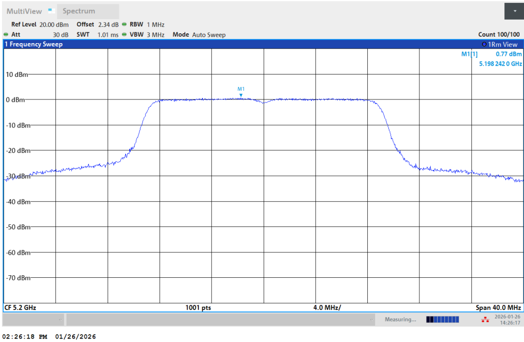
11AC20SISO-Ant1-5200-PASS
