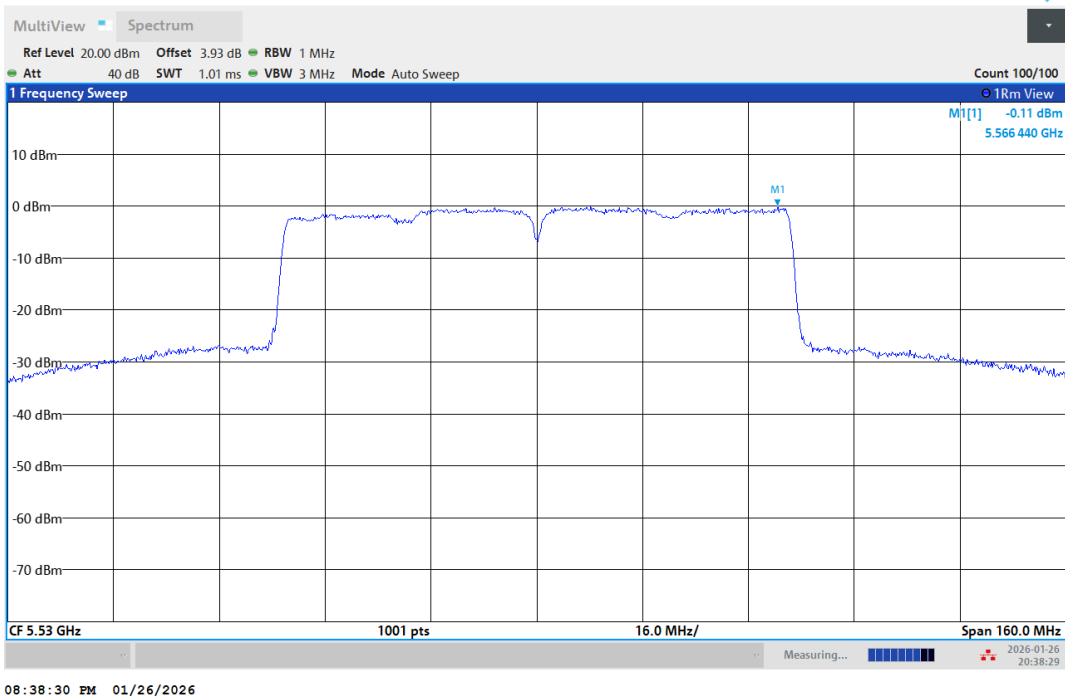
11AC80-5530-PASS
