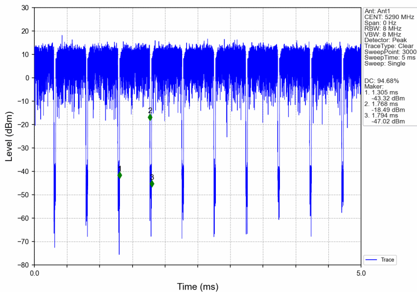
802.11ac(VHT80)_MCH_5290MHz_Ant1_NTNV
