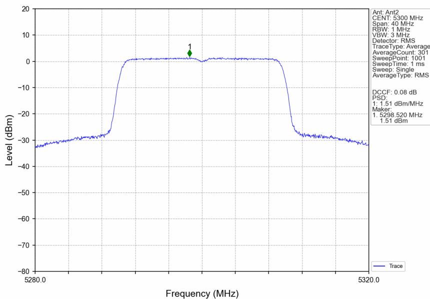
802.11ax(HEW20)_MCH_5300MHz_RU242_Left_Ant2_NTNV
