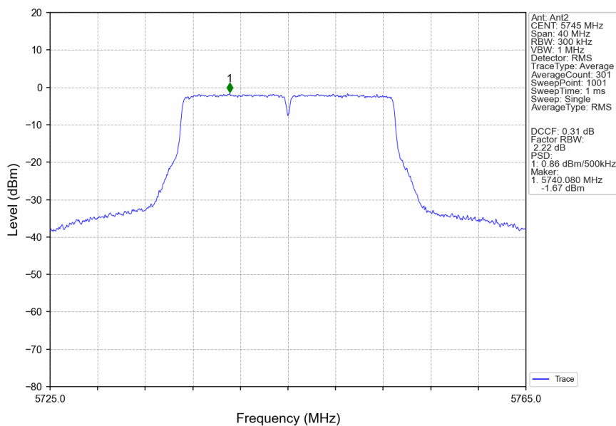
802.11n(HT20)_LCH_5745MHz_Ant2_NTNV
