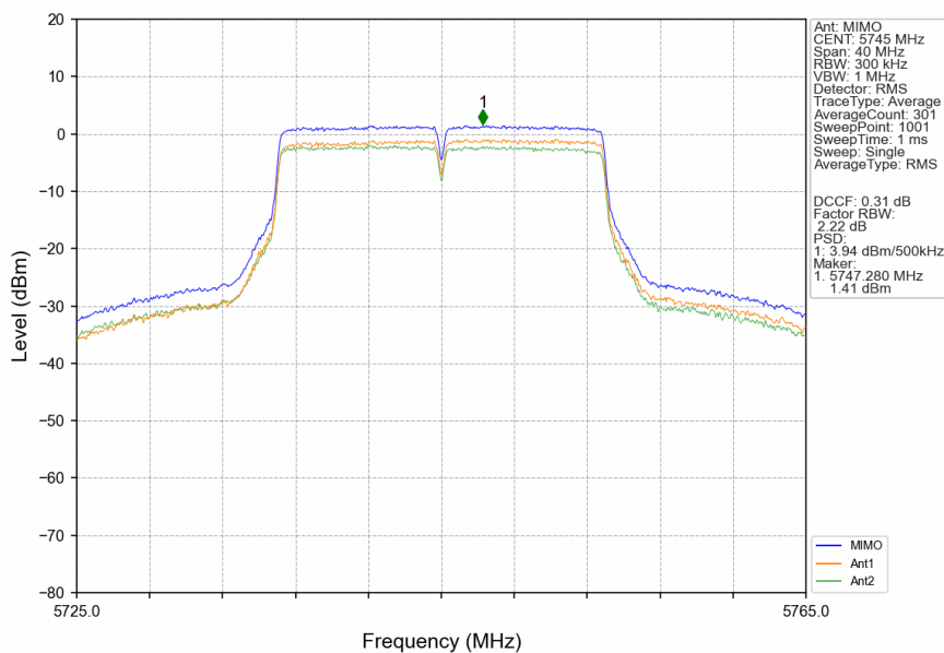
802.11ac(VHT20)_LCH_5745MHz_MIMO_NTNV
