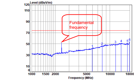
BLE_1M_TX_CH_00_Horizontal-Peak
