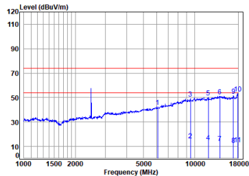
BT_DH5_TX_CH_78_Horizontal
