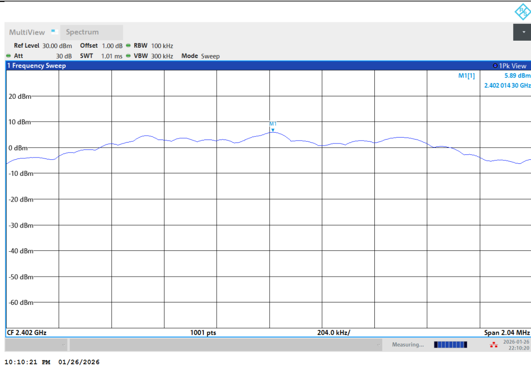
BLE_2M-Ant1-2402-PASS
