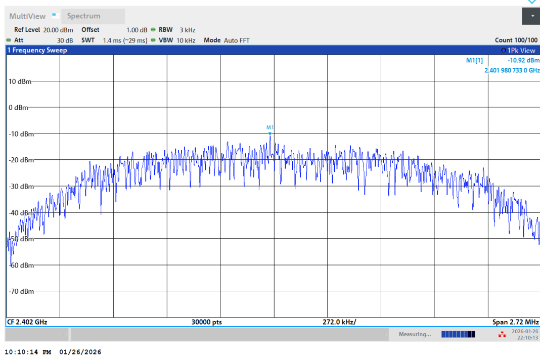
BLE_2M-Ant1-2402-PASS
