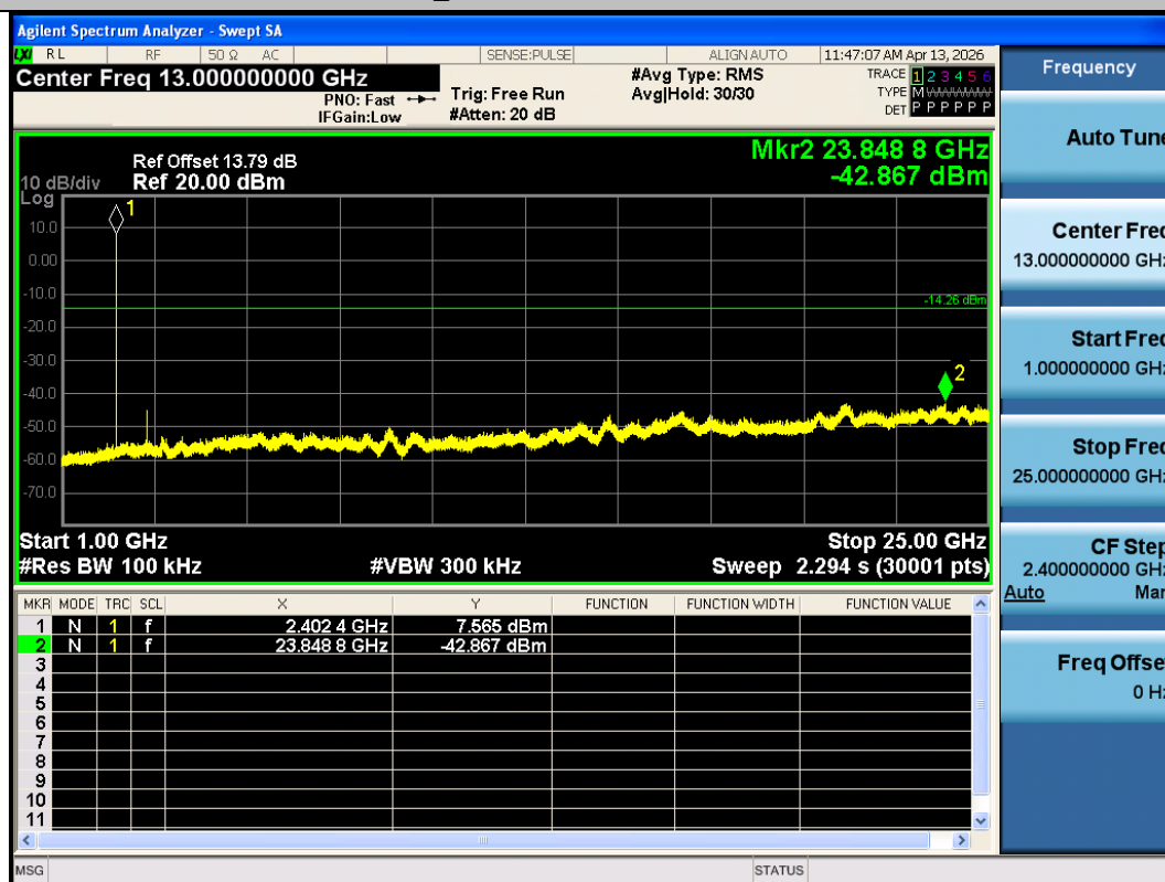
BLE_1M-Ant1-2402-1000~25000-PASS
