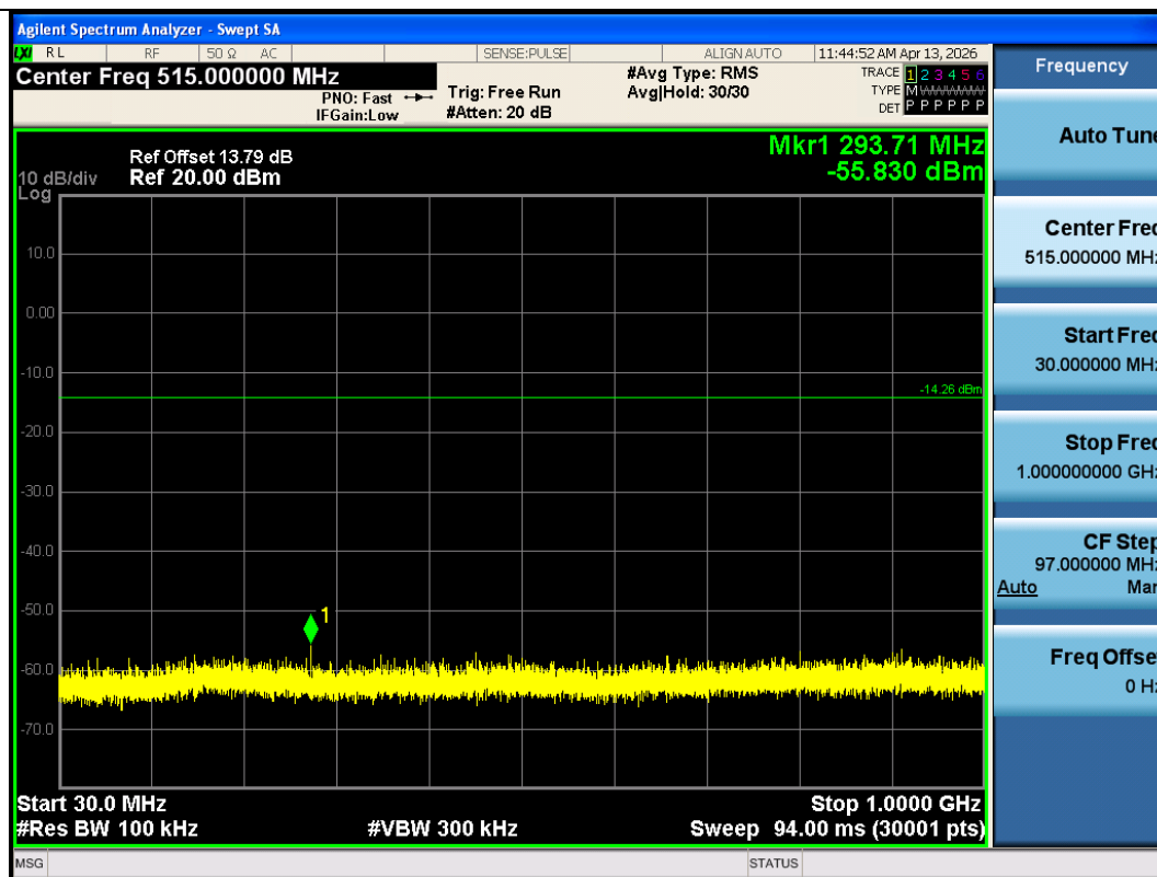
BLE_1M-Ant1-2402-30~1000-PASS
