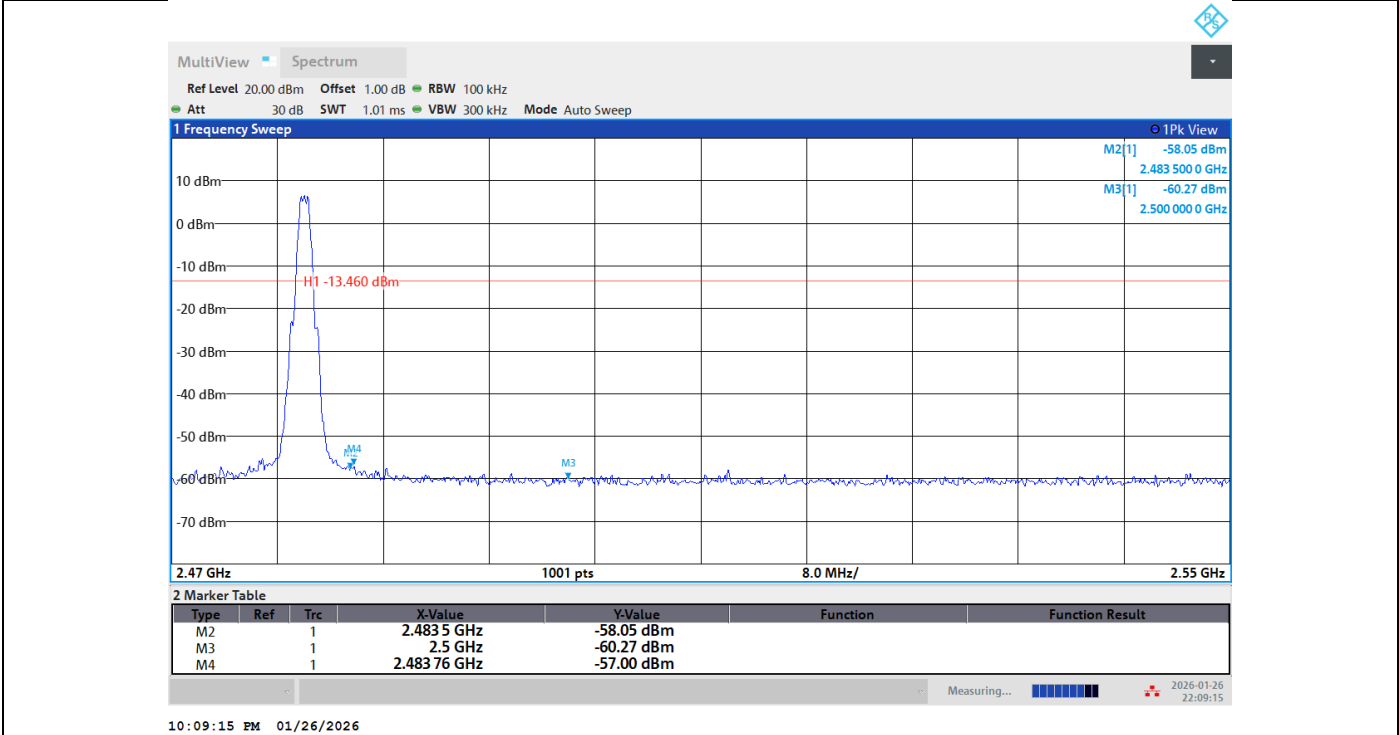
BLE_1M-Ant1-2480-PASS
