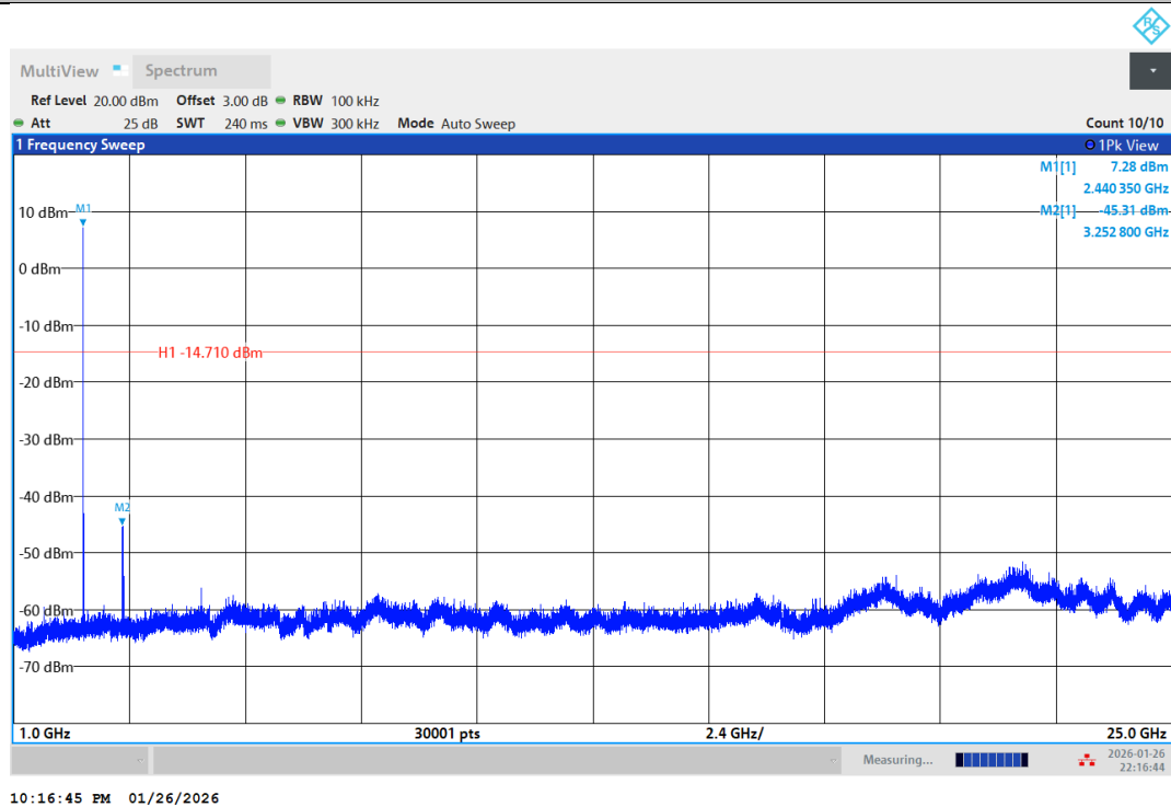
BLE_2M-Ant1-2440-1000~25000-PASS
