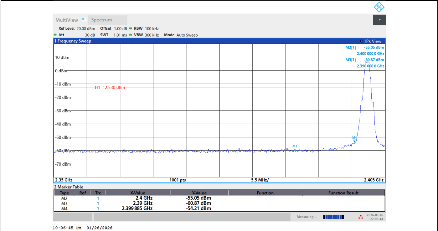
BLE_1M-Ant1-2402-PASS
