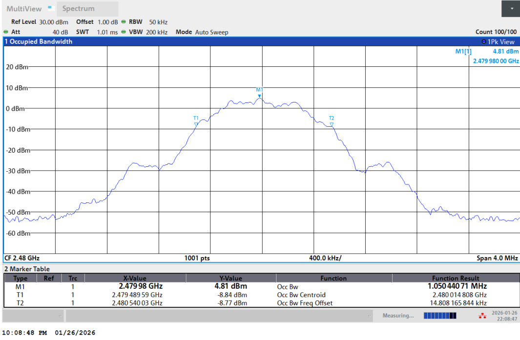
BLE_1M-Ant1-2480
