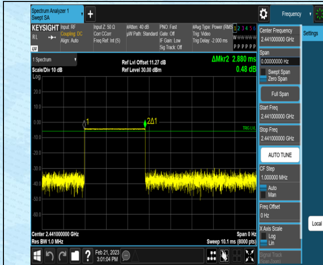
DH5-Ant1-Hop-2.880-106.67
