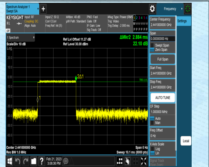
2DH5-Ant1-Hop-2.884-106.67
