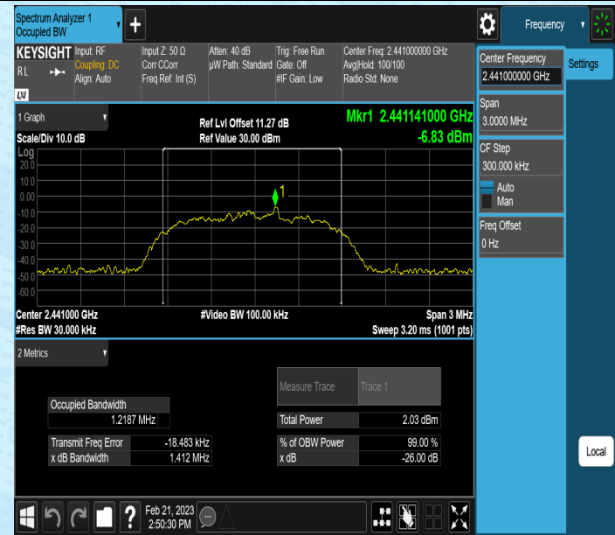
3DH5-Ant1-2441
