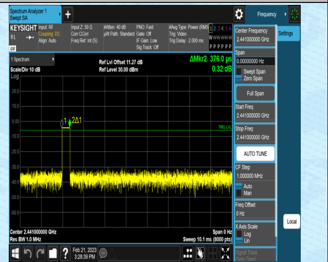
DH1-Ant1-Hop-0.376-320
