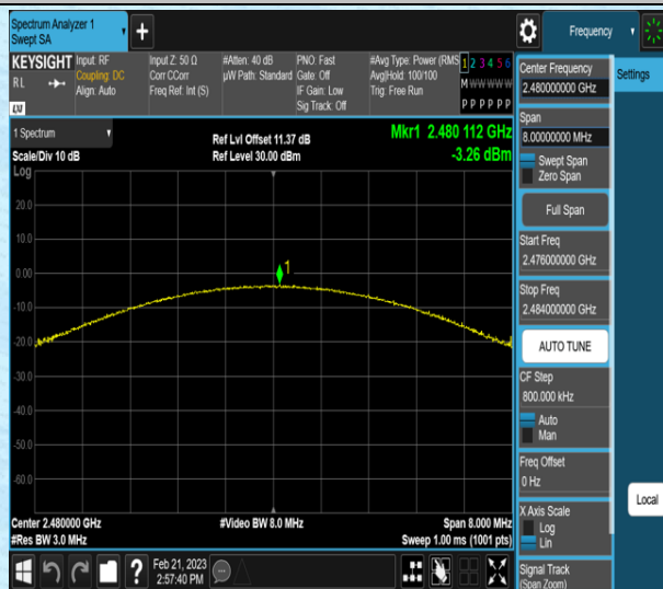
3DH5-Ant1-2480
