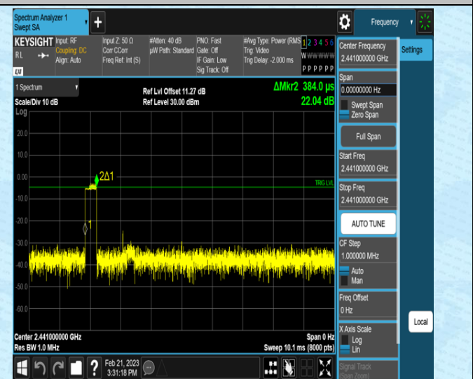
3DH1-Ant1-Hop-0.384-320
