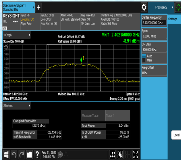
3DH5-Ant1-2402
