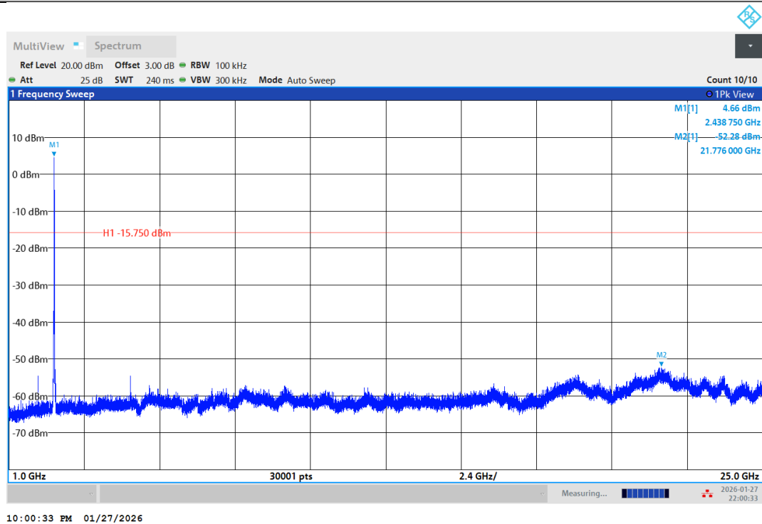
11B-Ant1-2437-1000~25000-PASS
