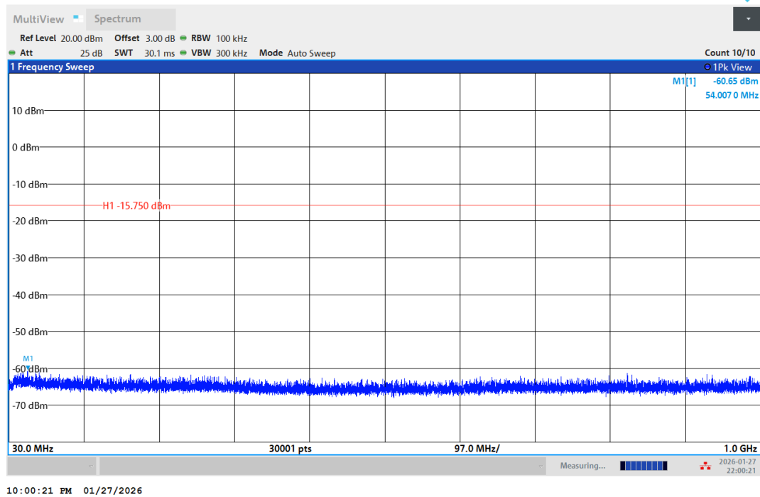
11B-Ant1-2437-30~1000-PASS
