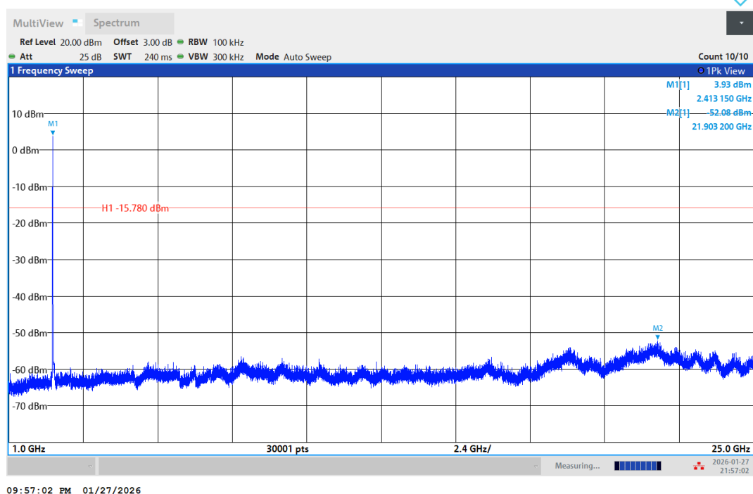
11B-Ant1-2412-1000~25000-PASS
