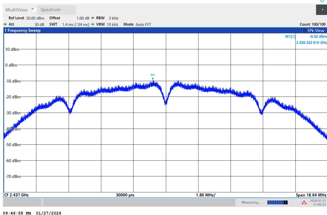
11B-Ant1-2437-PASS
