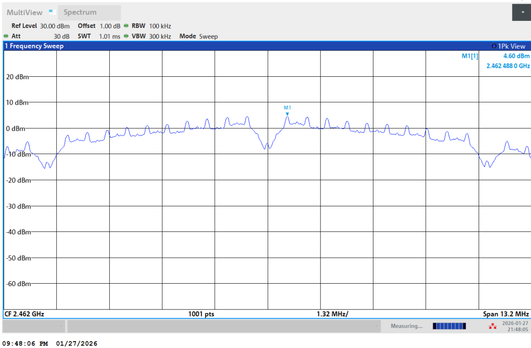
11B-Ant1-2462-PASS
