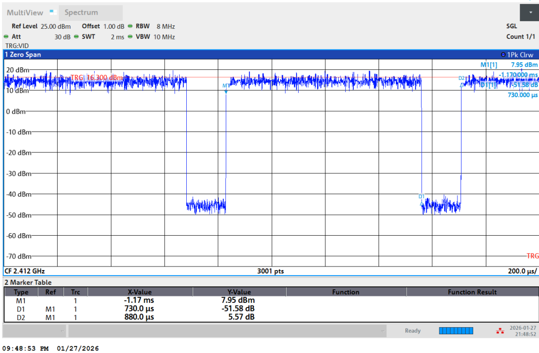
NTNV-11G-Ant1-2412
