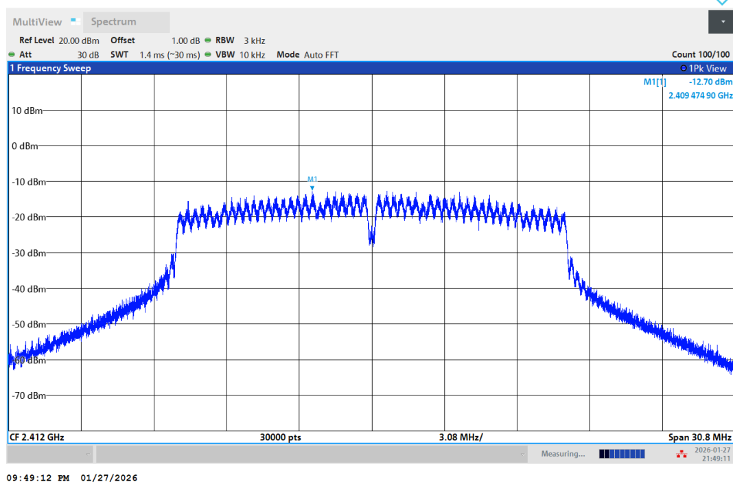
11G-Ant1-2412-PASS
