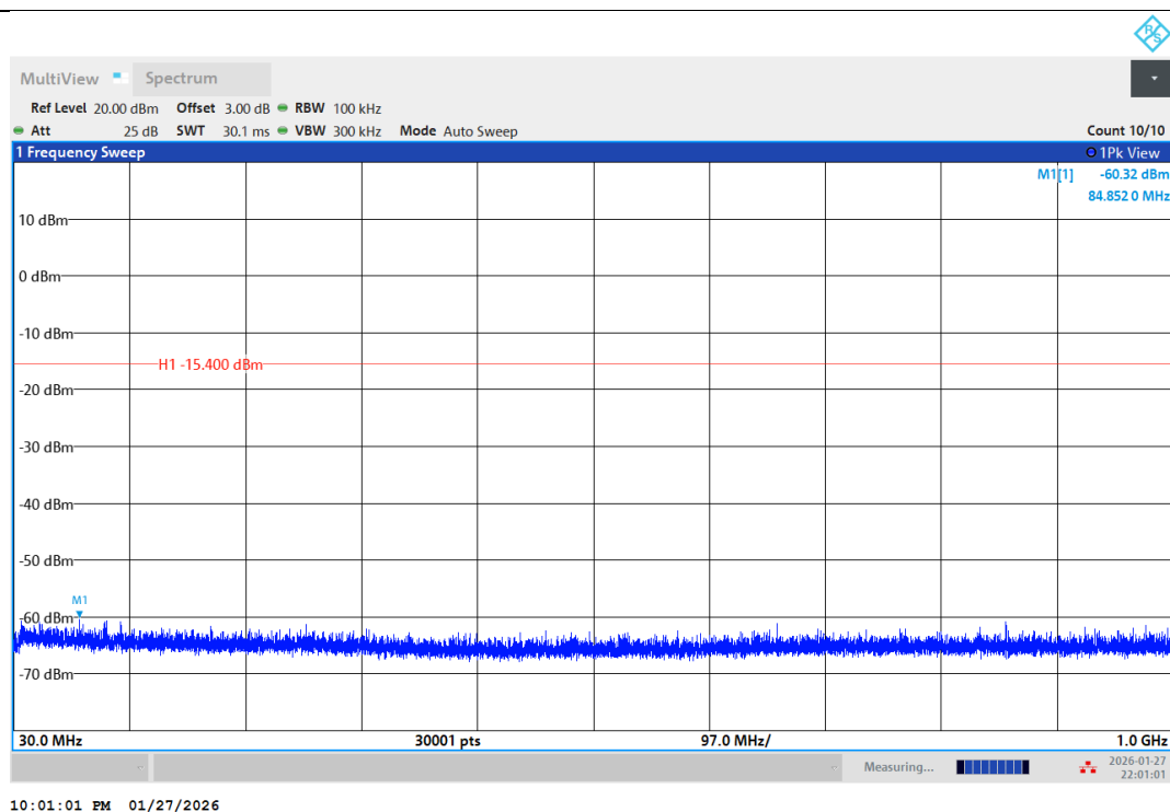
11B-Ant1-2462-30~1000-PASS
