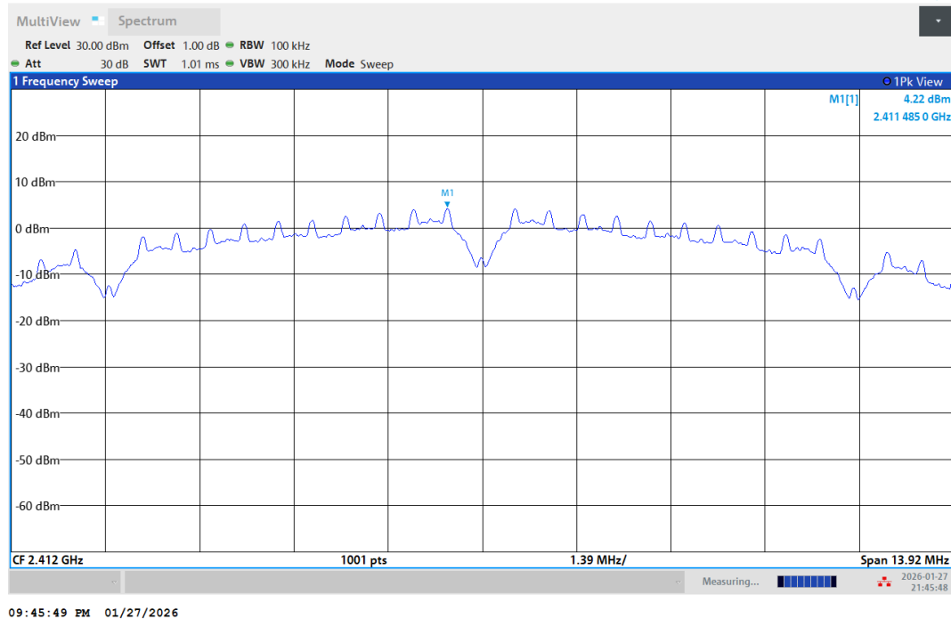
11B-Ant1-2412-PASS
