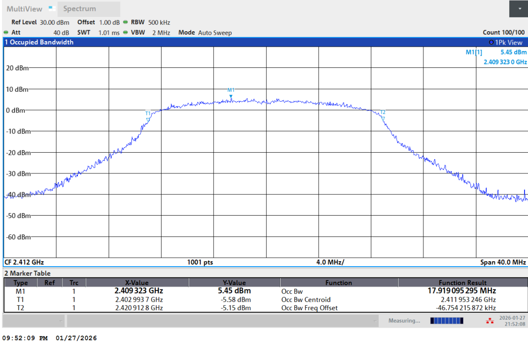
11N20SI-ISO-Ant1-2412
