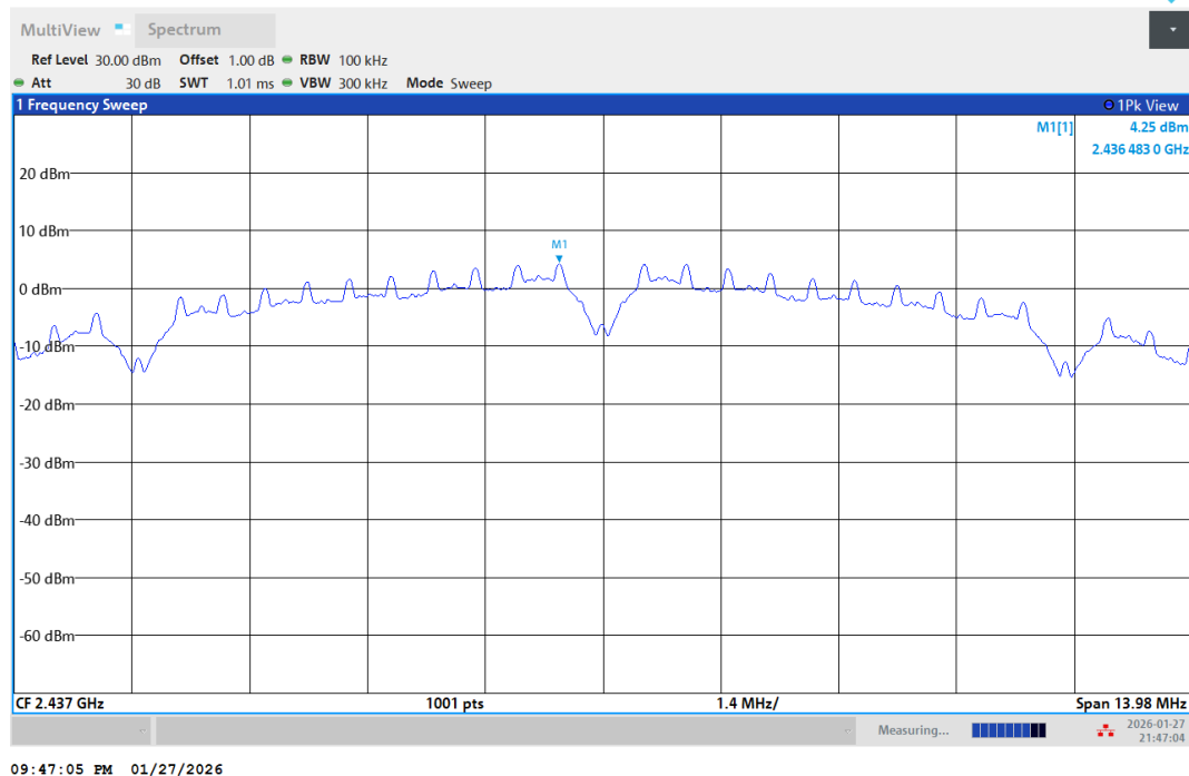
11B-Ant1-2437-PASS
