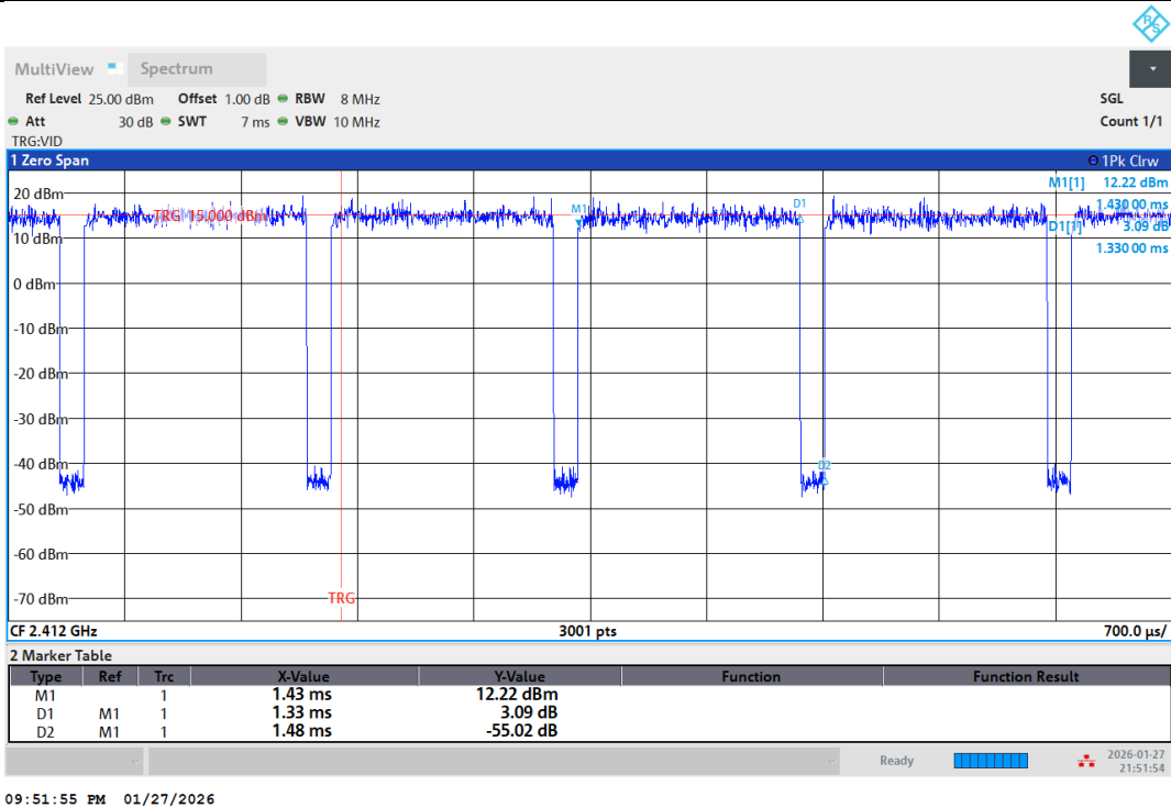
NTNV-11N20SISO-Ant1-2412
