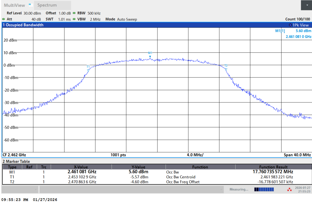
11N20SISO-Ant1-2462
