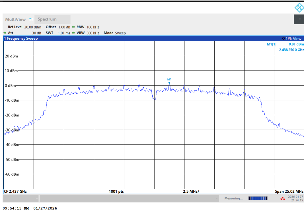
11N20SISO-Ant1-2437-PASS
