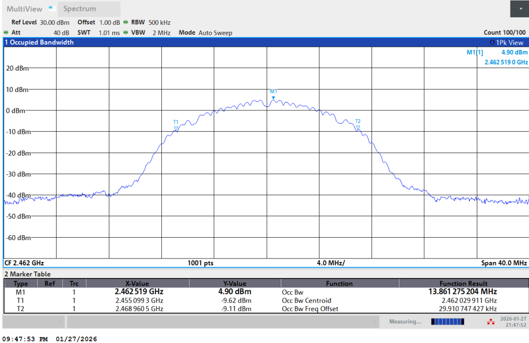
11B-Ant1-2462
