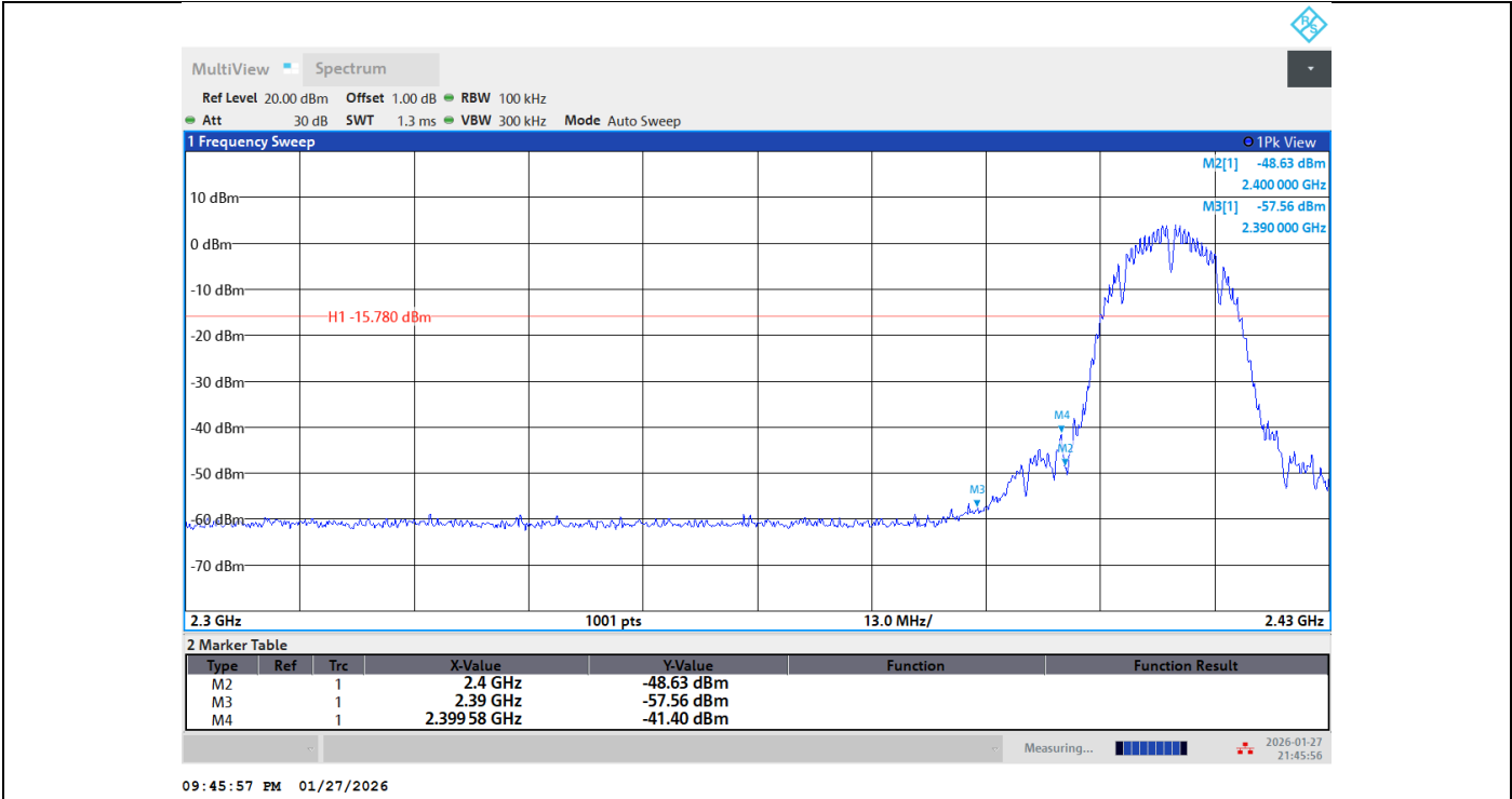
11B-Ant1-2412-PASS
