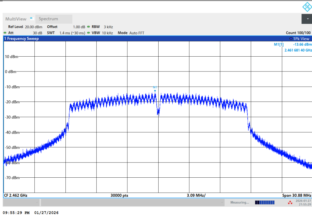
11N20SISO-Ant1-2462-PASS
