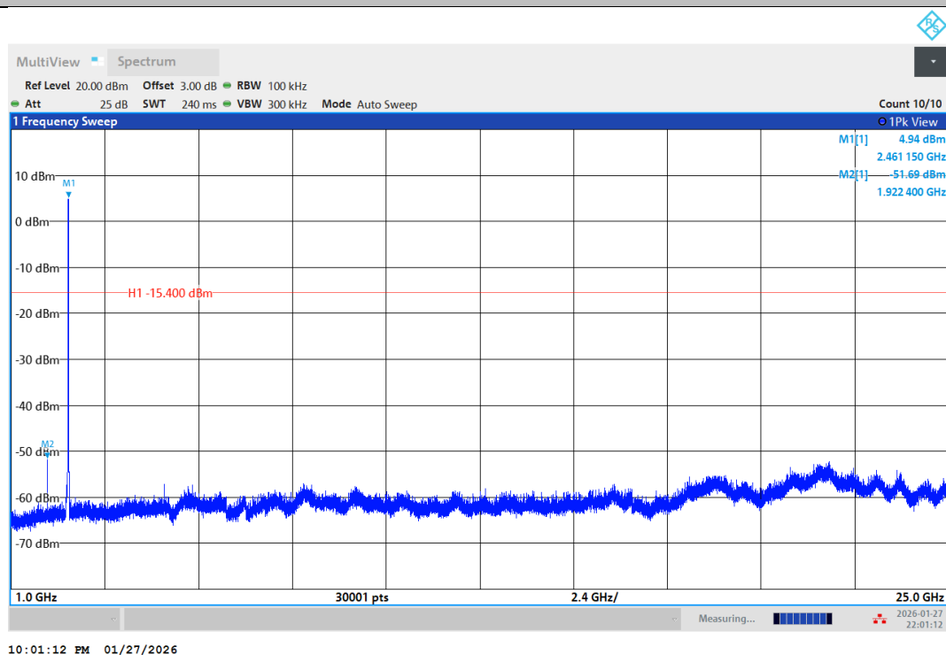
11B-Ant1-2462-1000~25000-PASS
