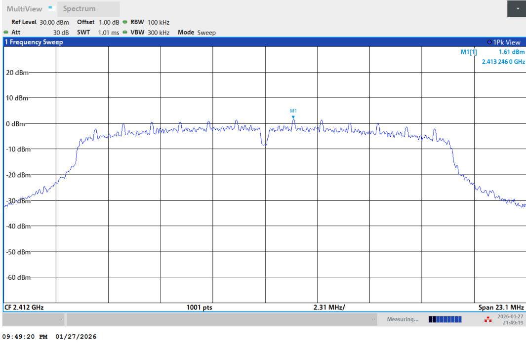
11G-Ant1-2412-PASS
