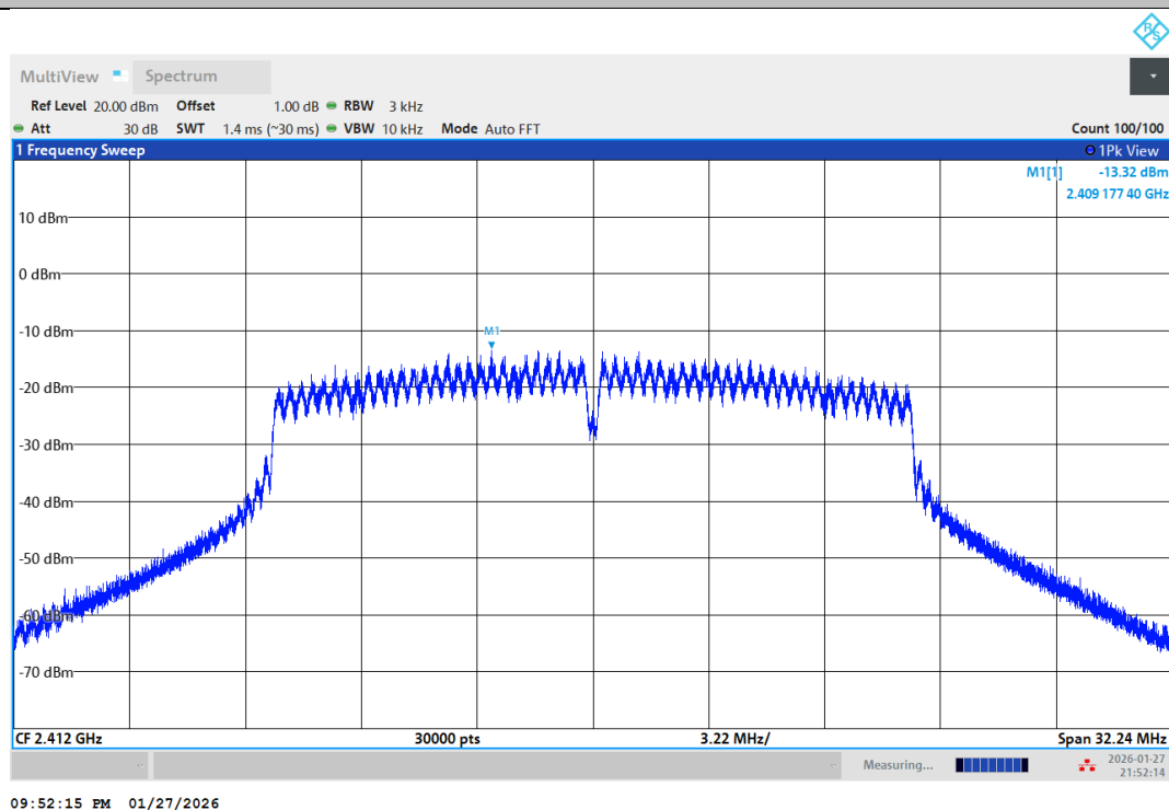
11N20SISO-Ant1-2412-PASS
