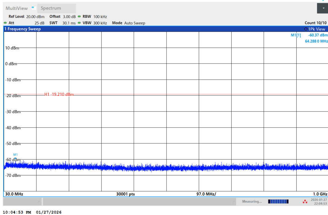
11N20SISO-Ant1-2462-30~1000-PASS
