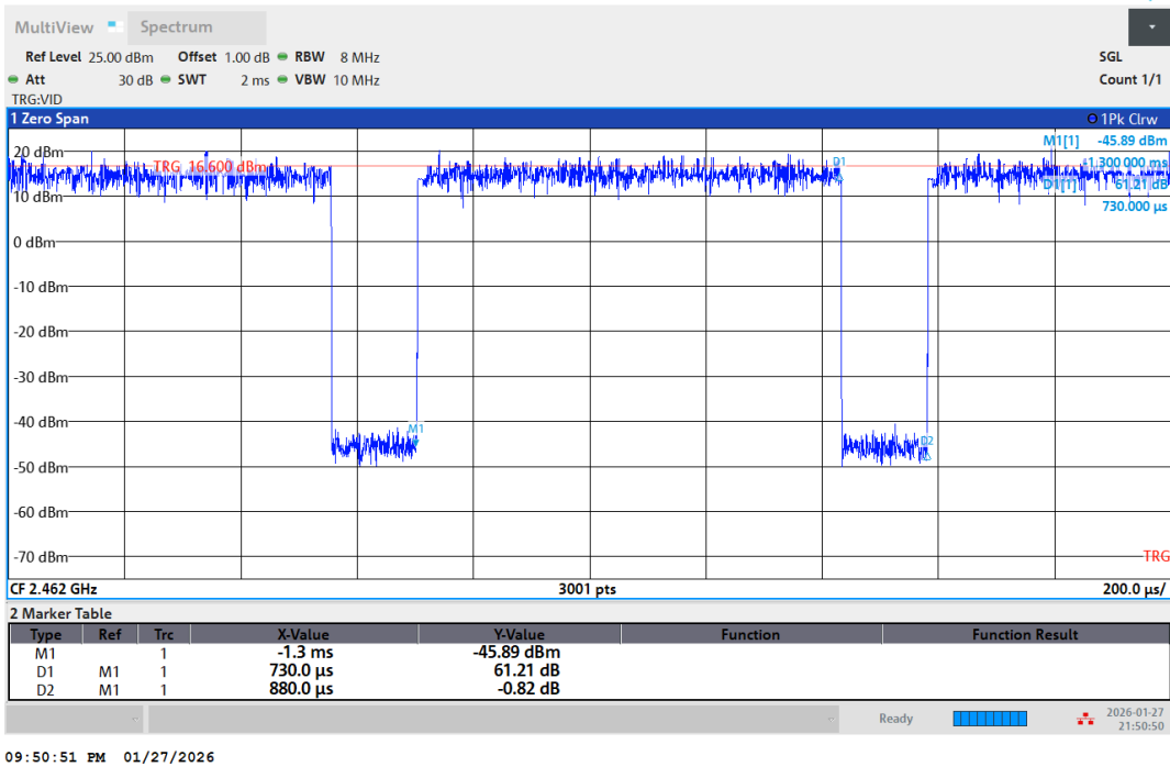
NTNV-11G-Ant1-2462
