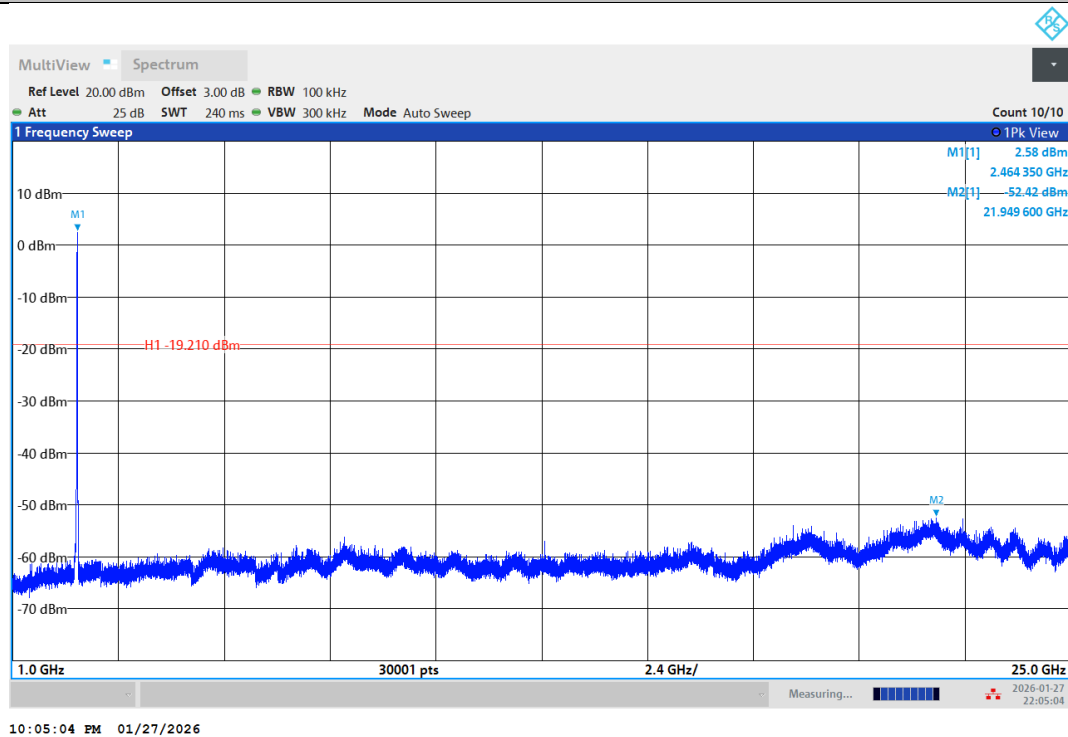
11N20SISO-Ant1-2462-1000~25000-PASS
