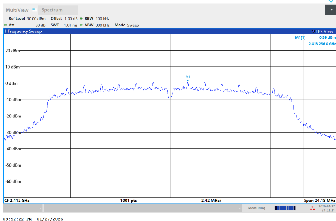
11N20SISO-Ant1-2412-PASS
