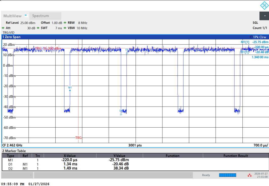
NTNV-11N20SISO-Ant1-2462
