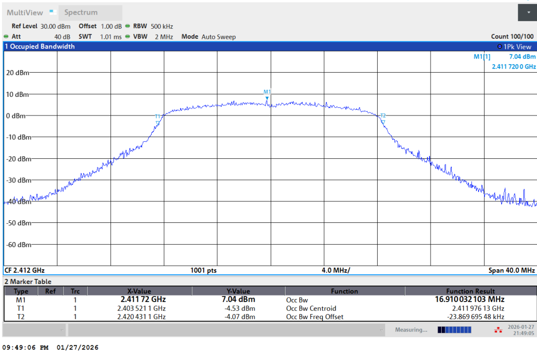
11G-Ant1-2412
