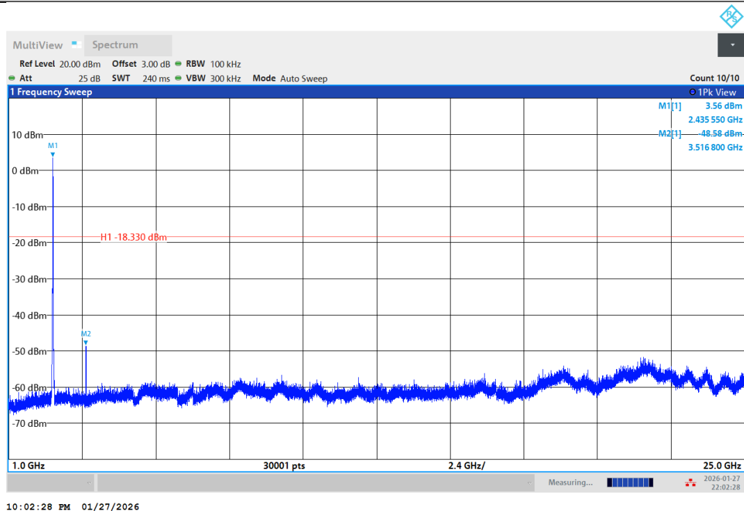
11G-Ant1-2437-1000~25000-PASS
