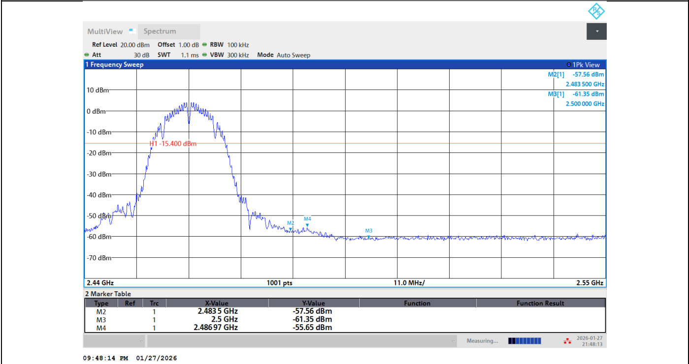
11B-Ant1-2462-PASS
