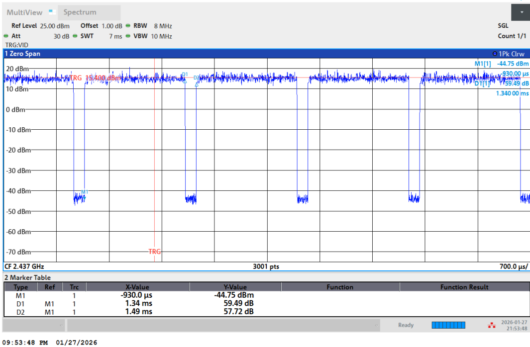
NTNV-11N20SISO-Ant1-2437
