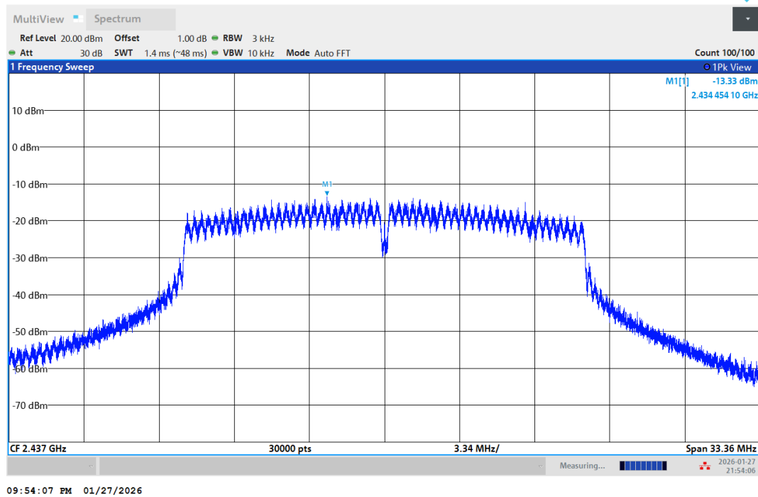
11N20SISO-Ant1-2437-PASS
