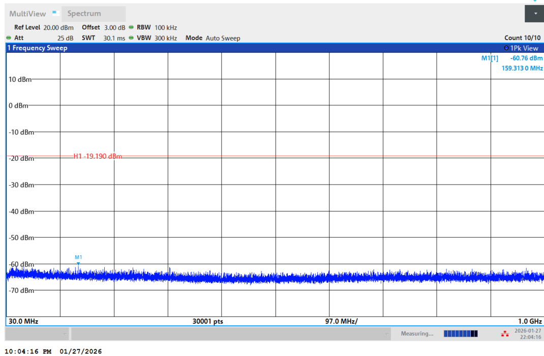
11N20SISO-Ant1-2437-30~1000-PASS
