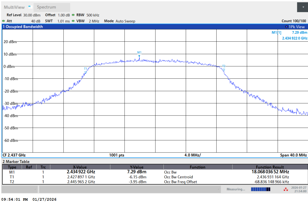
11N20SISO-Ant1-2437
