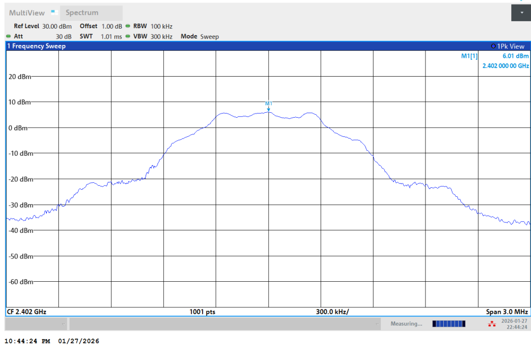
BLE_1M-Ant1-2402-PASS
