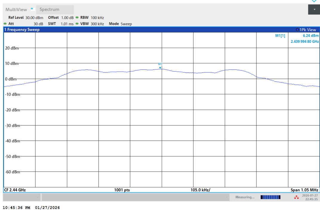
BLE_1M-Ant1-2440-PASS
