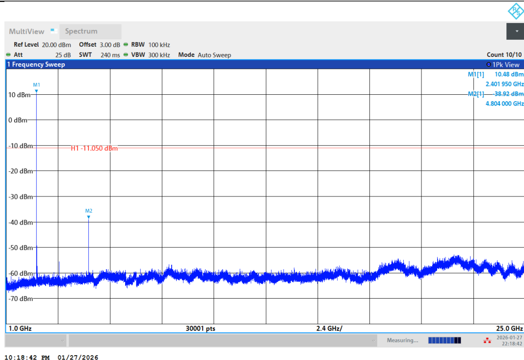
DH5-Ant1-2402-1000~25000-PASS
