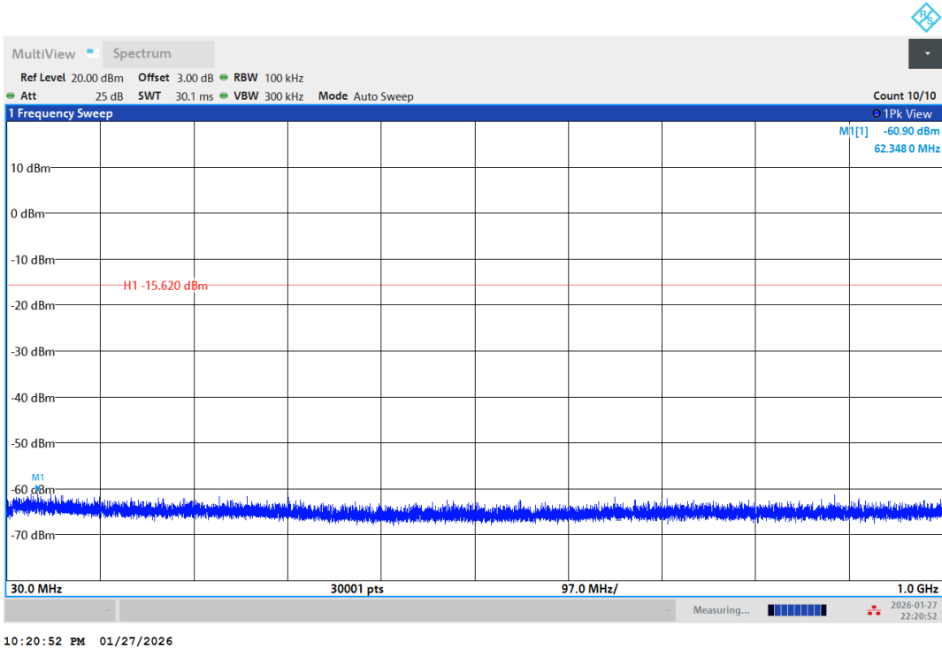
2DH5-Ant1-2402-30~1000-PASS
