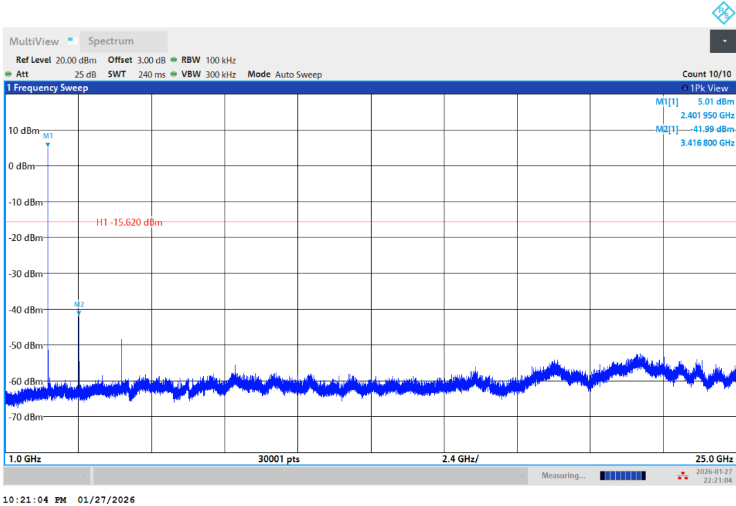
2DH5-Ant1-2402-1000~25000-PASS
