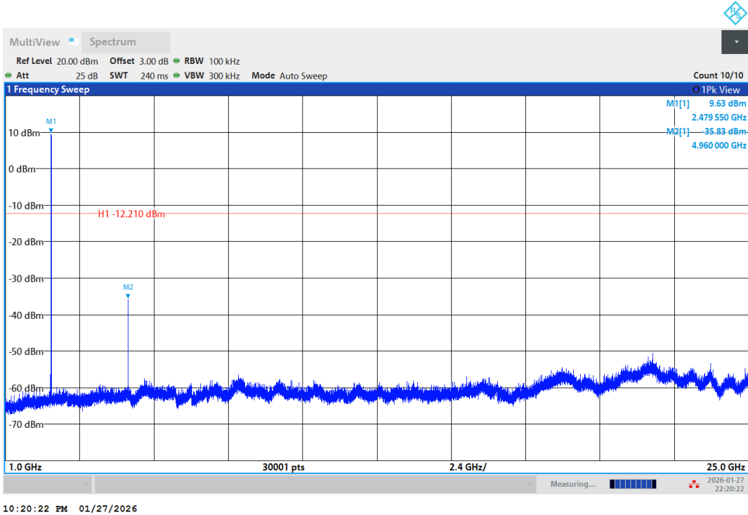
DH5-Ant1-2480-1000~25000-PASS
