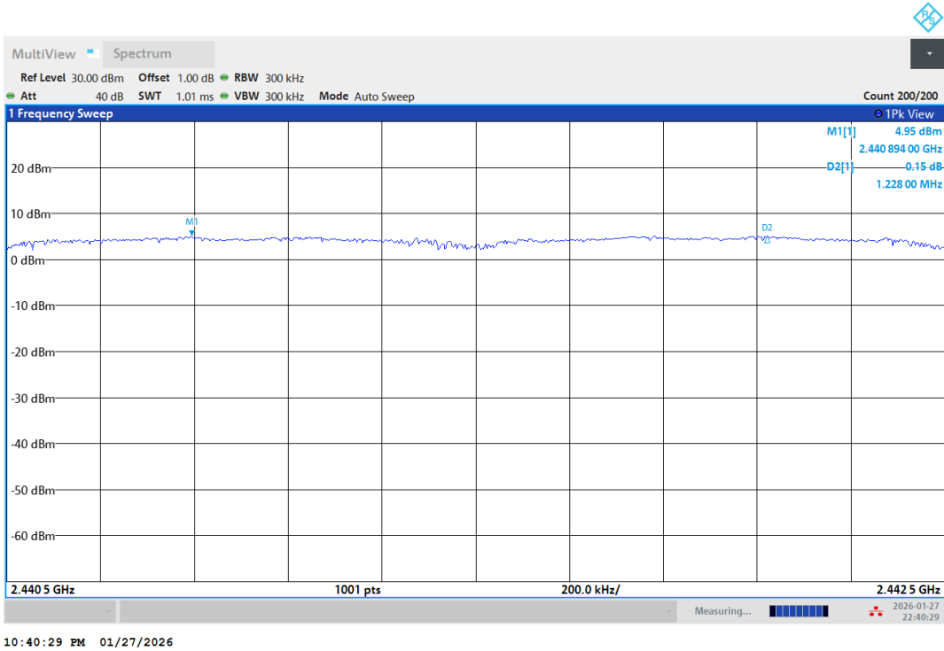
2DH5-Ant1-Hop-PASS
