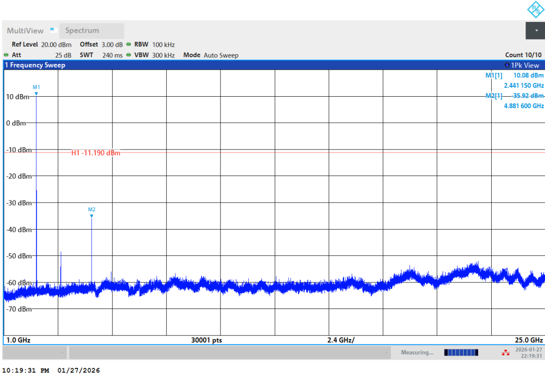
DH5-Ant1-2441-1000~25000-PASS
