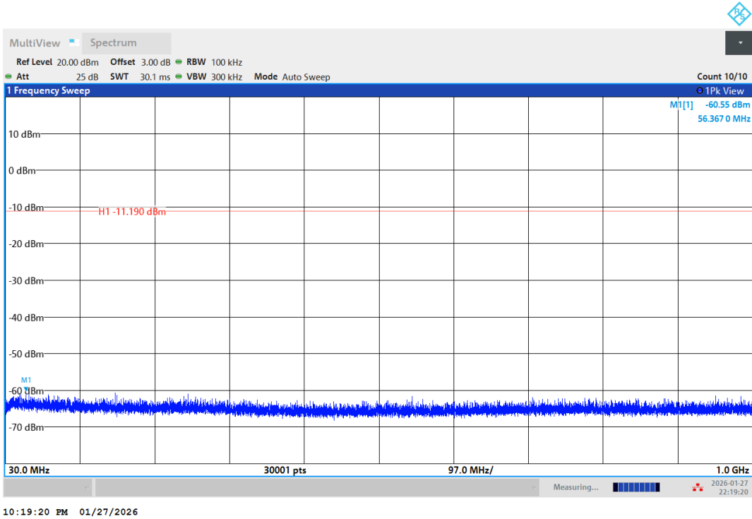
DH5-Ant1-2441-30~1000-PASS
