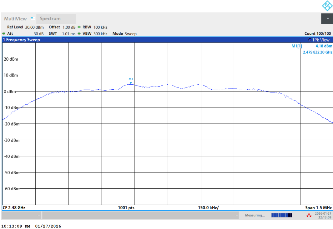
2DH5-Ant1-2480-PASS
