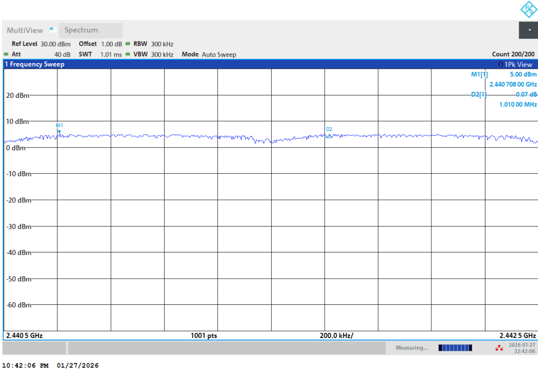
3DH5-Ant1-Hop-PASS
