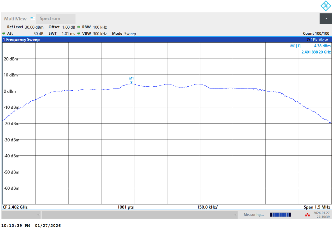
2DH5-Ant1-2402-PASS
