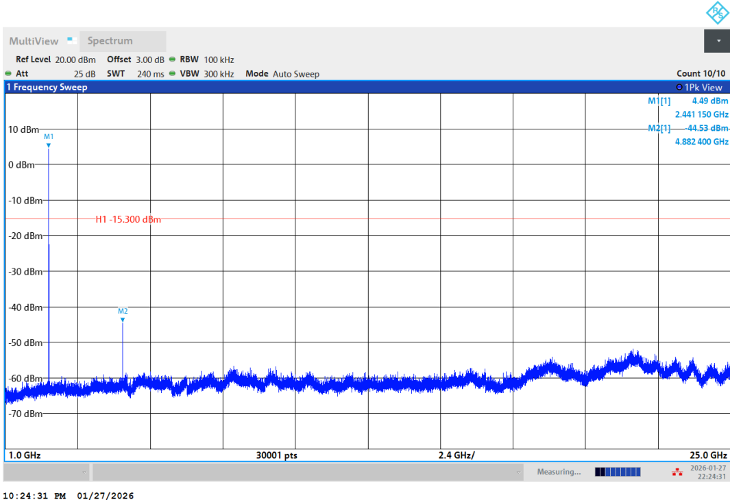
3DH5-Ant1-2441-1000~25000-PASS
