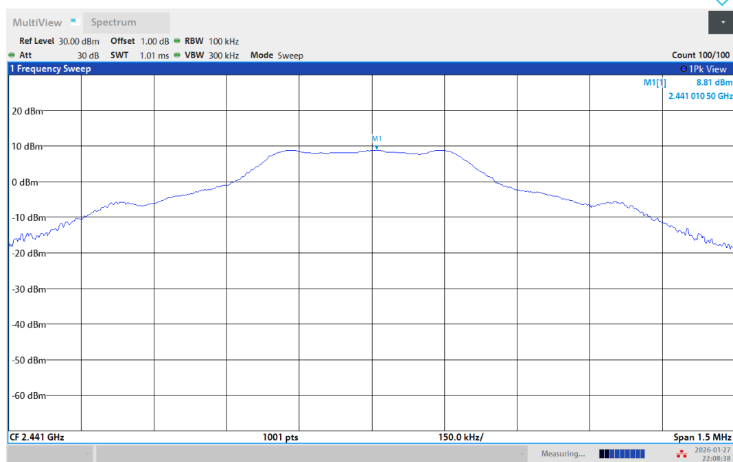
DH5-Ant1-2441-PASS
