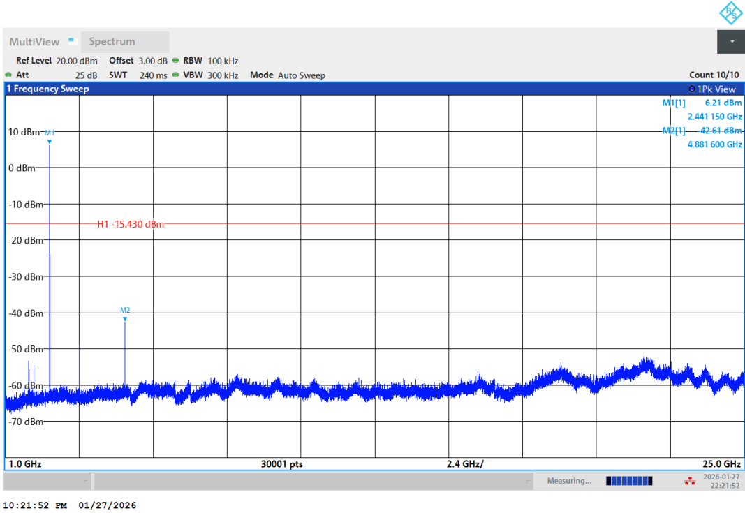
2DH5-Ant1-2441-1000~25000-PASS
