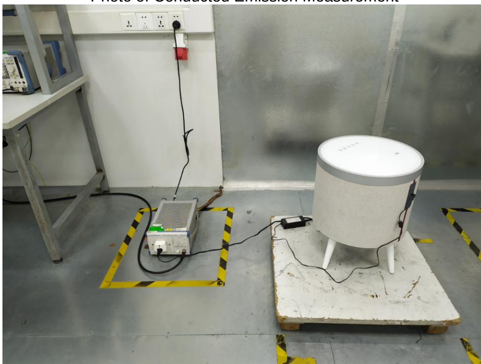
FCC ID: 2AWWQ-KBBM1111 Photo of Conducted Emission Measurement
