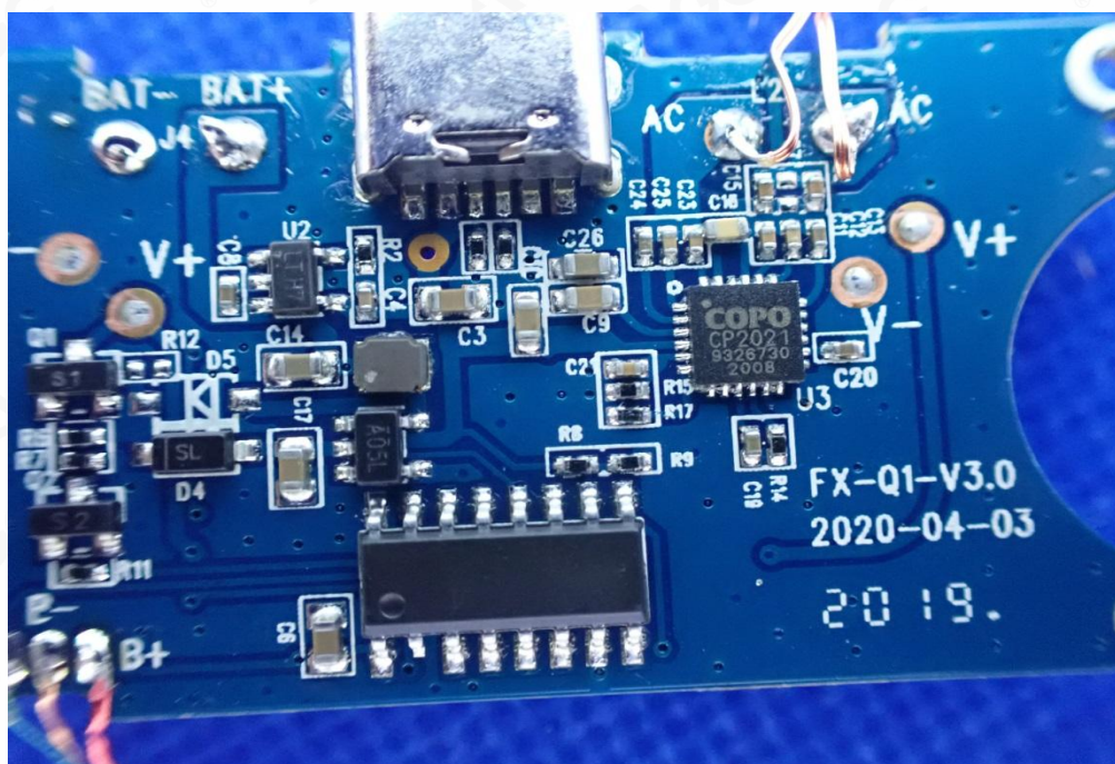
INTERNAL VIEW-6 OF Charging case
