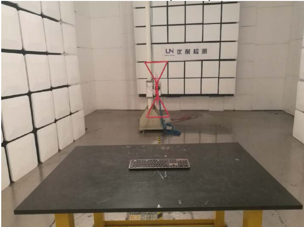
Radiated Emission (Below 1G)
