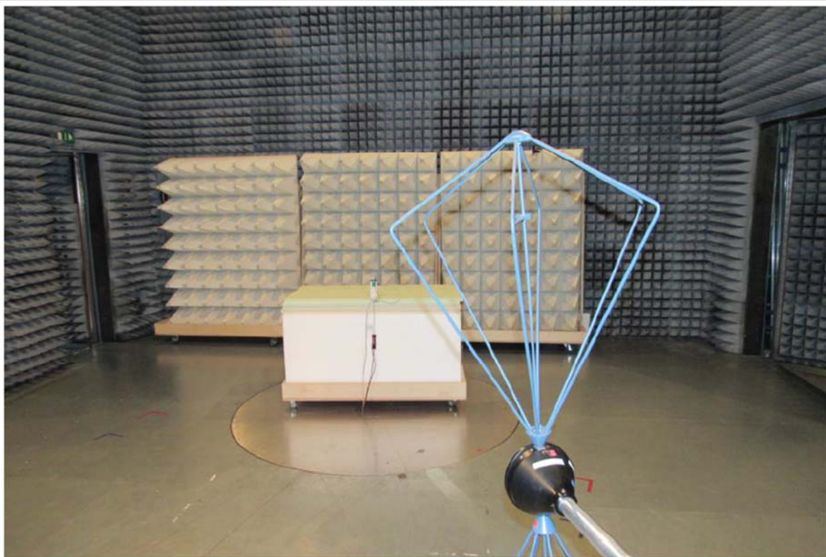
Test setup radiated below 200MHz
