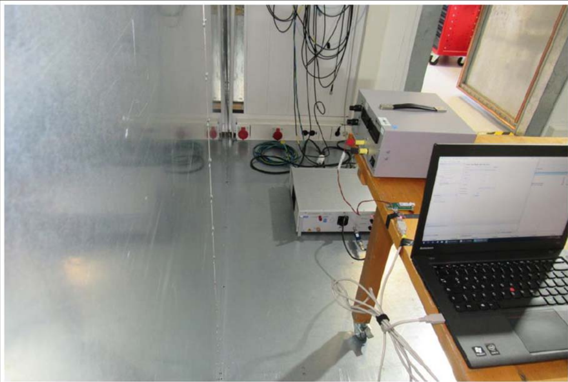
AC-Powerline Conducted Emission
