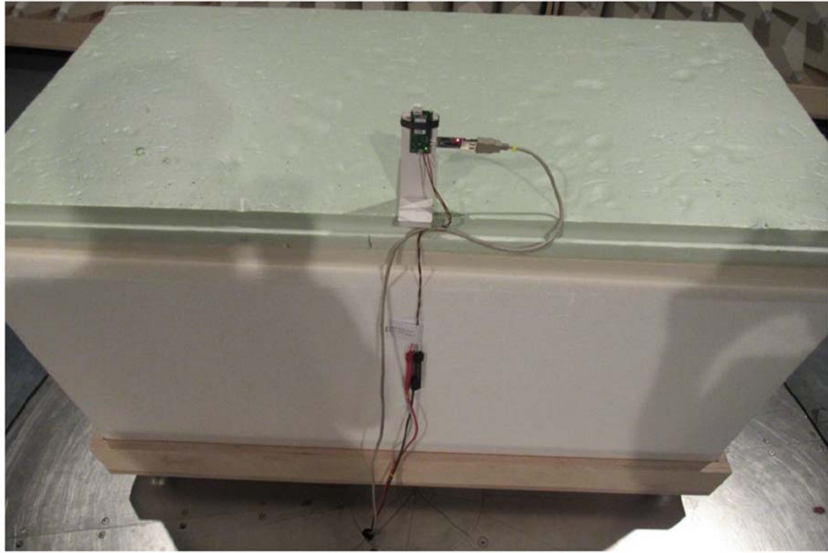
Test setup radiated EUT view
