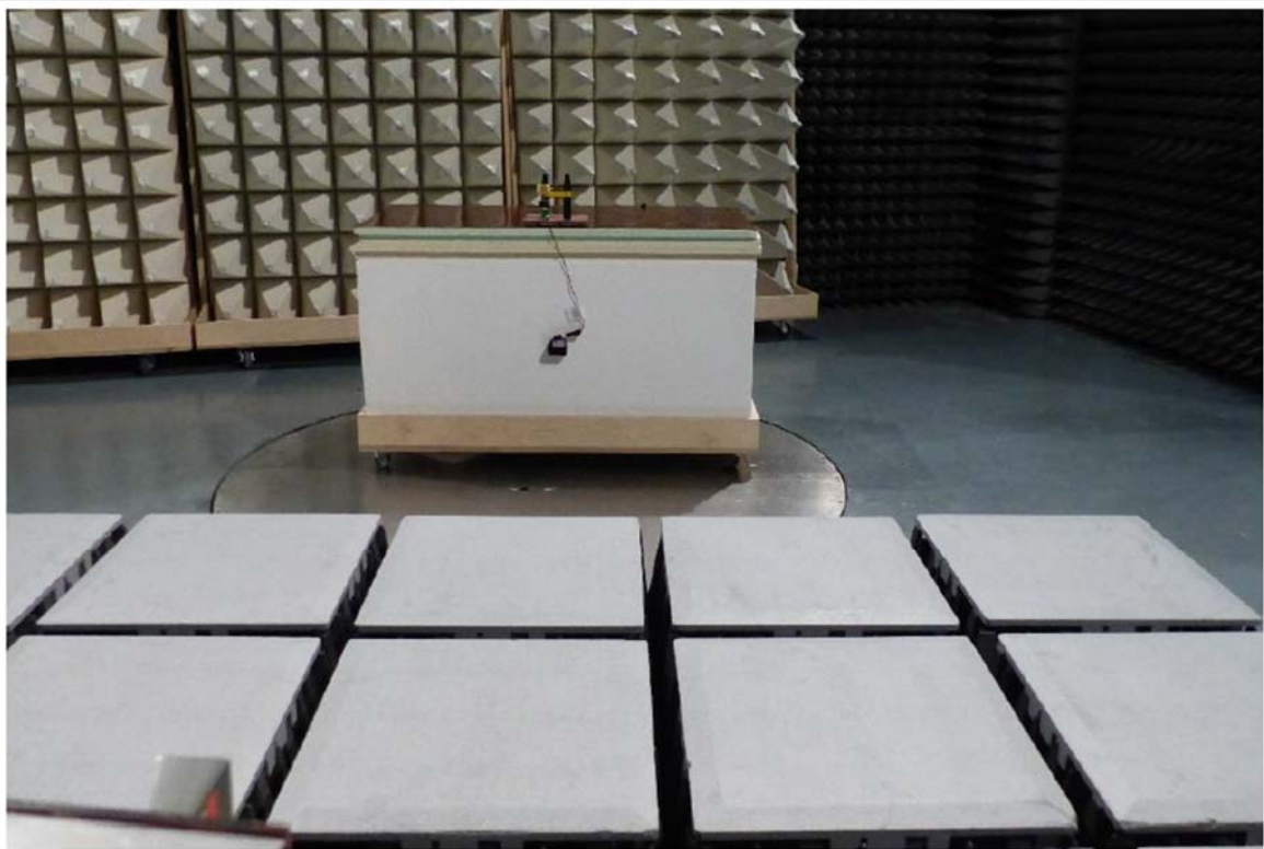
Test setup UWB 17-26.5GHz
