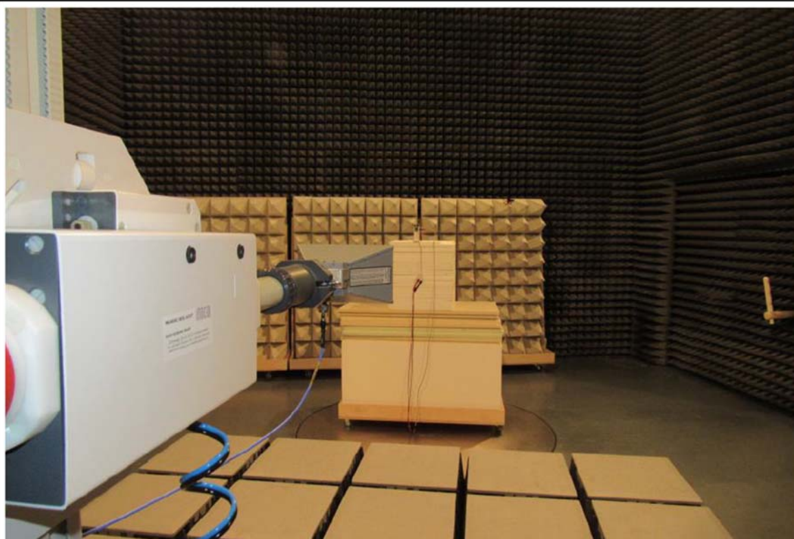
Test setup between 1 GHz and 17 GHz
