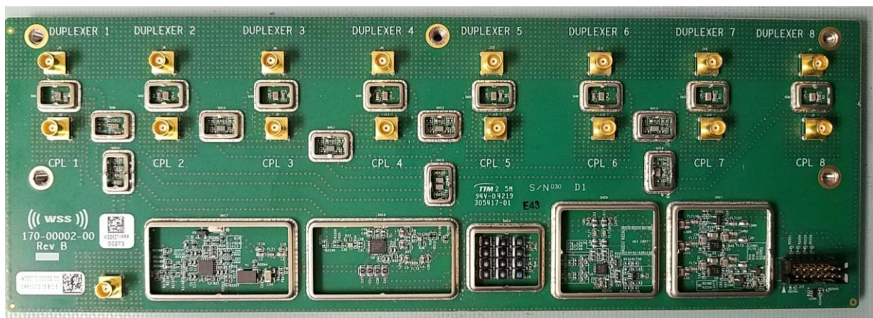
Figure 5 - RRH Phase Cal board (02 Board) Top view, Cut
