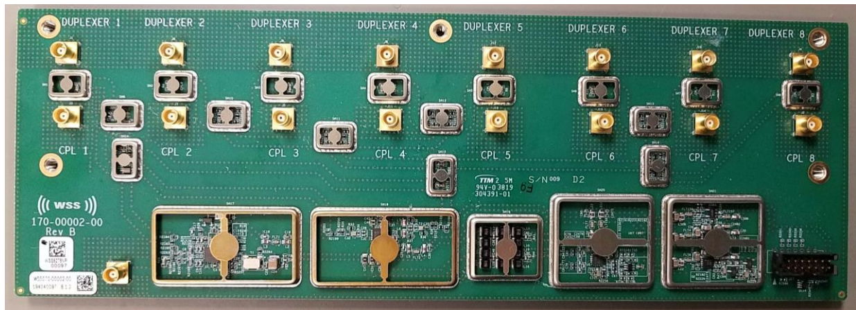
Figure 4 - RRH Phase Cal board (02 Board) Top view
