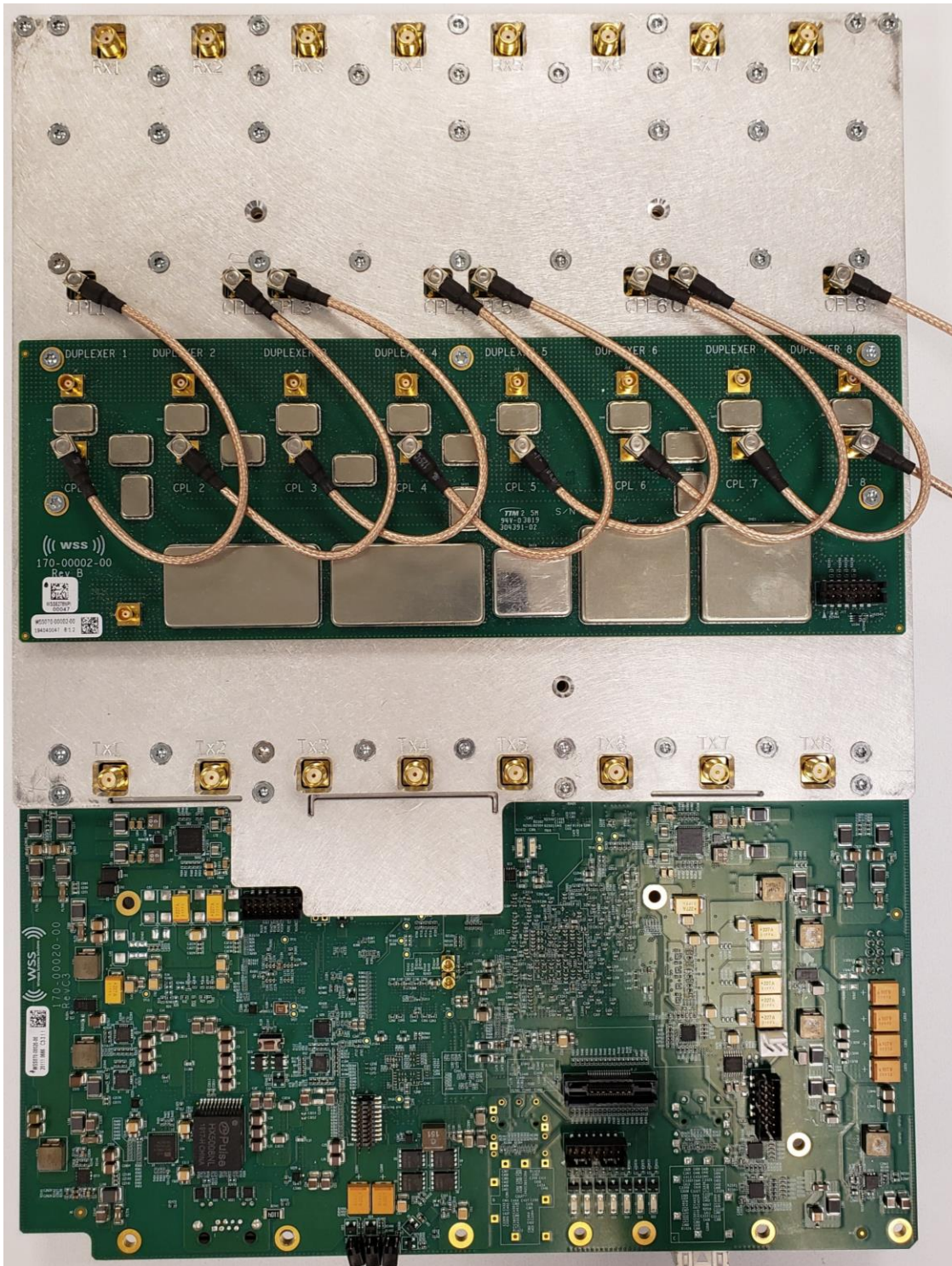
Figure 7 - RRH RF and Phase Cal board (02 Board)
