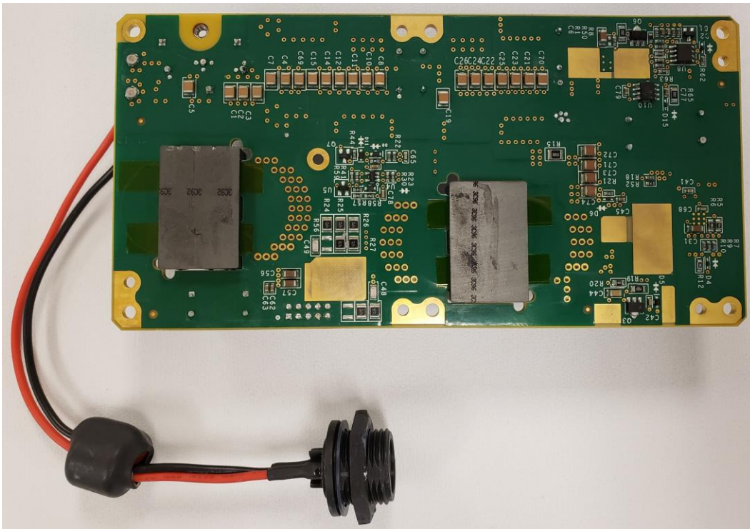
Figure 8 – Power Supply board Top view
