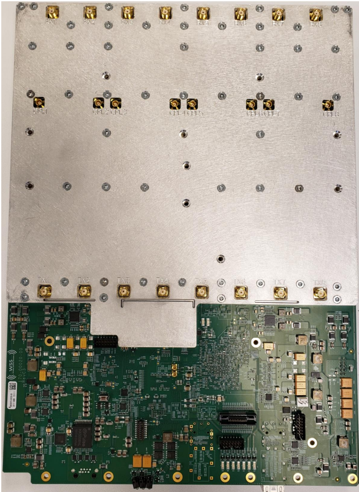
Figure 3 - RRH RF board (20 Board) Top view with shield and heaters
