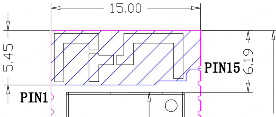
Antenna size diagram
