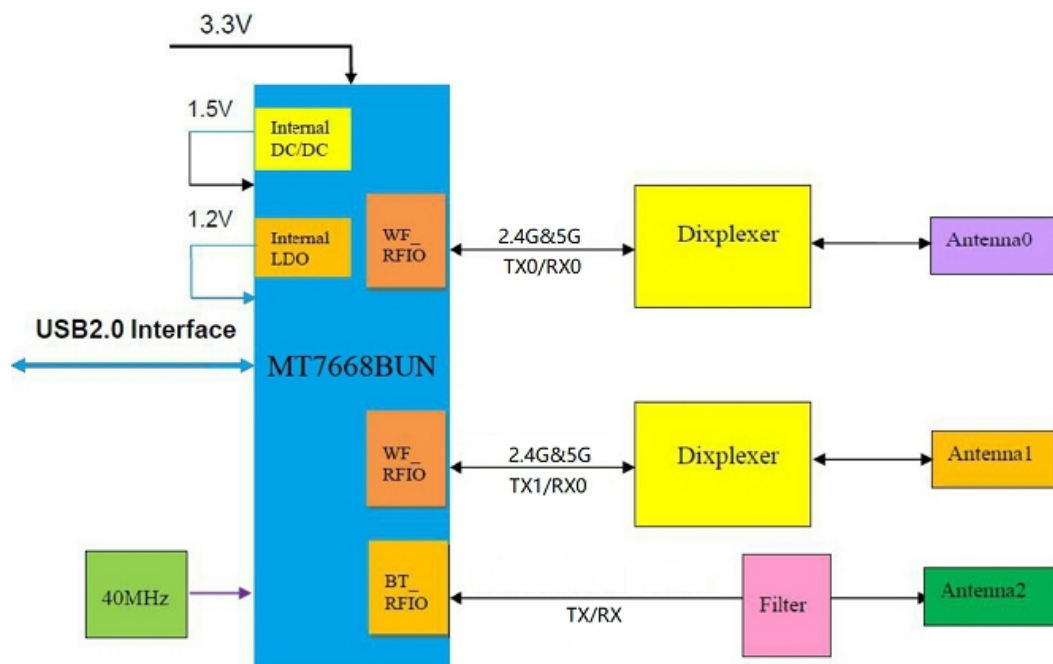
Figure 1 EL.MT7668BUN-WF Block Diagram
