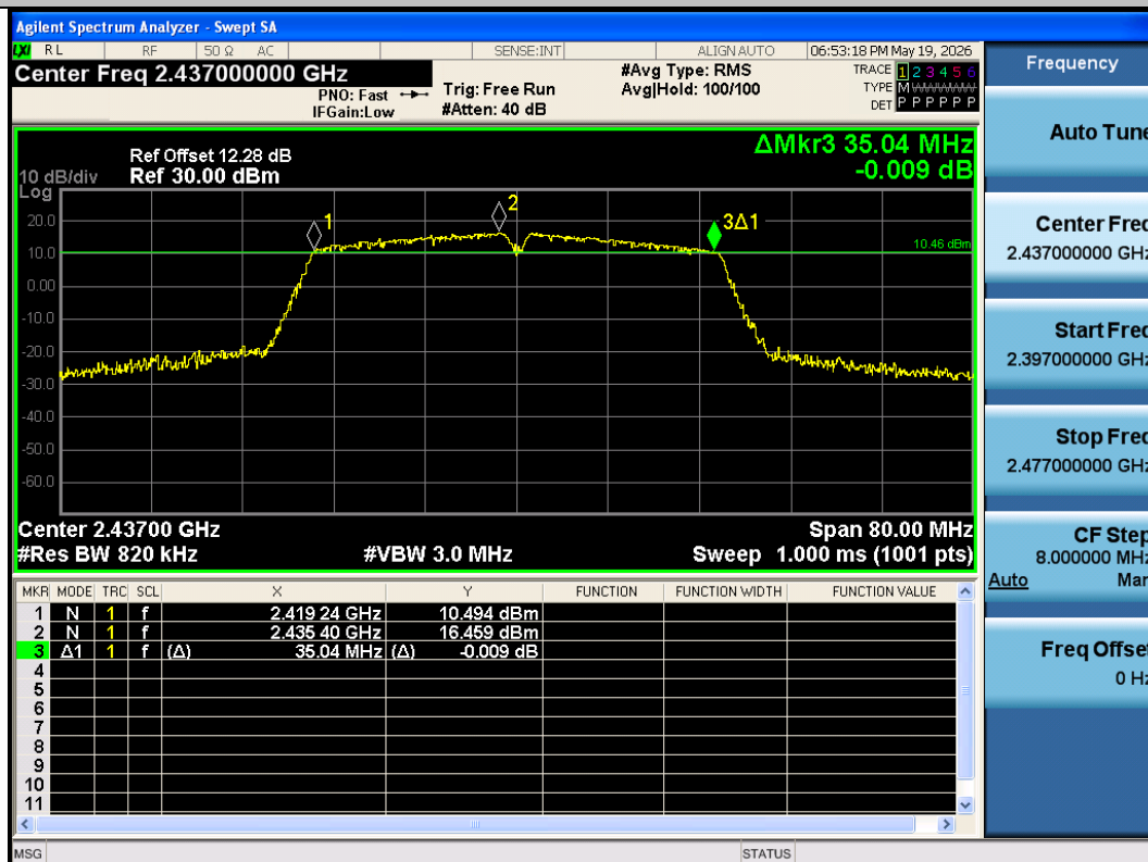
11N40SISO-Ant1-2437-PASS
