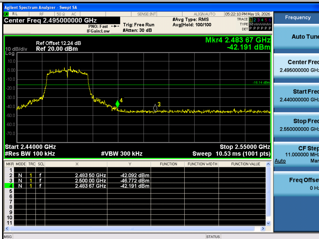
11N20SISO-Ant1-2462-PASS
