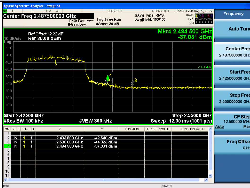
11N40SISO-Ant1-2452-PASS
