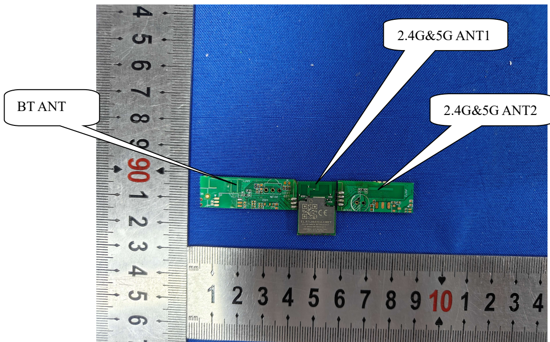
BT ANT and 2.4G/5G ATN 2 Parts used trace design.
