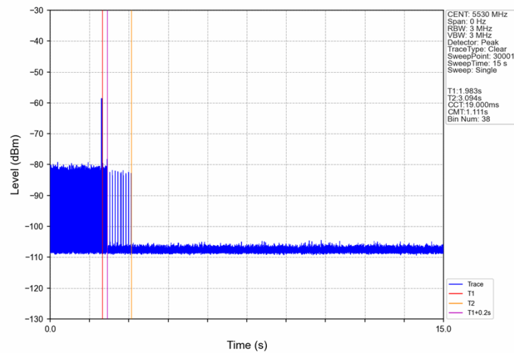
Channel Move Time and Closing Transmission Time_802.11ac(VHT80)_5530MHz
