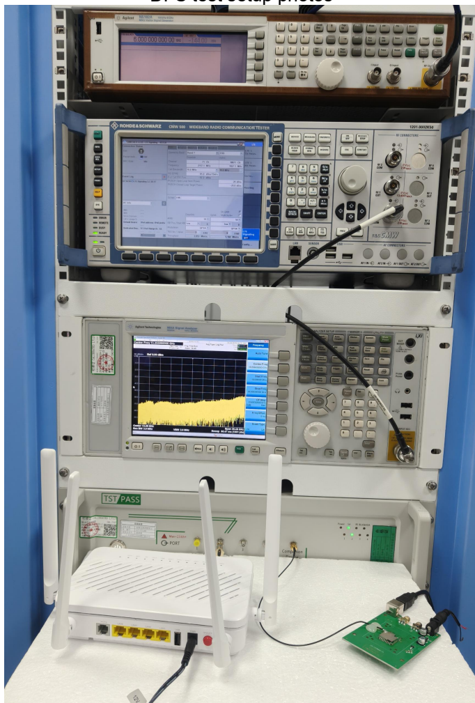
DFS test setup photos
