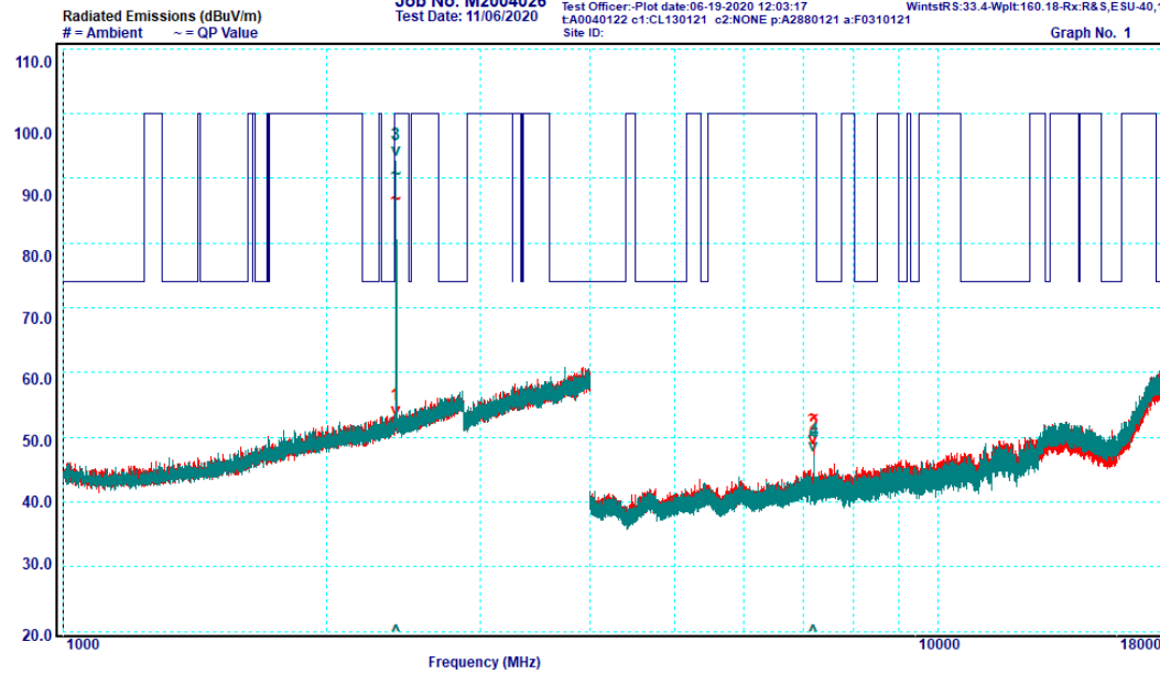
Graph 6-14: Transmitter Spurious Emissions, 1 – 18 GHz, Low Channel 2402 MHz, Peak
