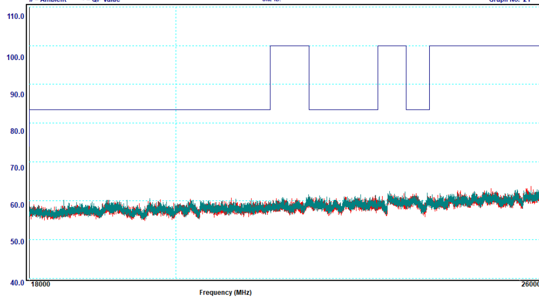
Graph 6-21: Transmitter Spurious Emissions, 18 – 26 GHz, 2440 MHz, Peak
