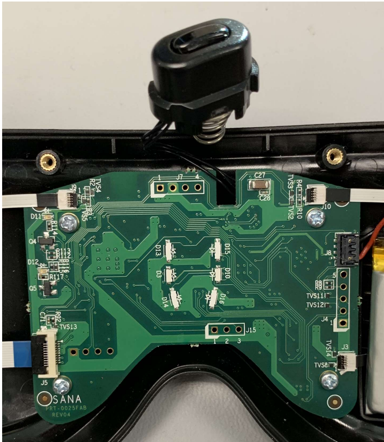
PRT-0025 Main PCBA (top)
