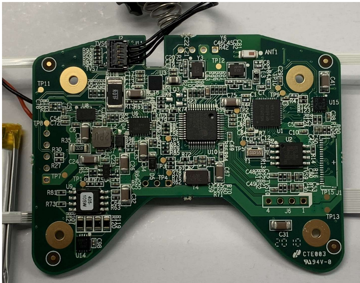
PRT-0026 Power Switch PCBA
