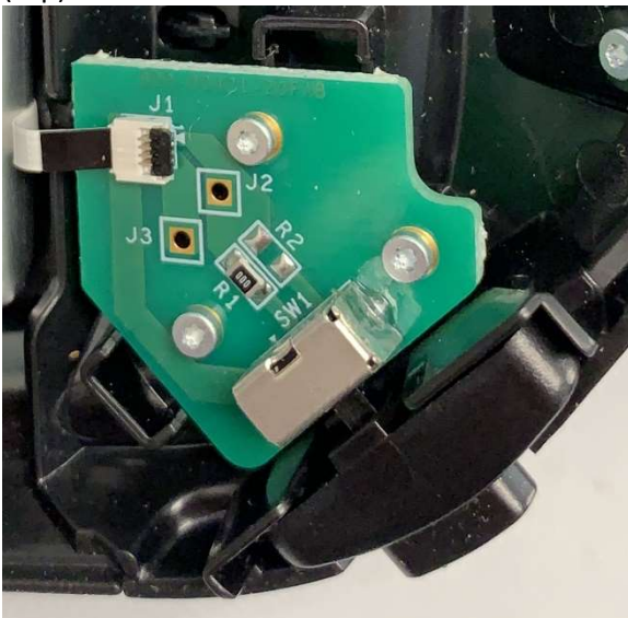
PRT-0026 Power Switch PCBA
