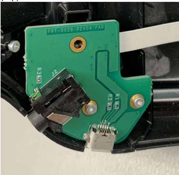
PRT-0028 Connector PCBA (top)
