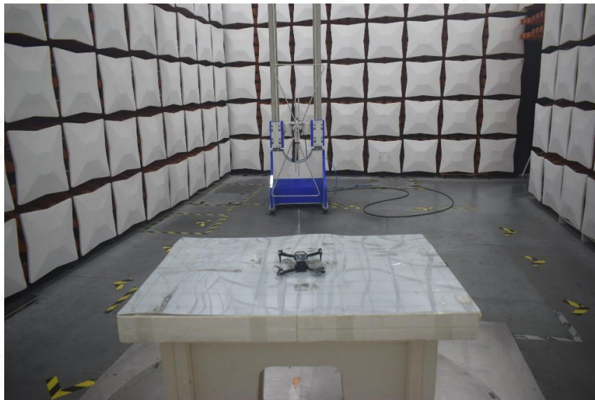
TX 30MHz~1GHz
