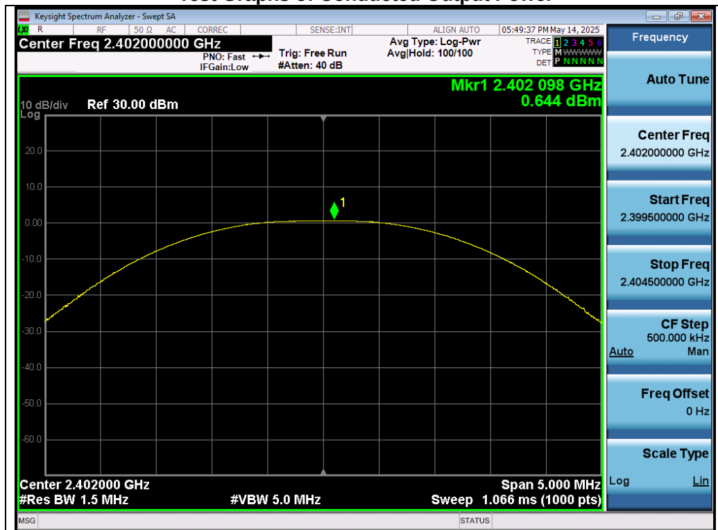
Test_Graph_2.4G_ANT1_2402_1Mbps_Peak Power
