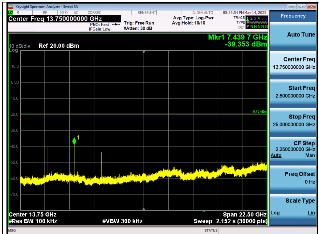
Test_Graph_2.4G_ANT1_2480_1Mbps_Higher Band Emissions
