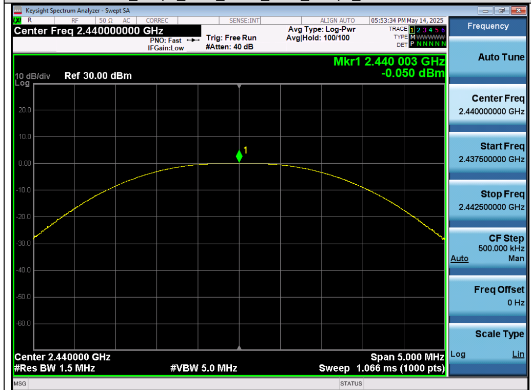
Test_Graph_2.4G_ANT1_2440_1Mbps_Peak Power
