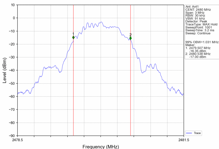
1M_HCH_2480MHz_Ant1_NTNV
