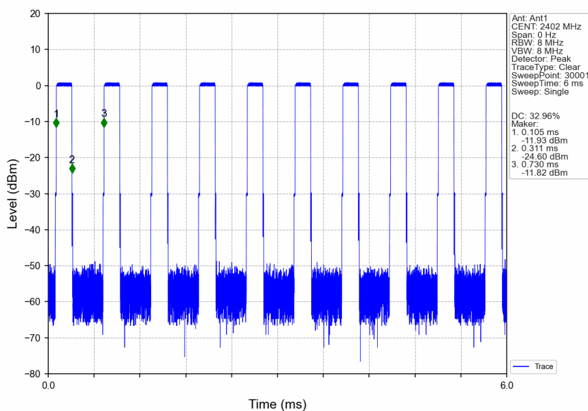
2M_LCH_2402MHz_Ant1_NTNV
