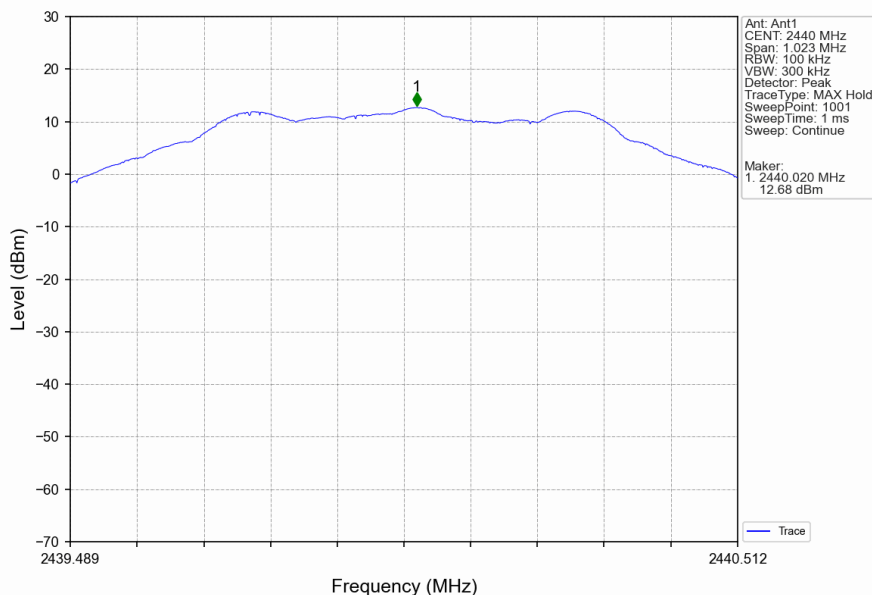
1M_MCH_2440MHz_Ant1_NTNV
