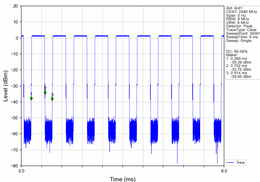
1M_HCH_2480MHz_Ant1_NTNV
