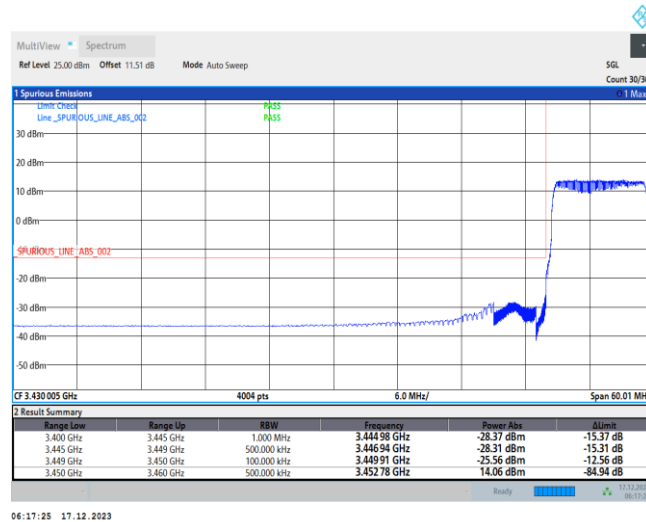
1-N78-3450-3550-PC2-30-10-L-3-DFT-PI2BPSK-Outer_Full-24@0-Ant0-1--PASS-see graph
