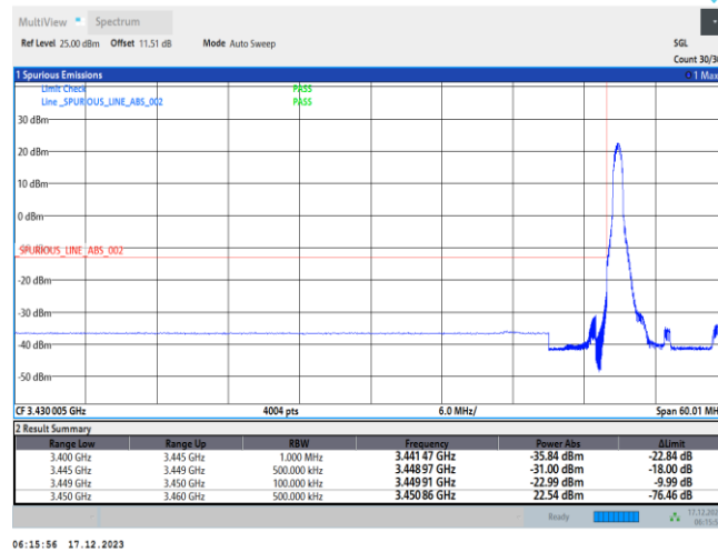
1-N78-3450-3550-PC2-30-10-L-1-DFT-PI2BPSK-Edge_1RB_Left-1@0-Ant0-1--PASS-see graph
