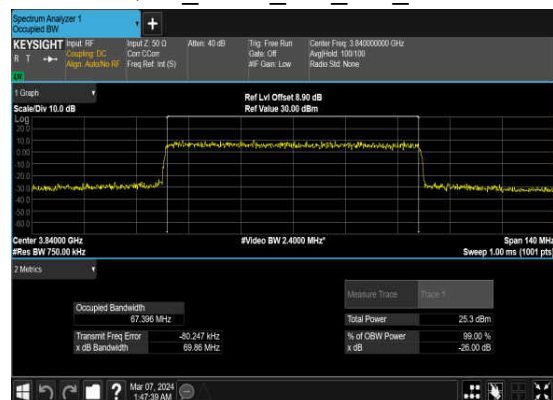
N77(70M)_CP-OFDM_16 QAM_Outer_Full_Mid_CH
