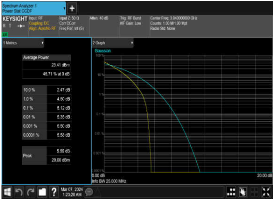
N77(20M)_DFT-s-OFDM_QPSK_Outer_Full_Mid_CH
