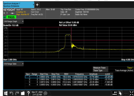
N77(10M)_DFT-s- OFDM_QPSK_Outer_Full_High_CH
