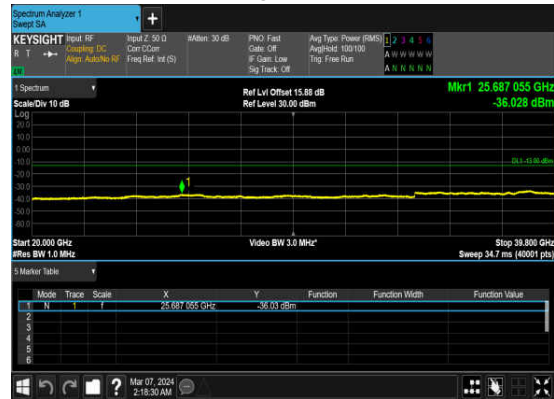
N77(50M)_DFT-s- OFDM_QPSK_Edge_1RB_Left_Mid_CH
