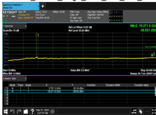
N77(100M)_DFT-s- OFDM_QPSK_Edge_1RB_Left_Mid_CH
