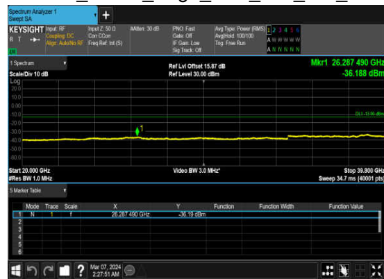
N77(100M)_DFT-s- OFDM_QPSK_Edge_1RB_Left_Mid_CH
