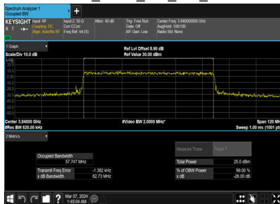
N77(60M)_CP-OFDM_64 QAM_Outer_Full_Mid_CH
