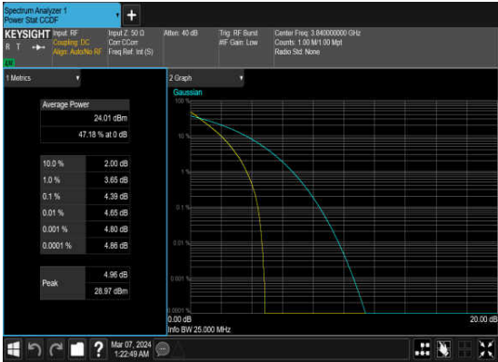
N77(20M)_DFT-s-OFDM_PI_2-BPSK_Outer_Full_Mid_CH
