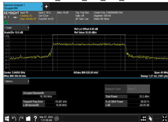
N77(20M)_CP-OFDM_256 QAM_Outer_Full_Mid_CH
