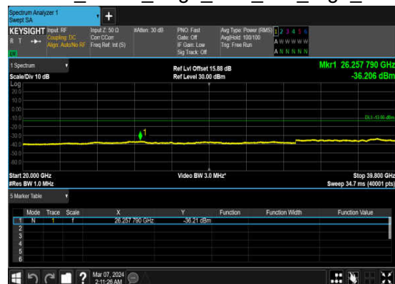
N77(10M)_DFT-s- OFDM_QPSK_Edge_1RB_Left_High_CH
