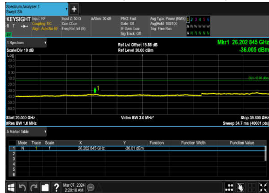
N77(50M)_DFT-s- OFDM_BPSK_Edge_1RB_Left_High_CH
