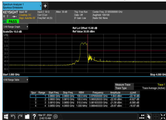
N77(10M)_DFT-s- OFDM_BPSK_Outer_Full_High_CH
