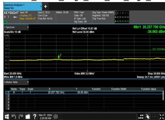
N77(100M)_DFT-s- OFDM_BPSK_Edge_1RB_Left_High_CH
