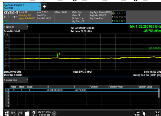
N77(50M)_DFT-s- OFDM_QPSK_Edge_1RB_Left_High_CH
