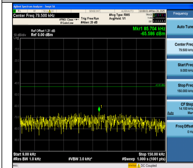
Band II-9538-0.009~0.15MHz-PASS
