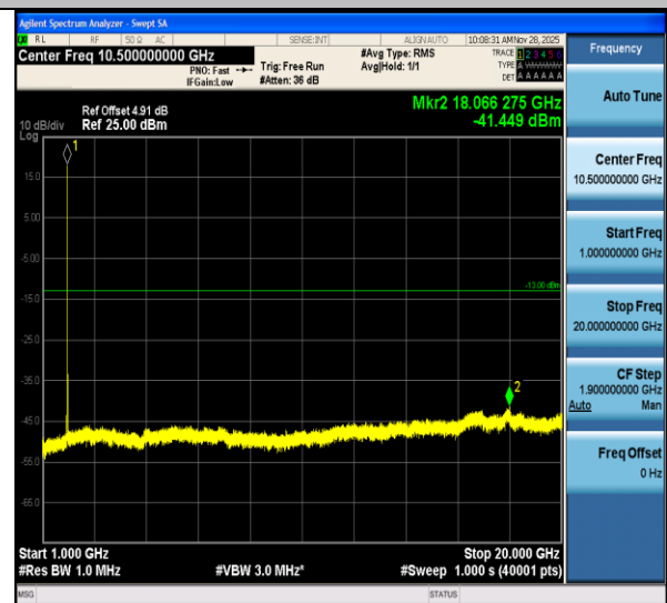
Band II-9538-1000~20000MHz-PASS
