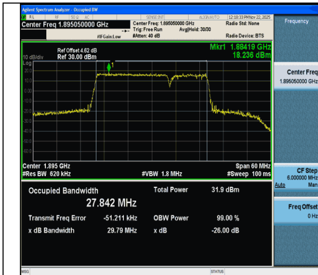
CA_2C-20MHz-10MHz-64QAM-64QAM-19001-19145-100RB#0-50RB#0-PASS
