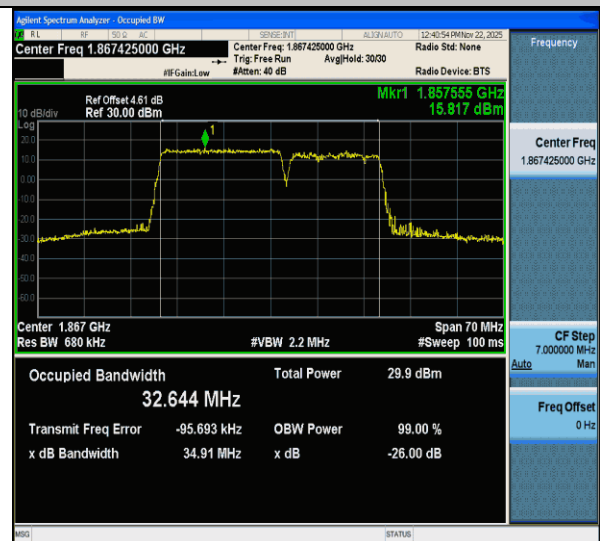
CA_2C-20MHz-15MHz-256QAM-256QAM-18700-18871-100RB#0-75RB#0-PASS
