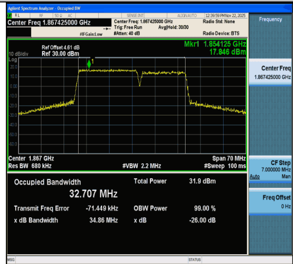
CA_2C-20MHz-15MHz-16QAM-16QAM-18700-18871-100RB#0-75RB#0-PASS
