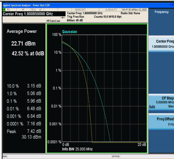
CA_2C-20MHz-5MHz-QPSK-QPSK-19050-19167-100RB#0-25RB#0-PASS
