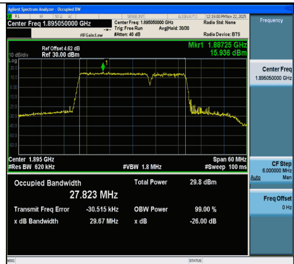
CA_2C-20MHz-10MHz-256QAM-256QAM-19001-19145-100RB#0-50RB#0-PASS
