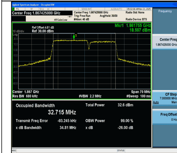
CA_2C-20MHz-15MHz-QPSK-QPSK-18700-18871-100RB#0-75RB#0-PASS
