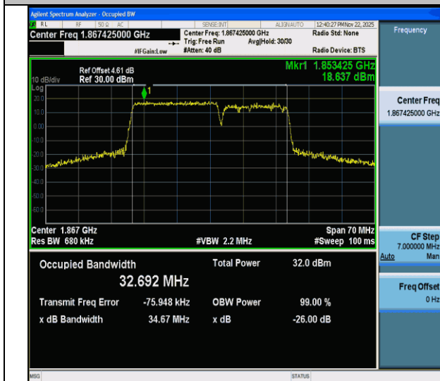
CA_2C-20MHz-15MHz-64QAM-64QAM-18700-18871-100RB#0-75RB#0-PASS
