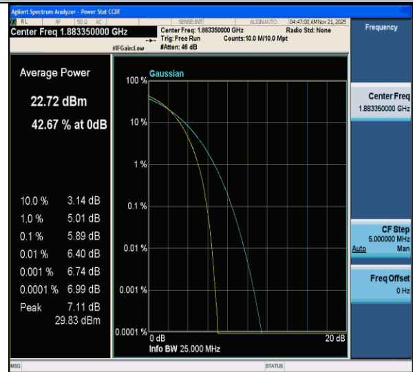
CA_2C-20MHz-5MHz-QPSK-QPSK-18875-18992-100RB#0-25RB#0-PASS
