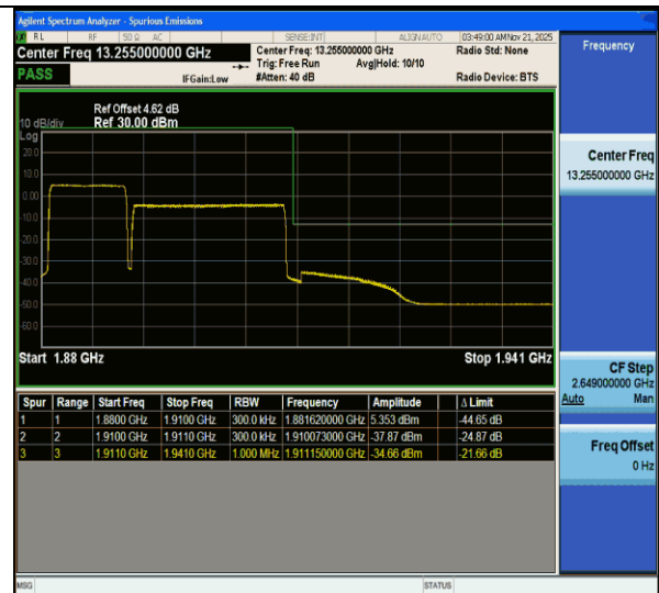
CA_2C-10MHz-20MHz-QPSK@QPSK-QPSK@QPSK-18956-19100-50RB#0@50RB#0-100RB#0@100RB#0-PASS
