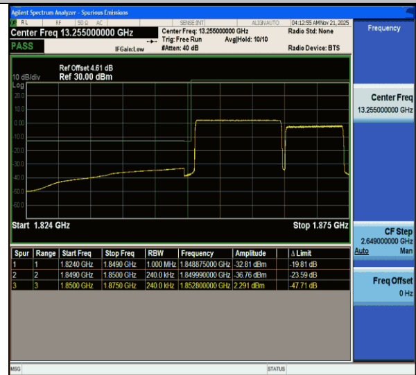
CA_2C-15MHz-10MHz-QPSK@QPSK-QPSK@QPSK-18675-18795-75RB#0@75RB#0-50RB#0@50RB#0-PASS
