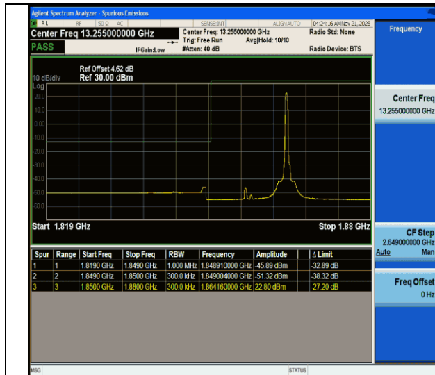
CA_2C-15MHz-15MHz-QPSK@QPSK-QPSK@QPSK-18675-18825-1RB#74@75RB#0-0RB#0@75RB#0-PASS
