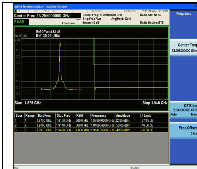
CA_2C-20MHz-15MHz-QPSK@QPSK-QPSK@QPSK-18951-19122-1RB#99@100RB#0-0RB#0@75RB#0-PASS
