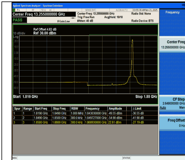
CA_2C-20MHz-10MHz-QPSK@QPSK-QPSK@QPSK-18700-18844-1RB#99@100RB#0-0RB#0@50RB#0-PASS
