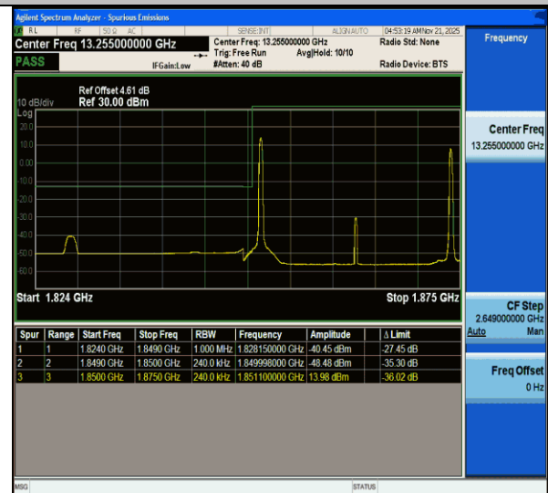
CA_2C-20MHz-5MHz-QPSK@QPSK-QPSK@QPSK-18700-18817-1RB#0@100RB#0-1RB#24@25RB#0-PASS
