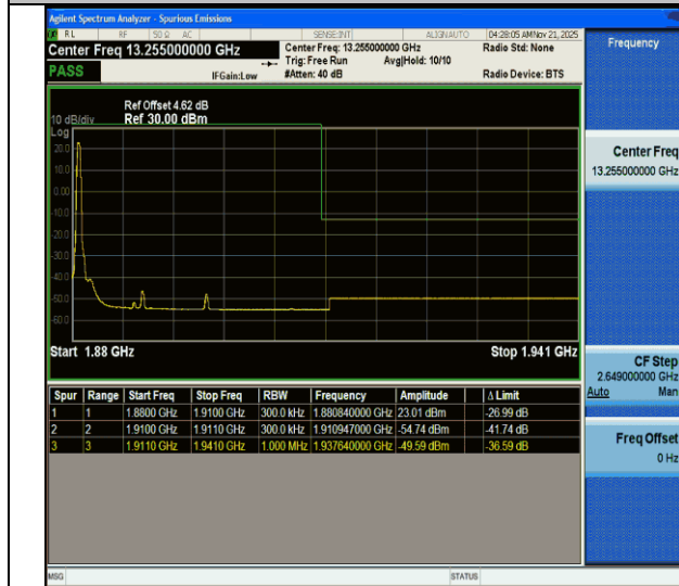
CA_2C-15MHz-15MHz-QPSK@QPSK-QPSK@QPSK-18975-19125-1RB#0@75RB#0-0RB#0@75RB#0-PASS
