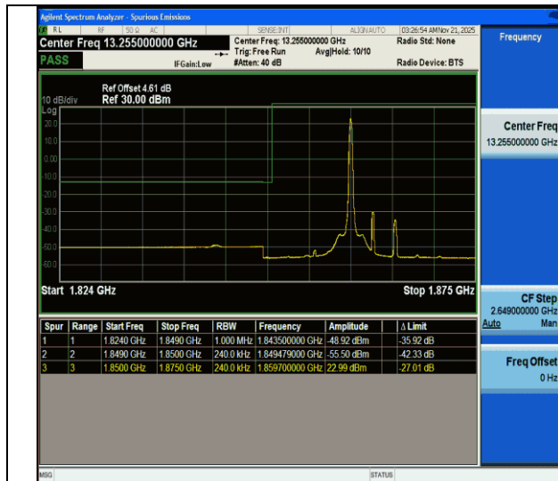
CA_2C-10MHz-15MHz-QPSK@QPSK-QPSK@QPSK-18653-18773-1RB#49@50RB#0-0RB#0@75RB#0-PASS
