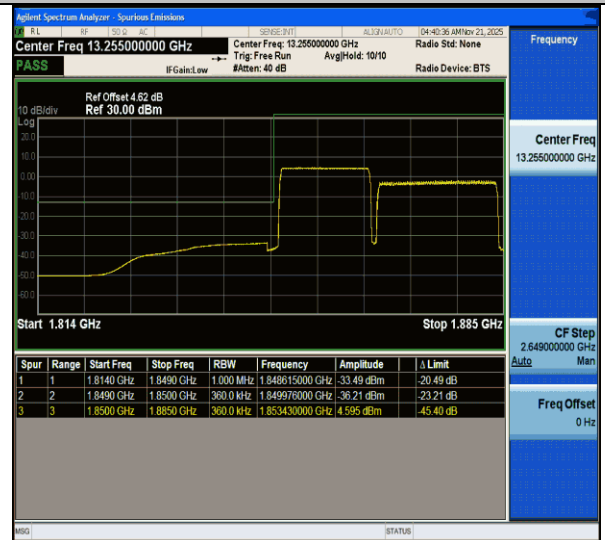
CA_2C-15MHz-20MHz-QPSK@QPSK-QPSK@QPSK-18678-18849-75RB#0@75RB#0-100RB#0@100RB#0-PASS
