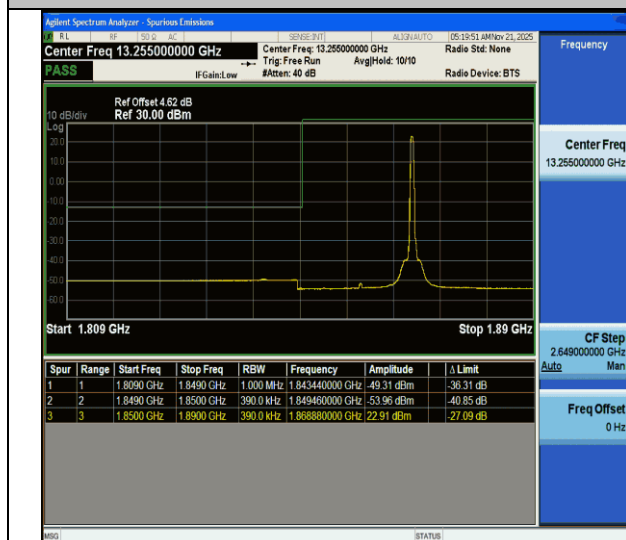
CA_2C-20MHz-20MHz-QPSK@QPSK-QPSK@QPSK-18700-18898-1RB#99@100RB#0-0RB#0@100RB#0-PASS
