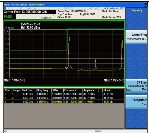
CA_2C-15MHz-20MHz-QPSK@QPSK-QPSK@QPSK-18678-18849-1RB#0@75RB#0-1RB#99@100RB#0-PASS
