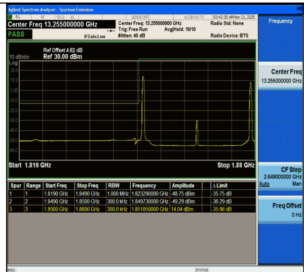
CA_2C-10MHz-20MHz-QPSK@QPSK-QPSK@QPSK-18655-18799-1RB#0@50RB#0-1RB#99@100RB#0-PASS
