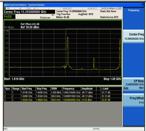
CA_2C-15MHz-15MHz-QPSK@QPSK-QPSK@QPSK-18675-18825-1RB#0@75RB#0-1RB#74@75RB#0-PASS
