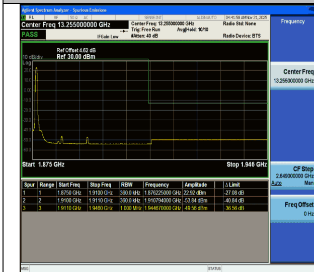
CA_2C-15MHz-20MHz-QPSK@QPSK-QPSK@QPSK-18929-19100-1RB#0@75RB#0-0RB#0@100RB#0-PASS
