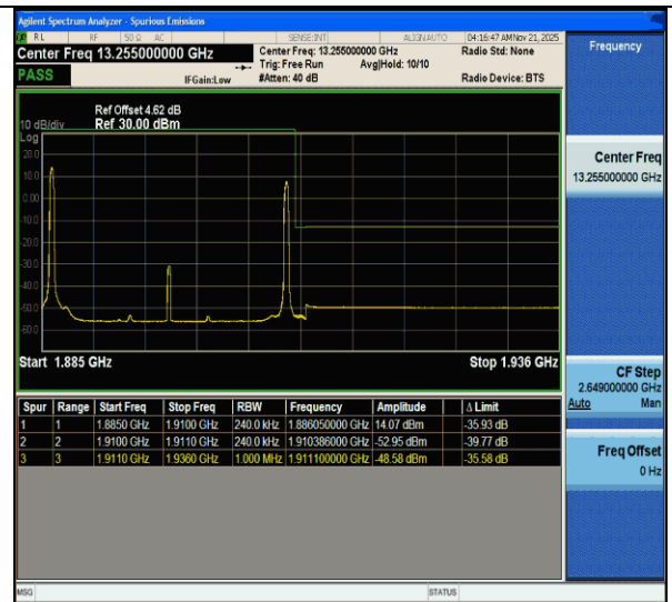
CA_2C-15MHz-10MHz-QPSK@QPSK-QPSK@QPSK-19027-19147-1RB#0@75RB#0-1RB#49@50RB#0-PASS
