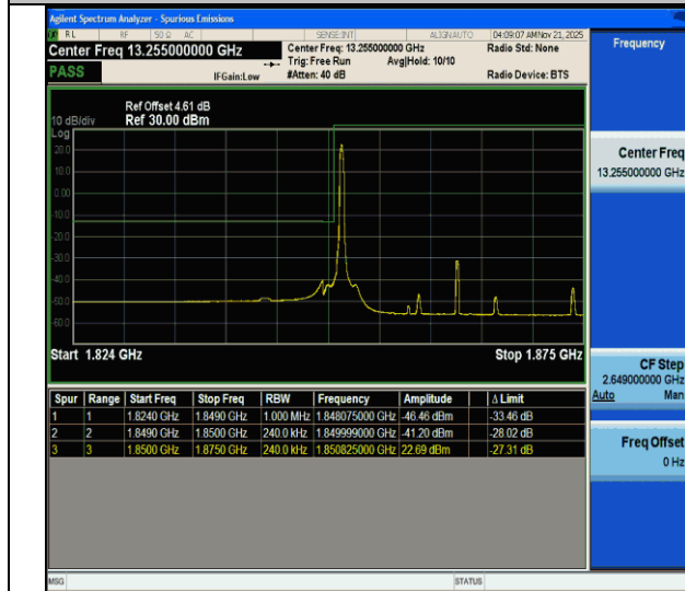
CA_2C-15MHz-10MHz-QPSK@QPSK-QPSK@QPSK-18675-18795-1RB#0@75RB#0-0RB#0@50RB#0-PASS
