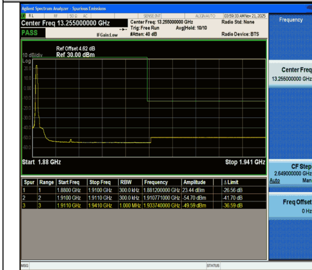
CA_2C-20MHz-10MHz-QPSK@QPSK-QPSK@QPSK-19001-19145-1RB#0@100RB#0-0RB#0@50RB#0-PASS
