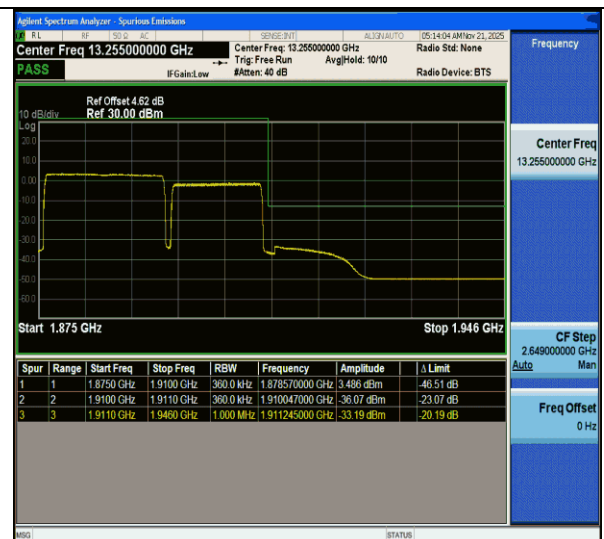
CA_2C-20MHz-15MHz-QPSK@QPSK-QPSK@QPSK-18951-19122-100RB#0@100RB#0-75RB#0@75RB#0-PASS
