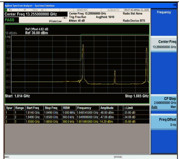
CA_2C-20MHz-15MHz-QPSK@QPSK-QPSK@QPSK-18700-18871-1RB#0@100RB#0-1RB#74@75RB#0-PASS
