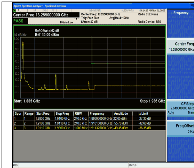
CA_2C-15MHz-10MHz-QPSK@QPSK-QPSK@QPSK-19027-19147-1RB#0@75RB#0-0RB#0@50RB#0-PASS
