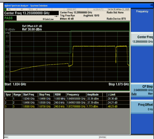
CA_2C-20MHz-5MHz-QPSK@QPSK-QPSK@QPSK-18700-18817-100RB#0@100RB#0-25RB#0@25RB#0-PASS
