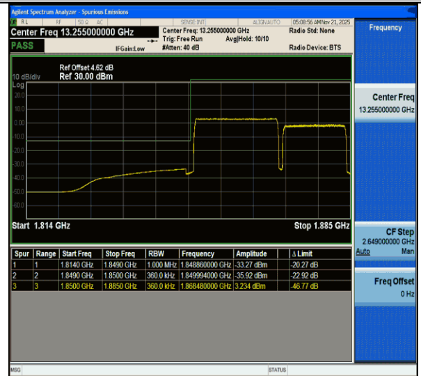
CA_2C-20MHz-15MHz-QPSK@QPSK-QPSK@QPSK-18700-18871-100RB#0@100RB#0-75RB#0@75RB#0-PASS
