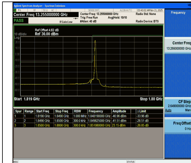
CA_2C-10MHz-20MHz-QPSK@QPSK-QPSK@QPSK-18655-18799-1RB#0@50RB#0-0RB#0@100RB#0-PASS
