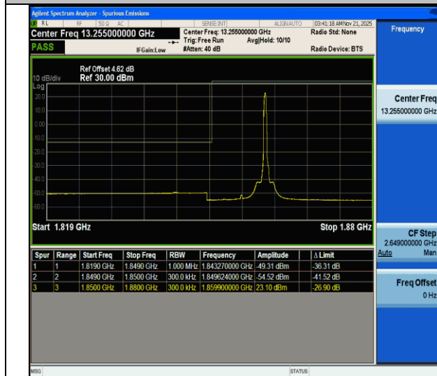
CA_2C-10MHz-20MHz-QPSK@QPSK-QPSK@QPSK-18655-18799-1RB#49@50RB#0-0RB#0@100RB#0-PASS
