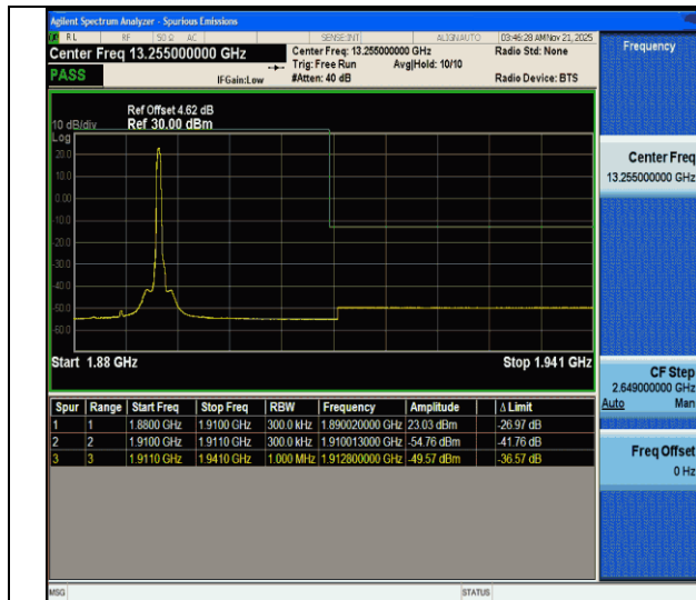
CA_2C-10MHz-20MHz-QPSK@QPSK-QPSK@QPSK-18956-19100-1RB#49@50RB#0-0RB#0@100RB#0-PASS
