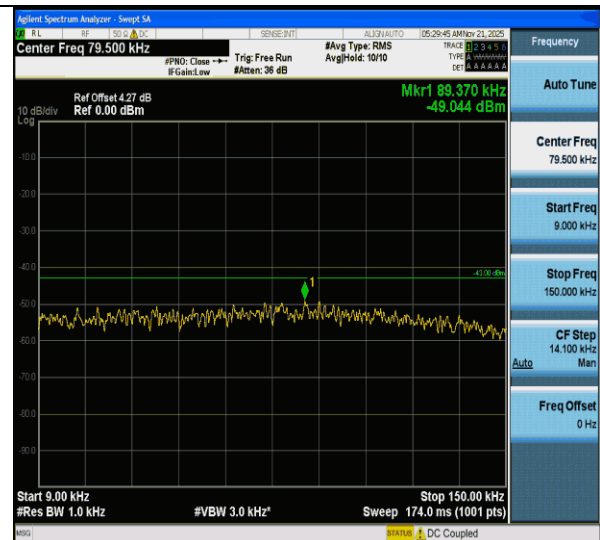
CA_2C-20MHz-20MHz-QPSK-QPSK-18801-18999-1RB#0- ORB#0-0.009~0.15MHz-PASS
