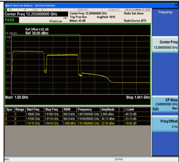
CA_2C-15MHz-15MHz-QPSK@QPSK-QPSK@QPSK-18975-19125-75RB#0@75RB#0-75RB#0@75RB#0-PASS
