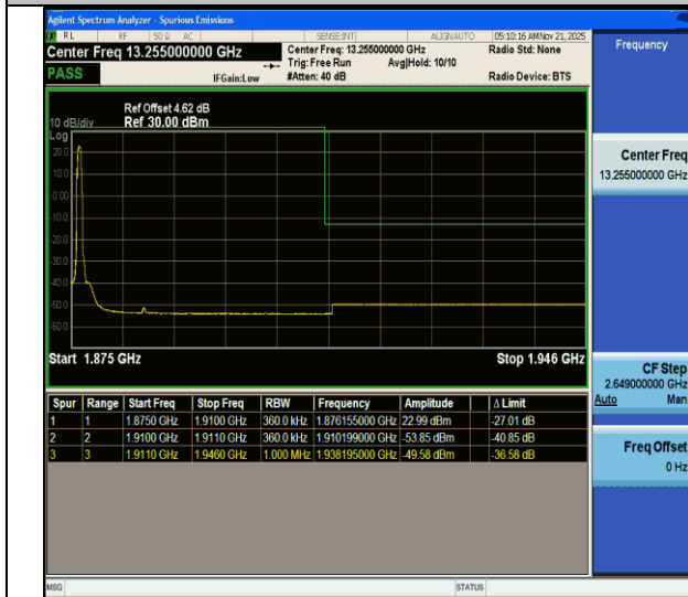
CA_2C-20MHz-15MHz-QPSK@QPSK-QPSK@QPSK-18951-19122-1RB#0@100RB#0-0RB#0@75RB#0-PASS
