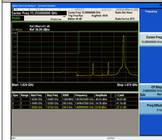
CA_2C-20MHz-5MHz-QPSK@QPSK-QPSK@QPSK-18700-18817-1RB#99@100RB#0-0RB#0@25RB#0-PASS
