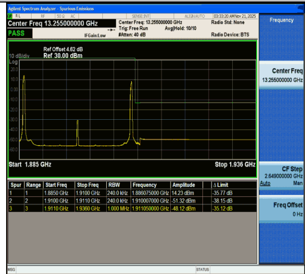
CA_2C-10MHz-15MHz-QPSK@QPSK-QPSK@QPSK-19005-19125-1RB#0@50RB#0-1RB#74@75RB#0-PASS
