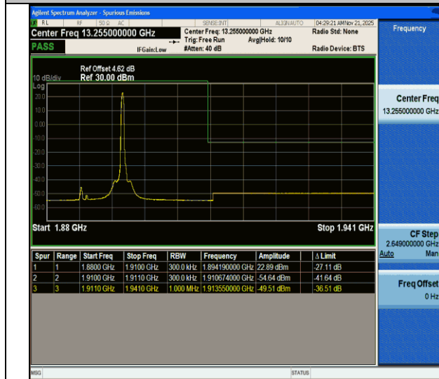
CA_2C-15MHz-15MHz-QPSK@QPSK-QPSK@QPSK-18975-19125-1RB#74@75RB#0-0RB#0@75RB#0-PASS
