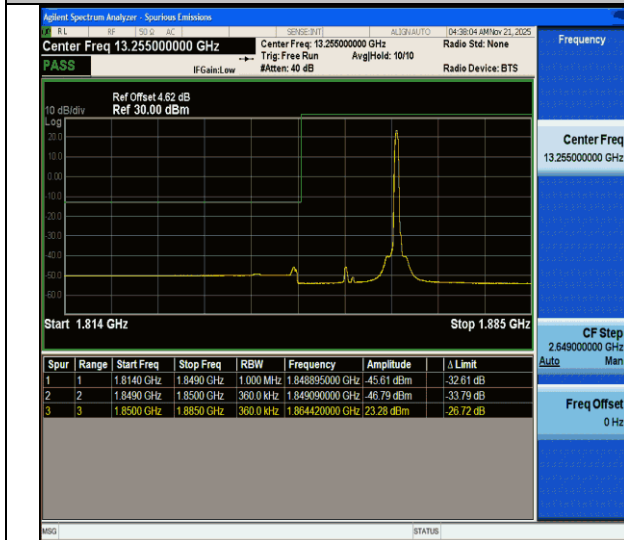
CA_2C-15MHz-20MHz-QPSK@QPSK-QPSK@QPSK-18678-18849-1RB#74@75RB#0-0RB#0@100RB#0-PASS
