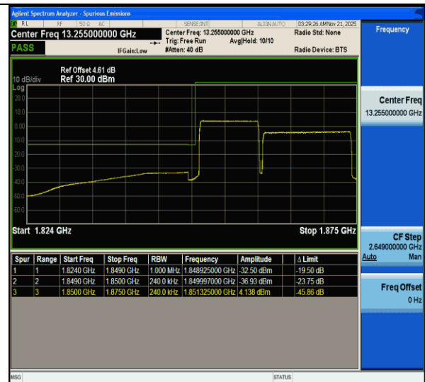
CA_2C-10MHz-15MHz-QPSK@QPSK-QPSK@QPSK-18653-18773-50RB#0@50RB#0-75RB#0@75RB#0-PASS
