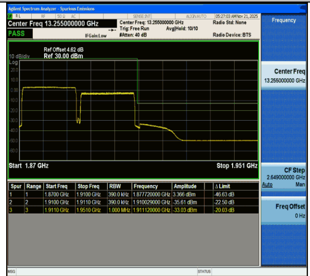
CA_2C-20MHz-20MHz-QPSK@QPSK-QPSK@QPSK-18902-19100-100RB#0@100RB#0-100RB#0@100RB#0-PASS
