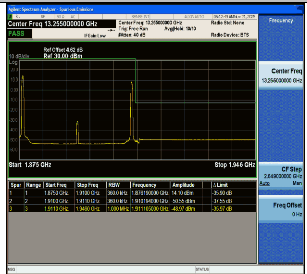
CA_2C-20MHz-15MHz-QPSK@QPSK-QPSK@QPSK-18951-19122-1RB#0@100RB#0-1RB#74@75RB#0-PASS
