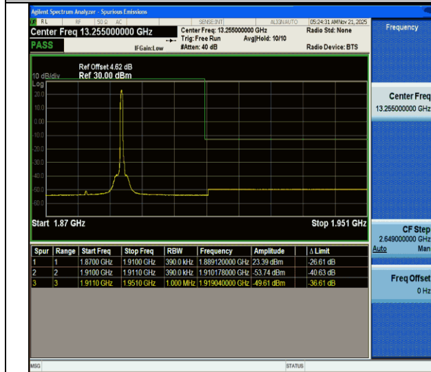
CA_2C-20MHz-20MHz-QPSK@QPSK-QPSK@QPSK-18902-19100-1RB#99@100RB#0-0RB#0@100RB#0-PASS
