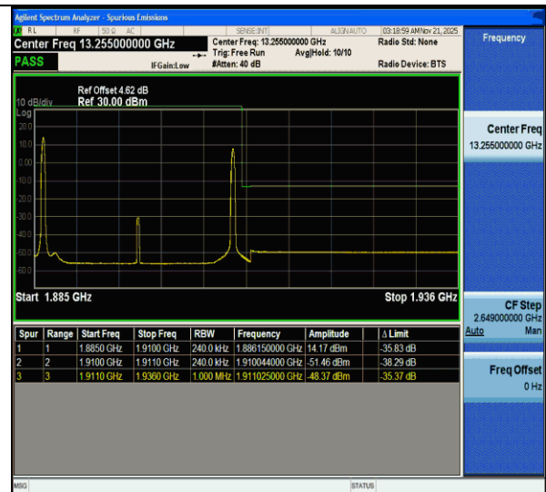
CA_2C-5MHz-20MHz-QPSK@QPSK-QPSK@QPSK-18983-19100-1RB#0@25RB#0-1RB#99@100RB#0-PASS
