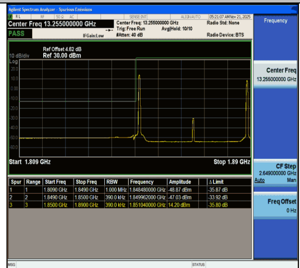
CA_2C-20MHz-20MHz-QPSK@QPSK-QPSK@QPSK-18700-18898-1RB#0@100RB#0-1RB#99@100RB#0-PASS
