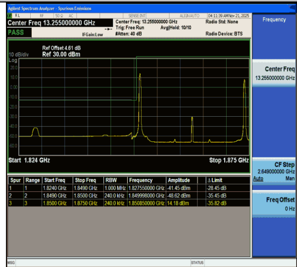
CA_2C-15MHz-10MHz-QPSK@QPSK-QPSK@QPSK-18675-18795-1RB#0@75RB#0-1RB#49@50RB#0-PASS
