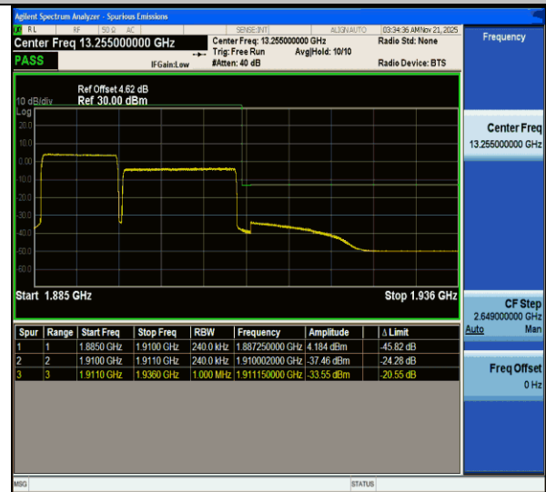
CA_2C-10MHz-15MHz-QPSK@QPSK-QPSK@QPSK-19005-19125-50RB#0@50RB#0-75RB#0@75RB#0-PASS
