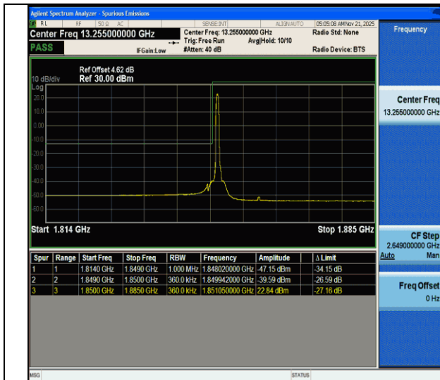
CA_2C-20MHz-15MHz-QPSK@QPSK-QPSK@QPSK-18700-18871-1RB#0@100RB#0-0RB#0@75RB#0-PASS
