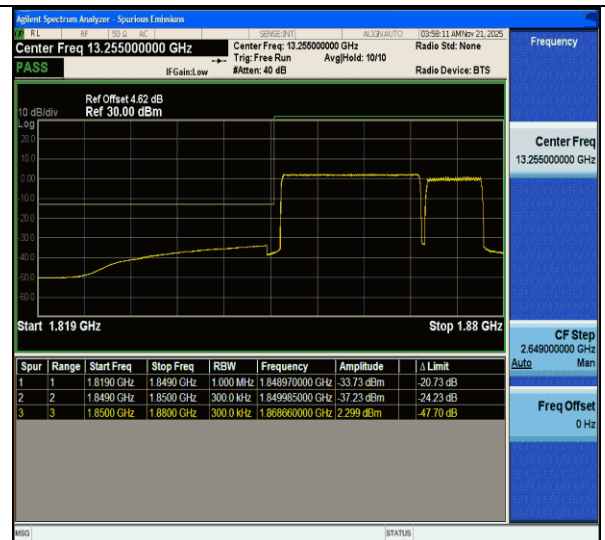
CA_2C-20MHz-10MHz-QPSK@QPSK-QPSK@QPSK-18700-18844-100RB#0@100RB#0-40RB#0@50RB#0-PASS
