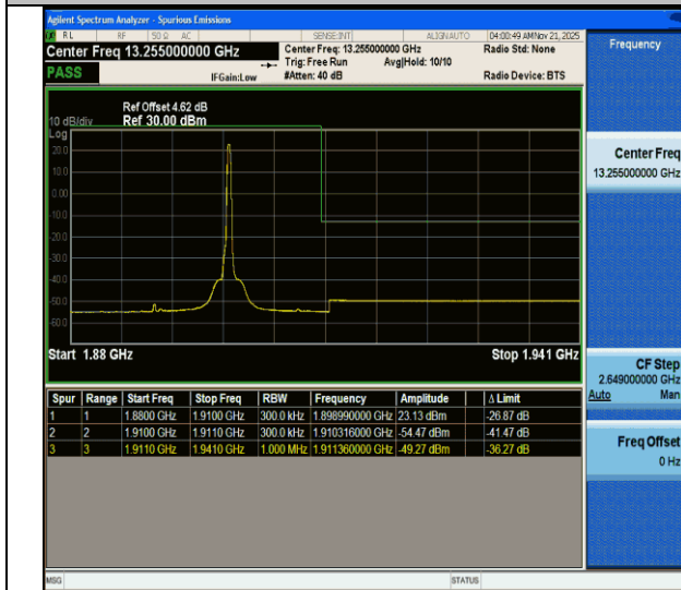
CA_2C-20MHz-10MHz-QPSK@QPSK-QPSK@QPSK-19001-19145-1RB#99@100RB#0-0RB#0@50RB#0-PASS
