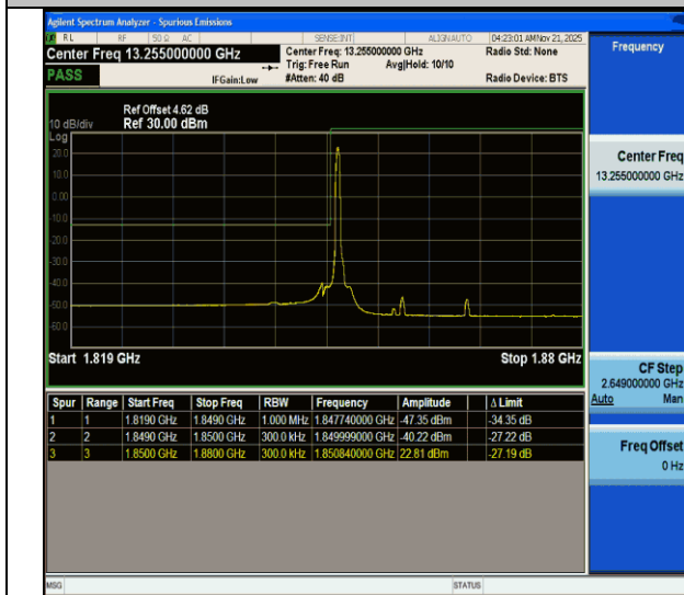
CA_2C-15MHz-15MHz-QPSK@QPSK-QPSK@QPSK-18675-18825-1RB#0@75RB#0-0RB#0@75RB#0-PASS
