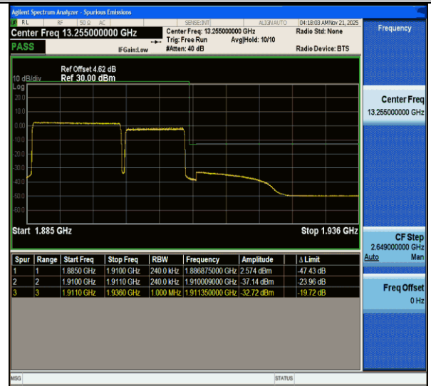
CA_2C-15MHz-10MHz-QPSK@QPSK-QPSK@QPSK-19027-19147-75RB#0@75RB#0-50RB#0@50RB#0-PASS
