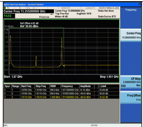
CA_2C-20MHz-20MHz-QPSK@QPSK-QPSK@QPSK-18902-19100-1RB#0@100RB#0-1RB#99@100RB#0-PASS
