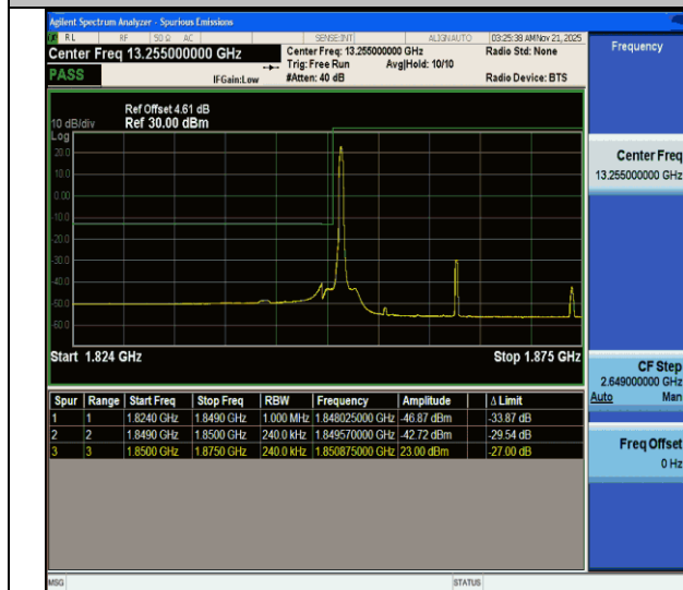
CA_2C-10MHz-15MHz-QPSK@QPSK-QPSK@QPSK-18653-18773-1RB#0@50RB#0-0RB#0@75RB#0-PASS
