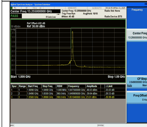
CA_2C-20MHz-20MHz-QPSK@QPSK-QPSK@QPSK-18700-18898-1RB#0@100RB#0-0RB#0@100RB#0-PASS
