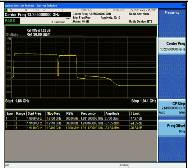
CA_2C-20MHz-10MHz-QPSK@QPSK-QPSK@QPSK-19001-19145-100RB#0@100RB#0-40RB#0@50RB#0-PASS
