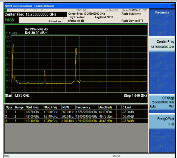
CA_2C-15MHz-20MHz-QPSK@QPSK-QPSK@QPSK-18929-19100-1RB#0@75RB#0-1RB#99@100RB#0-PASS
