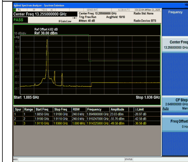
CA_2C-10MHz-15MHz-QPSK@QPSK-QPSK@QPSK-19005-19125-1RB#49@50RB#0-0RB#0@75RB#0-PASS
