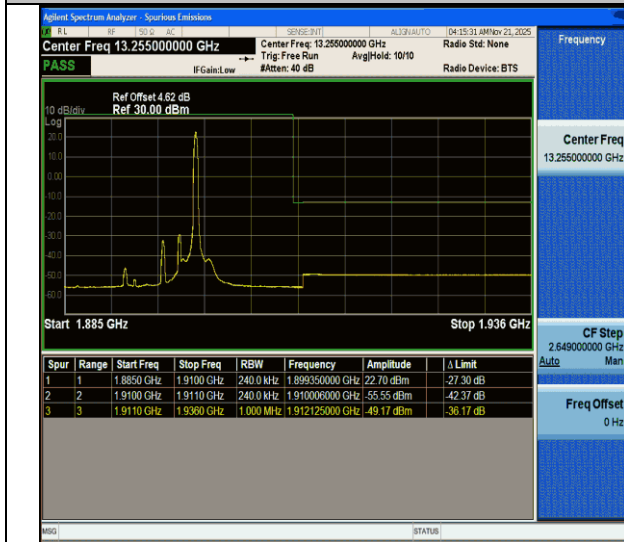
CA_2C-15MHz-10MHz-QPSK@QPSK-QPSK@QPSK-19027-19147-1RB#74@75RB#0-0RB#0@50RB#0-PASS
