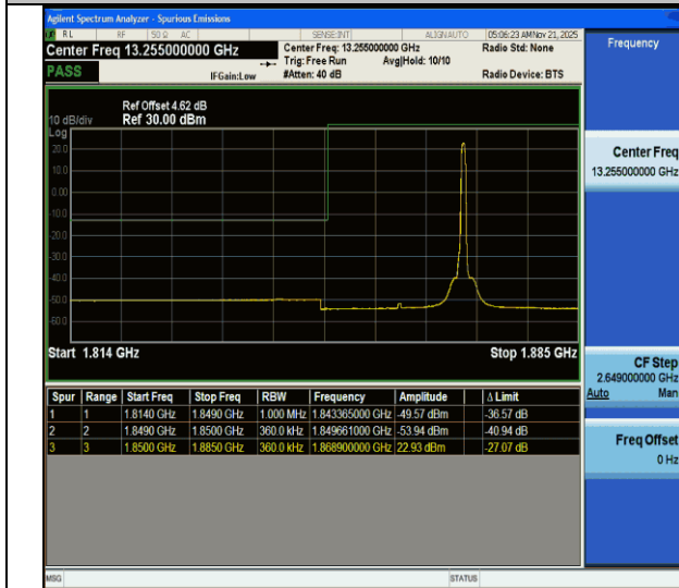
CA_2C-20MHz-15MHz-QPSK@QPSK-QPSK@QPSK-18700-18871-1RB#99@100RB#0-0RB#0@75RB#0-PASS
