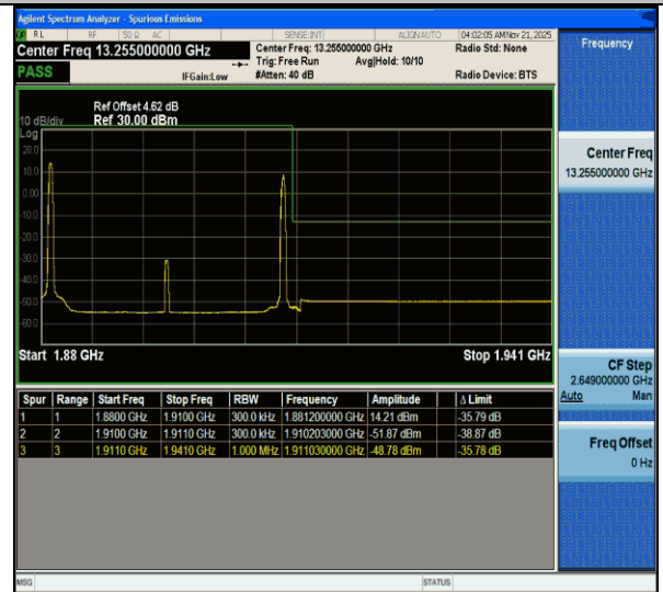
CA_2C-20MHz-10MHz-QPSK@QPSK-QPSK@QPSK-19001-19145-1RB#0@100RB#0-1RB#49@50RB#0-PASS
