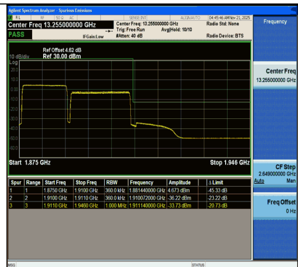
CA_2C-15MHz-20MHz-QPSK@QPSK-QPSK@QPSK-18929-19100-75RB#0@75RB#0-100RB#0@100RB#0-PASS
