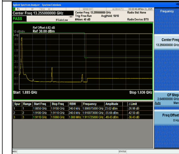
CA_2C-10MHz-15MHz-QPSK@QPSK-QPSK@QPSK-19005-19125-1RB#0@50RB#0-0RB#0@75RB#0-PASS
