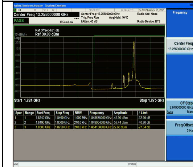
CA_2C-15MHz-10MHz-QPSK@QPSK-QPSK@QPSK-18675-18795-1RB#74@75RB#0-0RB#0@50RB#0-PASS
