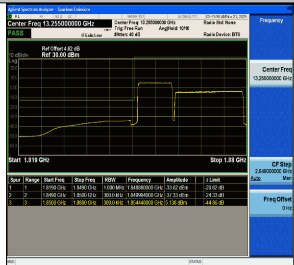
CA_2C-10MHz-20MHz-QPSK@QPSK-QPSK@QPSK-18655-18799-50RB#0@50RB#0-100RB#0@100RB#0-PASS
