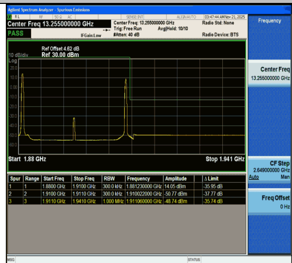
CA_2C-10MHz-20MHz-QPSK@QPSK-QPSK@QPSK-18956-19100-1RB#0@50RB#0-1RB#99@100RB#0-PASS
