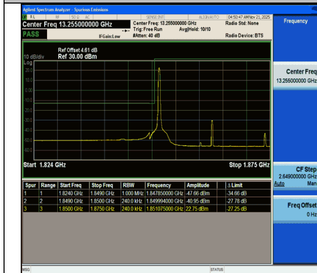
CA_2C-20MHz-5MHz-QPSK@QPSK-QPSK@QPSK-18700-18817-1RB#0@100RB#0-0RB#0@25RB#0-PASS
