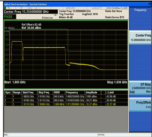
CA_2C-5MHz-20MHz-QPSK@QPSK-QPSK@QPSK-18983-19100-25RB#0@25RB#0-100RB#0@100RB#0-PASS
