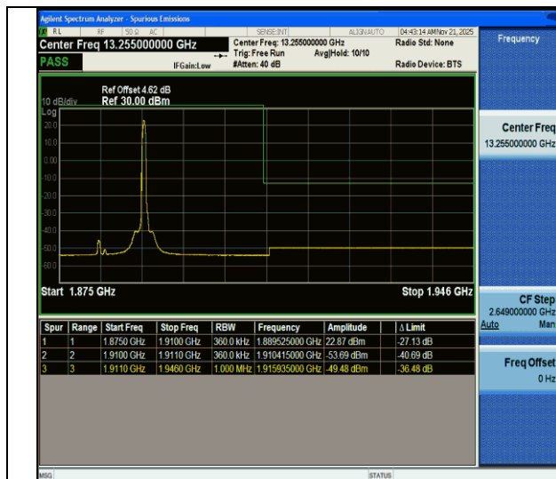
CA_2C-15MHz-20MHz-QPSK@QPSK-QPSK@QPSK-18929-19100-1RB#74@75RB#0-0RB#0@100RB#0-PASS
