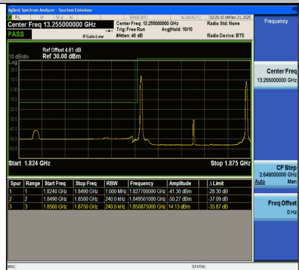
CA_2C-10MHz-15MHz-QPSK@QPSK-QPSK@QPSK-18653-18773-1RB#0@50RB#0-1RB#74@75RB#0-PASS
