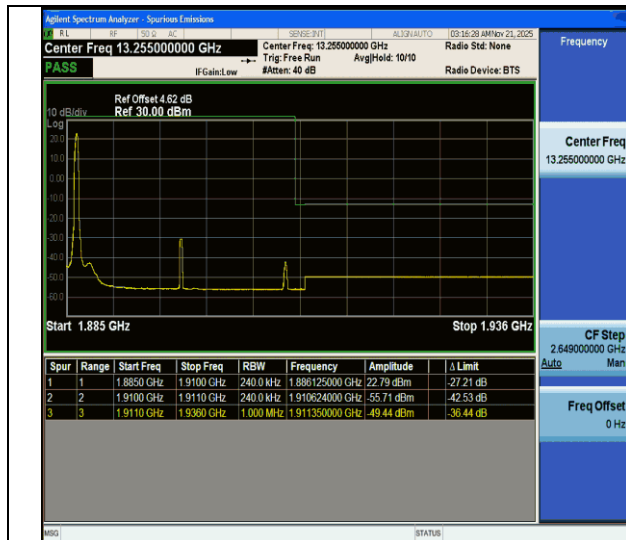
CA_2C-5MHz-20MHz-QPSK@QPSK-QPSK@QPSK-18983-19100-1RB#0@25RB#0-0RB#0@100RB#0-PASS
