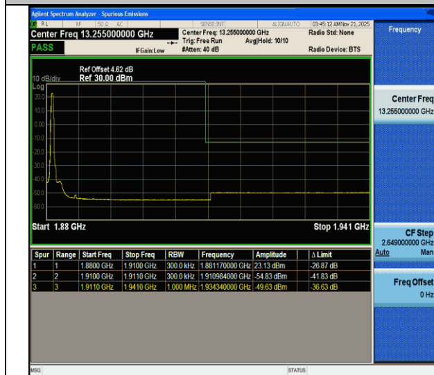
CA_2C-10MHz-20MHz-QPSK@QPSK-QPSK@QPSK-18956-19100-1RB#0@50RB#0-0RB#0@100RB#0-PASS
