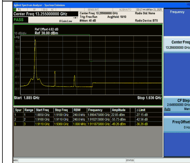
CA_2C-5MHz-20MHz-QPSK@QPSK-QPSK@QPSK-18983-19100-1RB#24@25RB#0-0RB#0@100RB#0-PASS
