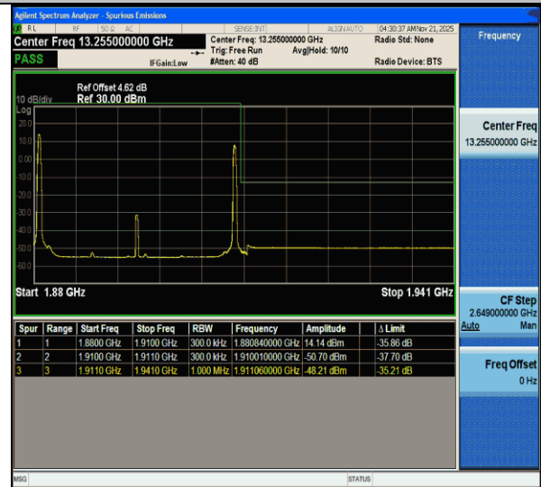
CA_2C-15MHz-15MHz-QPSK@QPSK-QPSK@QPSK-18975-19125-1RB#0@75RB#0-1RB#74@75RB#0-PASS
