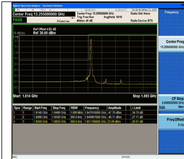
CA_2C-15MHz-20MHz-QPSK@QPSK-QPSK@QPSK-18678-18849-1RB#0@75RB#0-0RB#0@100RB#0-PASS
