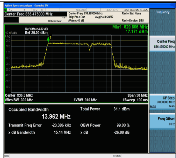
CA_5B-10MHz-5MHz-16QAM-16QAM-20500-20572-50RB#0-25RB#0-PASS
