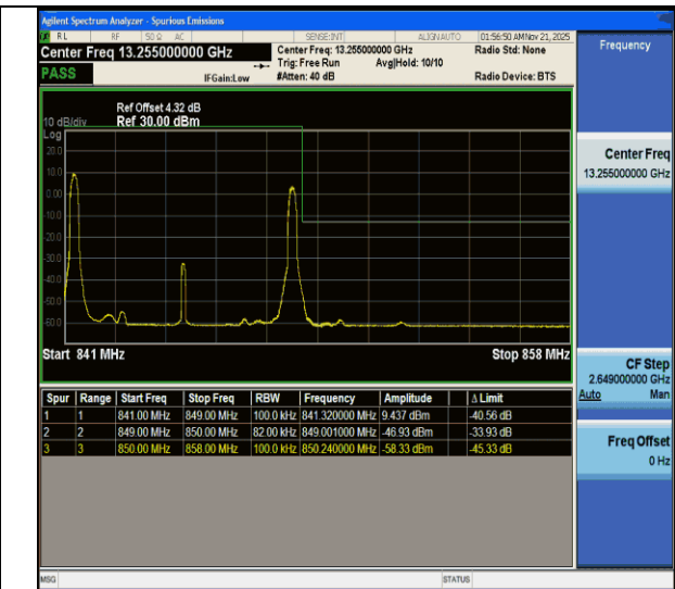
CA_5B-3MHz-5MHz-QPSK@QPSK-QPSK@QPSK-20586-20625-1RB#0@15RB#0-1RB#24@25RB#0-PASS
