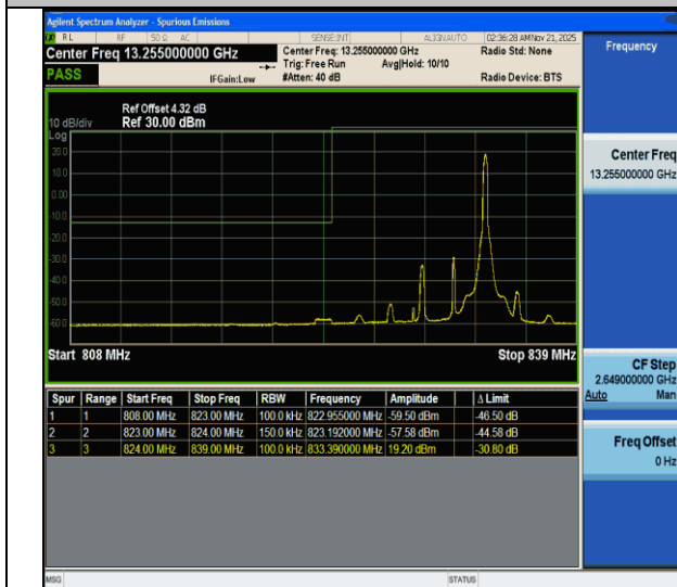
CA_5B-10MHz-5MHz-QPSK@QPSK-QPSK@QPSK-20450-20522-1RB#49@50RB#0-0RB#0@25RB#0-PASS
