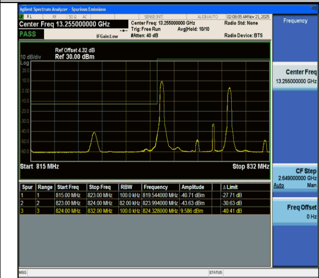
CA_5B-5MHz-3MHz-QPSK@QPSK-QPSK@QPSK-20425-20464-1RB#0@25RB#0-1RB#15@15RB#0-PASS
