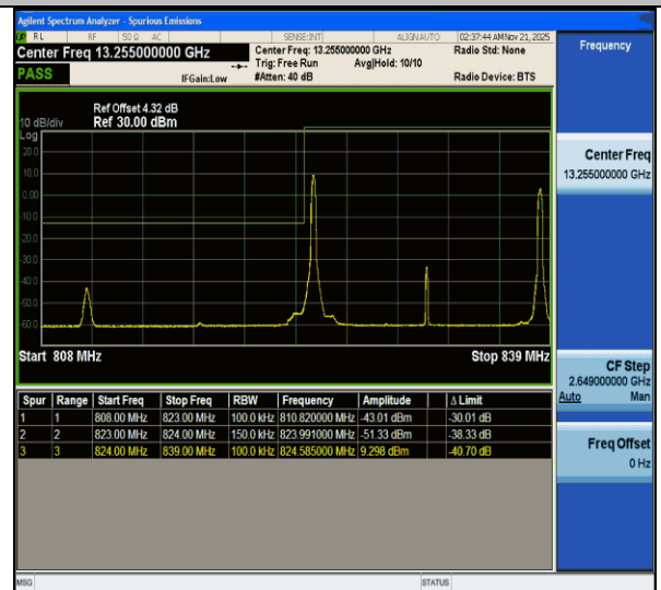
CA_5B-10MHz-5MHz-QPSK@QPSK-QPSK@QPSK-20450-20522-1RB#0@50RB#0-1RB#24@25RB#0-PASS
