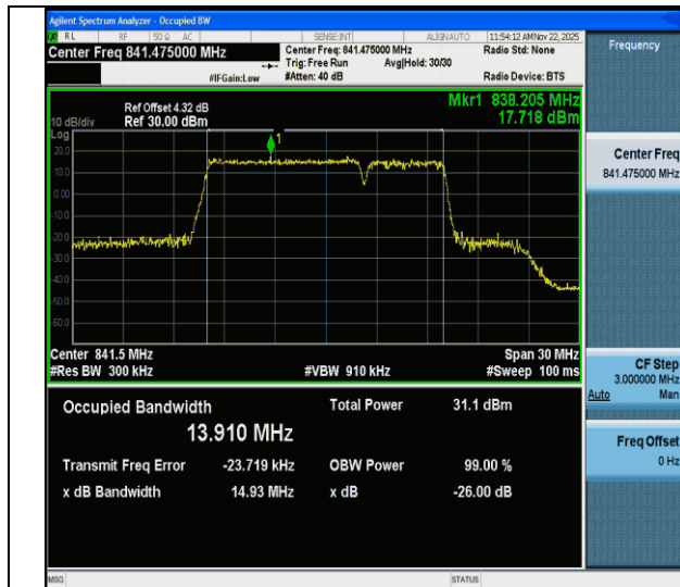
CA_5B-10MHz-5MHz-64QAM-64QAM-20550-20622-50RB#0- 25RB#0-PASS
