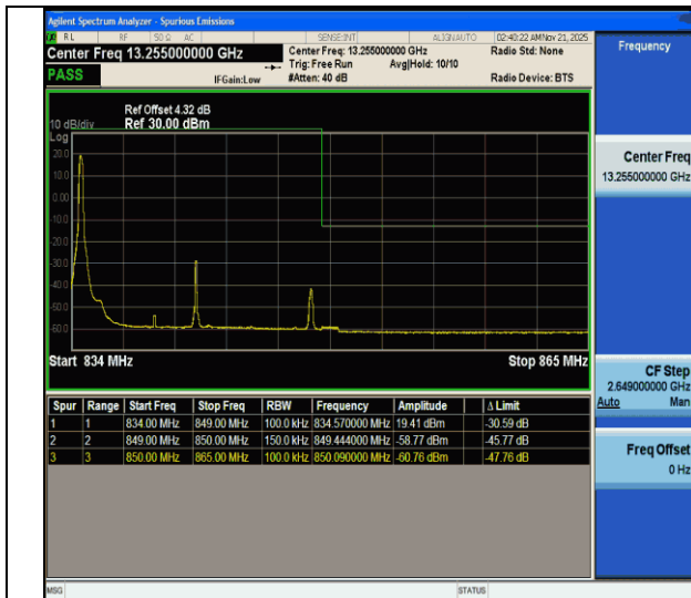
CA_5B-10MHz-5MHz-QPSK@QPSK-QPSK@QPSK-20550-20622-1RB#0@50RB#0-0RB#0@25RB#0-PASS
