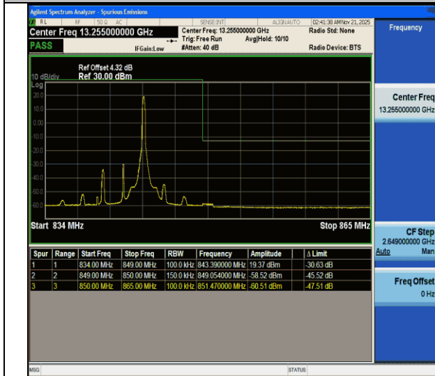
CA_5B-10MHz-5MHz-QPSK@QPSK-QPSK@QPSK-20550-20622-1RB#49@50RB#0-0RB#0@25RB#0-PASS
