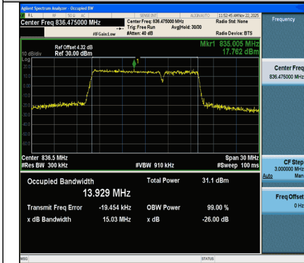
CA_5B-10MHz-5MHz-64QAM-64QAM-20500-20572-50RB#0-25RB#0-PASS
