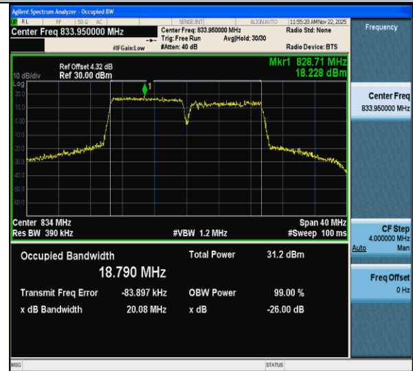
CA_5B-10MHz-10MHz-16QAM-16QAM-20450-20549-50RB#0- 50RB#0-PASS
