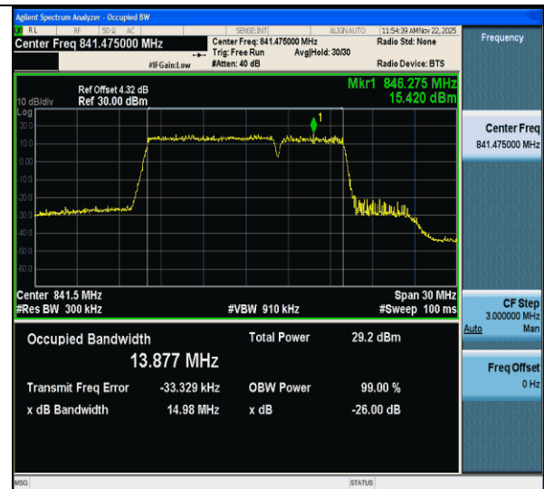
CA_5B-10MHz-5MHz-256QAM-256QAM-20550-20622-50RB#0- 25RB#0-PASS
