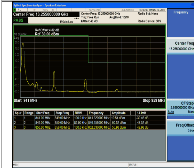
CA_5B-5MHz-3MHz-QPSK@QPSK-QPSK@QPSK-20595-20634-1RB#0@25RB#0-0RB#0@15RB#0-PASS
