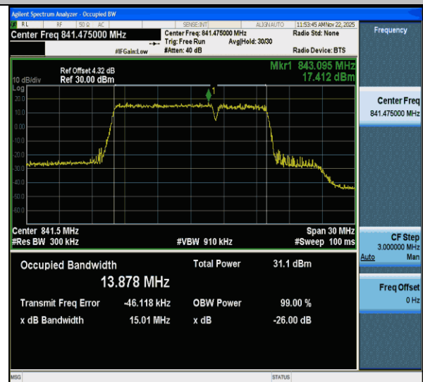
CA_5B-10MHz-5MHz-16QAM-16QAM-20550-20622-50RB#0-25RB#0-PASS
