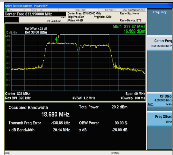
CA_5B-10MHz-10MHz-256QAM-256QAM-20450-20549-50RB#0- 50RB#0-PASS
