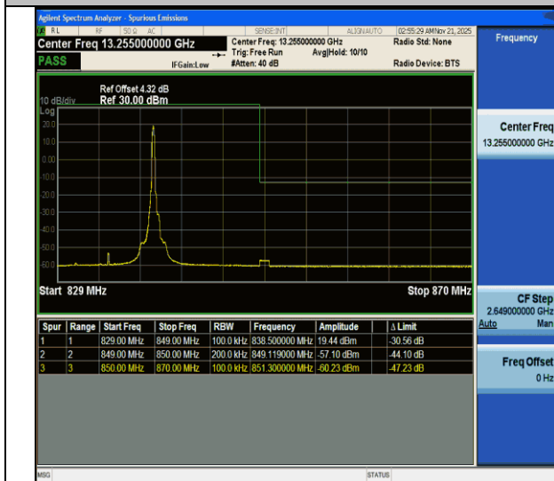
CA_5B-10MHz-10MHz-QPSK@QPSK-QPSK@QPSK-20501-20600-1RB#49@50RB#0-0RB#0@50RB#0-PASS
