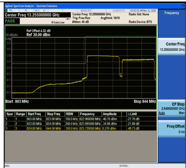
CA_5B-10MHz-10MHz-QPSK@QPSK-QPSK@QPSK-20450-20549-50RB#0@50RB#0-50RB#0@50RB#0-PASS
