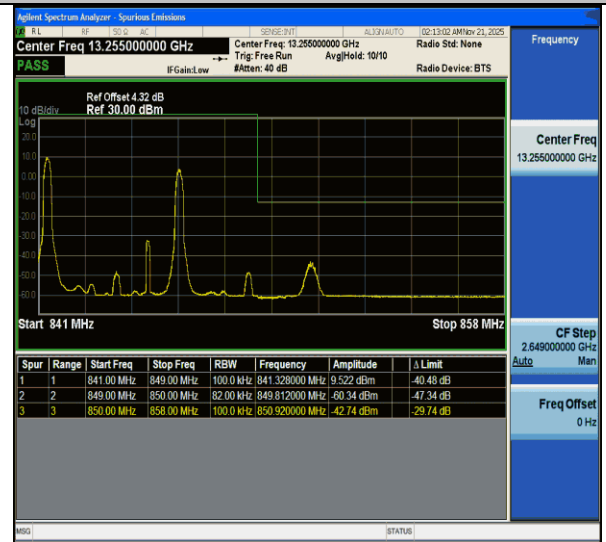
CA_5B-5MHz-3MHz-QPSK@QPSK-QPSK@QPSK-20595-20634-1RB#0@25RB#0-1RB#15@15RB#0-PASS
