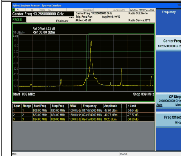
CA_5B-10MHz-5MHz-QPSK@QPSK-QPSK@QPSK-20450-20522-1RB#0@50RB#0-0RB#0@25RB#0-PASS
