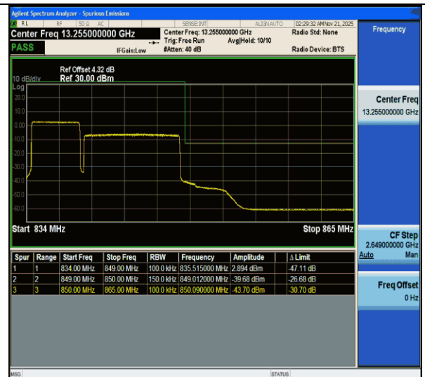
CA_5B-5MHz-10MHz-QPSK@QPSK-QPSK@QPSK-20528-20600-25RB#0@25RB#0-50RB#0@50RB#0-PASS
