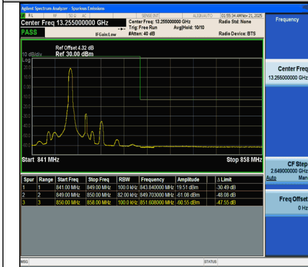
CA_5B-3MHz-5MHz-QPSK@QPSK-QPSK@QPSK-20586-20625-1RB#14@15RB#0-0RB#0@25RB#0-PASS
