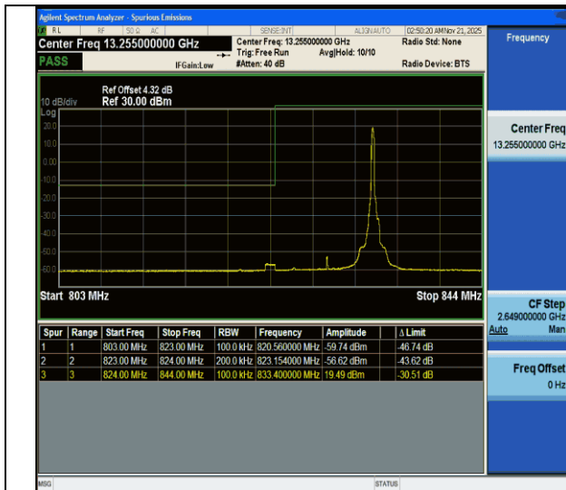
CA_5B-10MHz-10MHz-QPSK@QPSK-QPSK@QPSK-20450-20549-1RB#49@50RB#0-0RB#0@50RB#0-PASS
