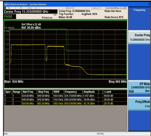
CA_5B-10MHz-5MHz-QPSK@QPSK-QPSK@QPSK-20550-20622-50RB#0@50RB#0-25RB#0@25RB#0-PASS
