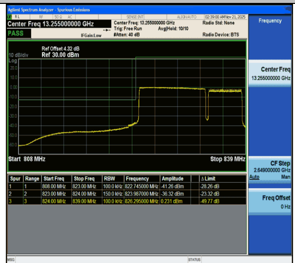
CA_5B-10MHz-5MHz-QPSK@QPSK-QPSK@QPSK-20450-20522-50RB#0@50RB#0-25RB#0@25RB#0-PASS
