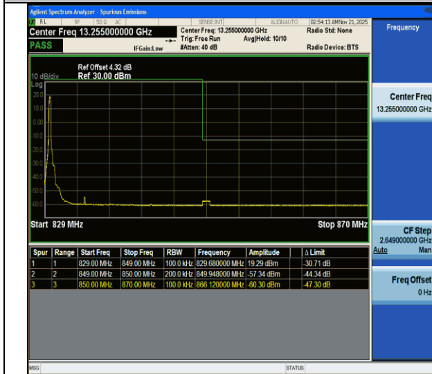
CA_5B-10MHz-10MHz-QPSK@QPSK-QPSK@QPSK-20501-20600-1RB#0@50RB#0-0RB#0@50RB#0-PASS
