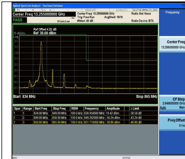
CA_5B-5MHz-10MHz-QPSK@QPSK-QPSK@QPSK-20528-20600-1RB#24@25RB#0-0RB#0@50RB#0-PASS
