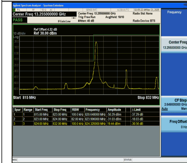
CA_5B-5MHz-3MHz-QPSK@QPSK-QPSK@QPSK-20425-20464-1RB#0@25RB#0-0RB#0@15RB#0-PASS
