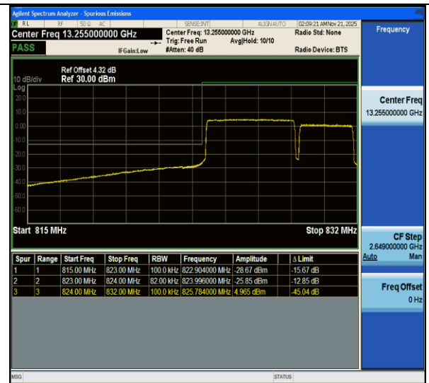
CA_5B-5MHz-3MHz-QPSK@QPSK-QPSK@QPSK-20425-20464-25RB#0@25RB#0-15RB#0@15RB#0-PASS
