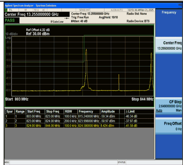
CA_5B-10MHz-10MHz-QPSK@QPSK-QPSK@QPSK-20450-20549-1RB#0@50RB#0-1RB#49@50RB#0-PASS
