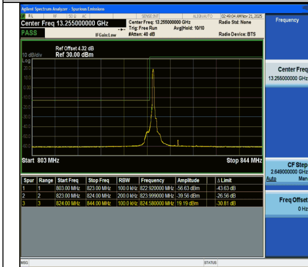
CA_5B-10MHz-10MHz-QPSK@QPSK-QPSK@QPSK-20450-20549-1RB#0@50RB#0-0RB#0@50RB#0-PASS
