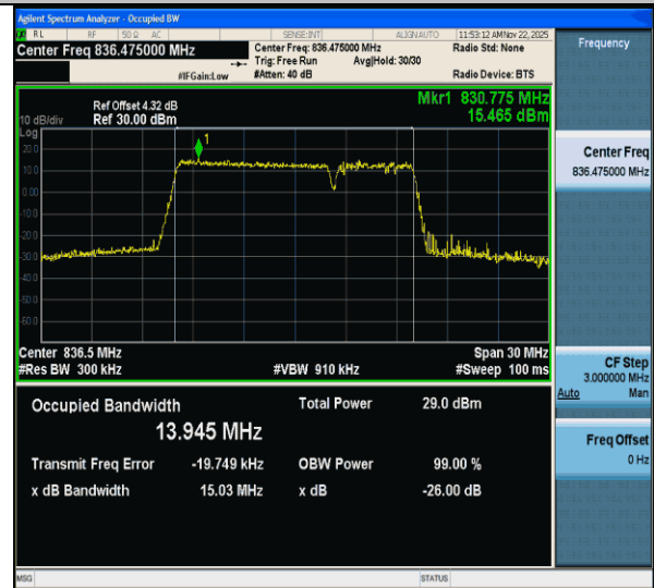
CA_5B-10MHz-5MHz-256QAM-256QAM-20500-20572-50RB#0-25RB#0-PASS
