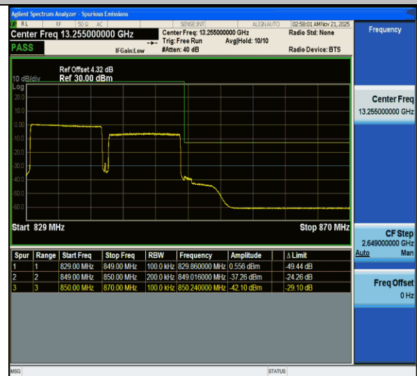
CA_5B-10MHz-10MHz-QPSK@QPSK-QPSK@QPSK-20501-20600-50RB#0@50RB#0-50RB#0@50RB#0-PASS
