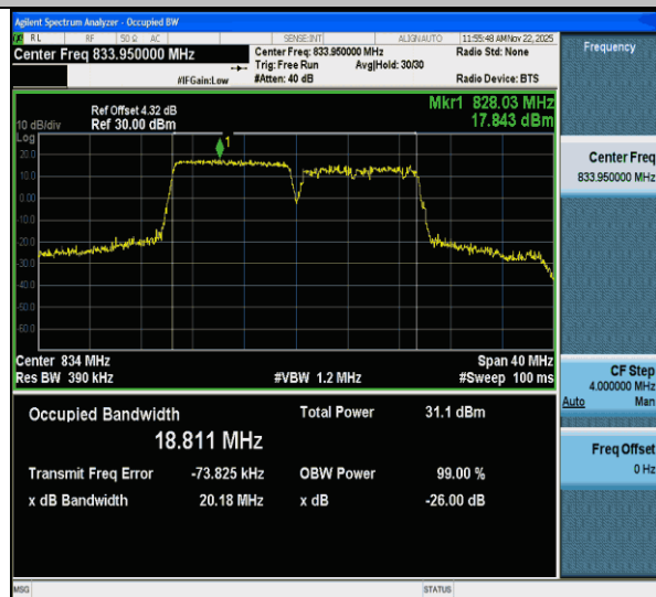
CA_5B-10MHz-10MHz-64QAM-64QAM-20450-20549-50RB#0- 50RB#0-PASS
