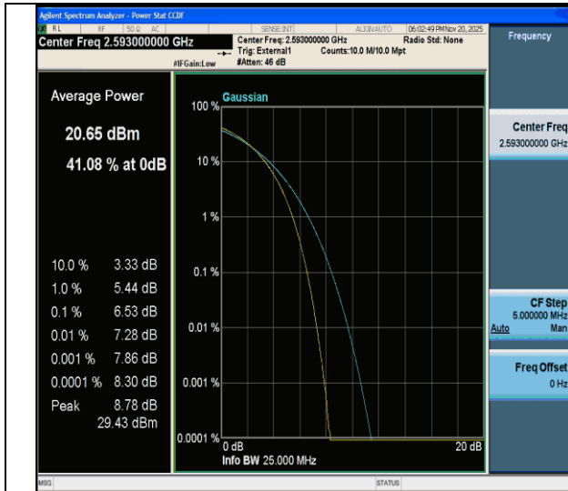
CA_41C-20MHz-20MHz-QPSK-QPSK-40521-40719-100RB#0- 100RB#0-PASS
