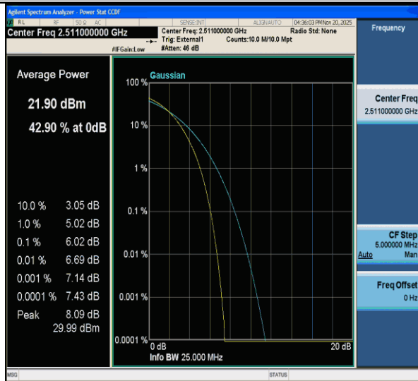
CA_41C-15MHz-15MHz-QPSK-QPSK-39725-39875-75RB#0-75RB#0-PASS
