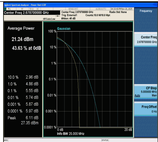
CA_41C-15MHz-10MHz-QPSK-QPSK-41417-41537-75RB#0-50RB#0-PASS
