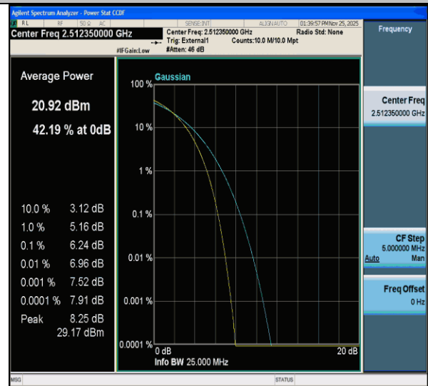
CA_41C-15MHz-20MHz-QPSK-QPSK-39728-39899-75RB#0-100RB#0-PASS
