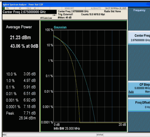
CA_41C-15MHz-15MHz-QPSK-QPSK-41365-41515-75RB#0-75RB#0-PASS
