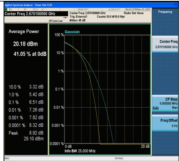
CA_41C-20MHz-20MHz-QPSK-QPSK-41292-41490-100RB#0- 100RB#0-PASS
