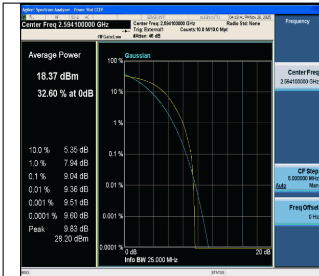
CA_41C-15MHz-10MHz-QPSK-QPSK-40571-40691-75RB#0-50RB#0-PASS
