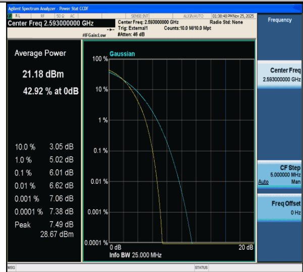
CA_41C-15MHz-15MHz-QPSK-QPSK-40545-40695-75RB#0-75RB#0-PASS
