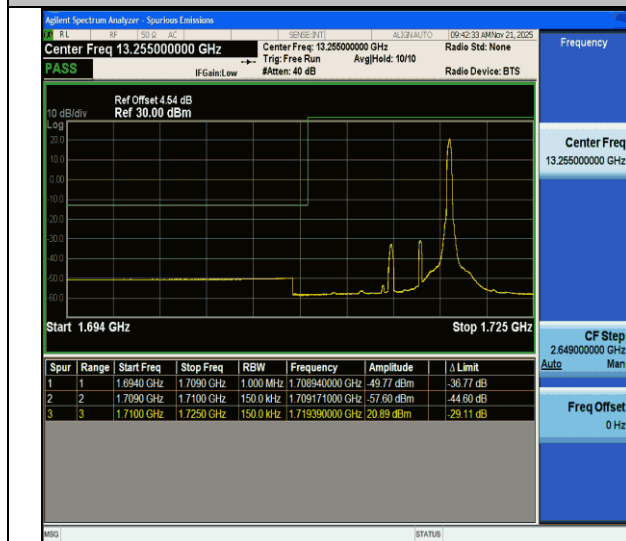
CA_66B-10MHz-5MHz-QPSK@QPSK-QPSK@QPSK-132022- 132094-1RB#49@50RB#0-0RB#0@25RB#0-PASS
