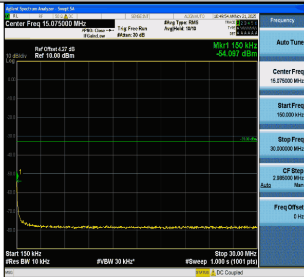
CA_66B-15MHz-5MHz-QPSK-QPSK-132398-132491-1RB#0-0RB#0-0.15~30MHz-PASS
