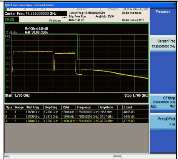
CA_66B-10MHz-5MHz-QPSK@QPSK-QPSK@QPSK-132572-132644-50RB#0@50RB#0-25RB#0@25RB#0-PASS
