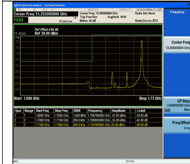
CA_66B-15MHz-5MHz-QPSK@QPSK-QPSK@QPSK-132047- 132140-1RB#74@75RB#0-0RB#0@25RB#0-PASS
