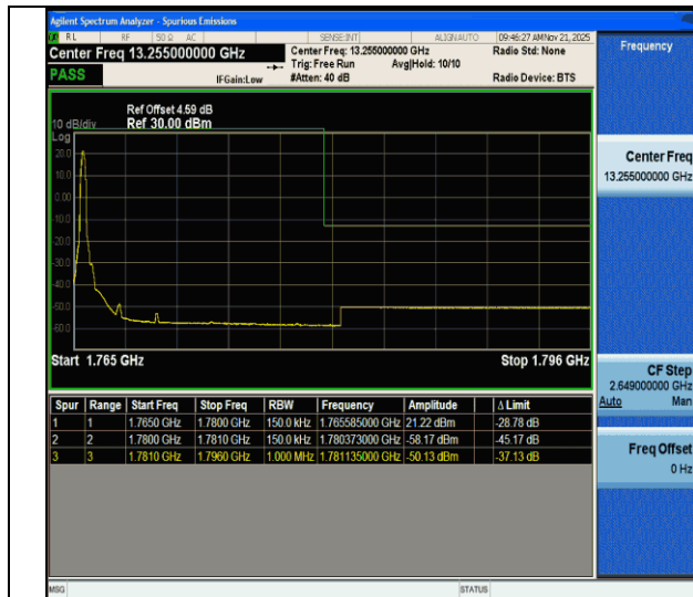
CA_66B-10MHz-5MHz-QPSK@QPSK-QPSK@QPSK-132572-132644-1RB#0@50RB#0-0RB#0@25RB#0-PASS
