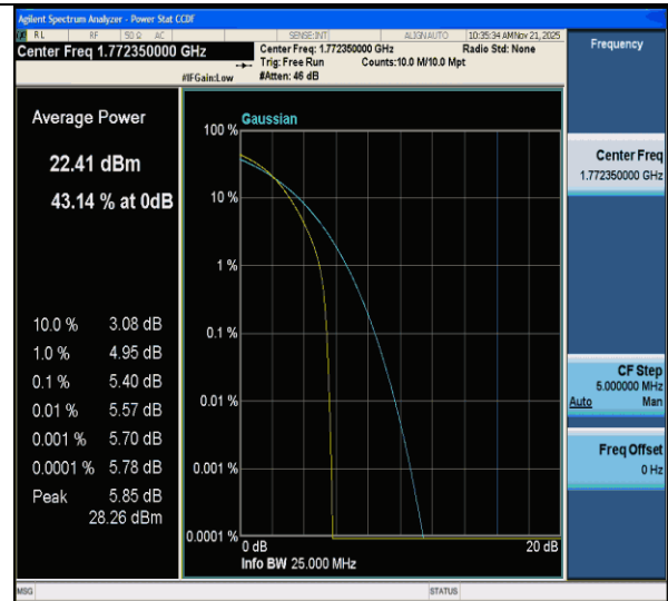
CA_66B-15MHz-5MHz-QPSK-QPSK-132549-132642-75RB#0- 25RB#0-PASS
