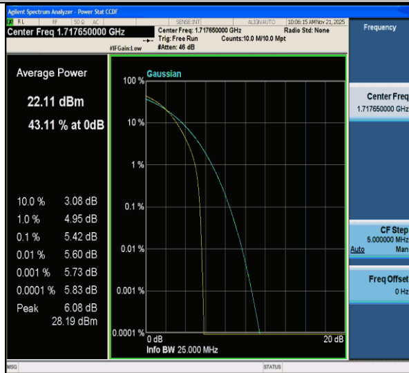
CA_66B-5MHz-15MHz-QPSK-QPSK-132002-132095-25RB#0-75RB#0-PASS
