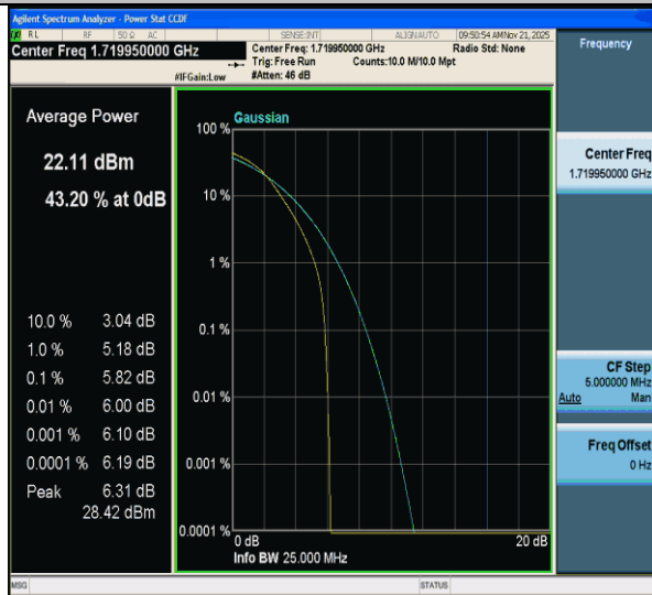
CA_66B-10MHz-10MHz-QPSK-QPSK-132022-132121-50RB#0-50RB#0-PASS
