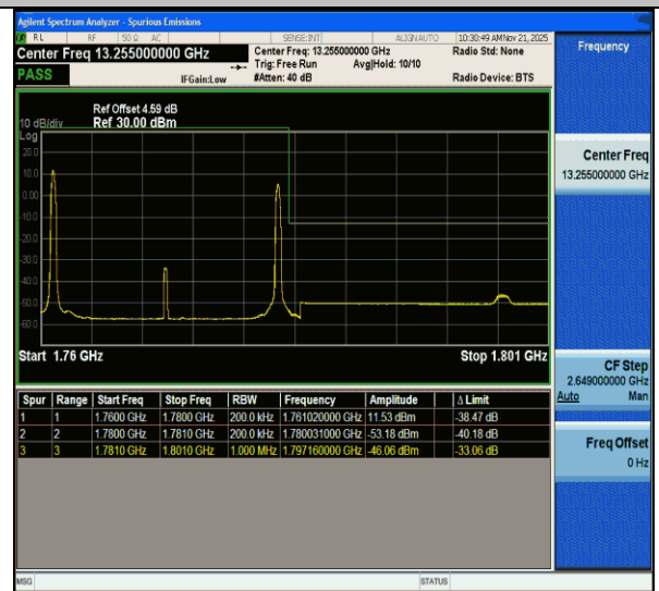
CA_66B-5MHz-15MHz-QPSK@QPSK-QPSK@QPSK-132504-132597-1RB#0@25RB#0-1RB#74@75RB#0-PASS
