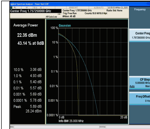
CA_66B-15MHz-5MHz-QPSK-QPSK-132398-132491-75RB#0- 25RB#0-PASS
