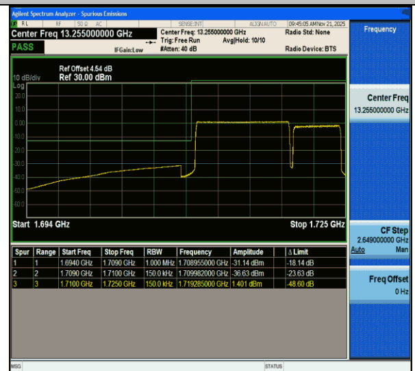
CA_66B-10MHz-5MHz-QPSK@QPSK-QPSK@QPSK-132022- 132094-50RB#0@50RB#0-25RB#0@25RB#0-PASS
