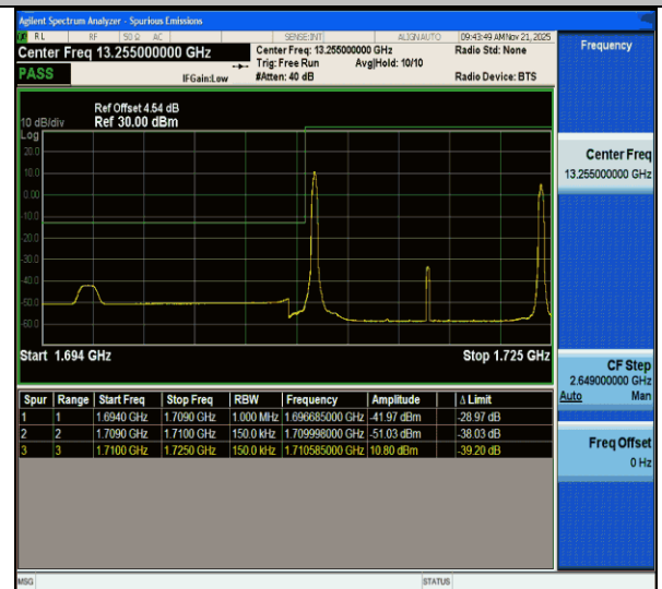
CA_66B-10MHz-5MHz-QPSK@QPSK-QPSK@QPSK-132022- 132094-1RB#0@50RB#0-1RB#24@25RB#0-PASS
