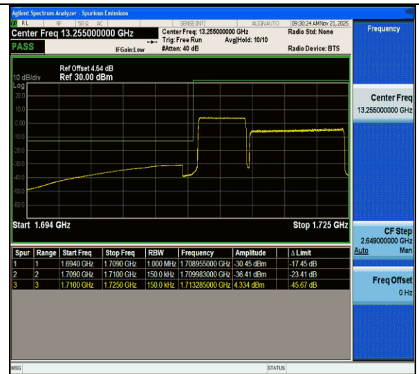
CA_66B-5MHz-10MHz-QPSK@QPSK-QPSK@QPSK-132000-132072-25RB#0@25RB#0-50RB#0@50RB#0-PASS
