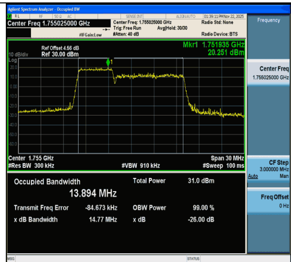
CA_66B-5MHz-10MHz-16QAM-16QAM-132375-132447-25RB#0-50RB#0-PASS
