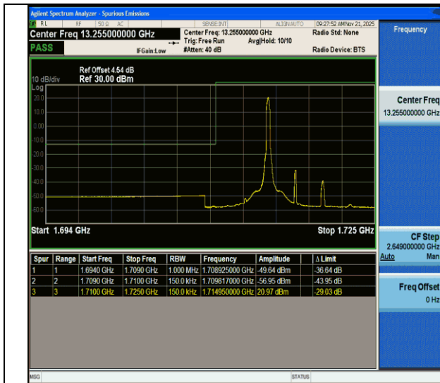
CA_66B-5MHz-10MHz-QPSK@QPSK-QPSK@QPSK-132000-132072-1RB#24@25RB#0-0RB#0@50RB#0-PASS
