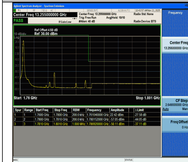
CA_66B-15MHz-5MHz-QPSK@QPSK-QPSK@QPSK-132549- 132642-1RB#0@75RB#0-0RB#0@25RB#0-PASS
