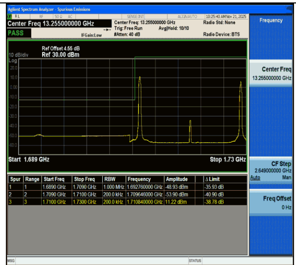
CA_66B-5MHz-15MHz-QPSK@QPSK-QPSK@QPSK-132002-132095-1RB#0@25RB#0-1RB#74@75RB#0-PASS
