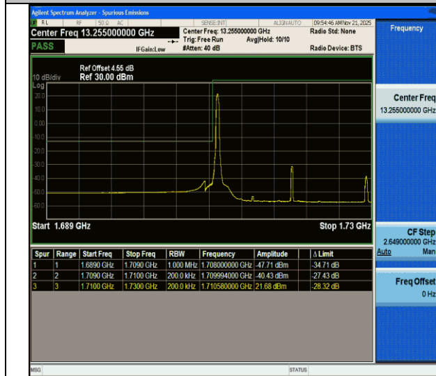
CA_66B-10MHz-10MHz-QPSK@QPSK-QPSK@QPSK-132022-132121-1RB#0@50RB#0-0RB#0@50RB#0-PASS
