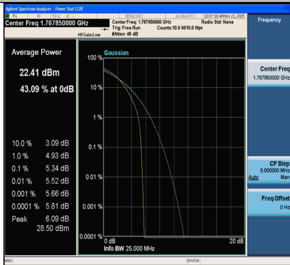
CA_66B-5MHz-15MHz-QPSK-QPSK-132504-132597-25RB#0-75RB#0-PASS
