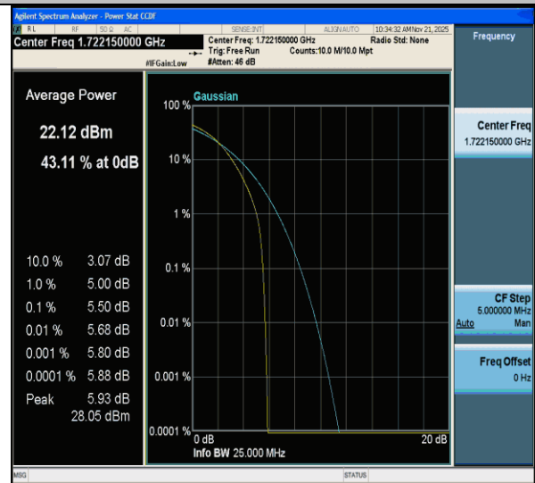
CA_66B-15MHz-5MHz-QPSK-QPSK-132047-132140-75RB#0-25RB#0-PASS
