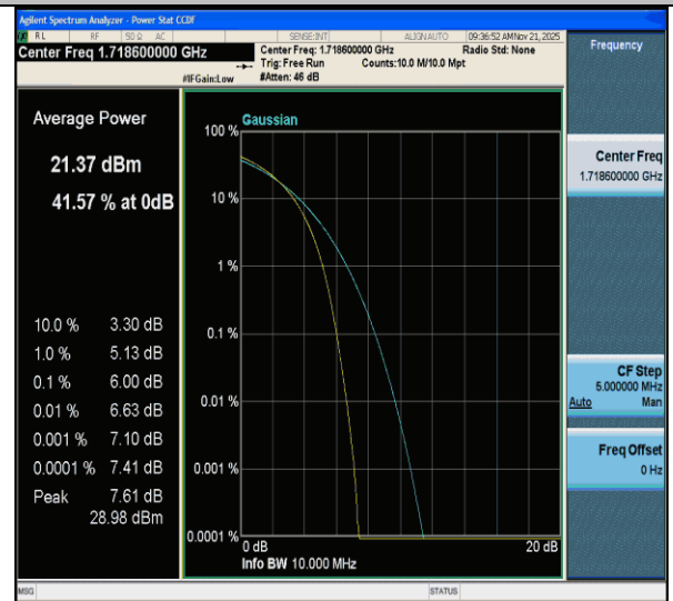
CA_66B-10MHz-5MHz-QPSK-QPSK-132022-132094-50RB#0-25RB#0-PASS
