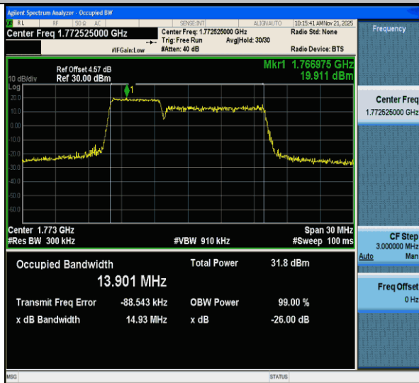
CA_66B-5MHz-10MHz-QPSK-QPSK-132550-132622-25RB#0-50RB#0-PASS
