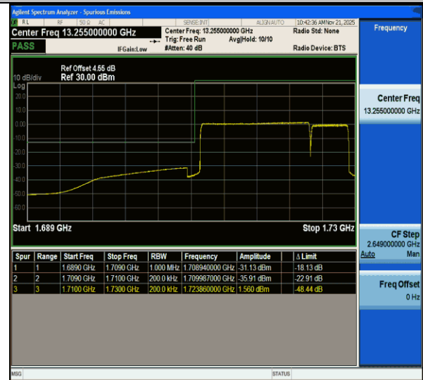
CA_66B-15MHz-5MHz-QPSK@QPSK-QPSK@QPSK-132047- 132140-75RB#0@75RB#0-25RB#0@25RB#0-PASS
