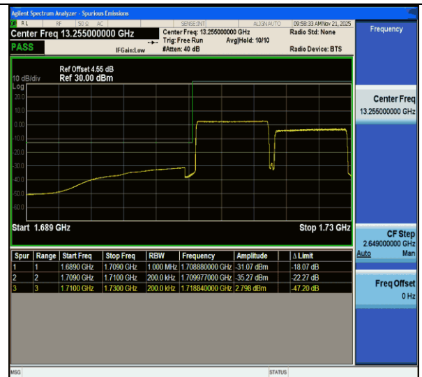
CA_66B-10MHz-10MHz-QPSK@QPSK-QPSK@QPSK-132022-132121-50RB#0@50RB#0-50RB#0@50RB#0-PASS
