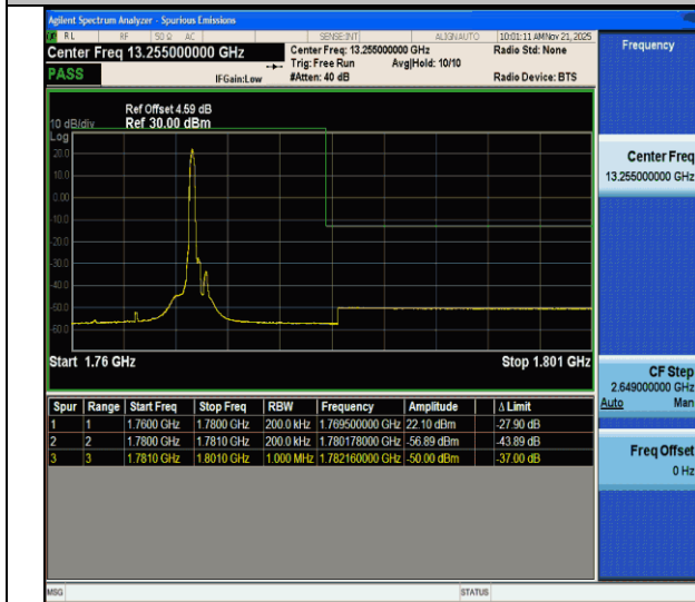
CA_66B-10MHz-10MHz-QPSK@QPSK-QPSK@QPSK-132523-132622-1RB#49@50RB#0-0RB#0@50RB#0-PASS
