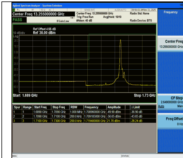
CA_66B-10MHz-10MHz-QPSK@QPSK-QPSK@QPSK-132022-132121-1RB#49@50RB#0-0RB#0@50RB#0-PASS
