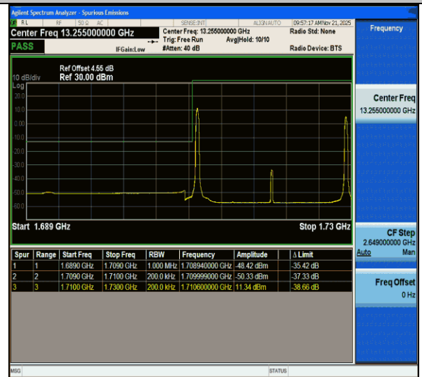
CA_66B-10MHz-10MHz-QPSK@QPSK-QPSK@QPSK-132022-132121-1RB#0@50RB#0-1RB#49@50RB#0-PASS
