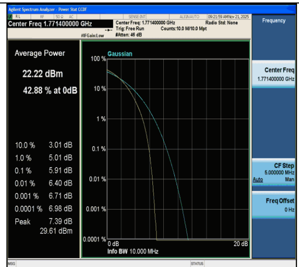
CA_66B-5MHz-10MHz-QPSK-QPSK-132550-132622-25RB#0-50RB#0-PASS
