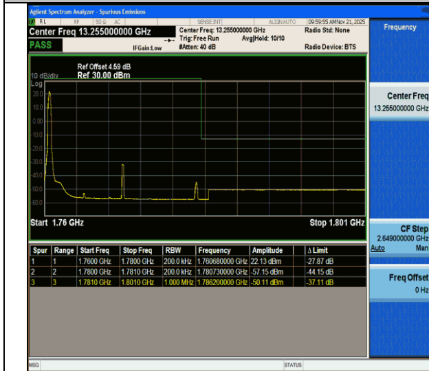
CA_66B-10MHz-10MHz-QPSK@QPSK-QPSK@QPSK-132523-132622-1RB#0@50RB#0-0RB#0@50RB#0-PASS
