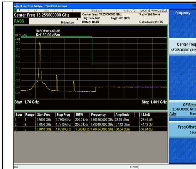
CA_66B-5MHz-15MHz-QPSK@QPSK-QPSK@QPSK-132504- 132597-1RB#24@25RB#0-0RB#0@75RB#0-PASS
