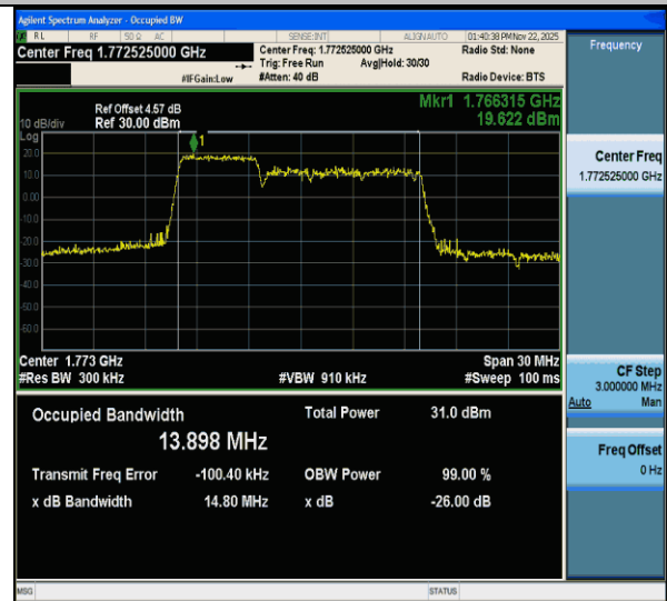
CA_66B-5MHz-10MHz-16QAM-16QAM-132550-132622-25RB#0-50RB#0-PASS
