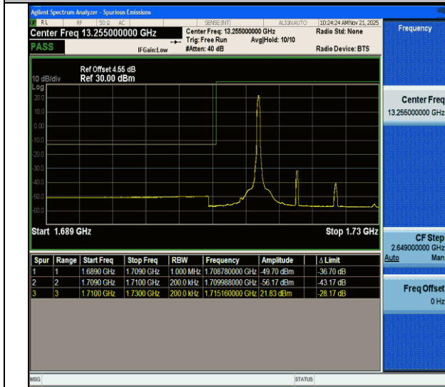
CA_66B-5MHz-15MHz-QPSK@QPSK-QPSK@QPSK-132002-132095-1RB#24@25RB#0-0RB#0@75RB#0-PASS
