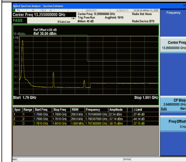
CA_66B-5MHz-15MHz-QPSK@QPSK-QPSK@QPSK-132504-132597-1RB#0@25RB#0-0RB#0@75RB#0-PASS
