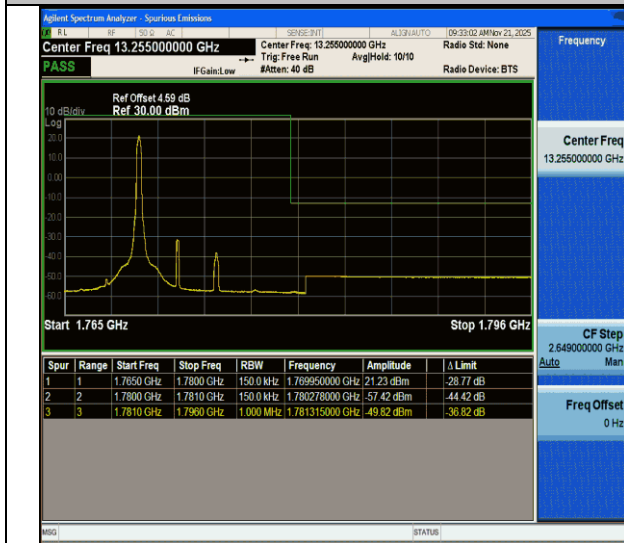
CA_66B-5MHz-10MHz-QPSK@QPSK-QPSK@QPSK-132550-132622-1RB#24@25RB#0-0RB#0@50RB#0-PASS
