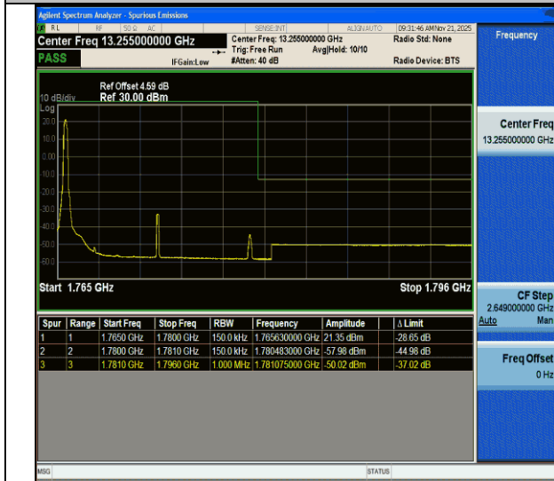
CA_66B-5MHz-10MHz-QPSK@QPSK-QPSK@QPSK-132550-132622-1RB#0@25RB#0-0RB#0@50RB#0-PASS
