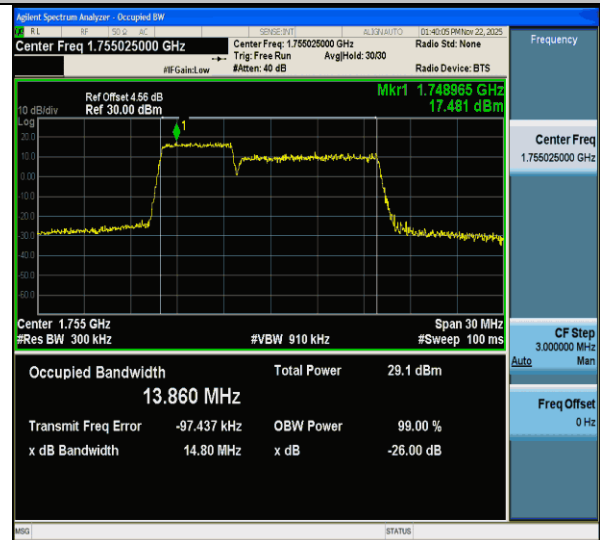
CA_66B-5MHz-10MHz-256QAM-256QAM-132375-132447-25RB#0-50RB#0-PASS
