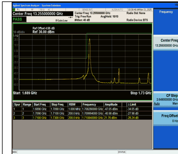
CA_66B-15MHz-5MHz-QPSK@QPSK-QPSK@QPSK-132047- 132140-1RB#0@75RB#0-0RB#0@25RB#0-PASS
