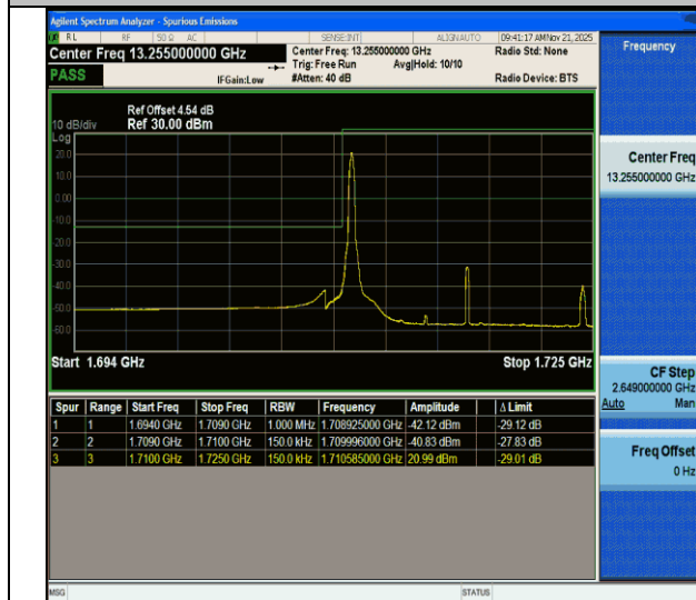
CA_66B-10MHz-5MHz-QPSK@QPSK-QPSK@QPSK-132022- 132094-1RB#0@50RB#0-0RB#0@25RB#0-PASS
