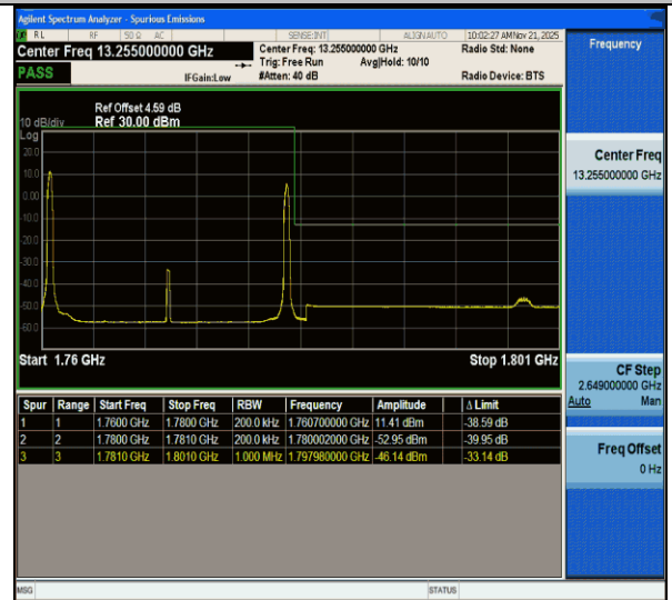
CA_66B-10MHz-10MHz-QPSK@QPSK-QPSK@QPSK-132523-132622-1RB#0@50RB#0-1RB#49@50RB#0-PASS
