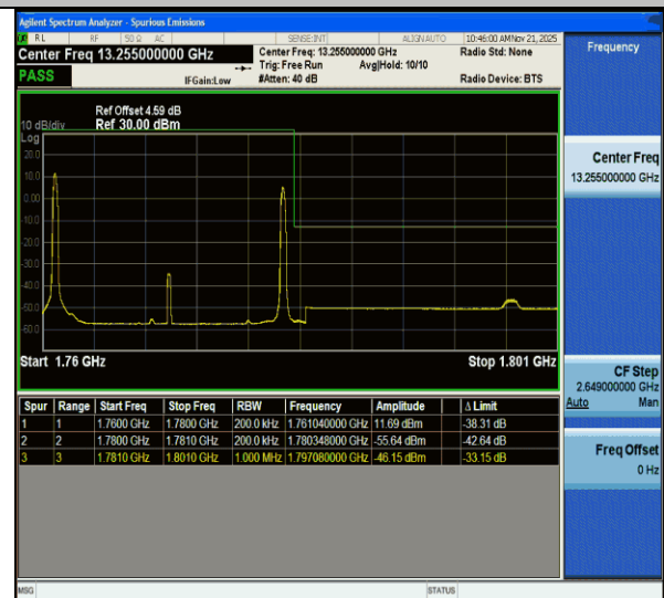
CA_66B-15MHz-5MHz-QPSK@QPSK-QPSK@QPSK-132549- 132642-1RB#0@75RB#0-1RB#24@25RB#0-PASS
