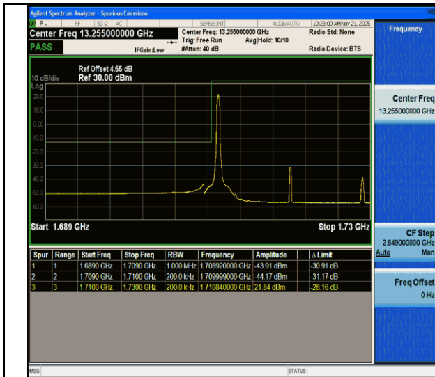
CA_66B-5MHz-15MHz-QPSK@QPSK-QPSK@QPSK-132002-132095-1RB#0@25RB#0-0RB#0@75RB#0-PASS
