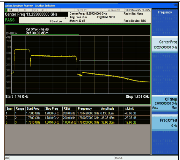
CA_66B-5MHz-15MHz-QPSK@QPSK-QPSK@QPSK-132504- 132597-25RB#0@25RB#0-75RB#0@75RB#0-PASS
