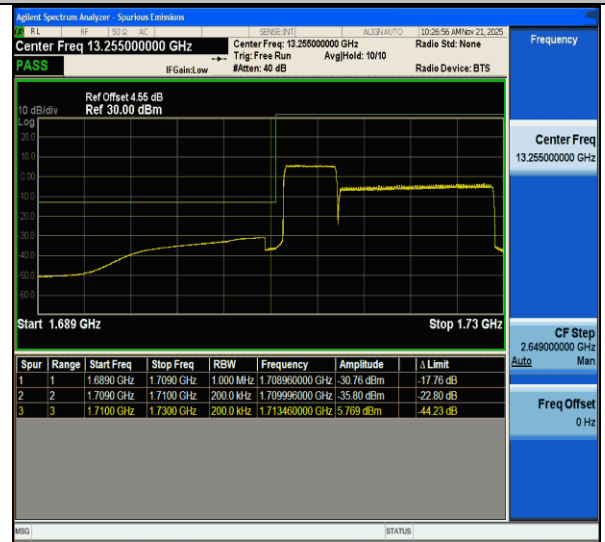
CA_66B-5MHz-15MHz-QPSK@QPSK-QPSK@QPSK-132002-132095-25RB#0@25RB#0-75RB#0@75RB#0-PASS
