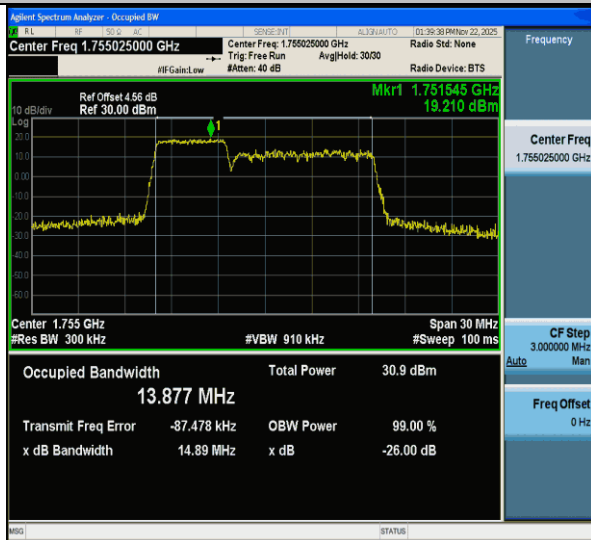
CA_66B-5MHz-10MHz-64QAM-64QAM-132375-132447-25RB#0-50RB#0-PASS
