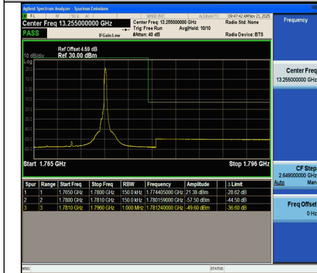
CA_66B-10MHz-5MHz-QPSK@QPSK-QPSK@QPSK-132572-132644-1RB#49@50RB#0-0RB#0@25RB#0-PASS
