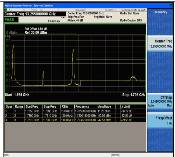
CA_66B-10MHz-5MHz-QPSK@QPSK-QPSK@QPSK-132572-132644-1RB#0@50RB#0-1RB#24@25RB#0-PASS
