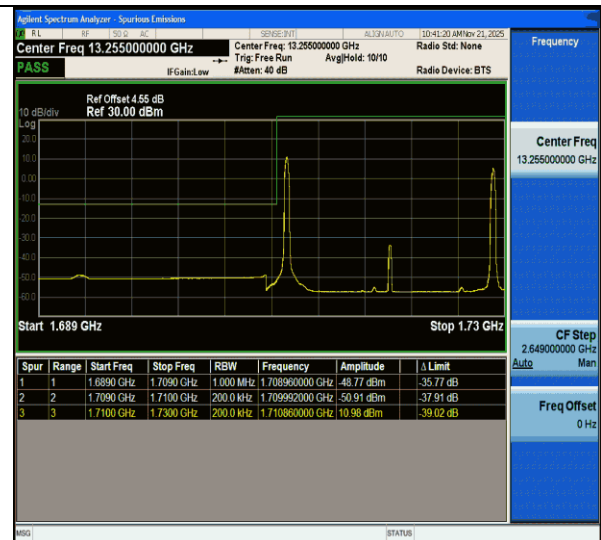
CA_66B-15MHz-5MHz-QPSK@QPSK-QPSK@QPSK-132047- 132140-1RB#0@75RB#0-1RB#24@25RB#0-PASS
