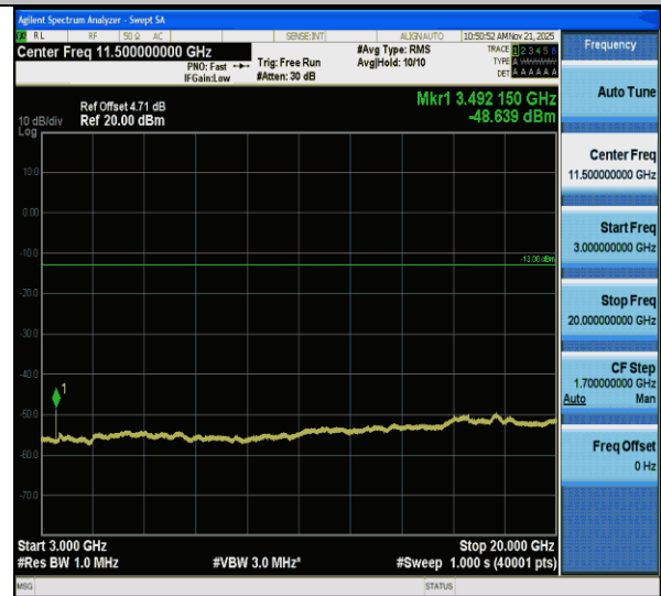
CA_66B-15MHz-5MHz-QPSK-QPSK-132398-132491-1RB#0-0RB#0-3000~20000MHz-PASS
