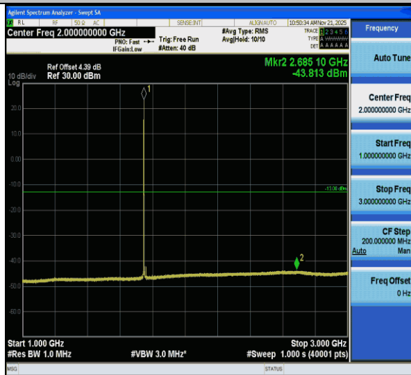
CA_66B-15MHz-5MHz-QPSK-QPSK-132398-132491-1RB#0-0RB#0-1000~3000MHz-PASS
