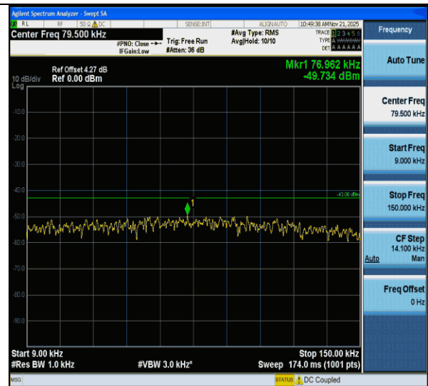
CA_66B-15MHz-5MHz-QPSK-QPSK-132398-132491-1RB#0-0RB#0-0.009~0.15MHz-PASS
