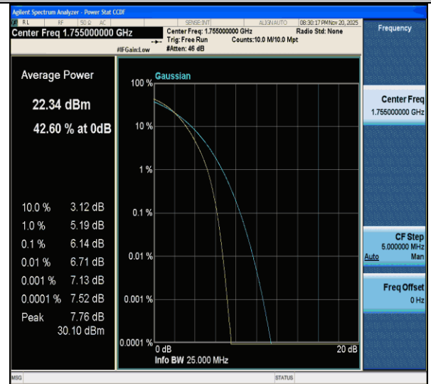
CA_66C-15MHz-15MHz-QPSK-QPSK-132347-132497-75RB#0-75RB#0-PASS
