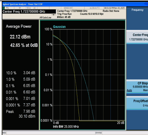
CA_66C-10MHz-20MHz-QPSK-QPSK-132027-132171-50RB#0-100RB#0-PASS
