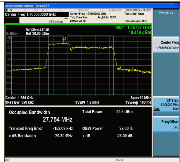
CA_66C-10MHz-20MHz-256QAM-256QAM-132428-132572-50RB#0-100RB#0-PASS
