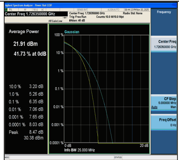
CA_66C-15MHz-20MHz-QPSK-QPSK-132050-132221-75RB#0-100RB#0-PASS
