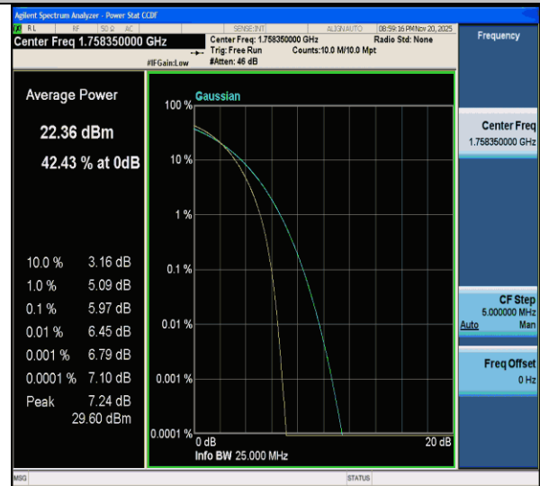
CA_66C-20MHz-5MHz-QPSK-QPSK-132397-132514-100RB#0-25RB#0-PASS
