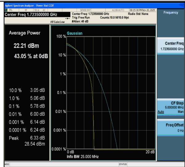
CA_66C-15MHz-10MHz-QPSK-QPSK-132047-132167-75RB#0-50RB#0-PASS
