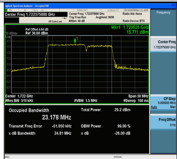
CA_66C-15MHz-10MHz-256QAM-256QAM-132047-132167-75RB#0-50RB#0-PASS
