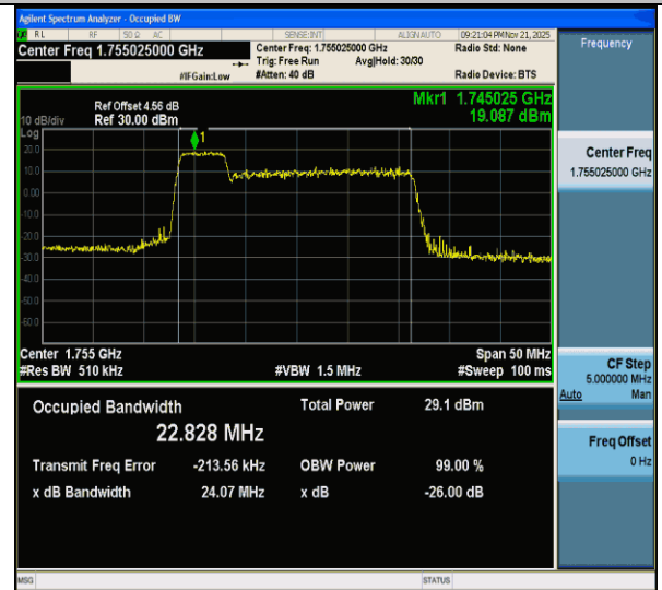
CA_66C-5MHz-20MHz-256QAM-256QAM-132330-132447-25RB#0-100RB#0-PASS
