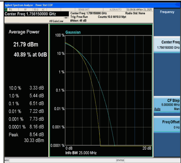
CA_66C-20MHz-15MHz-QPSK-QPSK-132348-132519-100RB#0-75RB#0-PASS
