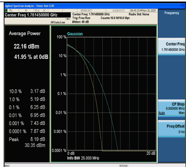
CA_66C-15MHz-20MHz-QPSK-QPSK-132401-132572-75RB#0-100RB#0-PASS
