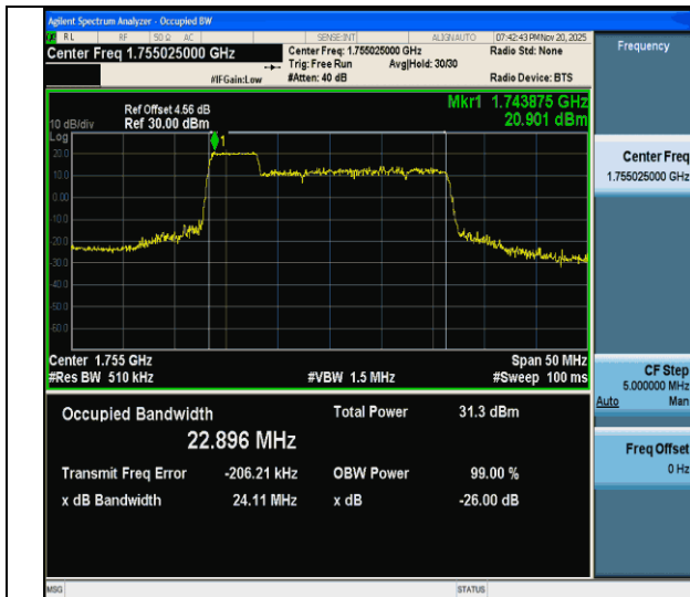
CA_66C-5MHz-20MHz-QPSK-QPSK-132330-132447-25RB#0-100RB#0-PASS
