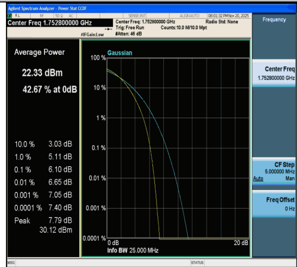
CA_66C-10MHz-20MHz-QPSK-QPSK-132328-132472-50RB#0-100RB#0-PASS
