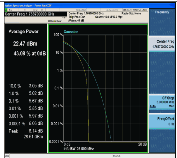
CA_66C-15MHz-10MHz-QPSK-QPSK-132499-132619-75RB#0-50RB#0-PASS
