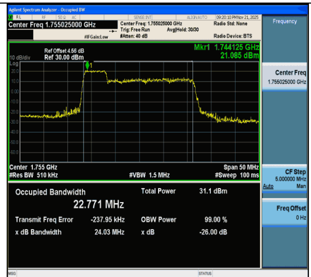
CA_66C-5MHz-20MHz-16QAM-16QAM-132330-132447-25RB#0-100RB#0-PASS
