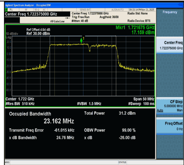
CA_66C-15MHz-10MHz-16QAM-16QAM-132047-132167-75RB#0-50RB#0-PASS
