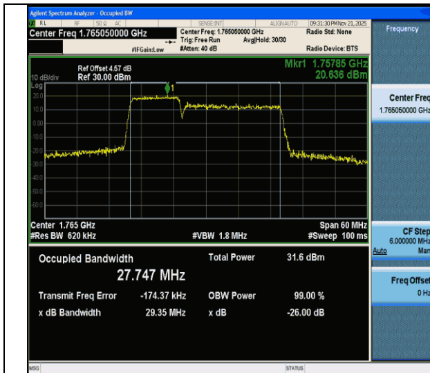
CA_66C-10MHz-20MHz-64QAM-64QAM-132428-132572-50RB#0-100RB#0-PASS
