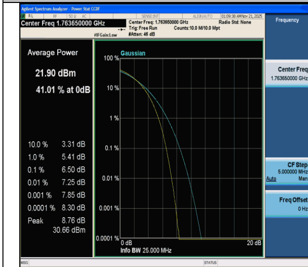
CA_66C-20MHz-15MHz-QPSK-QPSK-132423-132594-100RB#0-75RB#0-PASS
