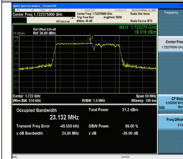
CA_66C-15MHz-10MHz-64QAM-64QAM-132047-132167-75RB#0-50RB#0-PASS
