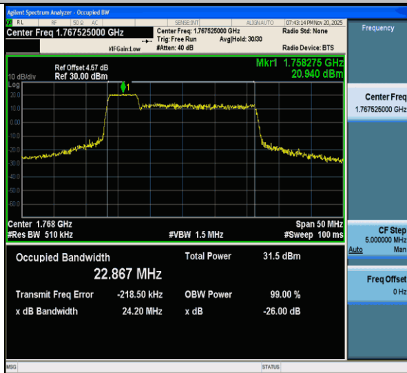
CA_66C-5MHz-20MHz-QPSK-QPSK-132455-132572-25RB#0-100RB#0-PASS
