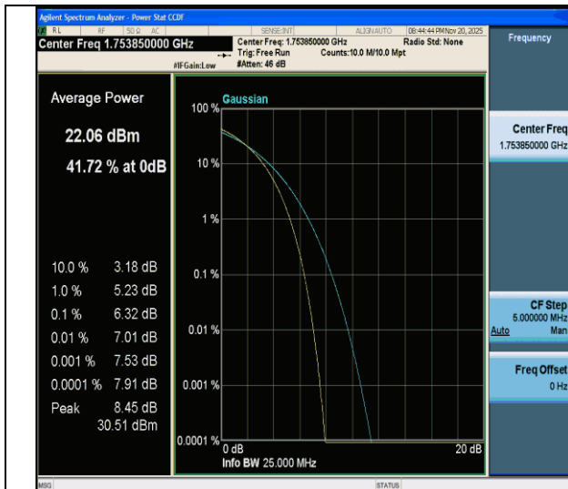
CA_66C-15MHz-20MHz-QPSK-QPSK-132325-132496-75RB#0-100RB#0-PASS
