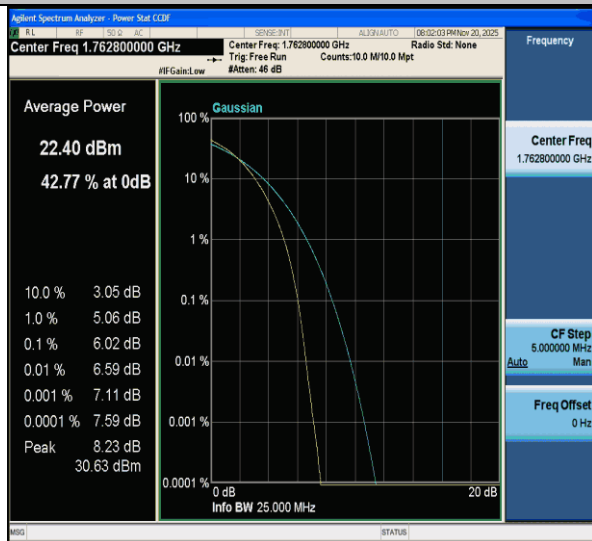
CA_66C-10MHz-20MHz-QPSK-QPSK-132428-132572-50RB#0-100RB#0-PASS
