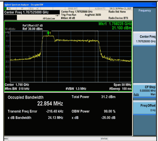
CA_66C-5MHz-20MHz-16QAM-16QAM-132455-132572-25RB#0-100RB#0-PASS
