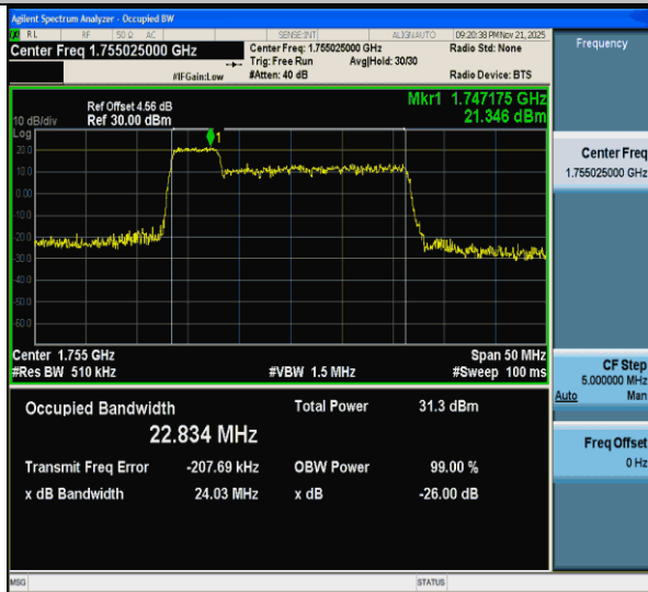
CA_66C-5MHz-20MHz-64QAM-64QAM-132330-132447-25RB#0-100RB#0-PASS
