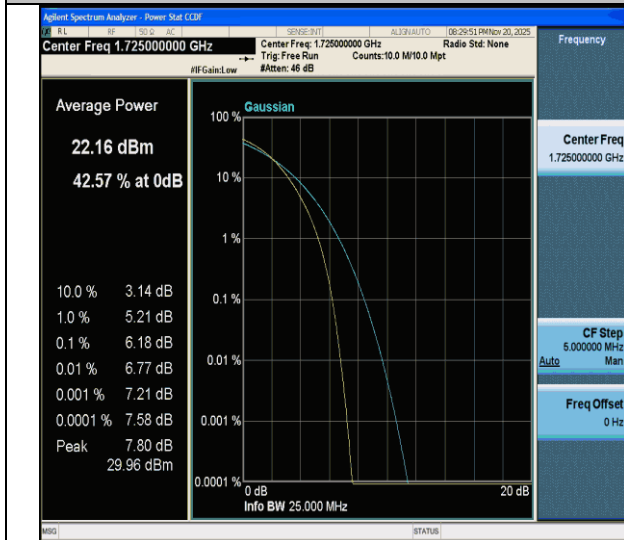
CA_66C-15MHz-15MHz-QPSK-QPSK-132047-132197-75RB#0-75RB#0-PASS
