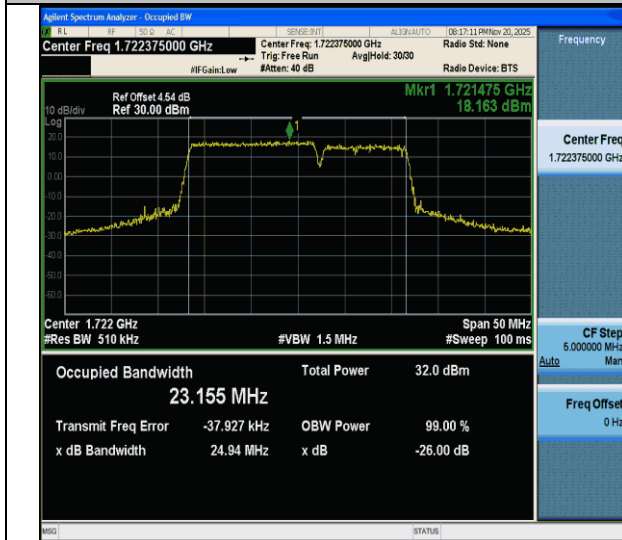
CA_66C-15MHz-10MHz-QPSK-QPSK-132047-132167-75RB#0-50RB#0-PASS
