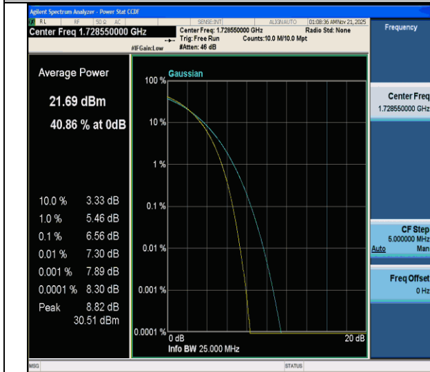
CA_66C-20MHz-15MHz-QPSK-QPSK-132072-132243-100RB#0-75RB#0-PASS
