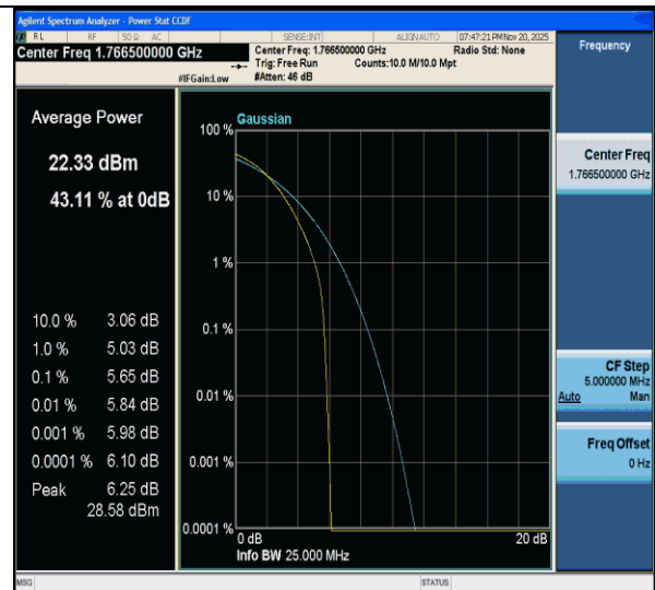
CA_66C-10MHz-15MHz-QPSK-QPSK-132477-132597-50RB#0-75RB#0-PASS
