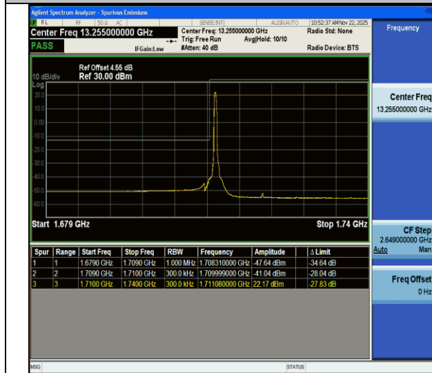
CA_66C-20MHz-10MHz-QPSK@QPSK-QPSK@QPSK-132072-132216-1RB#0@100RB#0-0RB#0@50RB#0-PASS
