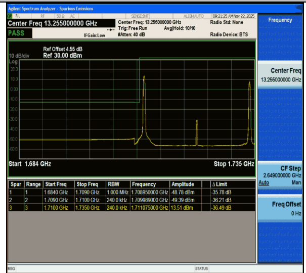
CA_66C-20MHz-5MHz-QPSK@QPSK-QPSK@QPSK-132072-132189-1RB#0@100RB#0-1RB#24@25RB#0-PASS
