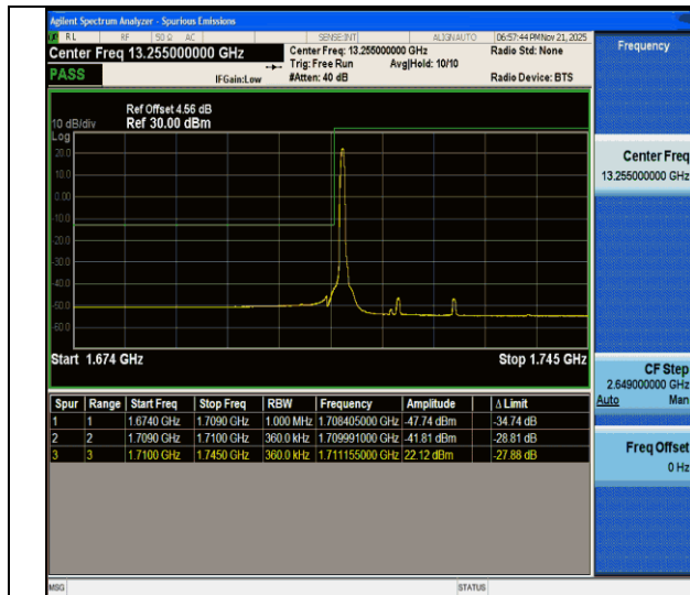
CA_66C-15MHz-20MHz-QPSK@QPSK-QPSK@QPSK-132050-132221-1RB#0@75RB#0-0RB#0@100RB#0-PASS
