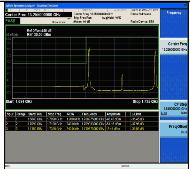
CA_66C-10MHz-15MHz-QPSK@QPSK-QPSK@QPSK-132025-132145-1RB#0@50RB#0-1RB#74@75RB#0-PASS
