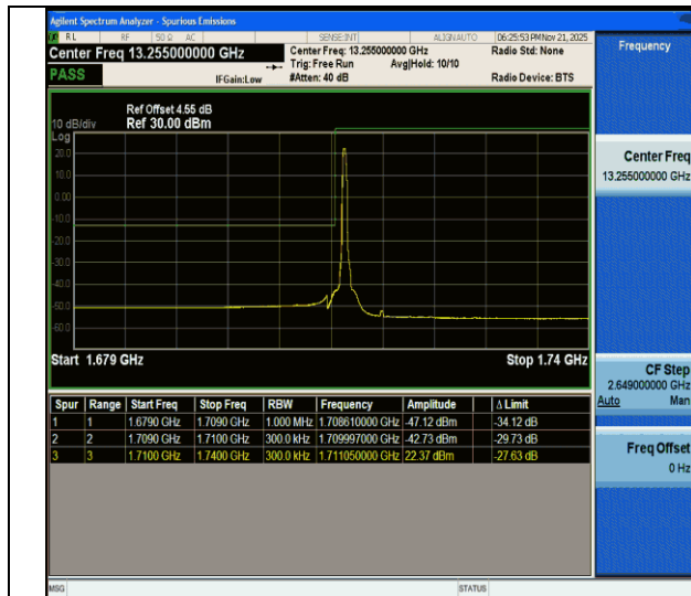
CA_66C-10MHz-20MHz-QPSK@QPSK-QPSK@QPSK-132027-132171-1RB#0@50RB#0-0RB#0@100RB#0-PASS
