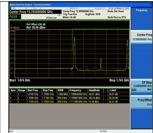
CA_66C-15MHz-20MHz-QPSK@QPSK-QPSK@QPSK-132050-132221-1RB#0@75RB#0-1RB#99@100RB#0-PASS
