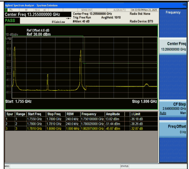
CA_66C-10MHz-15MHz-QPSK@QPSK-QPSK@QPSK-132477-132597-1RB#0@50RB#0-1RB#74@75RB#0-PASS
