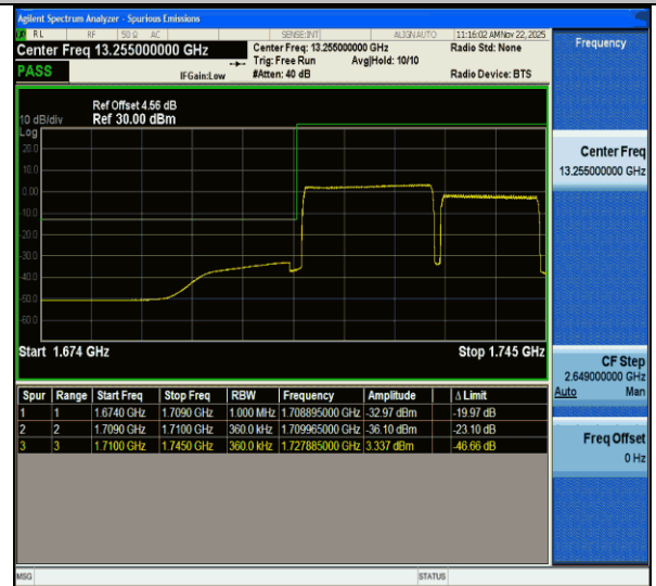
CA_66C-20MHz-15MHz-QPSK@QPSK-QPSK@QPSK-132072-132243-100RB#0@100RB#0-75RB#0@75RB#0-PASS
