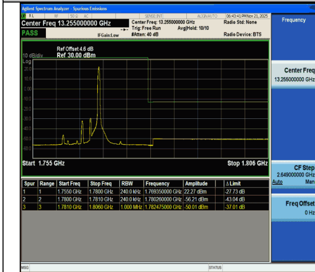
CA_66C-15MHz-10MHz-QPSK@QPSK-QPSK@QPSK-132499-132619-1RB#74@75RB#0-0RB#0@50RB#0-PASS
