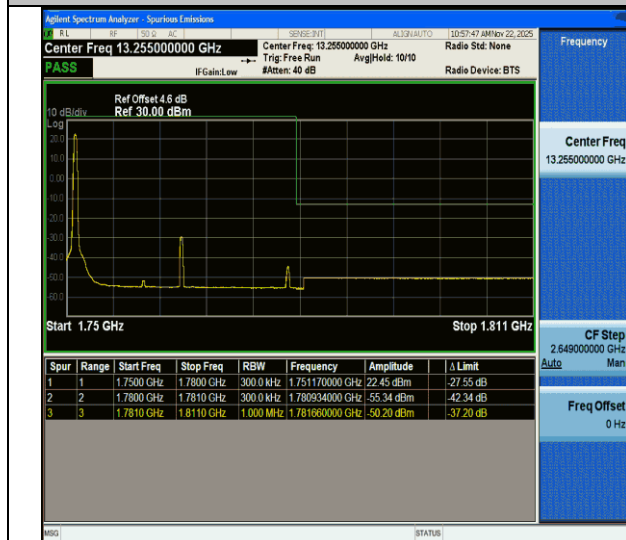
CA_66C-20MHz-10MHz-QPSK@QPSK-QPSK@QPSK-132473-132617-1RB#0@100RB#0-0RB#0@50RB#0-PASS
