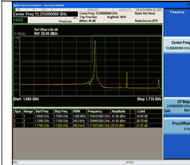
CA_66C-20MHz-5MHz-QPSK@QPSK-QPSK@QPSK-132072-132189-1RB#0@100RB#0-0RB#0@25RB#0-PASS
