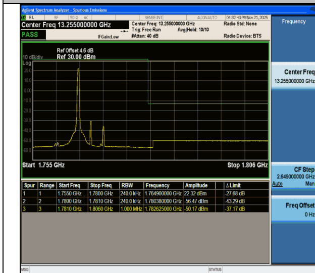
CA_66C-10MHz-15MHz-QPSK@QPSK-QPSK@QPSK-132477-132597-1RB#49@50RB#0-0RB#0@75RB#0-PASS
