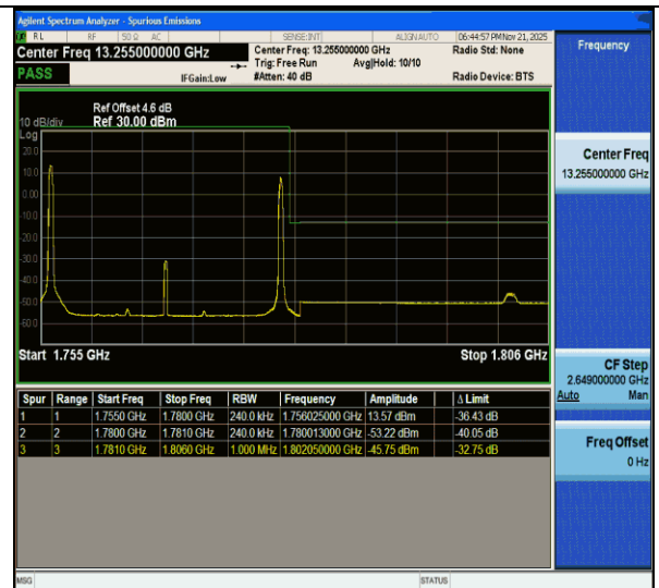
CA_66C-15MHz-10MHz-QPSK@QPSK-QPSK@QPSK-132499-132619-1RB#0@75RB#0-1RB#49@50RB#0-PASS
