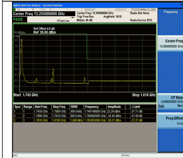
CA_66C-15MHz-20MHz-QPSK@QPSK-QPSK@QPSK-132401-132572-1RB#0@75RB#0-0RB#0@100RB#0-PASS
