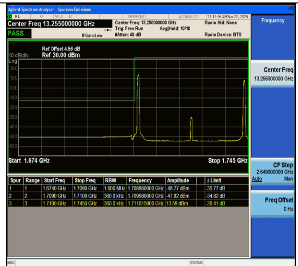
CA_66C-20MHz-15MHz-QPSK@QPSK-QPSK@QPSK-132072-132243-1RB#0@100RB#0-1RB#74@75RB#0-PASS
