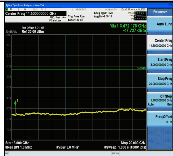
CA_66C-20MHz-20MHz-QPSK-QPSK-132323-132521-1RB#0- ORB#0-3000~20000MHz-PASS
