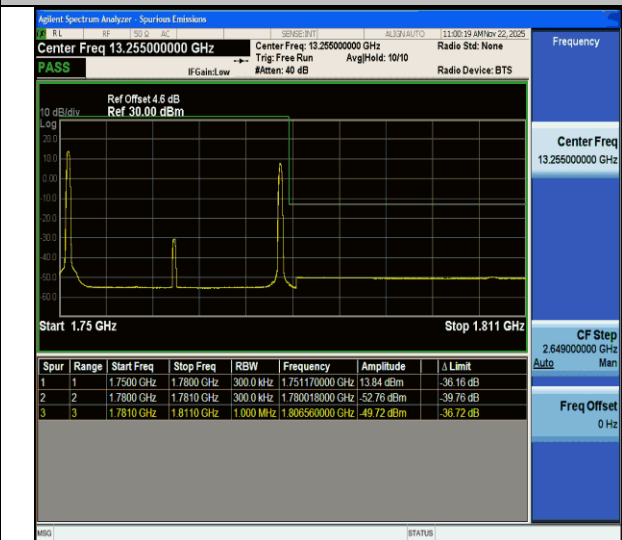
CA_66C-20MHz-10MHz-QPSK@QPSK-QPSK@QPSK-132473-132617-1RB#0@100RB#0-1RB#49@50RB#0-PASS
