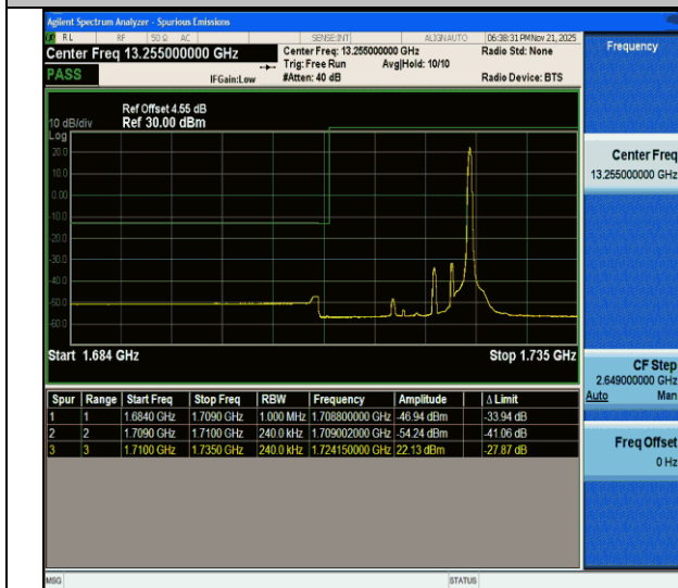
CA_66C-15MHz-10MHz-QPSK@QPSK-QPSK@QPSK-132047-132167-1RB#74@75RB#0-0RB#0@50RB#0-PASS
