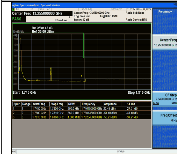
CA_66C-20MHz-15MHz-QPSK@QPSK-QPSK@QPSK-132423-132594-1RB#0@100RB#0-0RB#0@75RB#0-PASS
