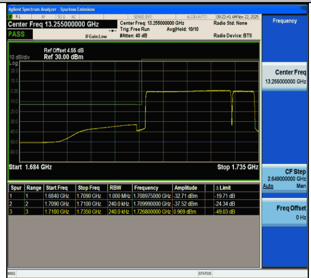
CA_66C-20MHz-5MHz-QPSK@QPSK-QPSK@QPSK-132072-132189-100RB#0@100RB#0-25RB#0@25RB#0-PASS
