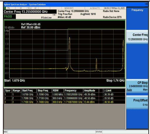
CA_66C-15MHz-15MHz-QPSK@QPSK-QPSK@QPSK-132047-132197-1RB#0@75RB#0-1RB#74@75RB#0-PASS
