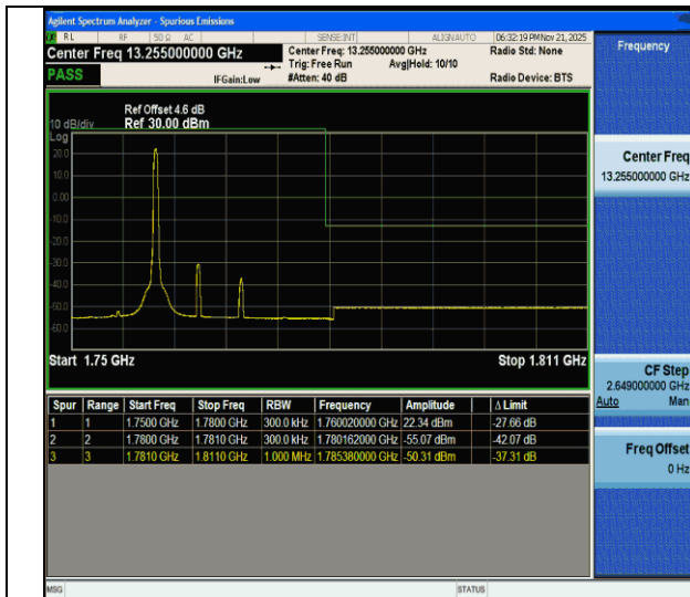
CA_66C-10MHz-20MHz-QPSK@QPSK-QPSK@QPSK-132428-132572-1RB#49@50RB#0-0RB#0@100RB#0-PASS
