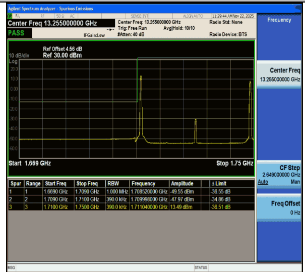
CA_66C-20MHz-20MHz-QPSK@QPSK-QPSK@QPSK-132072-132270-1RB#0@100RB#0-1RB#99@100RB#0-PASS
