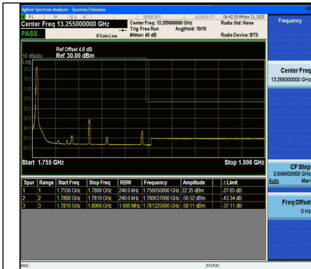
CA_66C-15MHz-10MHz-QPSK@QPSK-QPSK@QPSK-132499-132619-1RB#0@75RB#0-0RB#0@50RB#0-PASS
