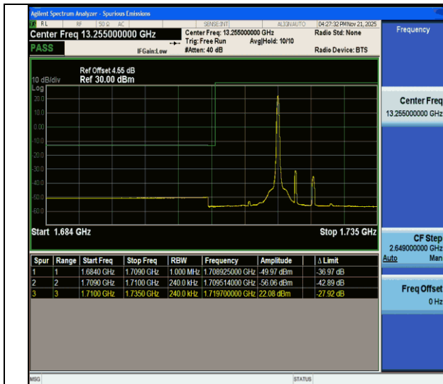
CA_66C-10MHz-15MHz-QPSK@QPSK-QPSK@QPSK-132025-132145-1RB#49@50RB#0-0RB#0@75RB#0-PASS
