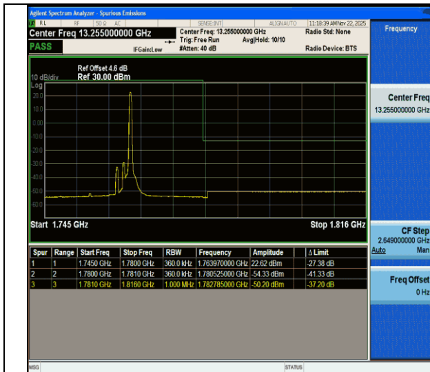
CA_66C-20MHz-15MHz-QPSK@QPSK-QPSK@QPSK-132423-132594-1RB#99@100RB#0-0RB#0@75RB#0-PASS
