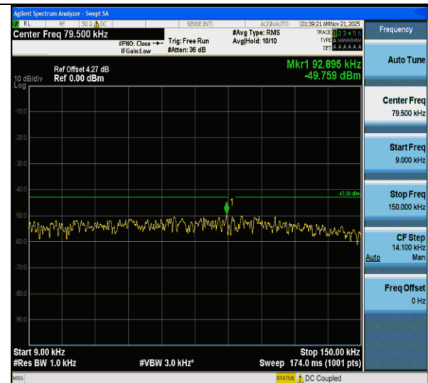
CA_66C-20MHz-20MHz-QPSK-QPSK-132323-132521-1RB#0- ORB#0-0.009~0.15MHz-PASS
