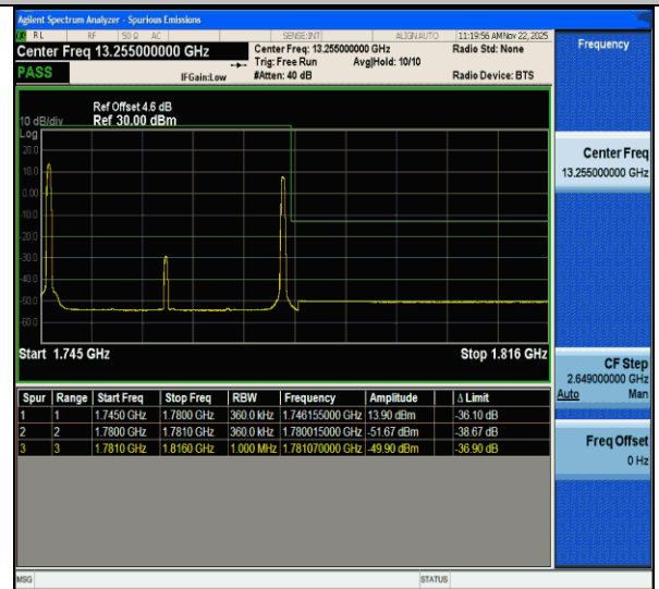
CA_66C-20MHz-15MHz-QPSK@QPSK-QPSK@QPSK-132423-132594-1RB#0@100RB#0-1RB#74@75RB#0-PASS
