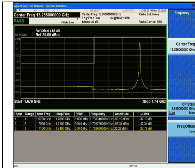
CA_66C-20MHz-10MHz-QPSK@QPSK-QPSK@QPSK-132072-132216-1RB#99@100RB#0-0RB#0@50RB#0-PASS
