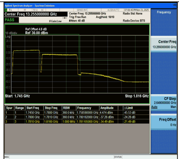
CA_66C-15MHz-20MHz-QPSK@QPSK-QPSK@QPSK-132401-132572-75RB#0@75RB#0-100RB#0@100RB#0-PASS
