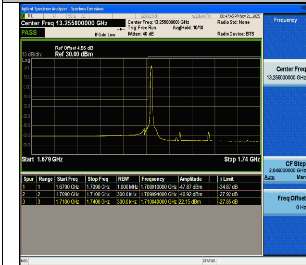
CA_66C-15MHz-15MHz-QPSK@QPSK-QPSK@QPSK-132047-132197-1RB#0@75RB#0-0RB#0@75RB#0-PASS
