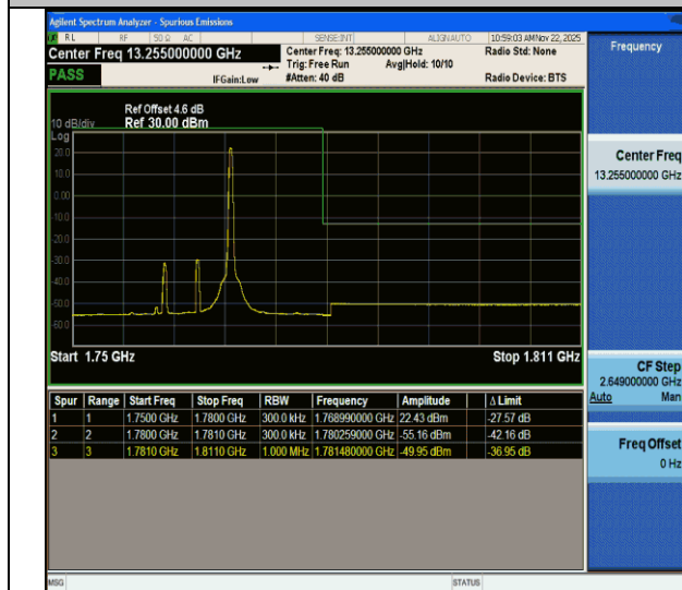
CA_66C-20MHz-10MHz-QPSK@QPSK-QPSK@QPSK-132473-132617-1RB#99@100RB#0-0RB#0@50RB#0-PASS
