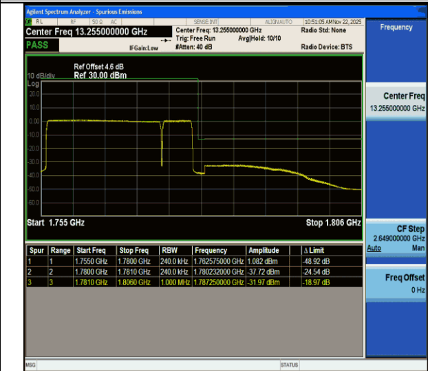
CA_66C-20MHz-5MHz-QPSK@QPSK-QPSK@QPSK-132522-132572-100RB#0@100RB#0-25RB#0@25RB#0-PASS
