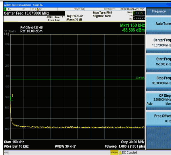
CA_66C-20MHz-20MHz-QPSK-QPSK-132323-132521-1RB#0- ORB#0-0.15~30MHz-PASS
