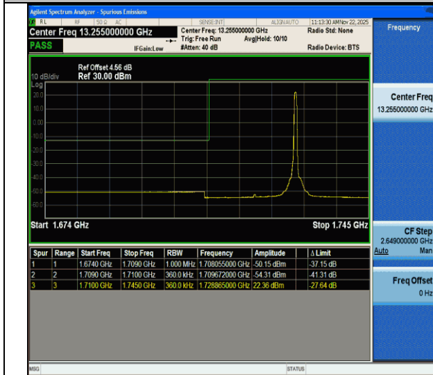
CA_66C-20MHz-15MHz-QPSK@QPSK-QPSK@QPSK-132072-132243-1RB#99@100RB#0-0RB#0@75RB#0-PASS
