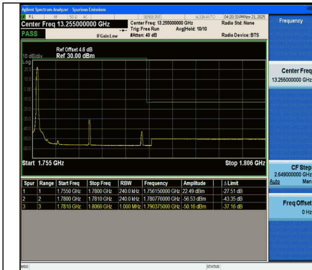
CA_66C-5MHz-20MHz-QPSK@QPSK-QPSK@QPSK-132455-132572-1RB#0@25RB#0-0RB#0@100RB#0-PASS
