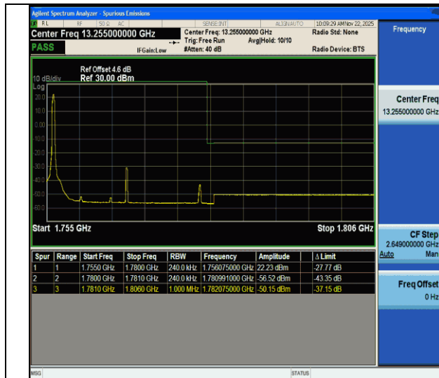
CA_66C-20MHz-5MHz-QPSK@QPSK-QPSK@QPSK-132522-132572-1RB#0@100RB#0-0RB#0@25RB#0-PASS
