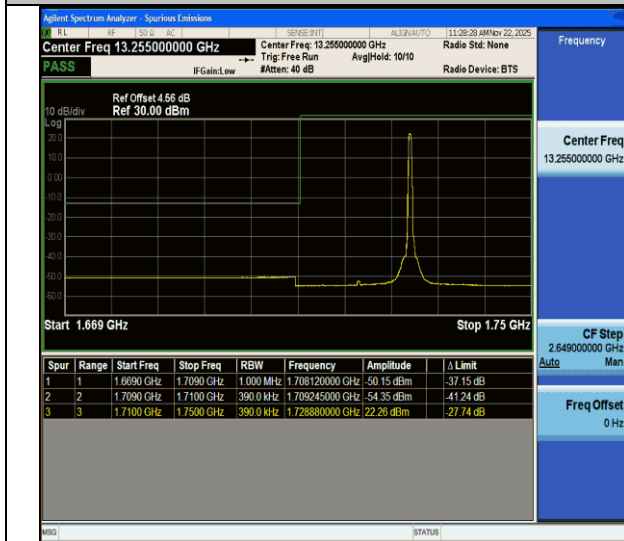
CA_66C-20MHz-20MHz-QPSK@QPSK-QPSK@QPSK-132072-132270-1RB#99@100RB#0-0RB#0@100RB#0-PASS
