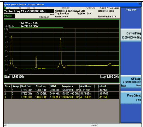
CA_66C-5MHz-20MHz-QPSK@QPSK-QPSK@QPSK-132455-132572-1RB#0@25RB#0-1RB#99@100RB#0-PASS
