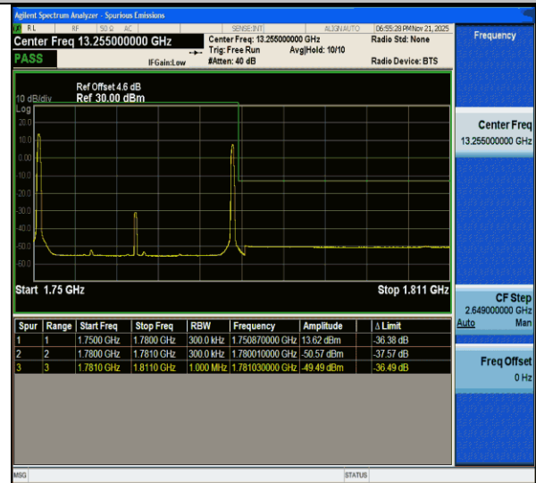
CA_66C-15MHz-15MHz-QPSK@QPSK-QPSK@QPSK-132447-132597-1RB#0@75RB#0-1RB#74@75RB#0-PASS
