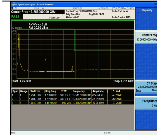
CA_66C-10MHz-20MHz-QPSK@QPSK-QPSK@QPSK-132428-132572-1RB#0@50RB#0-0RB#0@100RB#0-PASS
