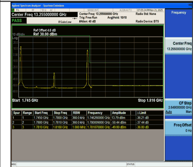
CA_66C-15MHz-20MHz-QPSK@QPSK-QPSK@QPSK-132401-132572-1RB#0@75RB#0-1RB#99@100RB#0-PASS
