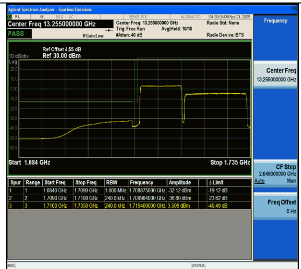
CA_66C-10MHz-15MHz-QPSK@QPSK-QPSK@QPSK-132025-132145-50RB#0@50RB#0-75RB#0@75RB#0-PASS
