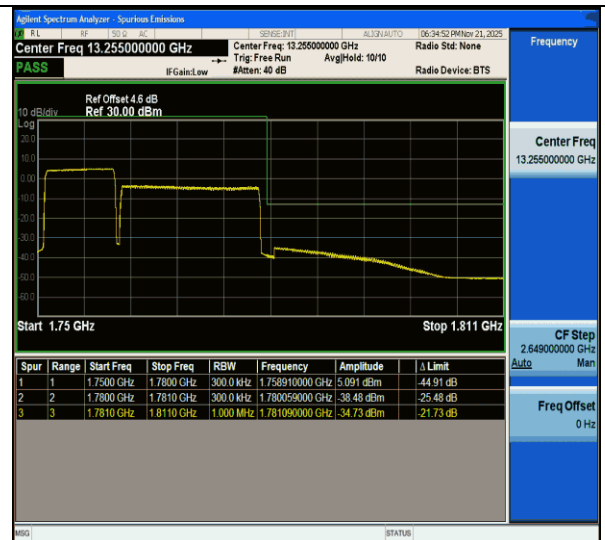
CA_66C-10MHz-20MHz-QPSK@QPSK-QPSK@QPSK-132428-132572-50RB#0@50RB#0-100RB#0@100RB#0-PASS
