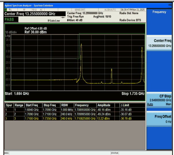
CA_66C-15MHz-10MHz-QPSK@QPSK-QPSK@QPSK-132047-132167-1RB#0@75RB#0-1RB#49@50RB#0-PASS
