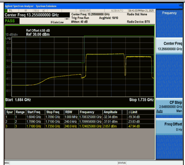
CA_66C-15MHz-10MHz-QPSK@QPSK-QPSK@QPSK-132047-132167-75RB#0@75RB#0-50RB#0@50RB#0-PASS
