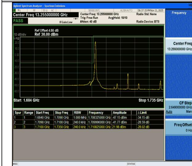
CA_66C-15MHz-10MHz-QPSK@QPSK-QPSK@QPSK-132047-132167-1RB#0@75RB#0-0RB#0@50RB#0-PASS
