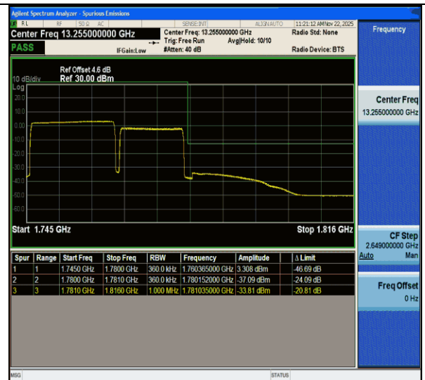
CA_66C-20MHz-15MHz-QPSK@QPSK-QPSK@QPSK-132423-132594-100RB#0@100RB#0-75RB#0@75RB#0-PASS
