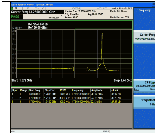
CA_66C-15MHz-15MHz-QPSK@QPSK-QPSK@QPSK-132047-132197-1RB#74@75RB#0-0RB#0@75RB#0-PASS
