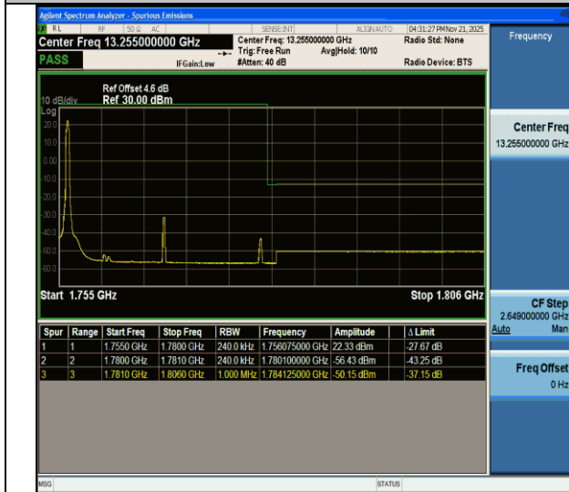
CA_66C-10MHz-15MHz-QPSK@QPSK-QPSK@QPSK-132477-132597-1RB#0@50RB#0-0RB#0@75RB#0-PASS
