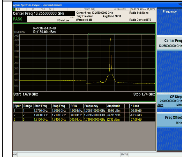
CA_66C-10MHz-20MHz-QPSK@QPSK-QPSK@QPSK-132027-132171-1RB#49@50RB#0-0RB#0@100RB#0-PASS
