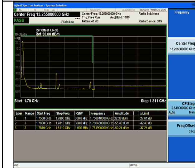
CA_66C-15MHz-15MHz-QPSK@QPSK-QPSK@QPSK-132447-132597-1RB#0@75RB#0-0RB#0@75RB#0-PASS
