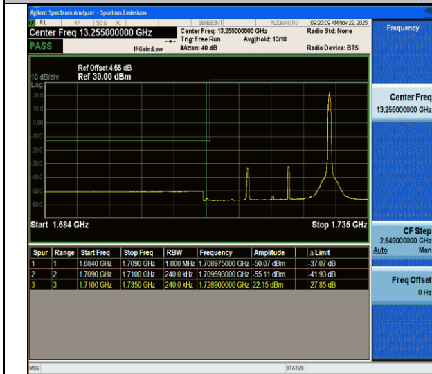
CA_66C-20MHz-5MHz-QPSK@QPSK-QPSK@QPSK-132072-132189-1RB#99@100RB#0-0RB#0@25RB#0-PASS
