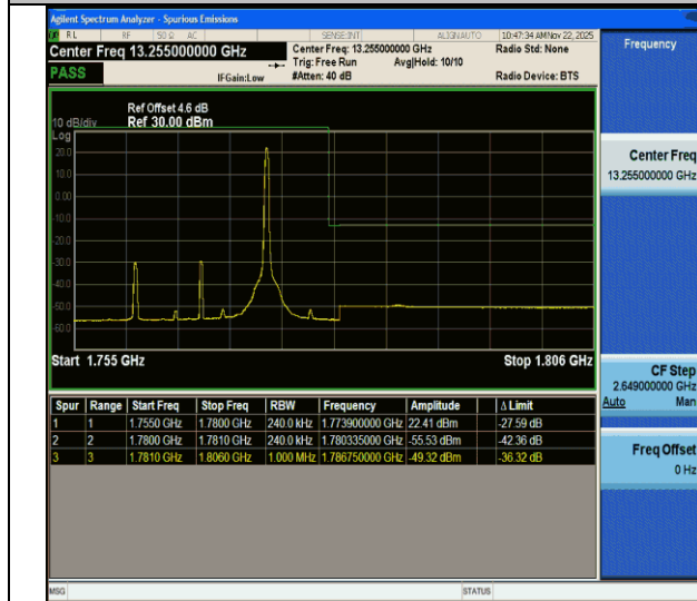
CA_66C-20MHz-5MHz-QPSK@QPSK-QPSK@QPSK-132522-132572-1RB#99@100RB#0-0RB#0@25RB#0-PASS
