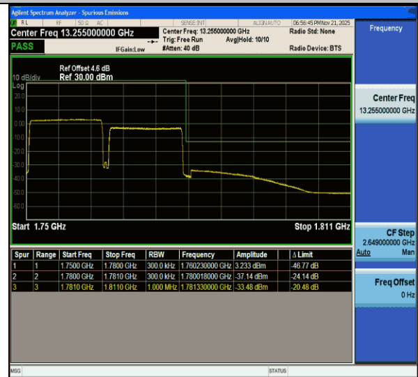
CA_66C-15MHz-15MHz-QPSK@QPSK-QPSK@QPSK-132447-132597-75RB#0@75RB#0-75RB#0@75RB#0-PASS
