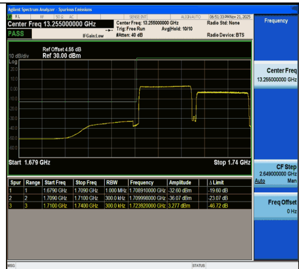
CA_66C-15MHz-15MHz-QPSK@QPSK-QPSK@QPSK-132047-132197-75RB#0@75RB#0-75RB#0@75RB#0-PASS
