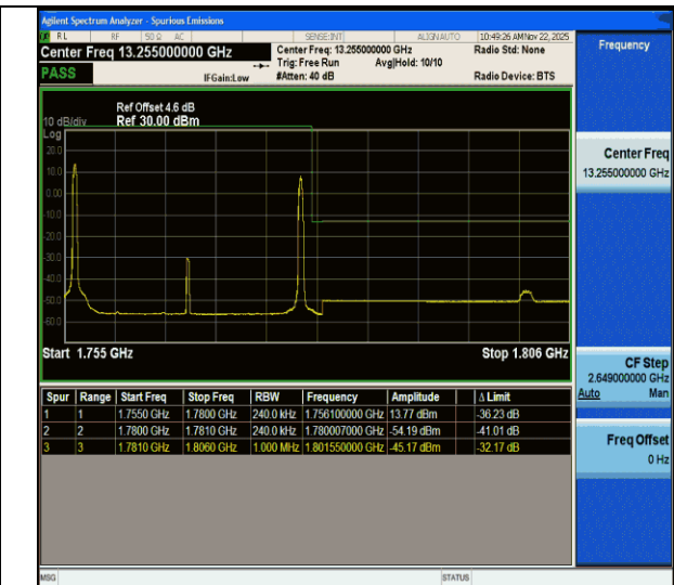
CA_66C-20MHz-5MHz-QPSK@QPSK-QPSK@QPSK-132522-132572-1RB#0@100RB#0-1RB#24@25RB#0-PASS
