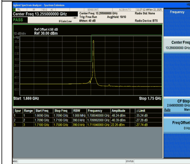
CA_66C-20MHz-20MHz-QPSK@QPSK-QPSK@QPSK-132072-132270-1RB#0@100RB#0-0RB#0@100RB#0-PASS
