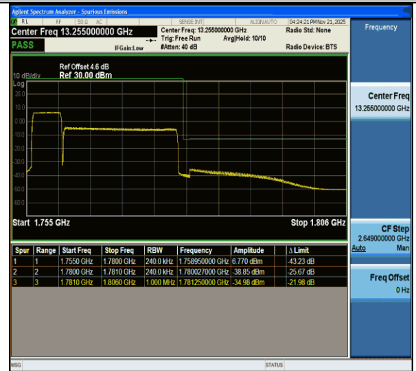
CA_66C-5MHz-20MHz-QPSK@QPSK-QPSK@QPSK-132455-132572-25RB#0@25RB#0-100RB#0@100RB#0-PASS
