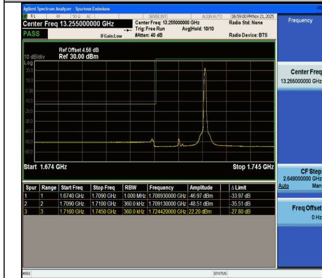
CA_66C-15MHz-20MHz-QPSK@QPSK-QPSK@QPSK-132050-132221-1RB#74@75RB#0-0RB#0@100RB#0-PASS
