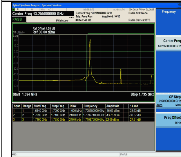
CA_66C-10MHz-15MHz-QPSK@QPSK-QPSK@QPSK-132025-132145-1RB#0@50RB#0-0RB#0@75RB#0-PASS
