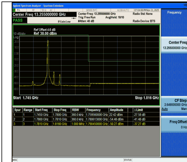
CA_66C-15MHz-20MHz-QPSK@QPSK-QPSK@QPSK-132401-132572-1RB#74@75RB#0-0RB#0@100RB#0-PASS
