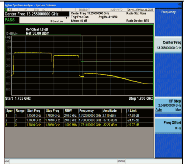
CA_66C-15MHz-10MHz-QPSK@QPSK-QPSK@QPSK-132499-132619-75RB#0@75RB#0-50RB#0@50RB#0-PASS
