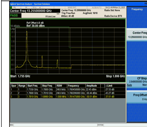
CA_66C-5MHz-20MHz-QPSK@QPSK-QPSK@QPSK-132455-132572-1RB#24@25RB#0-0RB#0@100RB#0-PASS
