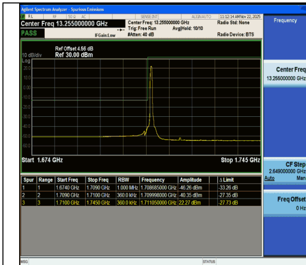
CA_66C-20MHz-15MHz-QPSK@QPSK-QPSK@QPSK-132072-132243-1RB#0@100RB#0-0RB#0@75RB#0-PASS
