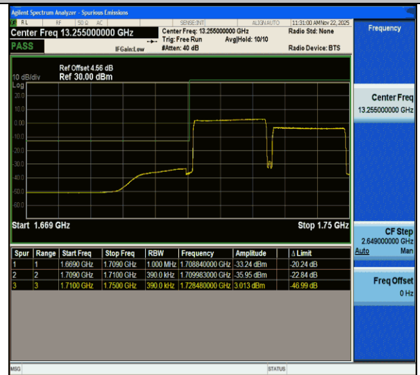
CA_66C-20MHz-20MHz-QPSK@QPSK-QPSK@QPSK-132072-132270-100RB#0@100RB#0-100RB#0@100RB#0-PASS
