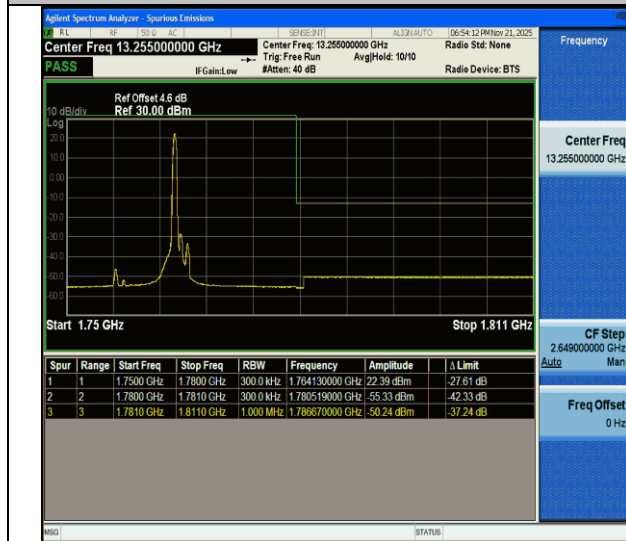
CA_66C-15MHz-15MHz-QPSK@QPSK-QPSK@QPSK-132447-132597-1RB#74@75RB#0-0RB#0@75RB#0-PASS
