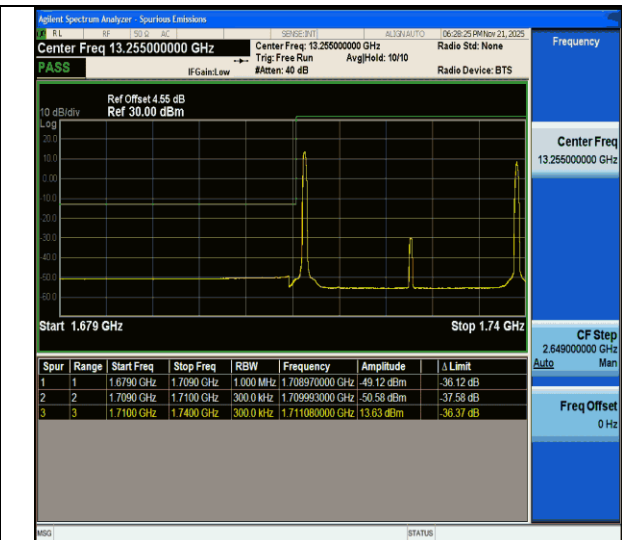
CA_66C-10MHz-20MHz-QPSK@QPSK-QPSK@QPSK-132027-132171-1RB#0@50RB#0-1RB#99@100RB#0-PASS
