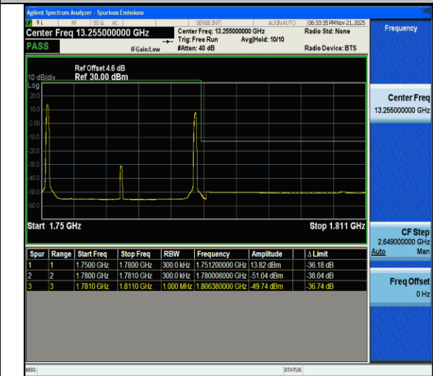
CA_66C-10MHz-20MHz-QPSK@QPSK-QPSK@QPSK-132428-132572-1RB#0@50RB#0-1RB#99@100RB#0-PASS
