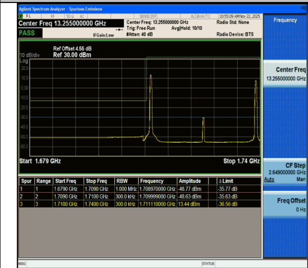
CA_66C-20MHz-10MHz-QPSK@QPSK-QPSK@QPSK-132072-132216-1RB#0@100RB#0-1RB#49@50RB#0-PASS
