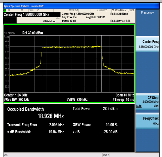
NTNV-n2-PC3-15-20-L-CP-16QAM-Outer_Full-Ant1-PASS
