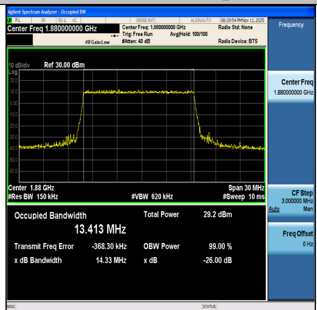
NTNV-n2-PC3-15-15-M-DFT-256QAM-Outer_Full-Ant1-PASS
