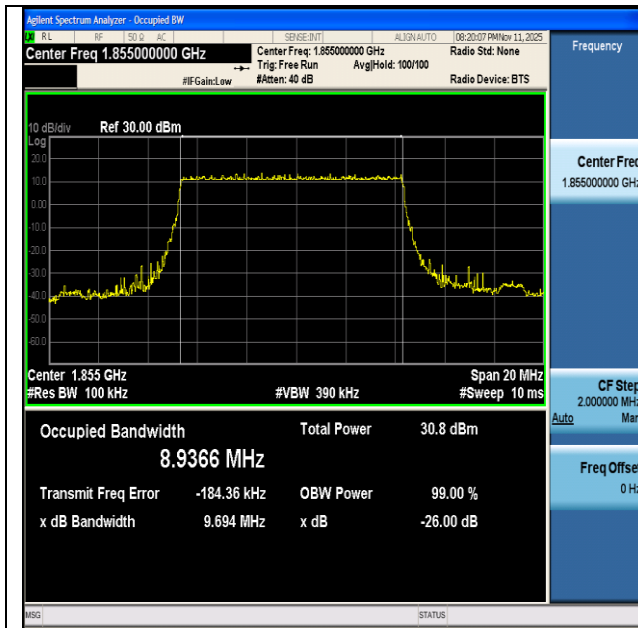
NTNV-n2-PC3-15-10-L-DFT-QPSK-Outer_Full-Ant1-PASS
