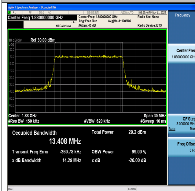
NTNV-n2-PC3-15-15-M-DFT-64QAM-Outer_Full-Ant1-PASS
