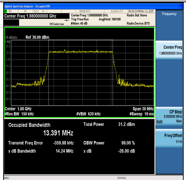
NTNV-n2-PC3-15-15-M-DFT-BPSK-Outer_Full-Ant1-PASS
