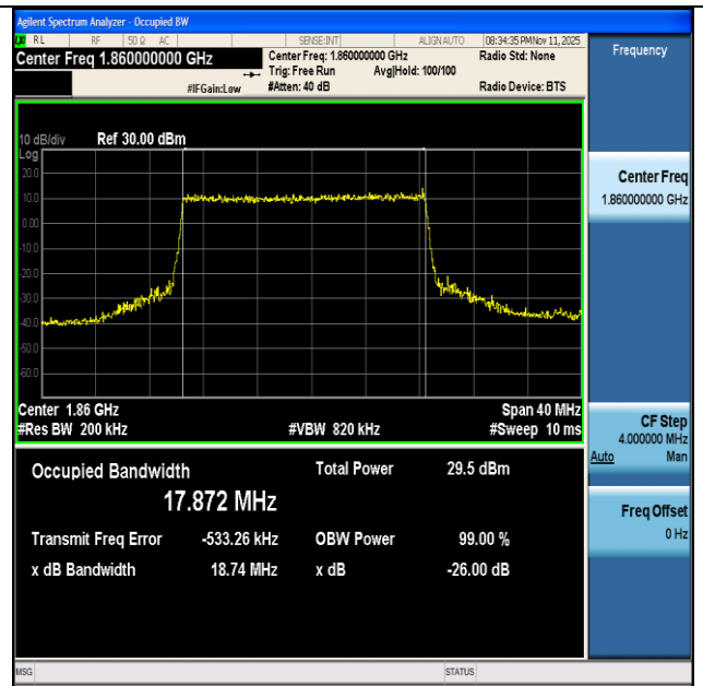
NTNV-n2-PC3-15-20-L-DFT-256QAM-Outer_Full-Ant1-PASS
