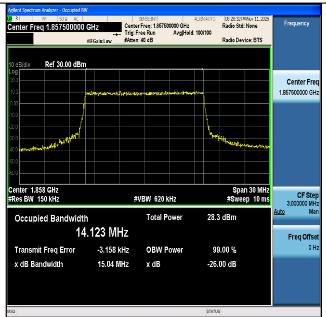
NTNV-n2-PC3-15-15-L-CP-64QAM-Outer_Full-Ant1-PASS
