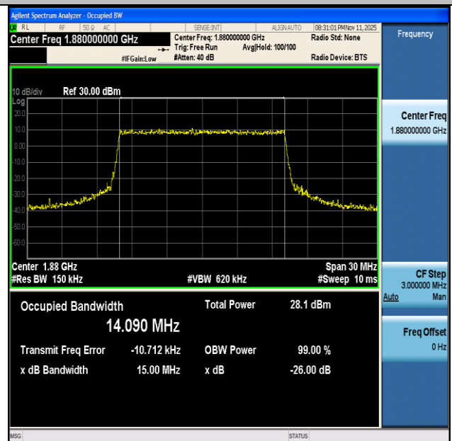
NTVN-n2-PC3-15-15-M-CP-256QAM-Outer_Full-Ant1-PASS
