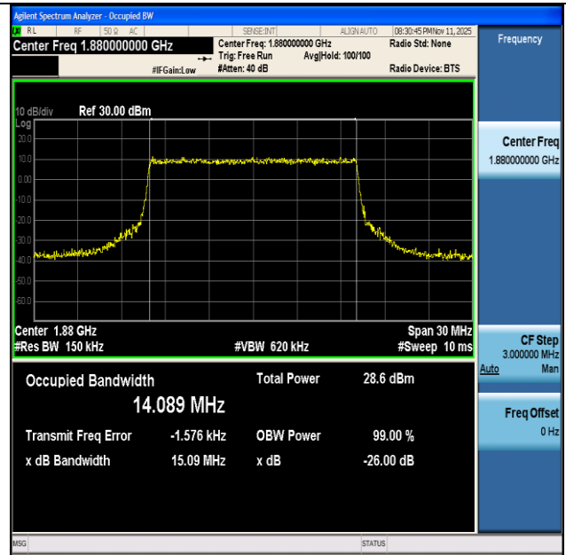
NTVN-n2-PC3-15-15-M-CP-16QAM-Outer_Full-Ant1-PASS
