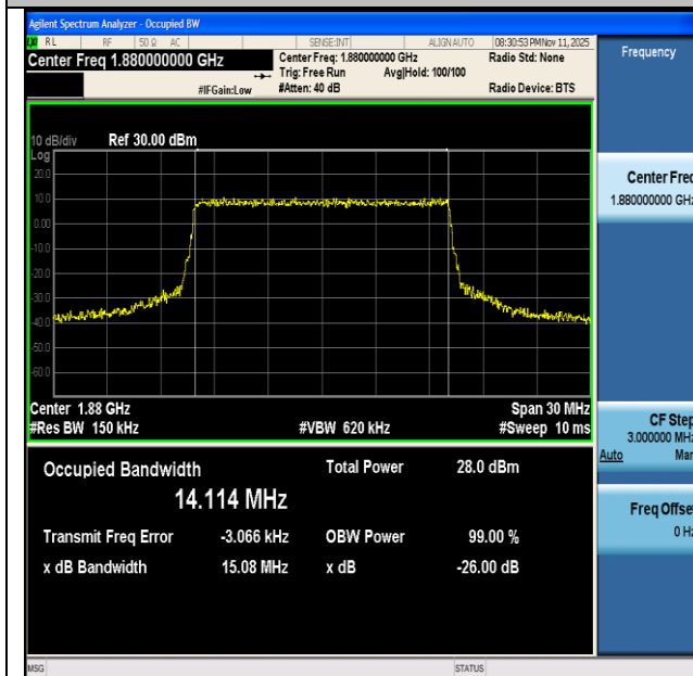
NTVN-n2-PC3-15-15-M-CP-64QAM-Outer_Full-Ant1-PASS
