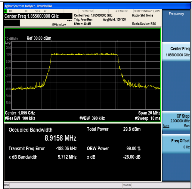
NTNV-n2-PC3-15-10-L-DFT-16QAM-Outer_Full-Ant1-PASS
