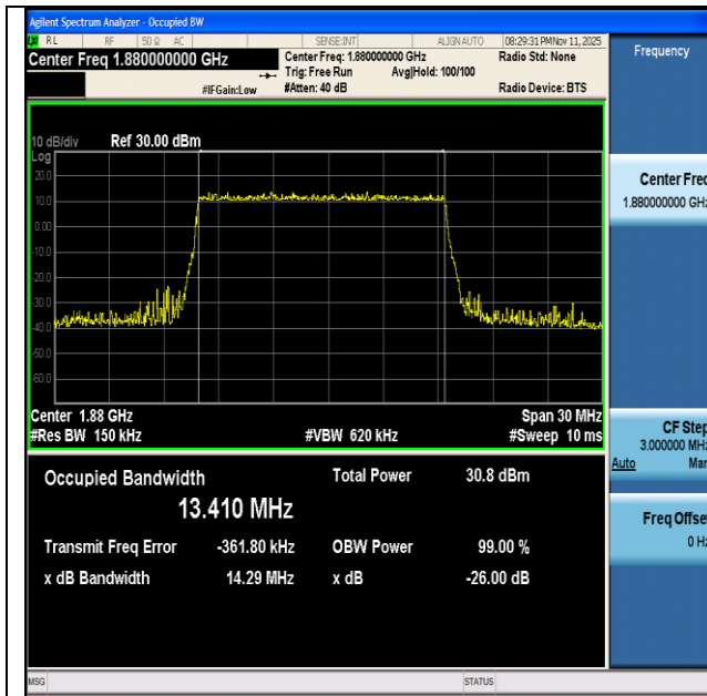
NTNV-n2-PC3-15-15-M-DFT-QPSK-Outer_Full-Ant1-PASS
