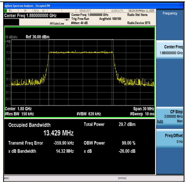
NTNV-n2-PC3-15-15-M-DFT-16QAM-Outer_Full-Ant1-PASS
