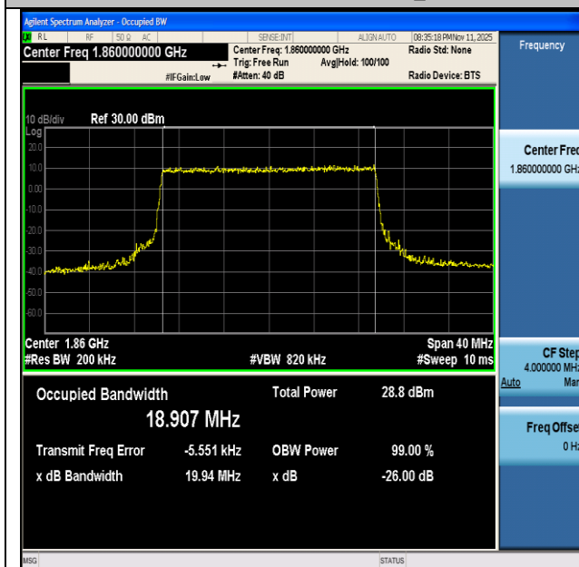
NTNV-n2-PC3-15-20-L-CP-QPSK-Outer_Full-Ant1-PASS
