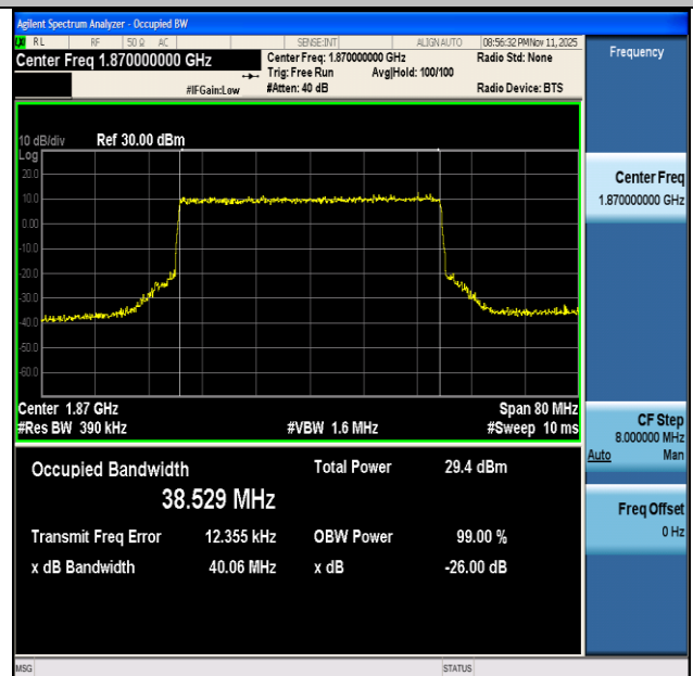
NTNV-n2-PC3-15-40-L-CP-QPSK-Outer_Full-Ant1-PASS
