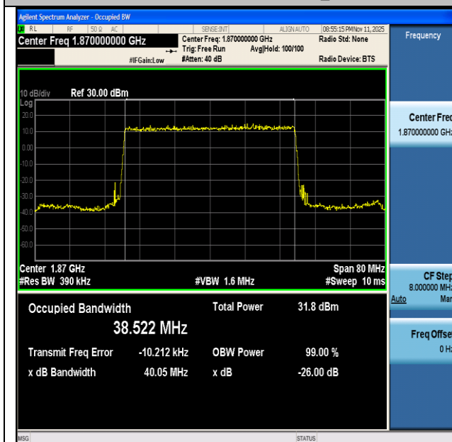
NTNV-n2-PC3-15-40-L-DFT-BPSK-Outer_Full-Ant1-PASS
