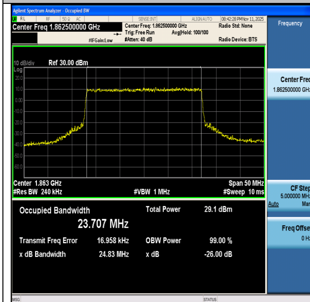
NTNV-n2-PC3-15-25-L-CP-16QAM-Outer_Full-Ant1-PASS
