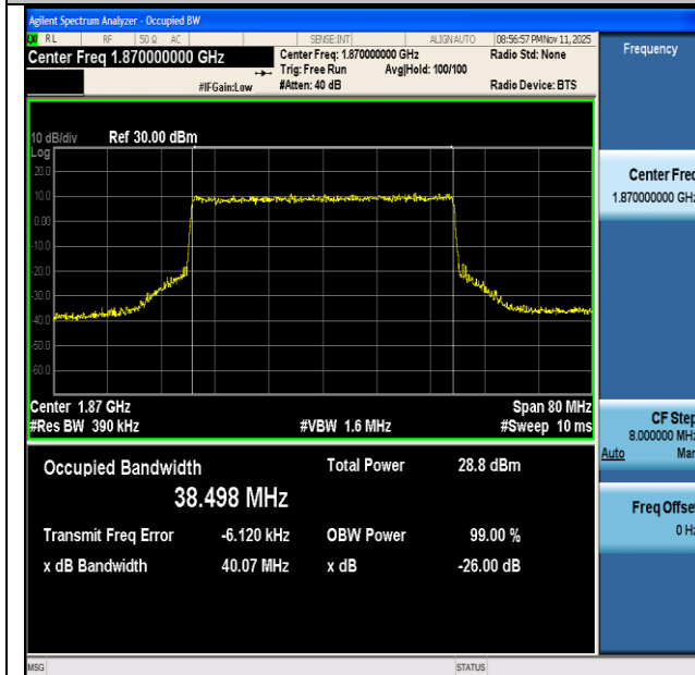
NTNV-n2-PC3-15-40-L-CP-256QAM-Outer_Full-Ant1-PASS
