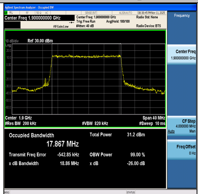
NTNV-n2-PC3-15-20-H-DFT-BPSK-Outer_Full-Ant1-PASS
