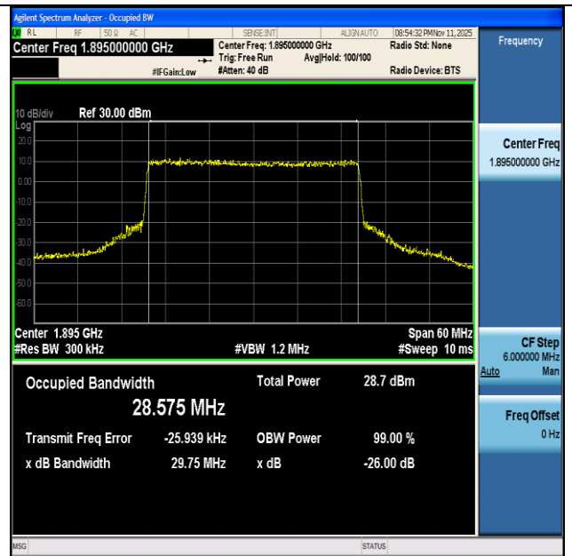
NTNV-n2-PC3-15-30-H-CP-256QAM-Outer_Full-Ant1-PASS
