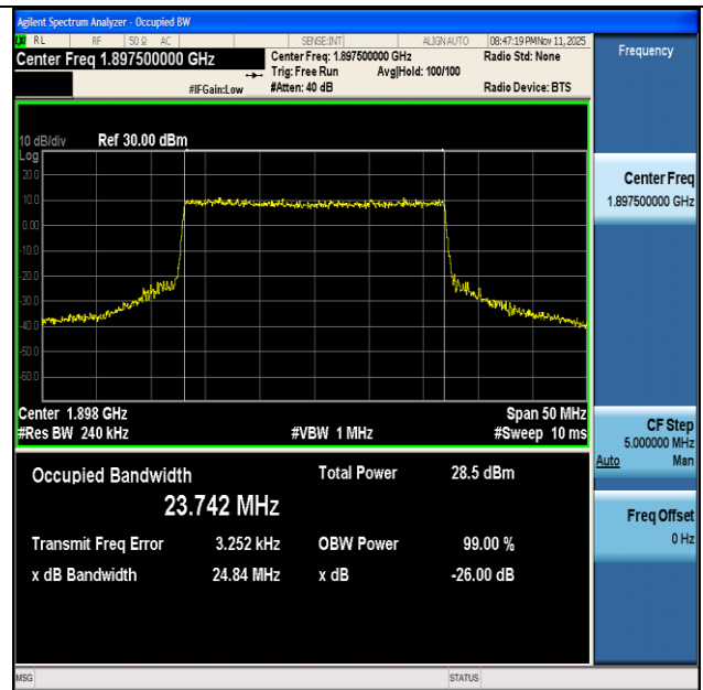
NTNV-n2-PC3-15-25-H-CP-64QAM-Outer_Full-Ant1-PASS
