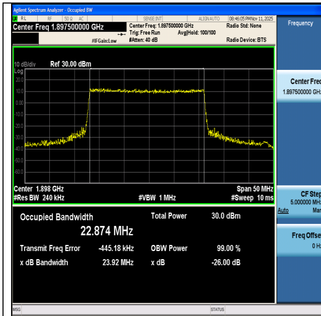
NTNV-n2-PC3-15-25-H-DFT-16QAM-Outer_Full-Ant1-PASS
