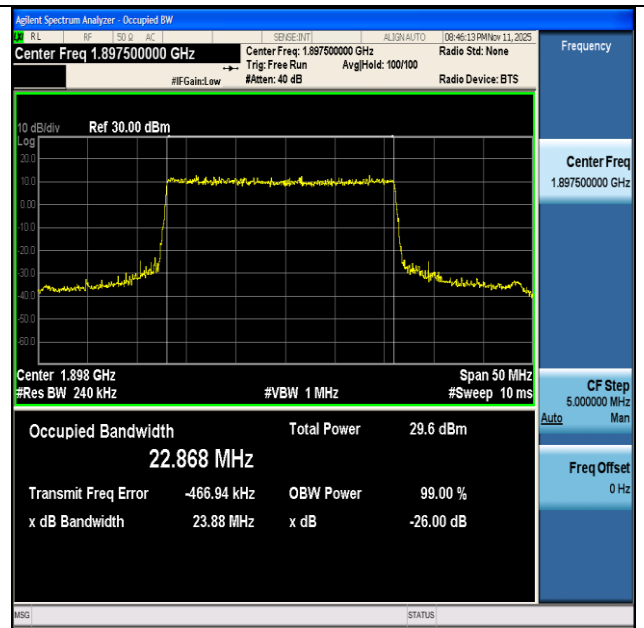
NTNV-n2-PC3-15-25-H-DFT-64QAM-Outer_Full-Ant1-PASS
