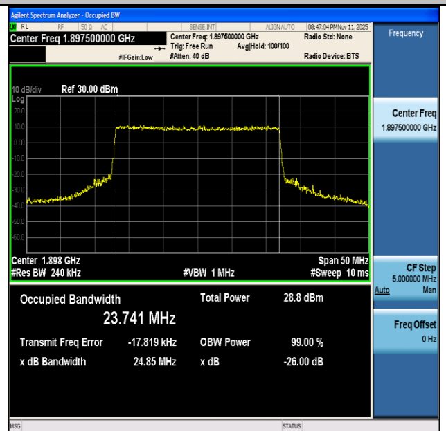
NTNV-n2-PC3-15-25-H-CP-QPSK-Outer_Full-Ant1-PASS
