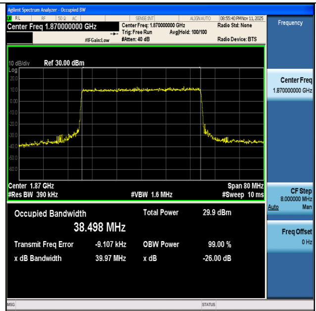
NTNV-n2-PC3-15-40-L-DFT-64QAM-Outer_Full-Ant1-PASS
