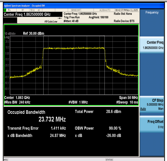
NTNV-n2-PC3-15-25-L-CP-64QAM-Outer_Full-Ant1-PASS
