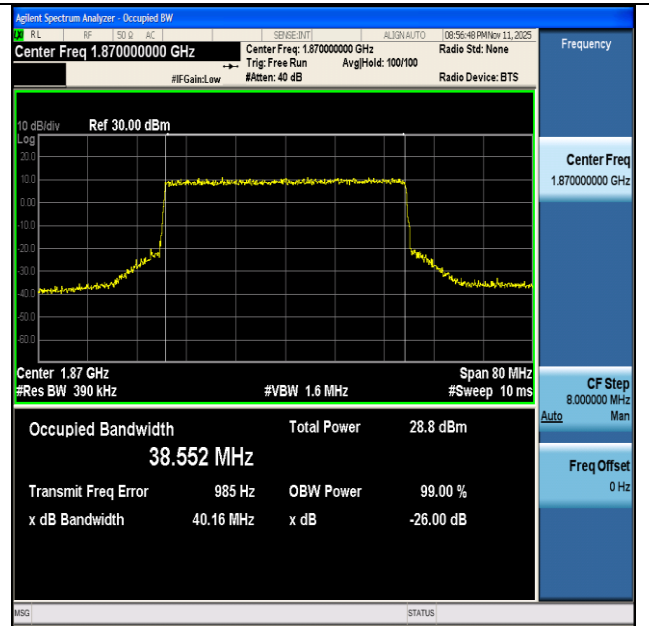
NTNV-n2-PC3-15-40-L-CP-64QAM-Outer_Full-Ant1-PASS
