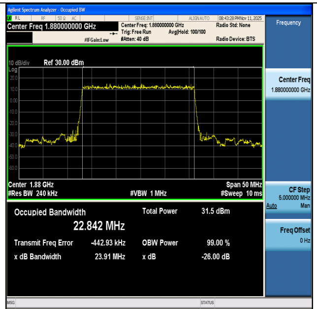
NTNV-n2-PC3-15-25-M-DFT-BPSK-Outer_Full-Ant1-PASS
