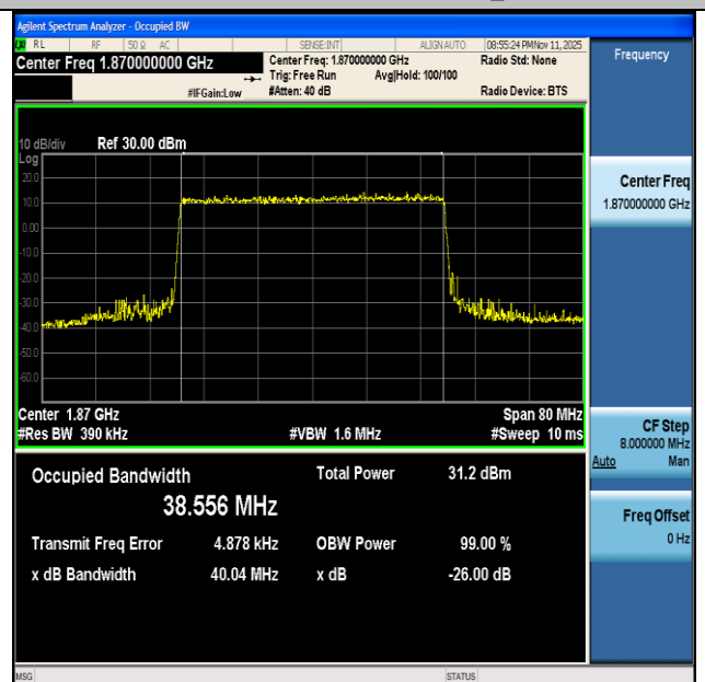
NTNV-n2-PC3-15-40-L-DFT-QPSK-Outer_Full-Ant1-PASS
