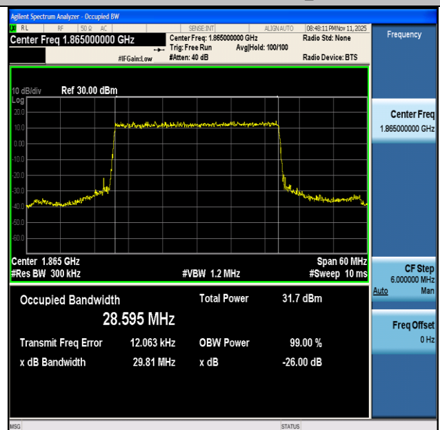
NTNV-n2-PC3-15-30-L-DFT-BPSK-Outer_Full-Ant1-PASS
