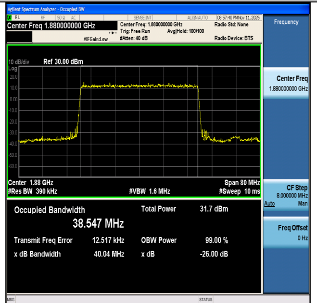
NTNV-n2-PC3-15-40-M-DFT-BPSK-Outer_Full-Ant1-PASS
