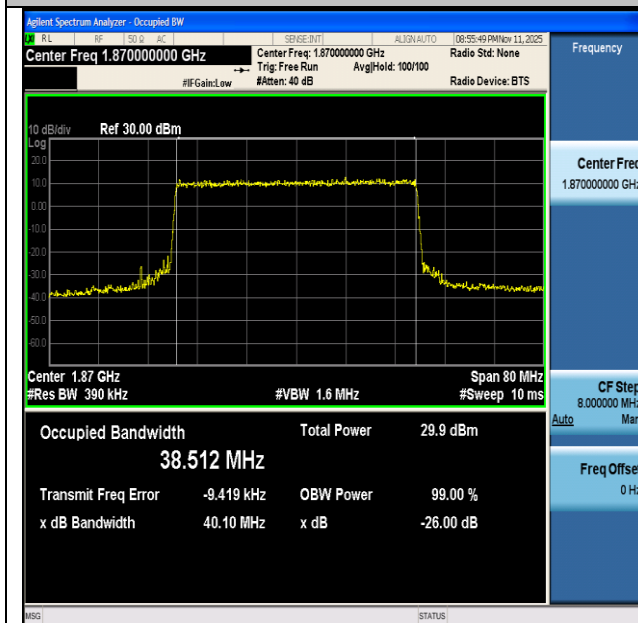
NTNV-n2-PC3-15-40-L-DFT-256QAM-Outer_Full-Ant1-PASS
