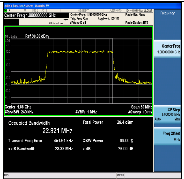
NTNV-n2-PC3-15-25-M-DFT-256QAM-Outer_Full-Ant1-PASS
