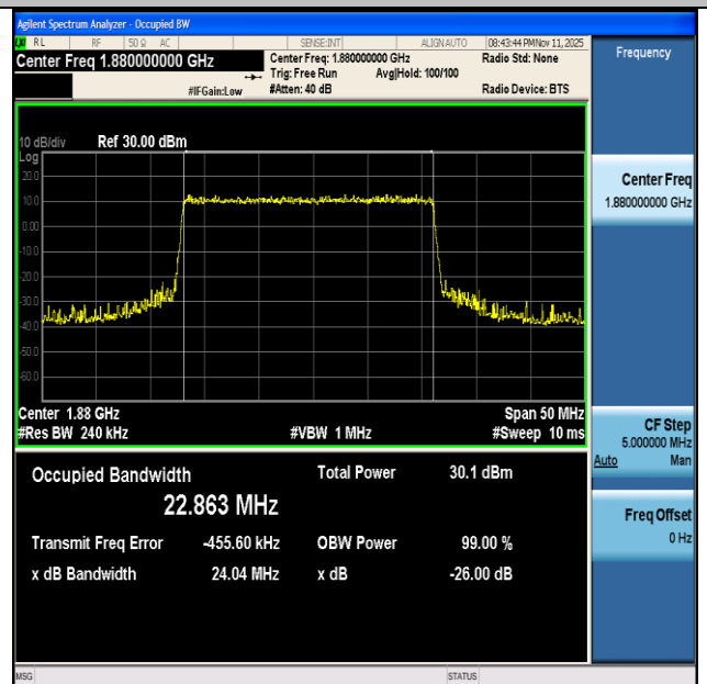
NTNV-n2-PC3-15-25-M-DFT-16QAM-Outer_Full-Ant1-PASS
