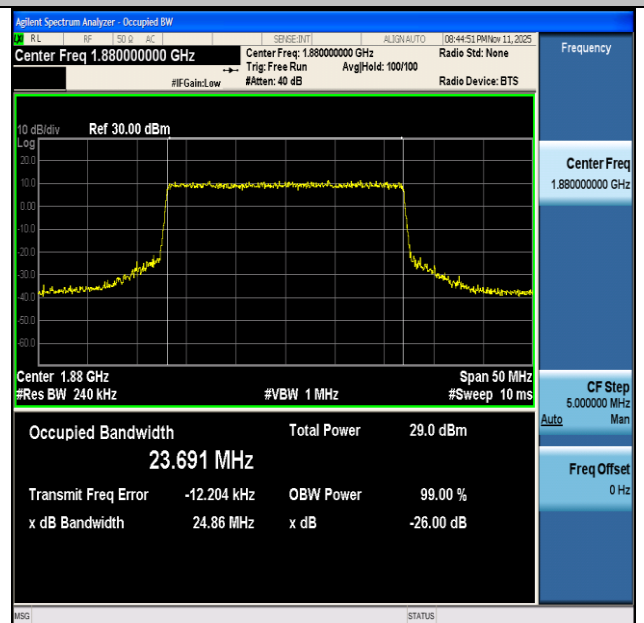
NTNV-n2-PC3-15-25-M-CP-16QAM-Outer_Full-Ant1-PASS
