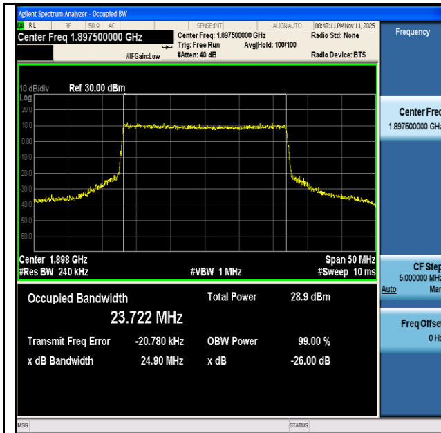
NTNV-n2-PC3-15-25-H-CP-16QAM-Outer_Full-Ant1-PASS
