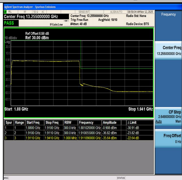
NTNV-n2-PC3-15-30-H-CP-QPSK-Outer_Full-PASS
