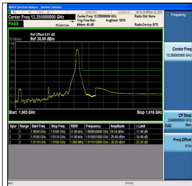
NTNV-n2-PC3-15-5-H-DFT-BPSK-Edge_1RB_Right-PASS
