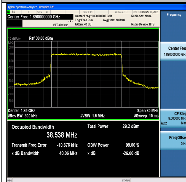
NTNV-n2-PC3-15-40-H-CP-16QAM-Outer_Full-Ant1-PASS
