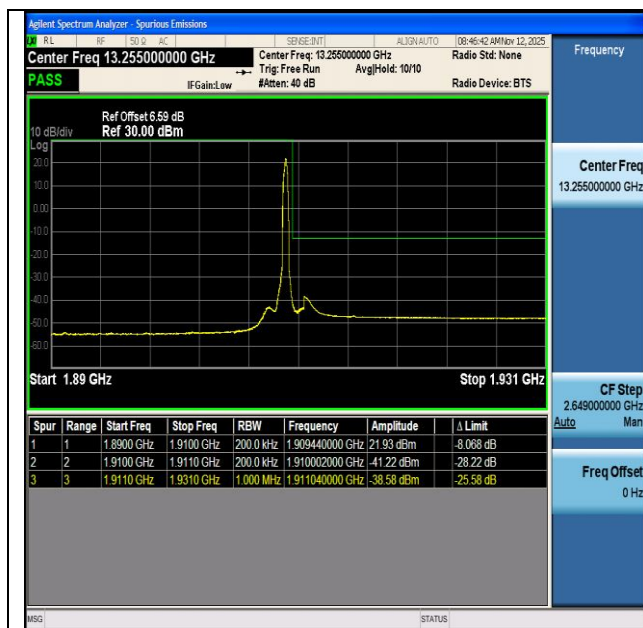
NTNV-n2-PC3-15-20-H-DFT-BPSK-Edge_1RB_Right-PASS
