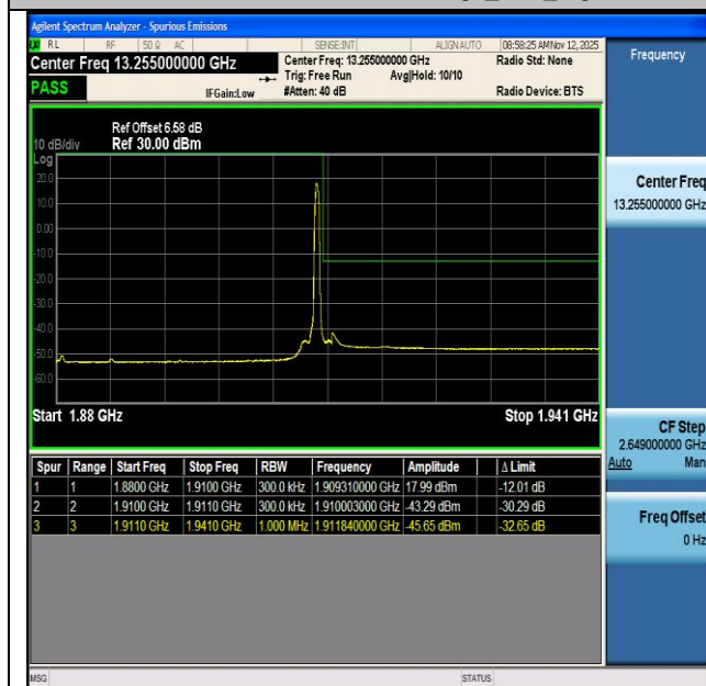
NTNV-n2-PC3-15-30-H-CP-QPSK-Edge_1RB_Right-PASS
