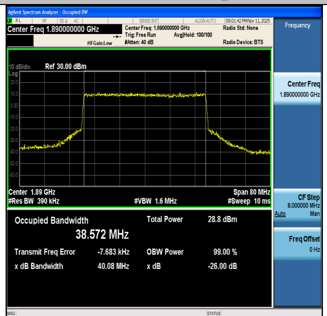
NTNV-n2-PC3-15-40-H-CP-64QAM-Outer_Full-Ant1-PASS
