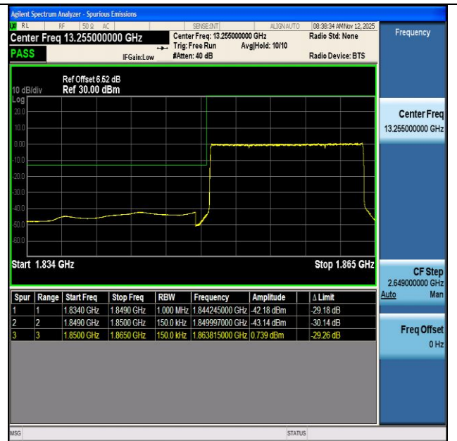
NTNV-n2-PC3-15-15-L-DFT-BPSK-Outer_Full-PASS
