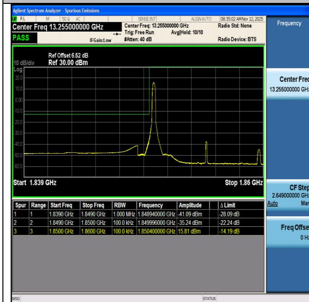
NTNV-n2-PC3-15-10-L-CP-QPSK-Edge_1RB_Left-PASS
