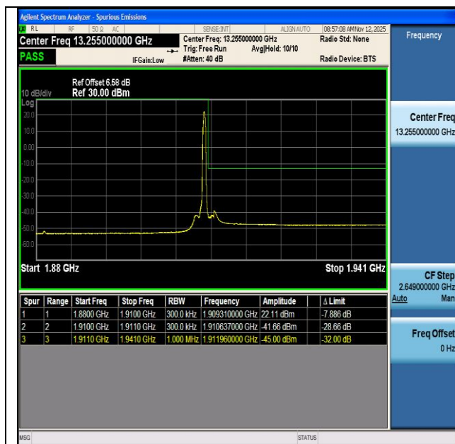
NTNV-n2-PC3-15-30-H-DFT-BPSK-Edge_1RB_Right-PASS
