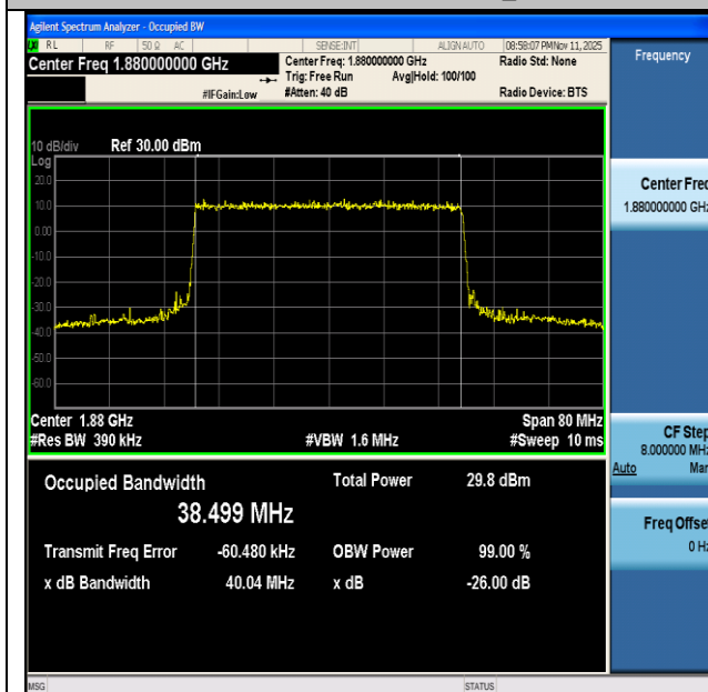
NTNV-n2-PC3-15-40-M-DFT-64QAM-Outer_Full-Ant1-PASS
