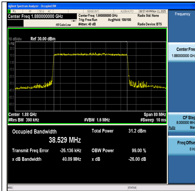
NTNV-n2-PC3-15-40-M-DFT-QPSK-Outer_Full-Ant1-PASS
