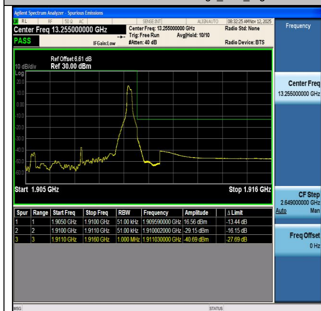
NTNV-n2-PC3-15-5-H-CP-QPSK-Edge_1RB_Right-PASS
