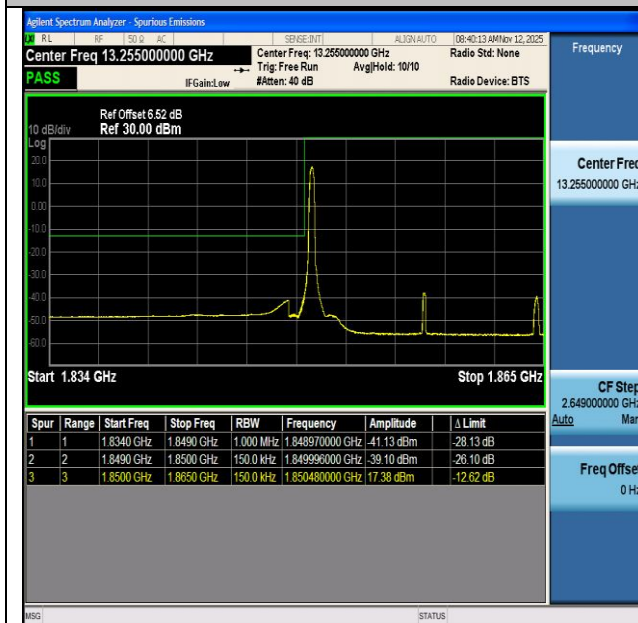
NTNV-n2-PC3-15-15-L-CP-QPSK-Edge_1RB_Left-PASS
