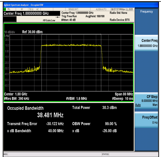
NTNV-n2-PC3-15-40-M-DFT-16QAM-Outer_Full-Ant1-PASS
