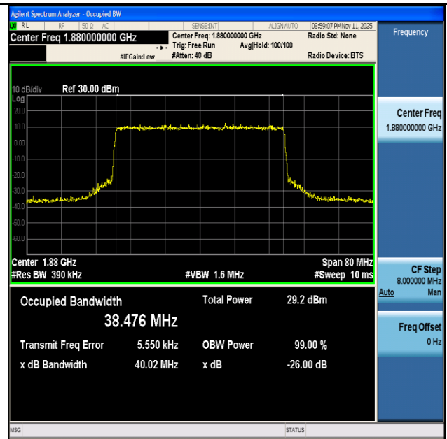
NTNV-n2-PC3-15-40-M-CP-16QAM-Outer_Full-Ant1-PASS
