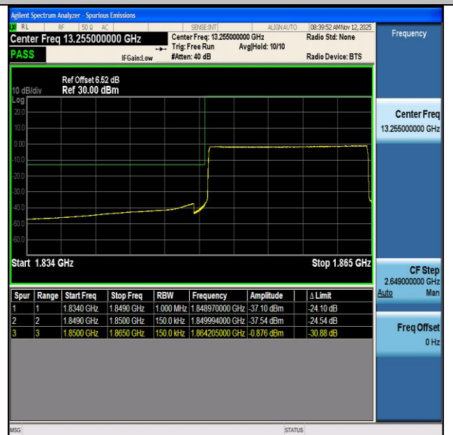
NTNV-n2-PC3-15-15-L-CP-QPSK-Outer_Full-PASS
