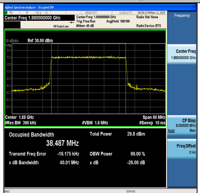
NTNV-n2-PC3-15-40-M-DFT-256QAM-Outer_Full-Ant1-PASS
