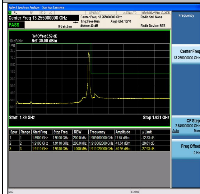
NTNV-n2-PC3-15-20-H-CP-QPSK-Edge_1RB_Right-PASS
