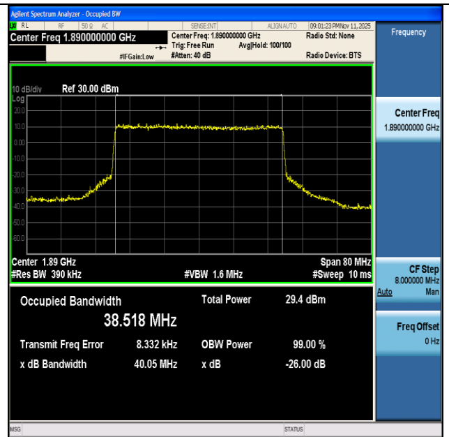
NTNV-n2-PC3-15-40-H-CP-QPSK-Outer_Full-Ant1-PASS
