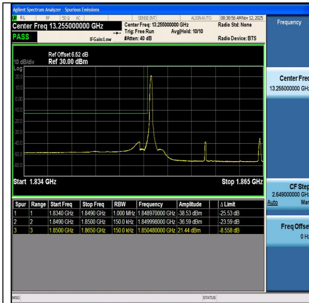
NTNV-n2-PC3-15-15-L-DFT-BPSK-Edge_1RB_Left-PASS
