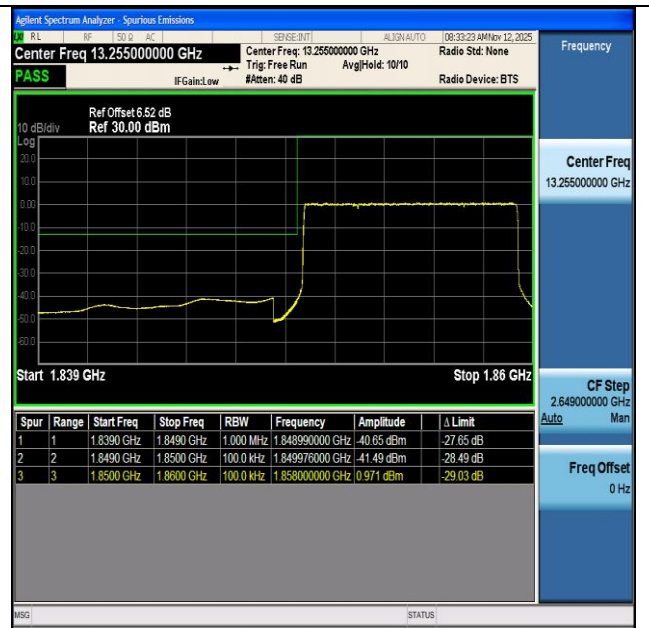
NTNV-n2-PC3-15-10-L-DFT-BPSK-Outer_Full-PASS
