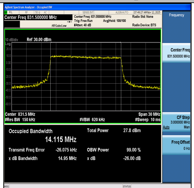
NTNV-n5-PC3-15-15-L-CP-QPSK-Outer_Full-Ant1-PASS
