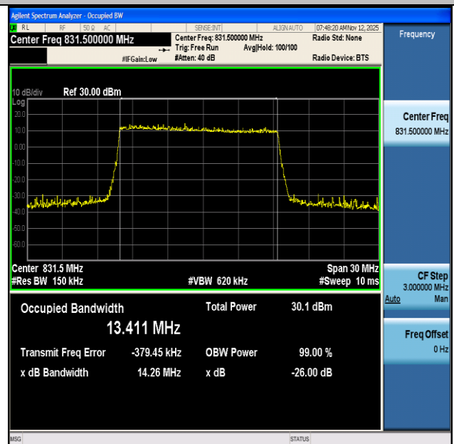
NTNV-n5-PC3-15-15-L-DFT-QPSK-Outer_Full-Ant1-PASS
