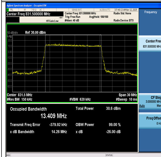
NTNV-n5-PC3-15-15-L-DFT-BPSK-Outer_Full-Ant1-PASS
