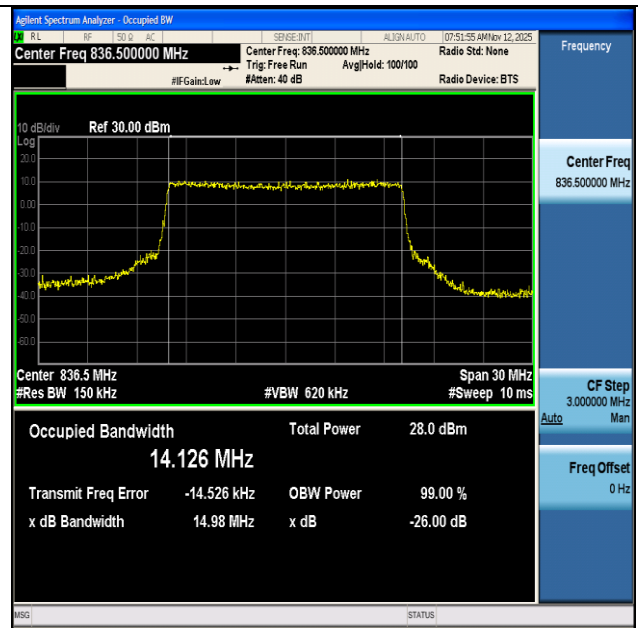
NTNV-n5-PC3-15-15-M-CP-16QAM-Outer_Full-Ant1-PASS
