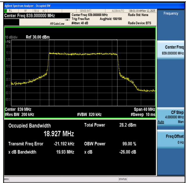
NTNV-n5-PC3-15-20-H-CP-16QAM-Outer_Full-Ant1-PASS
