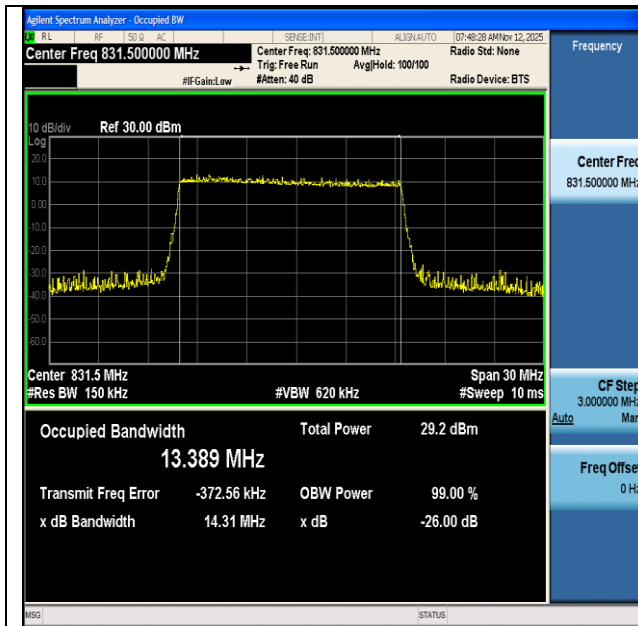
NTNV-n5-PC3-15-15-L-DFT-16QAM-Outer_Full-Ant1-PASS
