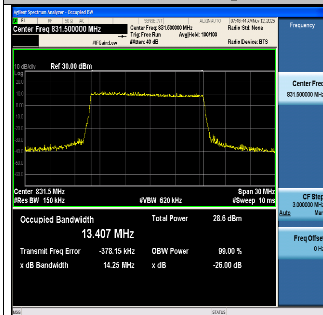
NTNV-n5-PC3-15-15-L-DFT-256QAM-Outer_Full-Ant1-PASS
