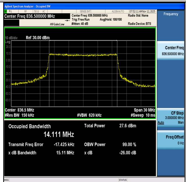
NTNV-n5-PC3-15-15-M-CP-256QAM-Outer_Full-Ant1-PASS
