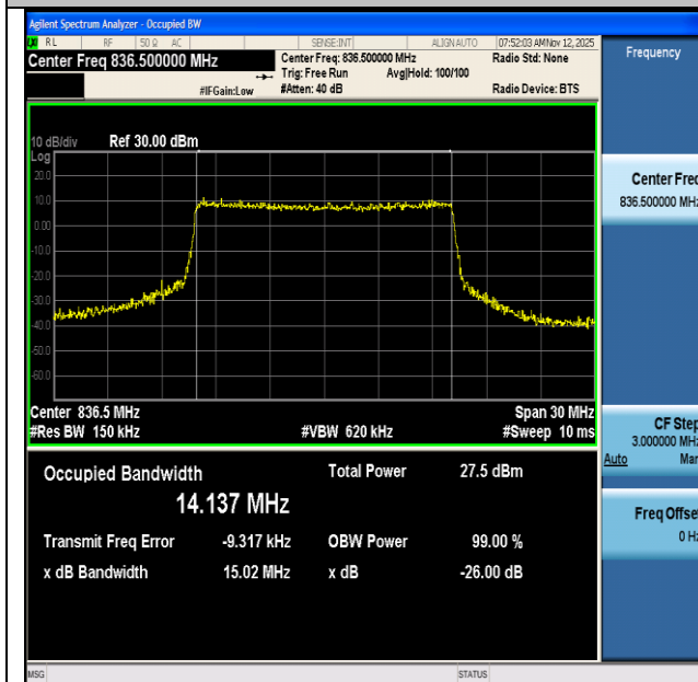
NTNV-n5-PC3-15-15-M-CP-64QAM-Outer_Full-Ant1-PASS
