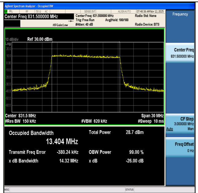
NTNV-n5-PC3-15-15-L-DFT-64QAM-Outer_Full-Ant1-PASS
