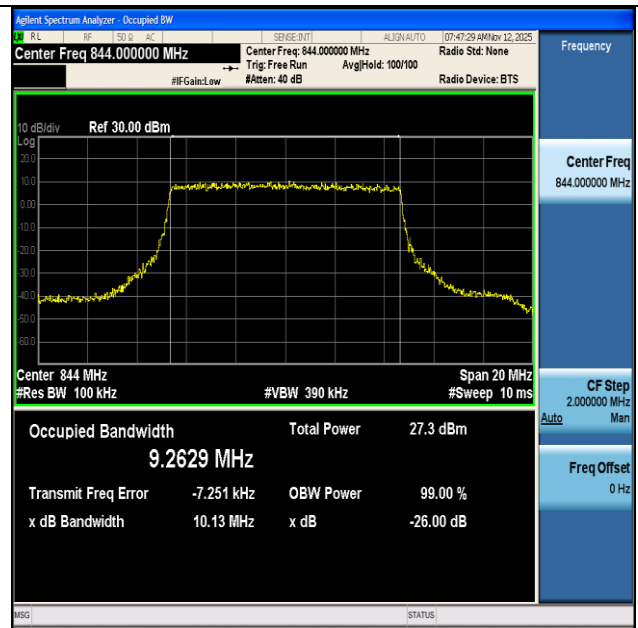
NTNV-n5-PC3-15-10-H-CP-256QAM-Outer_Full-Ant1-PASS
