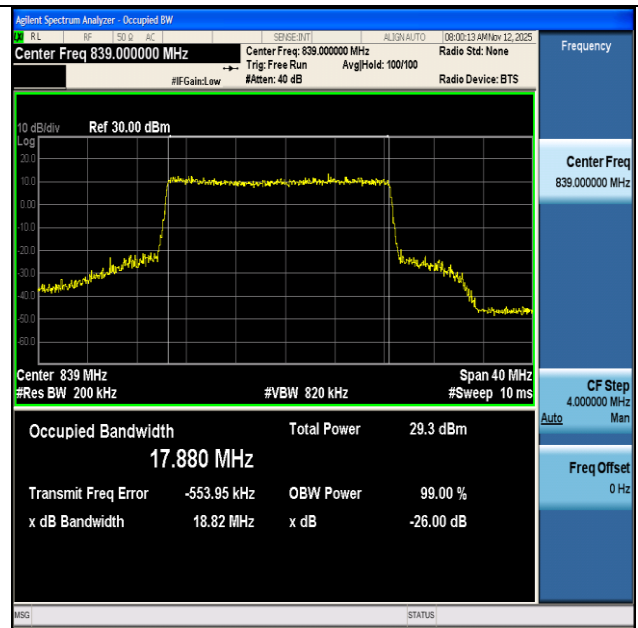
NTNV-n5-PC3-15-20-H-DFT-16QAM-Outer_Full-Ant1-PASS
