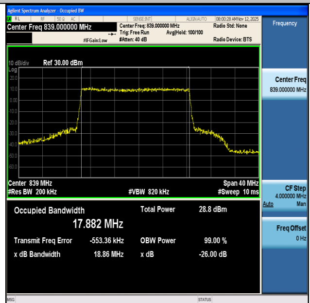
NTNV-n5-PC3-15-20-H-DFT-256QAM-Outer_Full-Ant1-PASS
