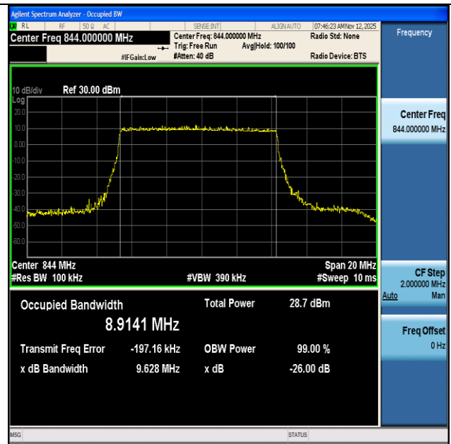
NTNV-n5-PC3-15-10-H-DFT-256QAM-Outer_Full-Ant1-PASS
