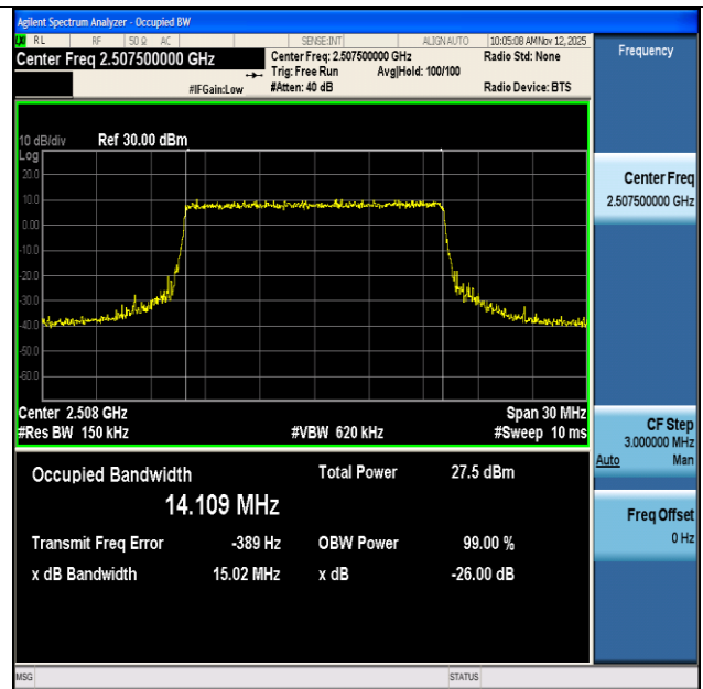
NTNV-n7-PC3-15-15-L-CP-64QAM-Outer_Full-Ant1-PASS
