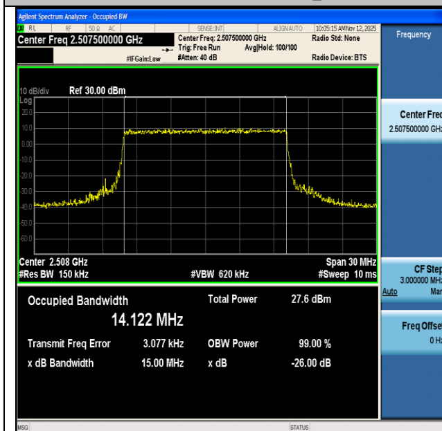
NTNV-n7-PC3-15-15-L-CP-256QAM-Outer_Full-Ant1-PASS
