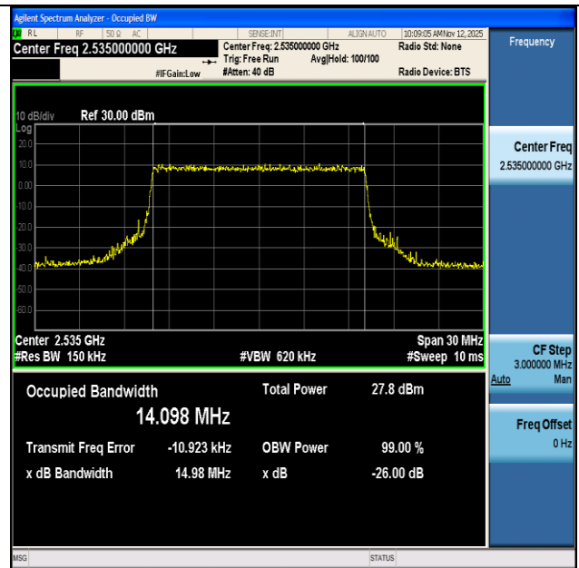
NTNV-n7-PC3-15-15-M-CP-16QAM-Outer_Full-Ant1-PASS
