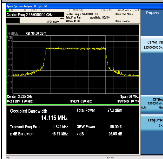
NTNV-n7-PC3-15-15-M-CP-64QAM-Outer_Full-Ant1-PASS
