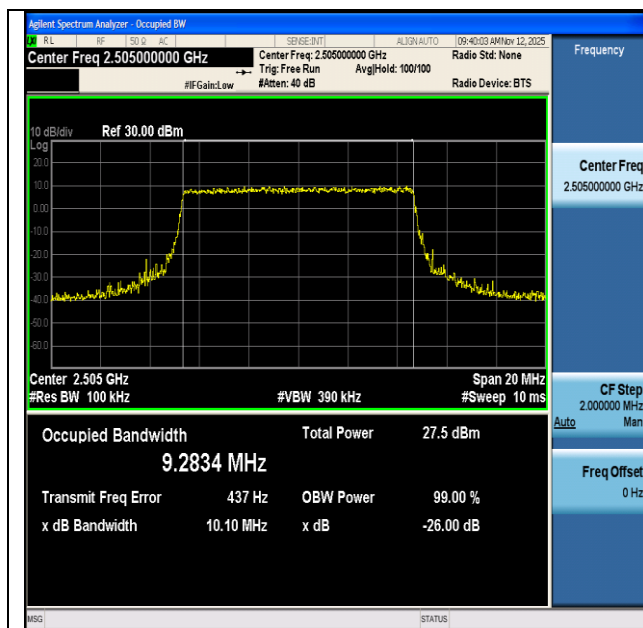
NTNV-n7-PC3-15-10-L-CP-QPSK-Outer_Full-Ant1-PASS
