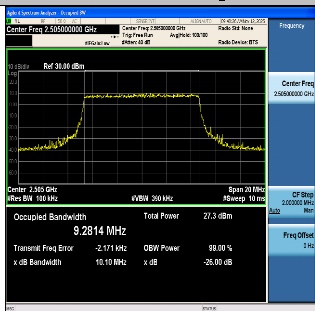
NTNV-n7-PC3-15-10-L-CP-256QAM-Outer_Full-Ant1-PASS
