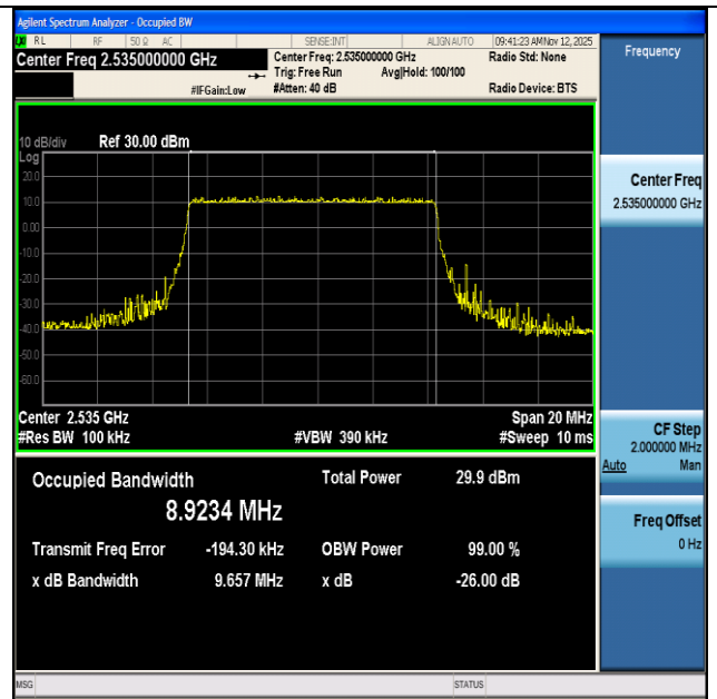
NTNV-n7-PC3-15-10-M-DFT-QPSK-Outer_Full-Ant1-PASS
