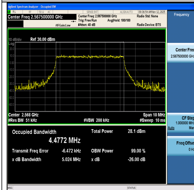
NTNV-n7-PC3-15-5-H-DFT-256QAM-Outer_Full-Ant1-PASS
