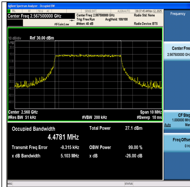
NTNV-n7-PC3-15-5-H-CP-16QAM-Outer_Full-Ant1-PASS
