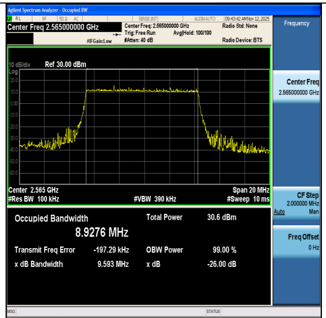
NTNV-n7-PC3-15-10-H-DFT-BPSK-Outer_Full-Ant1-PASS
