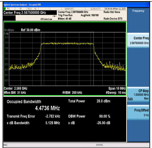
NTNV-n7-PC3-15-5-H-DFT-64QAM-Outer_Full-Ant1-PASS
