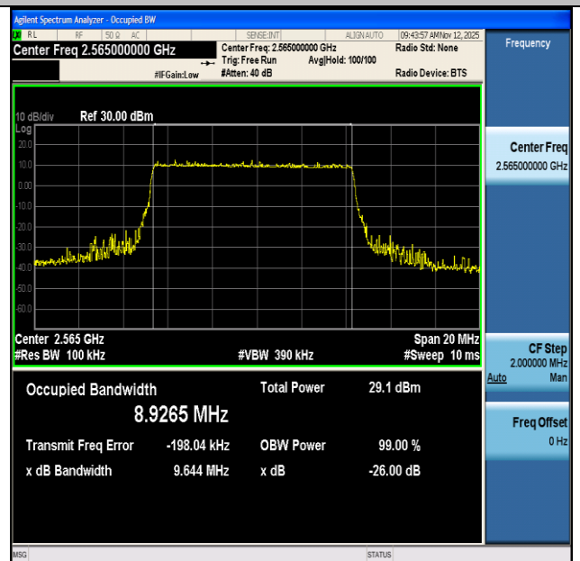
NTNV-n7-PC3-15-10-H-DFT-16QAM-Outer_Full-Ant1-PASS
