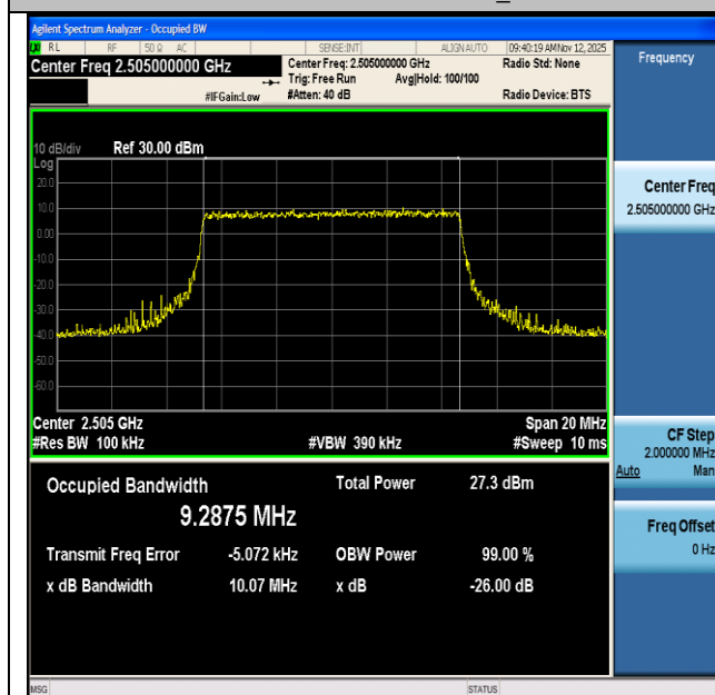
NTNV-n7-PC3-15-10-L-CP-64QAM-Outer_Full-Ant1-PASS
