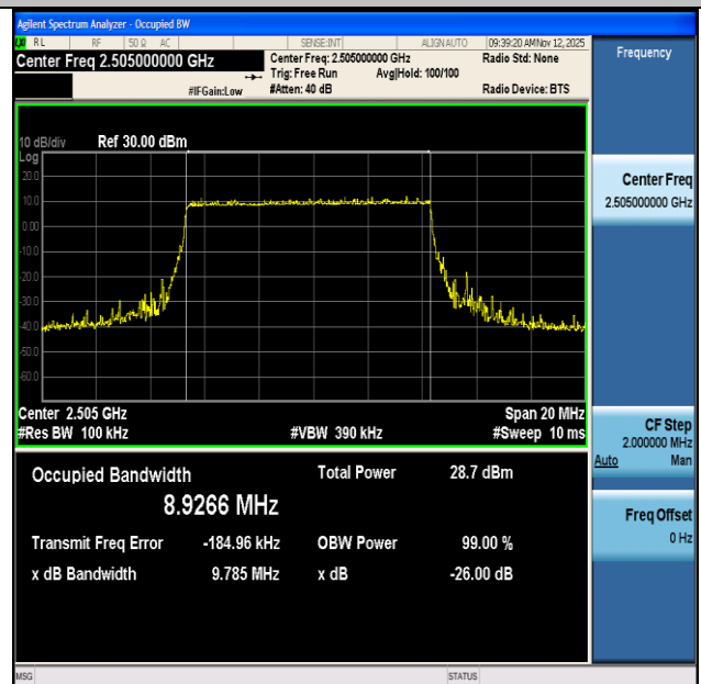
NTNV-n7-PC3-15-10-L-DFT-256QAM-Outer_Full-Ant1-PASS
