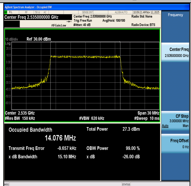
NTNV-n7-PC3-15-15-M-CP-256QAM-Outer_Full-Ant1-PASS
