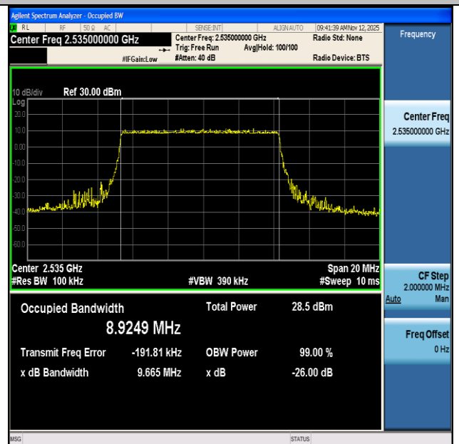
NTNV-n7-PC3-15-10-M-DFT-64QAM-Outer_Full-Ant1-PASS
