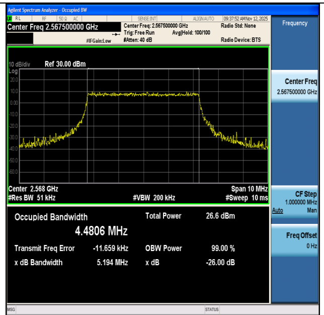
NTNV-n7-PC3-15-5-H-CP-64QAM-Outer_Full-Ant1-PASS
