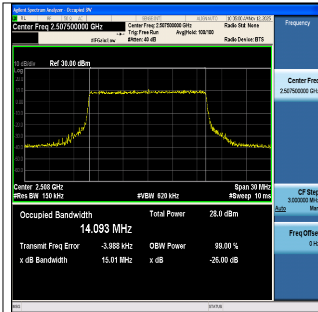
NTNV-n7-PC3-15-15-L-CP-16QAM-Outer_Full-Ant1-PASS
