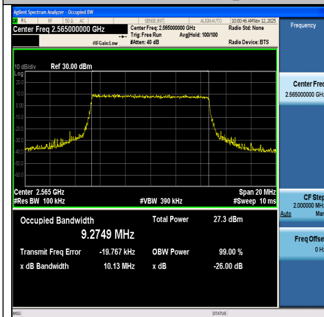
NTNV-n7-PC3-15-10-H-CP-QPSK-Outer_Full-Ant1-PASS
