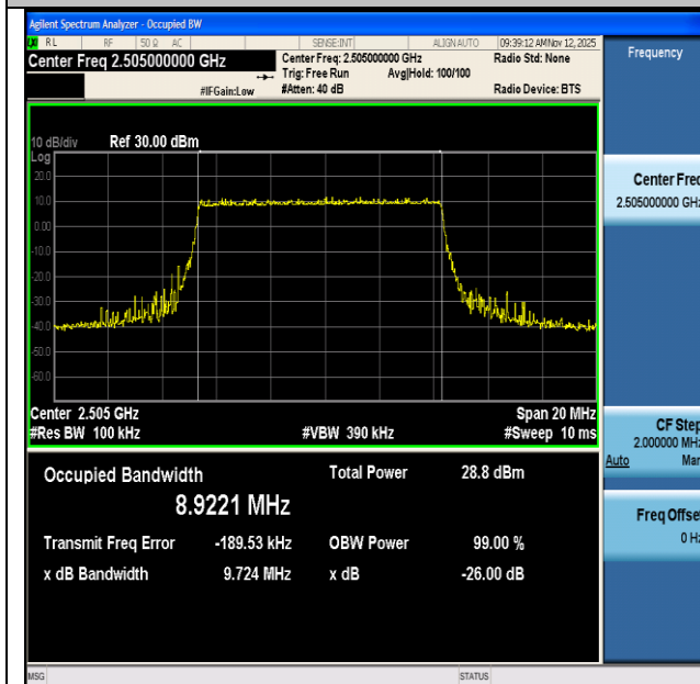
NTNV-n7-PC3-15-10-L-DFT-64QAM-Outer_Full-Ant1-PASS
