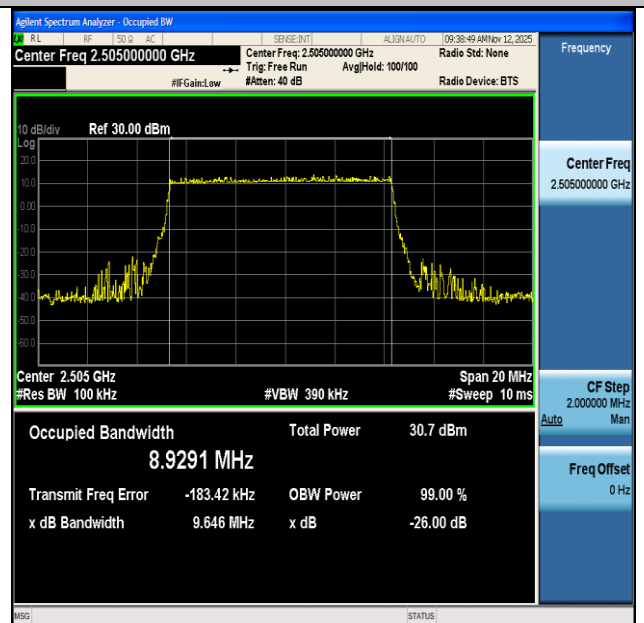
NTNV-n7-PC3-15-10-L-DFT-BPSK-Outer_Full-Ant1-PASS
