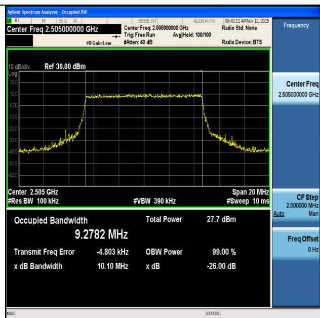
NTNV-n7-PC3-15-10-L-CP-16QAM-Outer_Full-Ant1-PASS
