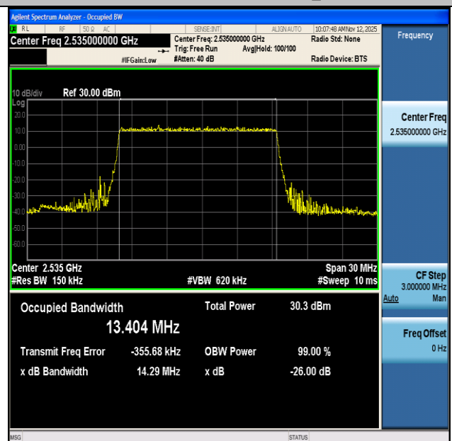
NTNV-n7-PC3-15-15-M-DFT-BPSK-Outer_Full-Ant1-PASS
