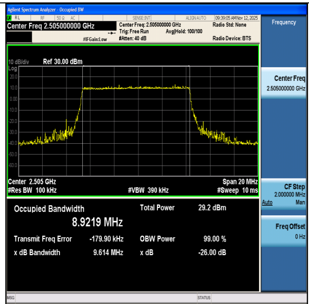
NTNV-n7-PC3-15-10-L-DFT-16QAM-Outer_Full-Ant1-PASS
