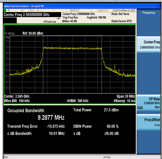
NTNV-n7-PC3-15-10-H-CP-16QAM-Outer_Full-Ant1-PASS
