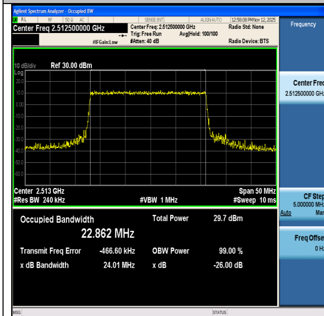
NTNV-n7-PC3-15-25-L-DFT-16QAM-Outter_Full-Ant1-PASS
