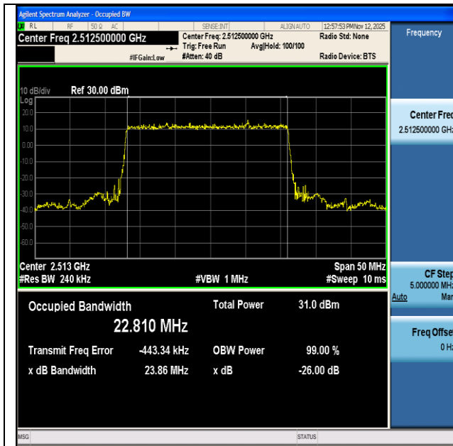
NTNV-n7-PC3-15-25-L-DFT-BPSK-Outter_Full-Ant1-PASS
