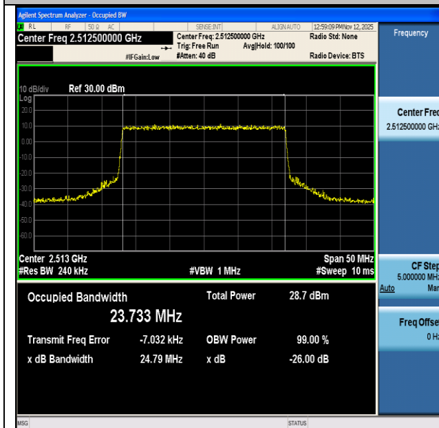
NTNV-n7-PC3-15-25-L-CP-16QAM-Outer_Full-Ant1-PASS
