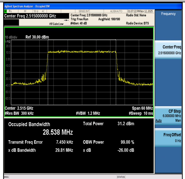
NTNV-n7-PC3-15-30-L-DFT-BPSK-Outer_Full-Ant1-PASS
