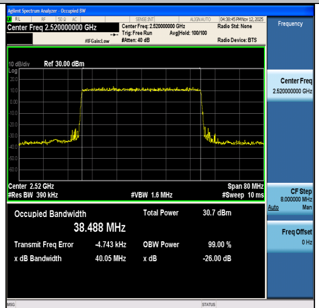
NTNV-n7-PC3-15-40-L-DFT-QPSK-Outer_Full-Ant1-PASS
