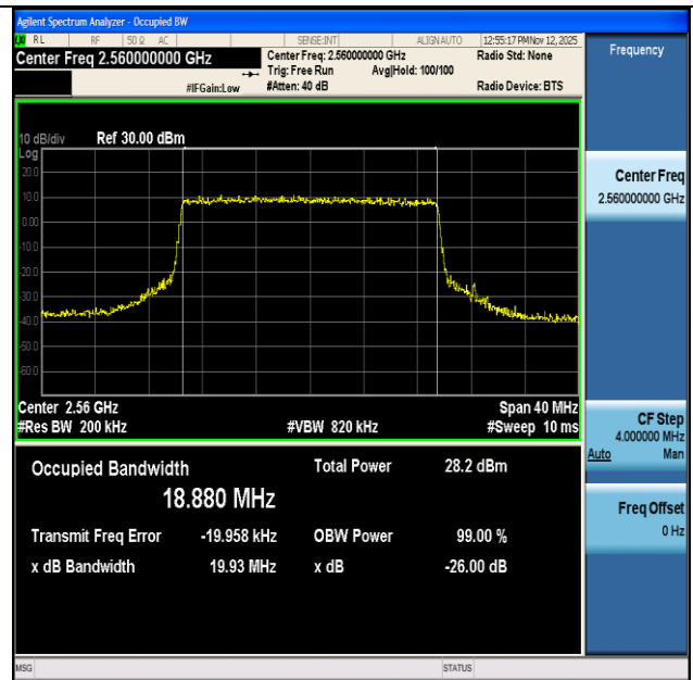
NTNV-n7-PC3-15-20-H-CP-16QAM-Outer_Full-Ant1-PASS
