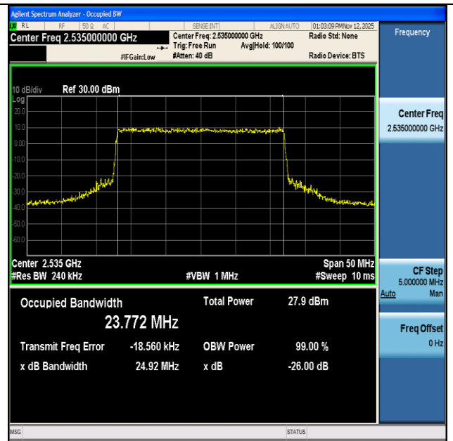
NTNV-n7-PC3-15-25-M-CP-256QAM-Outer_Full-Ant1-PASS
