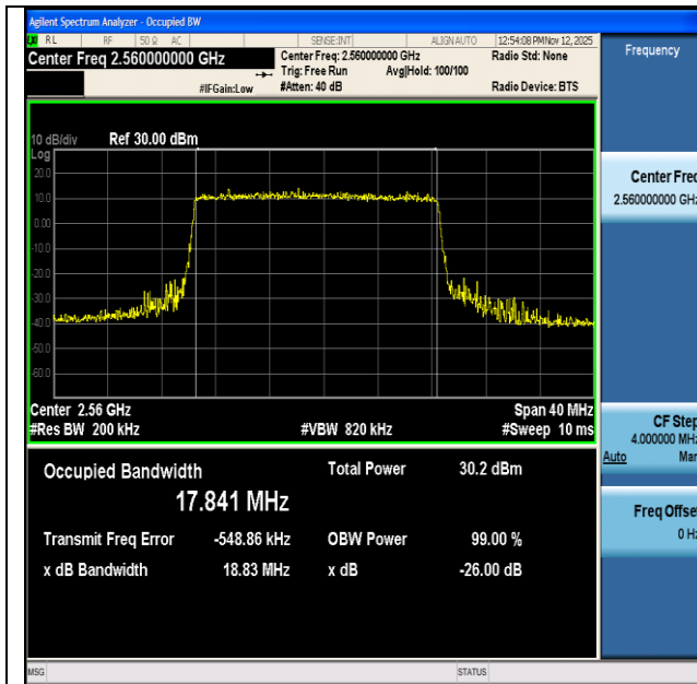
NTNV-n7-PC3-15-20-H-DFT-QPSK-Outer_Full-Ant1-PASS
