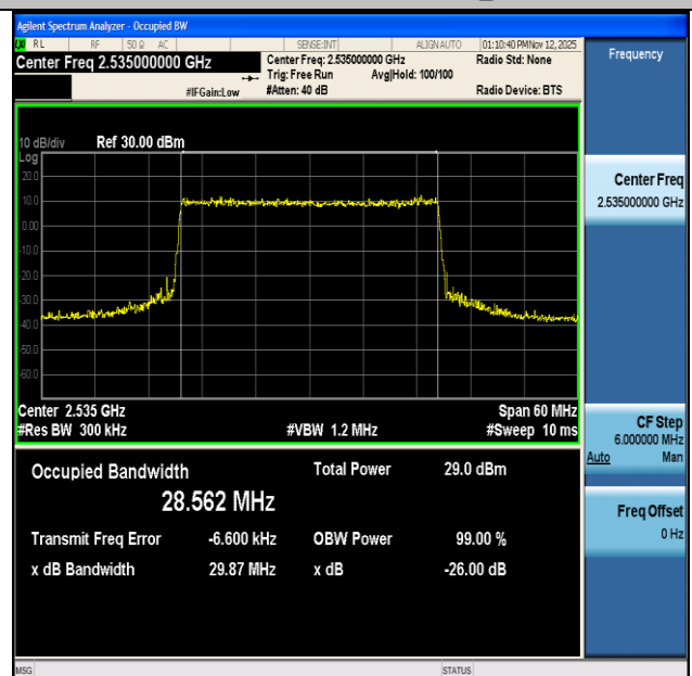
NTNV-n7-PC3-15-30-M-DFT-64QAM-Outer_Full-Ant1-PASS
