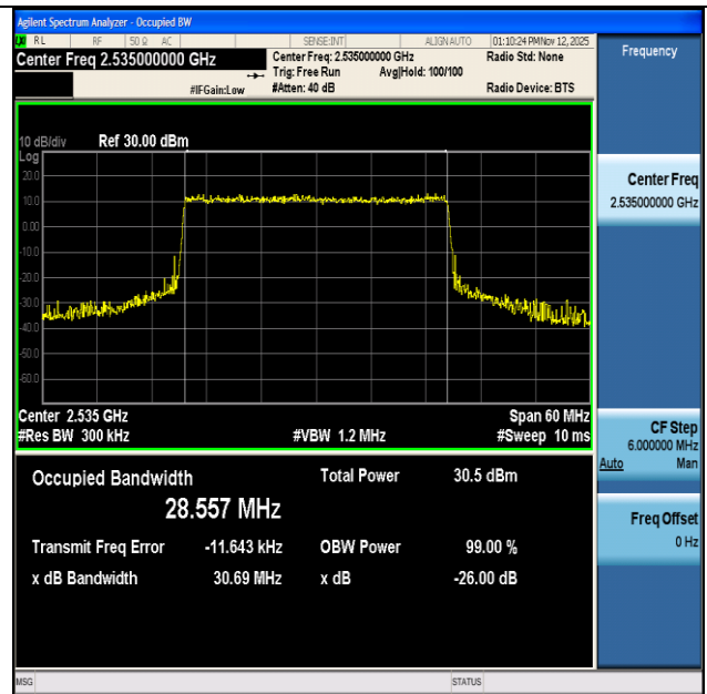
NTNV-n7-PC3-15-30-M-DFT-QPSK-Outer_Full-Ant1-PASS
