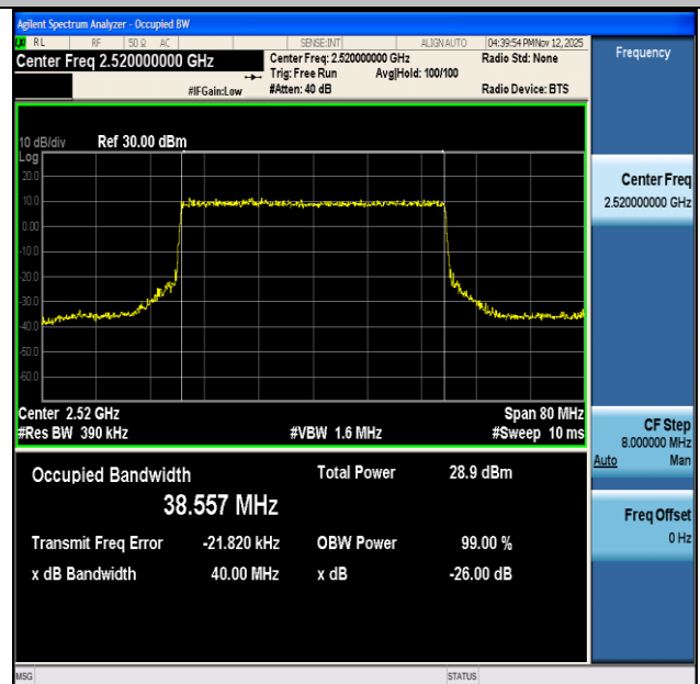
NTNV-n7-PC3-15-40-L-CP-QPSK-Outer_Full-Ant1-PASS
