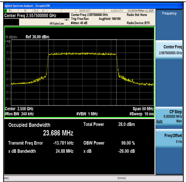
NTNV-n7-PC3-15-25-H-CP-64QAM-Outer_Full-Ant1-PASS
