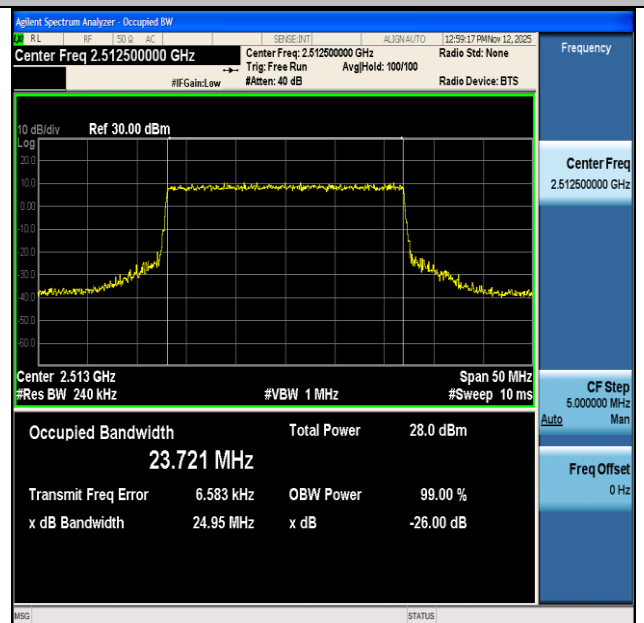
NTNV-n7-PC3-15-25-L-CP-64QAM-Outer_Full-Ant1-PASS
