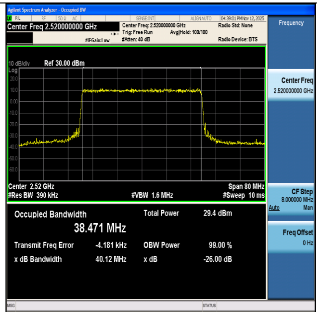
NTNV-n7-PC3-15-40-L-DFT-64QAM-Outer_Full-Ant1-PASS
