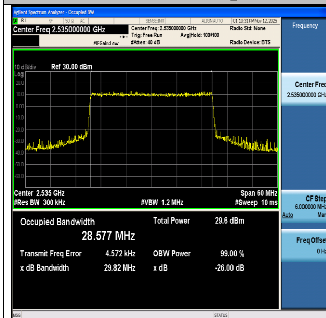
NTNV-n7-PC3-15-30-M-DFT-16QAM-Outer_Full-Ant1-PASS
