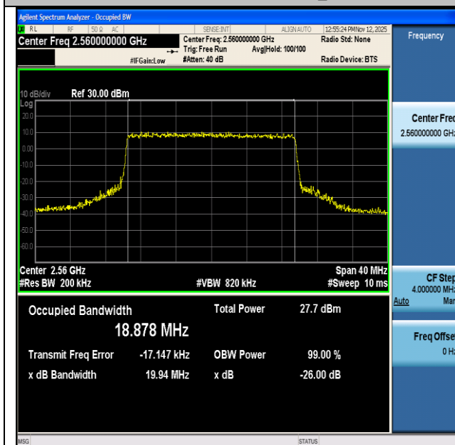
NTNV-n7-PC3-15-20-H-CP-64QAM-Outer_Full-Ant1-PASS
