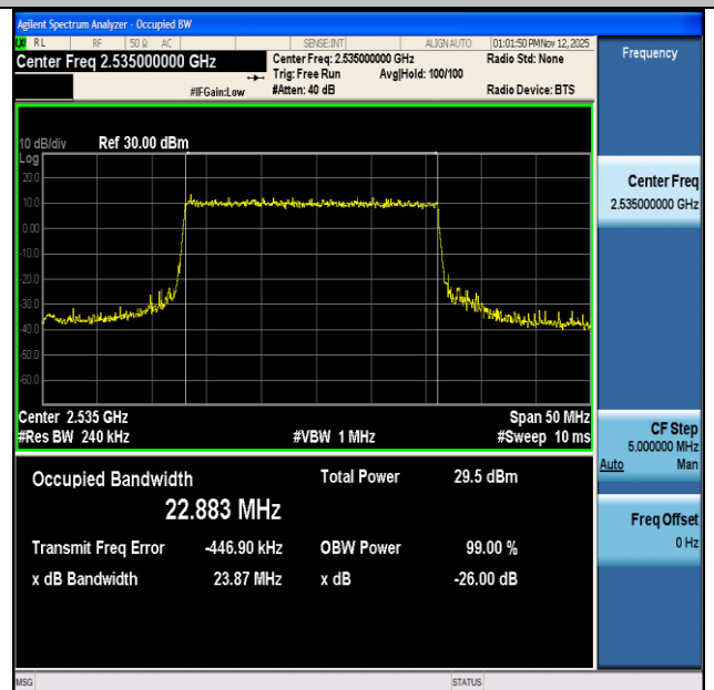
NTNV-n7-PC3-15-25-M-DFT-16QAM-Outer_Full-Ant1-PASS
