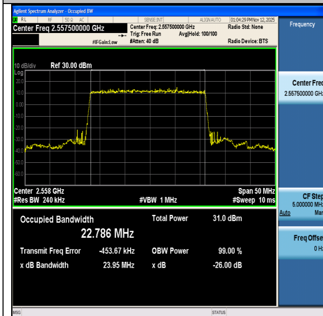
NTNV-n7-PC3-15-25-H-DFT-BPSK-Outer_Full-Ant1-PASS
