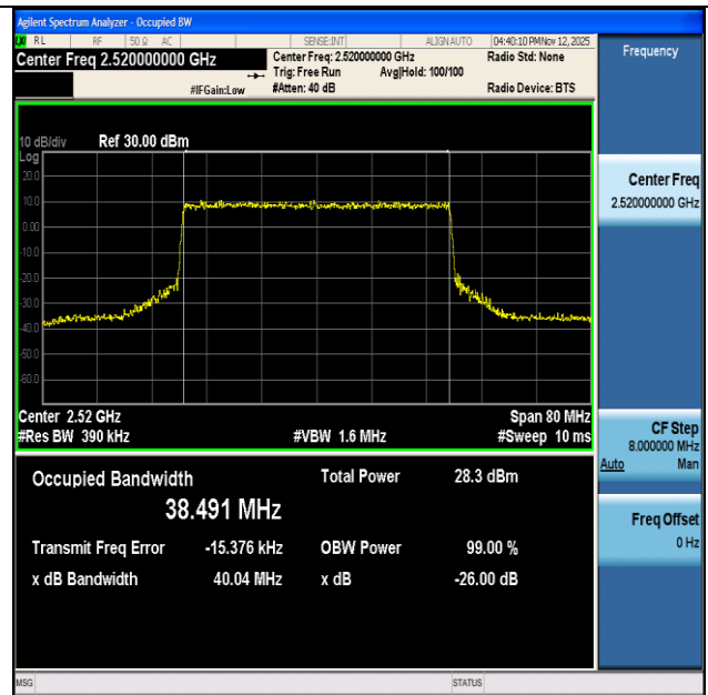
NTNV-n7-PC3-15-40-L-CP-64QAM-Outer_Full-Ant1-PASS
