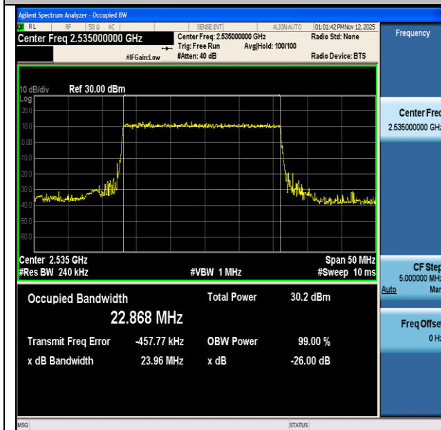
NTNV-n7-PC3-15-25-M-DFT-QPSK-Outer_Full-Ant1-PASS
