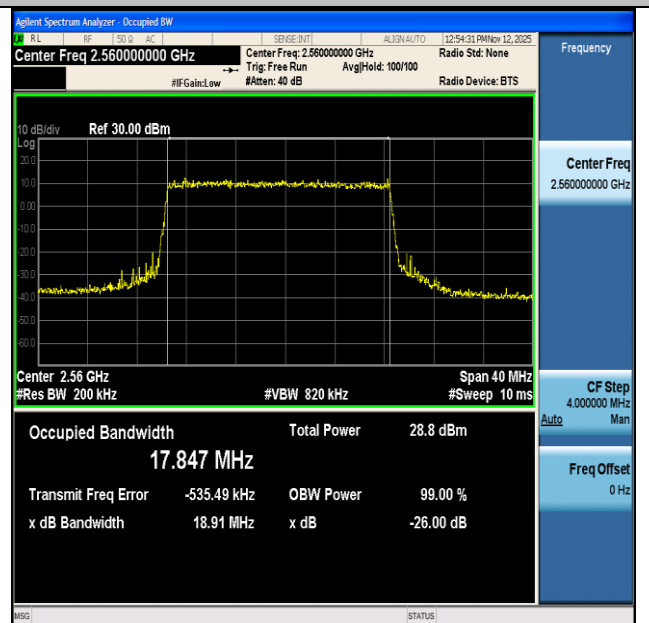
NTNV-n7-PC3-15-20-H-DFT-256QAM-Outer_Full-Ant1-PASS
