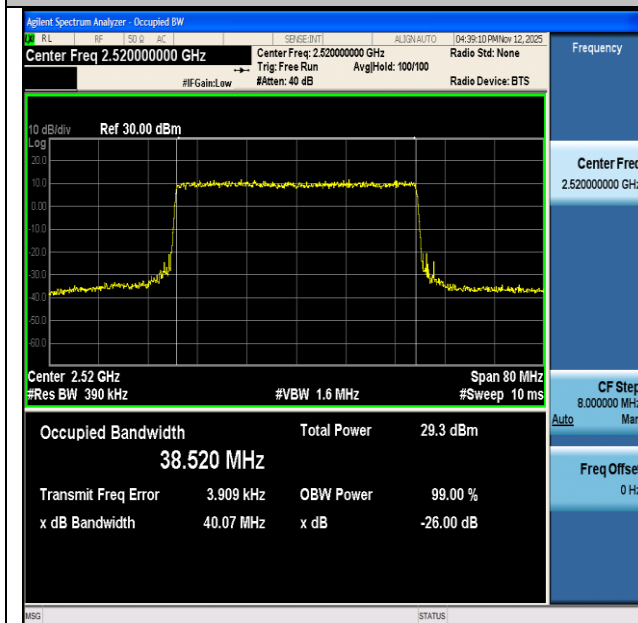
NTNV-n7-PC3-15-40-L-DFT-256QAM-Outer_Full-Ant1-PASS
