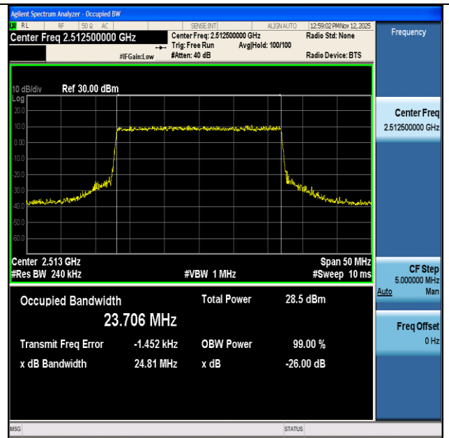
NTNV-n7-PC3-15-25-L-CP-QPSK-Outer_Full-Ant1-PASS
