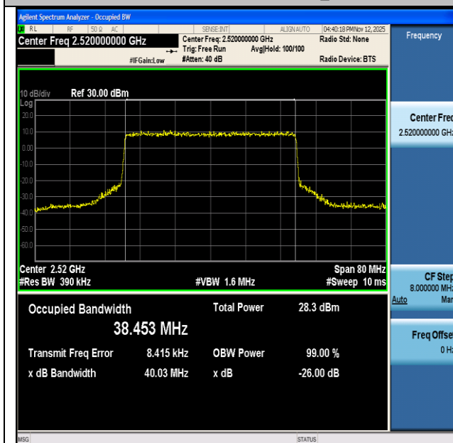
NTNV-n7-PC3-15-40-L-CP-256QAM-Outer_Full-Ant1-PASS
