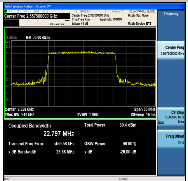
NTNV-n7-PC3-15-25-H-DFT-QPSK-Outer_Full-Ant1-PASS
