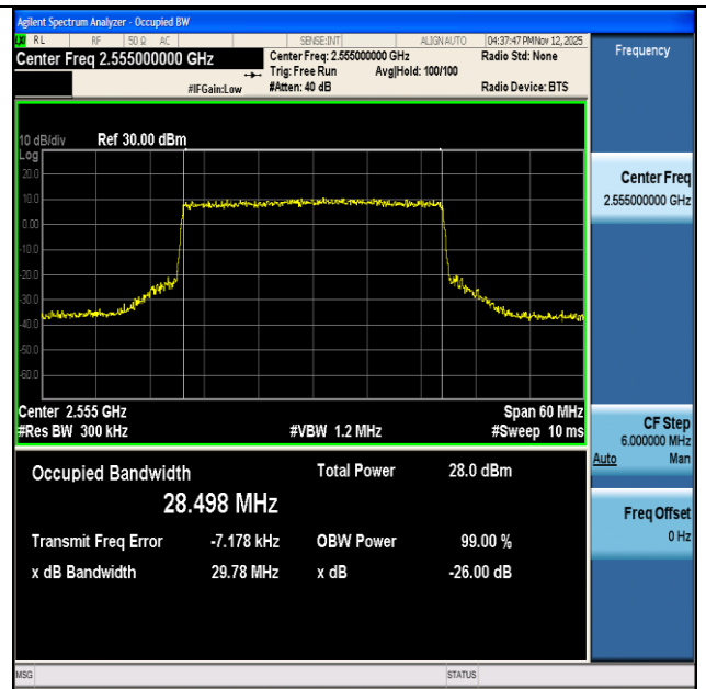
NTNV-n7-PC3-15-30-H-CP-256QAM-Outer_Full-Ant1-PASS
