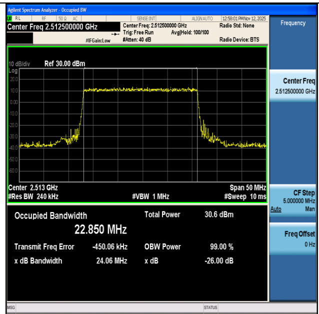
NTNV-n7-PC3-15-25-L-DFT-QPSK-Outter_Full-Ant1-PASS
