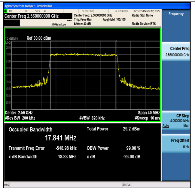
NTNV-n7-PC3-15-20-H-DFT-16QAM-Outer_Full-Ant1-PASS
