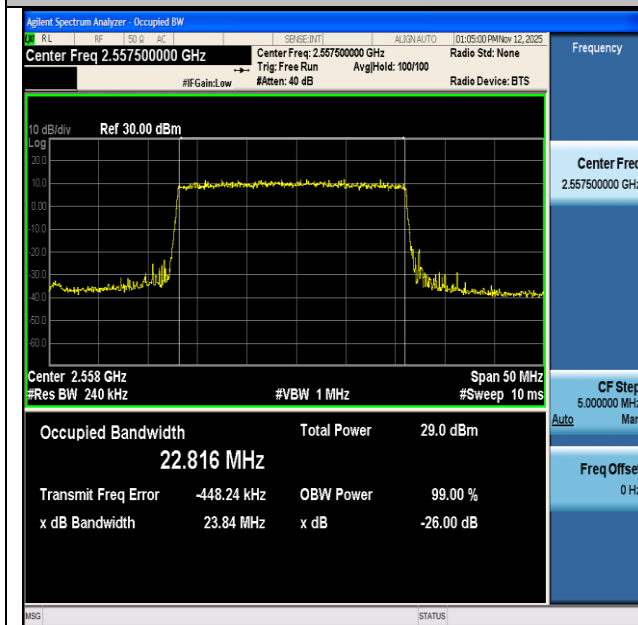
NTNV-n7-PC3-15-25-H-DFT-256QAM-Outer_Full-Ant1-PASS
