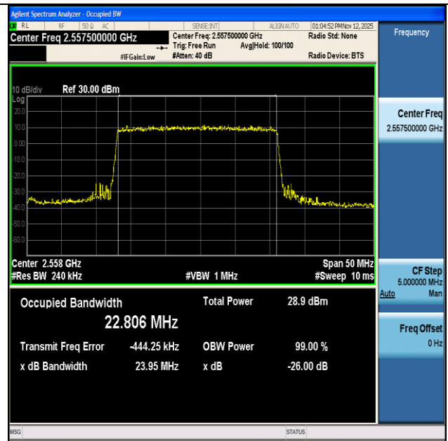
NTNV-n7-PC3-15-25-H-DFT-64QAM-Outer_Full-Ant1-PASS
