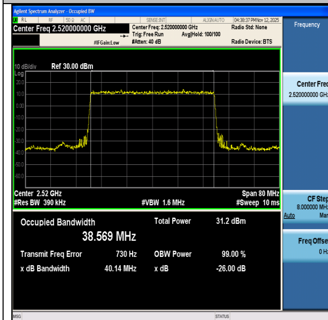
NTNV-n7-PC3-15-40-L-DFT-BPSK-Outer_Full-Ant1-PASS
