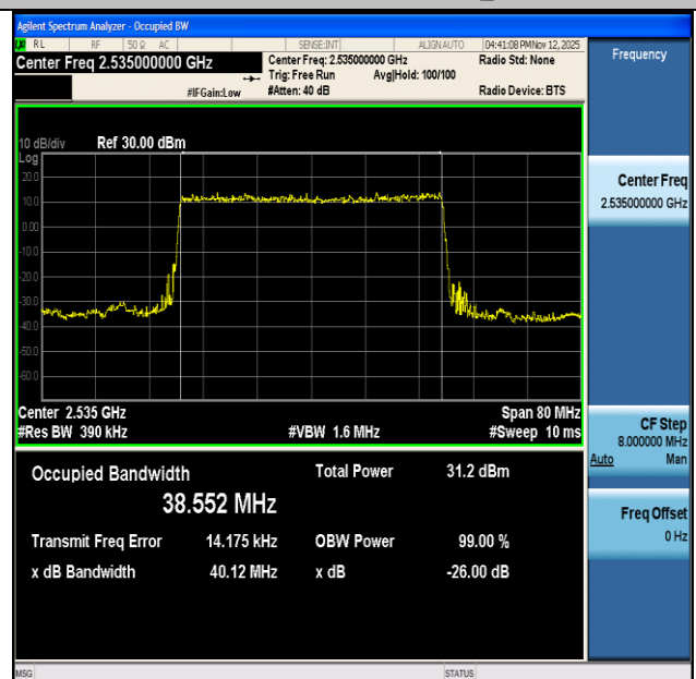
NTNV-n7-PC3-15-40-M-DFT-BPSK-Outer_Full-Ant1-PASS
