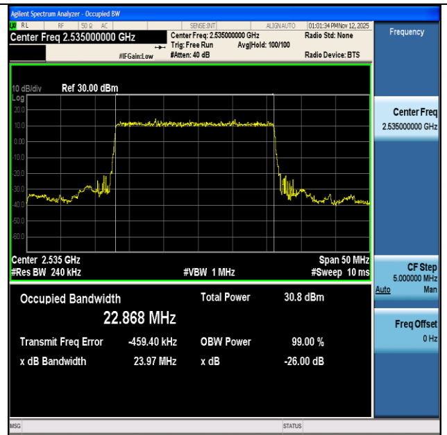
NTNV-n7-PC3-15-25-M-DFT-BPSK-Outer_Full-Ant1-PASS
