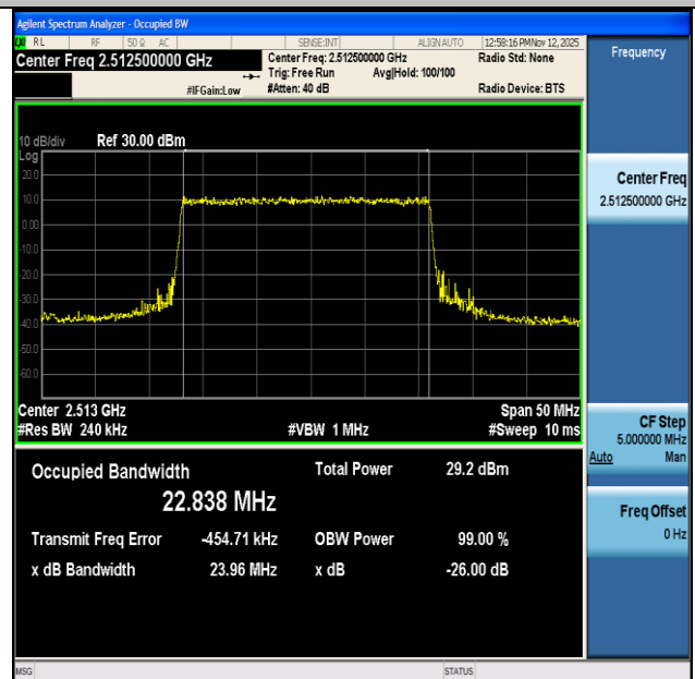
NTNV-n7-PC3-15-25-L-DFT-64QAM-Outter_Full-Ant1-PASS
