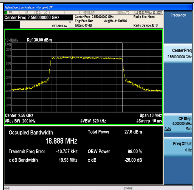
NTNV-n7-PC3-15-20-H-CP-256QAM-Outer_Full-Ant1-PASS
