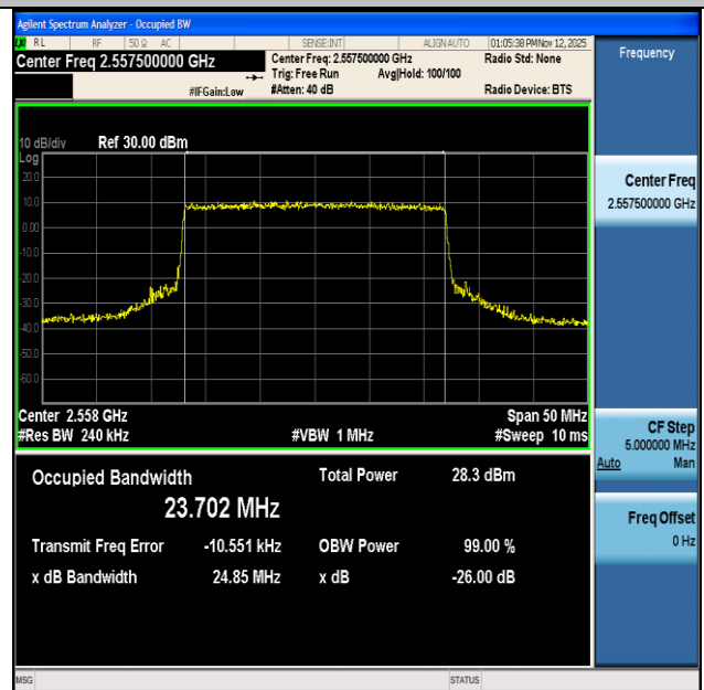
NTNV-n7-PC3-15-25-H-CP-QPSK-Outer_Full-Ant1-PASS
