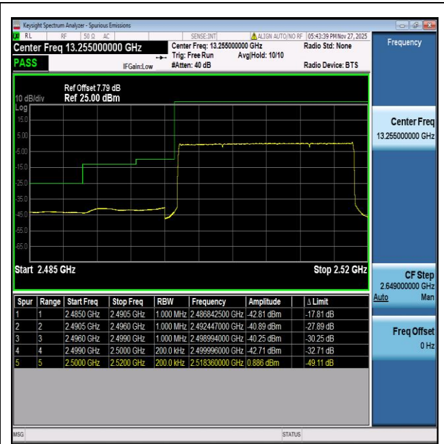
NTVN-n7-PC3-15-20-L-DFT-BPSK-Outer_Full-PASS
