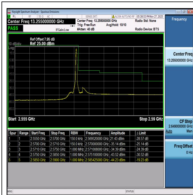
NTNV-n7-PC3-15-15-H-DFT-BPSK-Edge_1RB_Right-PASS
