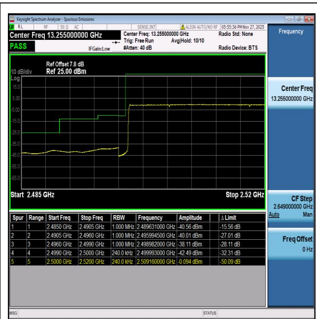
NTVN-n7-PC3-15-25-L-DFT-BPSK-Outer_Full-PASS
