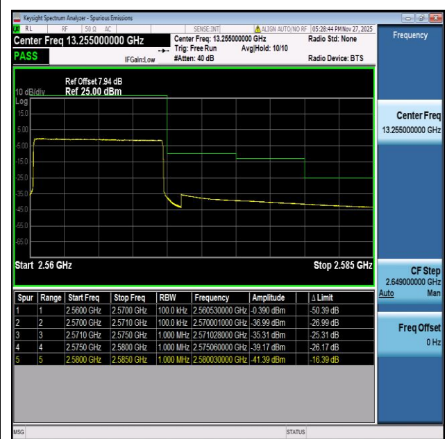
NTNV-n7-PC3-15-10-H-CP-QPSK-Outer_Full-PASS
