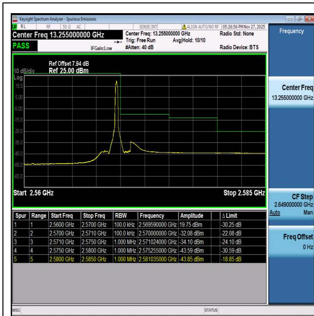
NTNV-n7-PC3-15-10-H-DFT-BPSK-Edge_1RB_Right-PASS
