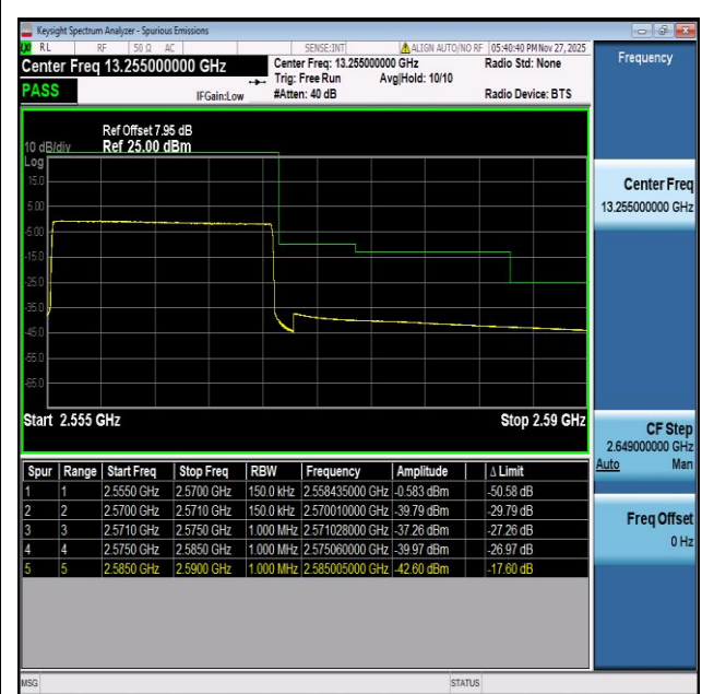
NTNV-n7-PC3-15-15-H-CP-QPSK-Outer_Full-PASS
