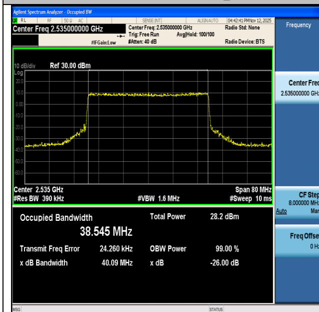
NTNV-n7-PC3-15-40-M-CP-64QAM-Outer_Full-Ant1-PASS
