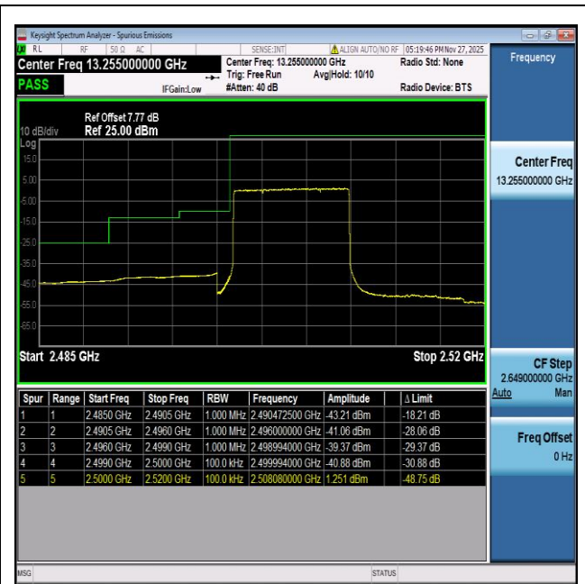
NTVN-n7-PC3-15-10-L-DFT-BPSK-Outer_Full-PASS
