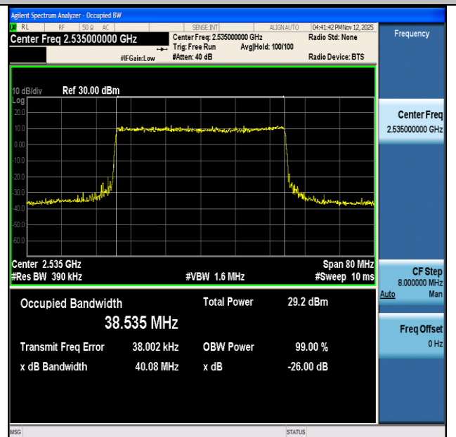
NTVN-n7-PC3-15-40-M-DFT-256QAM-Outer_Full-Ant1-PASS
