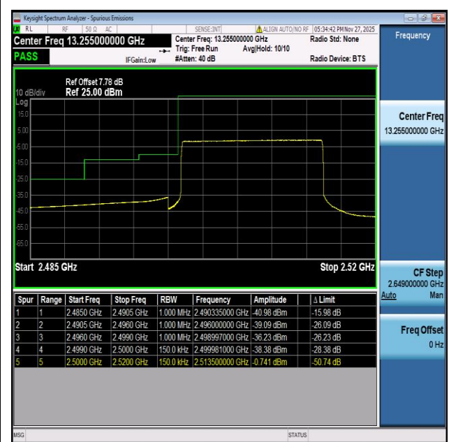
NTNV-n7-PC3-15-15-L-CP-QPSK-Outer_Full-PASS
