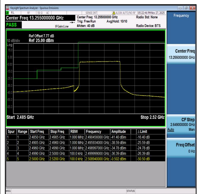
NTVN-n7-PC3-15-10-L-CP-QPSK-Outer_Full-PASS
