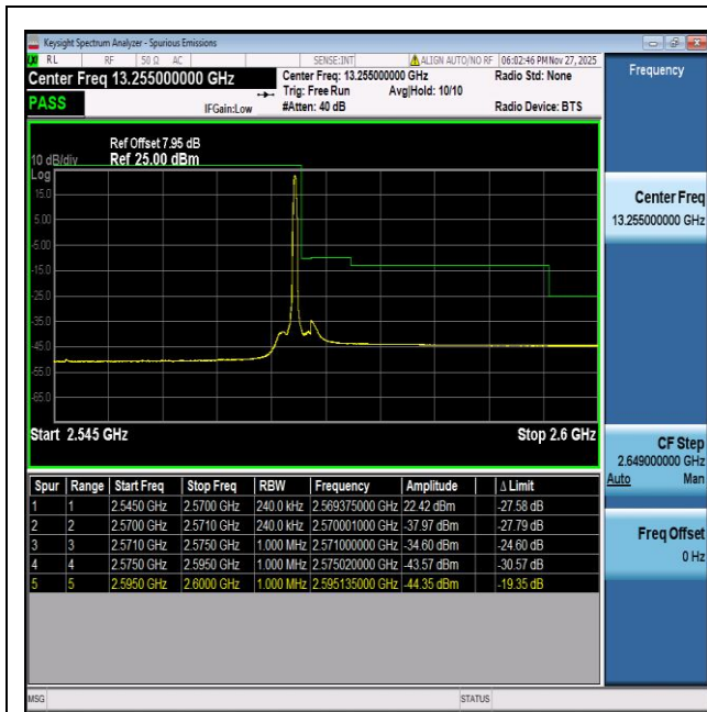
NTNV-n7-PC3-15-25-H-DFT-BPSK-Edge_1RB_Right-PASS
