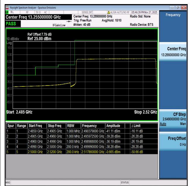
NTVN-n7-PC3-15-20-L-CP-QPSK-Outer_Full-PASS
