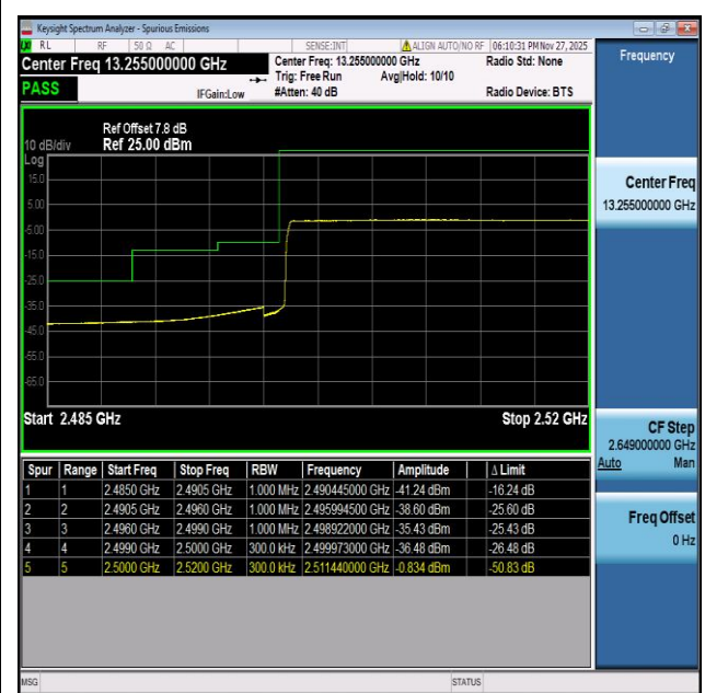
NTVN-n7-PC3-15-30-L-CP-QPSK-Outer_Full-PASS
