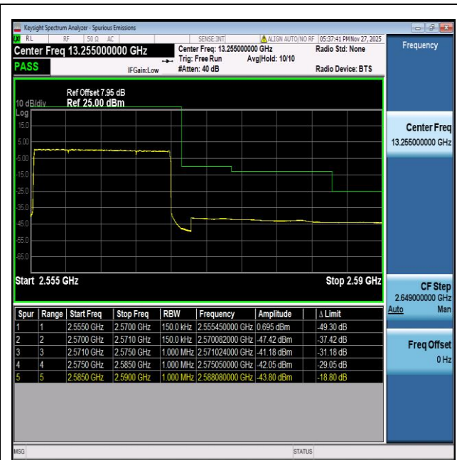
NTNV-n7-PC3-15-15-H-DFT-BPSK-Outer_Full-PASS
