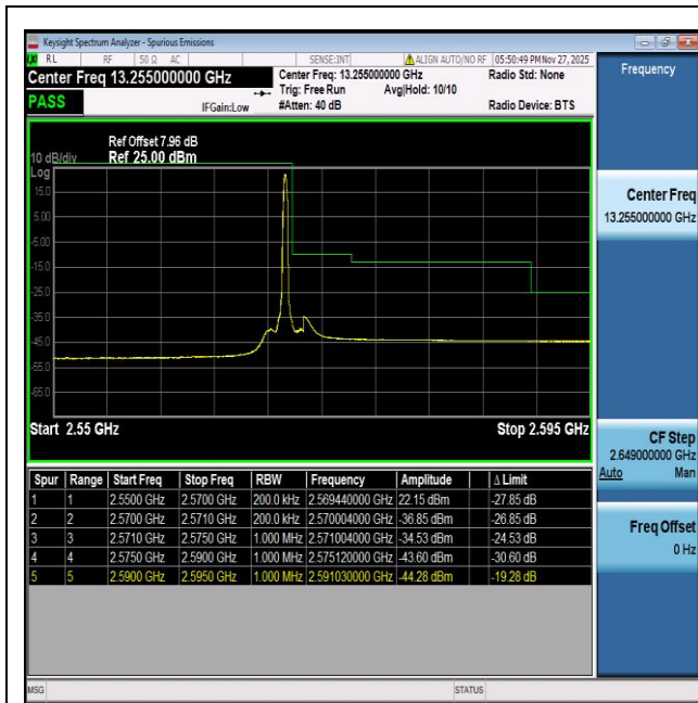
NTNV-n7-PC3-15-20-H-DFT-BPSK-Edge_1RB_Right-PASS
