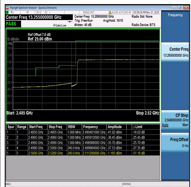
NTVN-n7-PC3-15-25-L-CP-QPSK-Outer_Full-PASS
