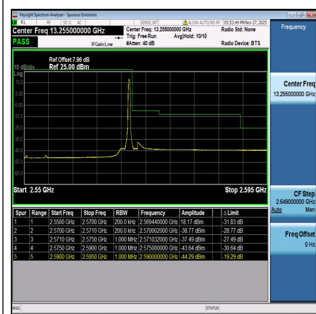
NTNV-n7-PC3-15-20-H-CP-QPSK-Edge_1RB_Right-PASS
