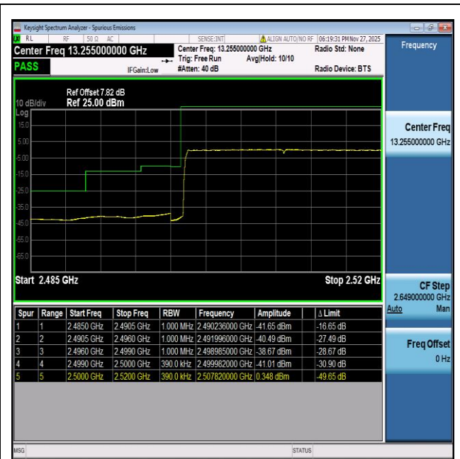
NTVN-n7-PC3-15-40-L-DFT-BPSK-Outer_Full-PASS
