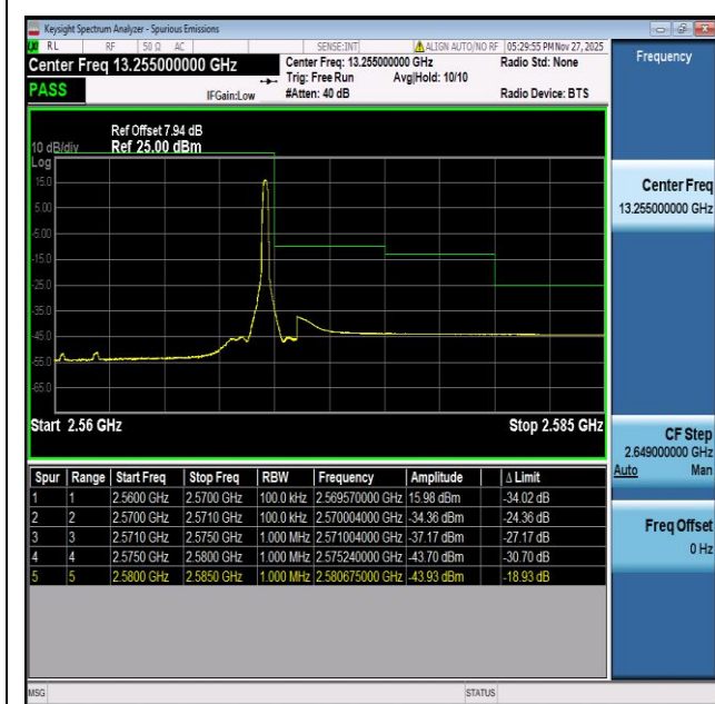
NTNV-n7-PC3-15-10-H-CP-QPSK-Edge_1RB_Right-PASS
