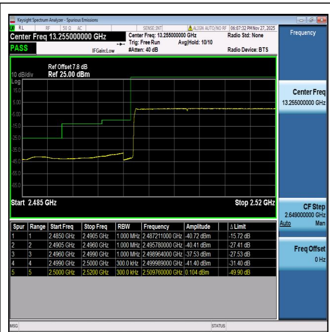
NTVN-n7-PC3-15-30-L-DFT-BPSK-Outer_Full-PASS
