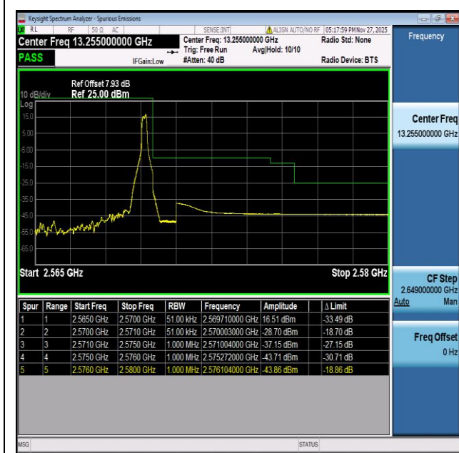
NTNV-n7-PC3-15-5-H-CP-QPSK-Edge_1RB_Right-PASS
