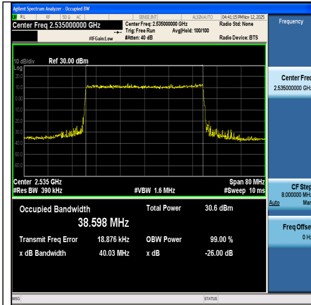
NTVN-n7-PC3-15-40-M-DFT-QPSK-Outer_Full-Ant1-PASS
