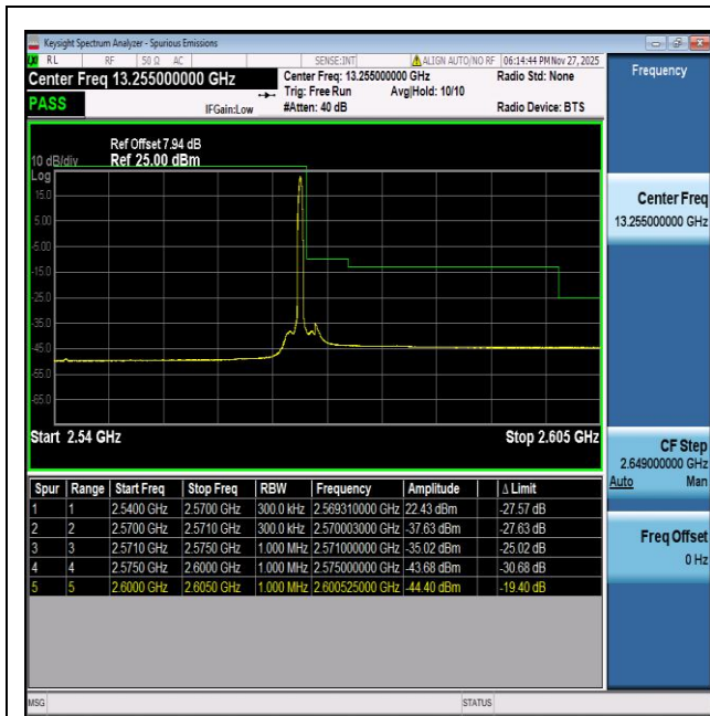
NTNV-n7-PC3-15-30-H-DFT-BPSK-Edge_1RB_Right-PASS
