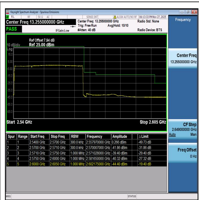
NTNV-n7-PC3-15-30-H-DFT-BPSK-Outer_Full-PASS
