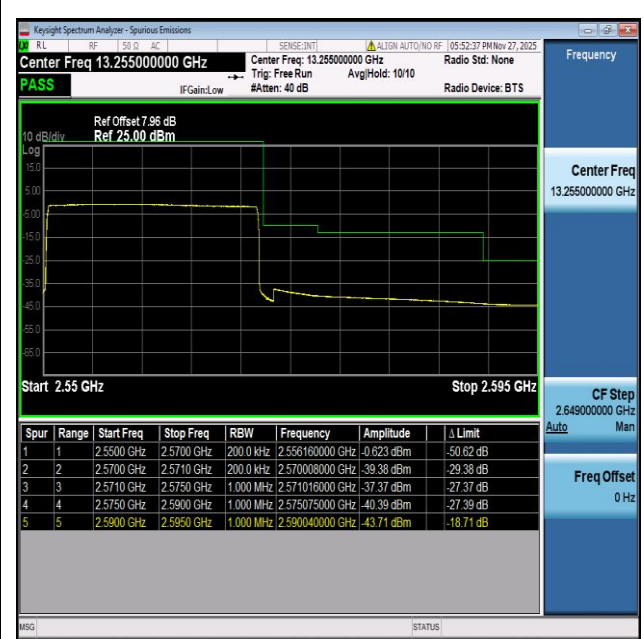
NTNV-n7-PC3-15-20-H-CP-QPSK-Outer_Full-PASS
