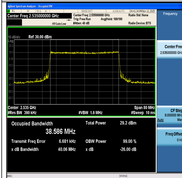
NTVN-n7-PC3-15-40-M-DFT-64QAM-Outer_Full-Ant1-PASS
