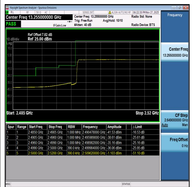
NTVN-n7-PC3-15-40-L-CP-QPSK-Outer_Full-PASS
