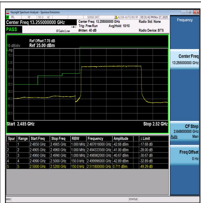
NTNV-n7-PC3-15-15-L-DFT-BPSK-Outer_Full-PASS
