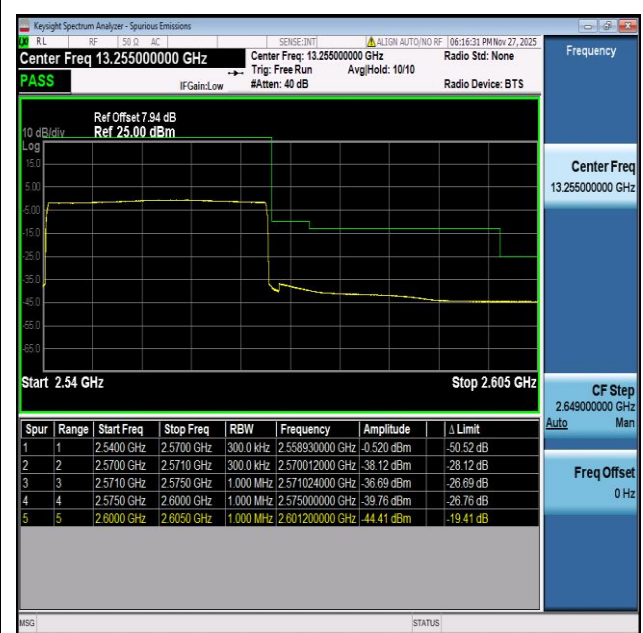
NTNV-n7-PC3-15-30-H-CP-QPSK-Outer_Full-PASS
