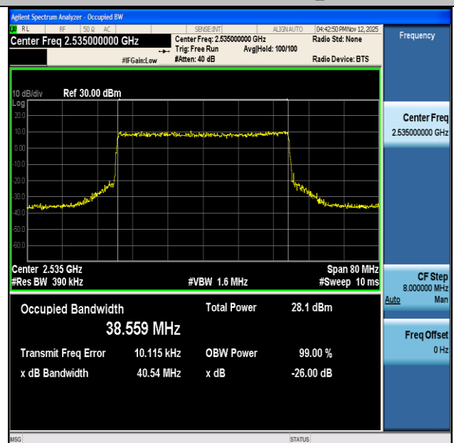
NTNV-n7-PC3-15-40-M-CP-256QAM-Outer_Full-Ant1-PASS
