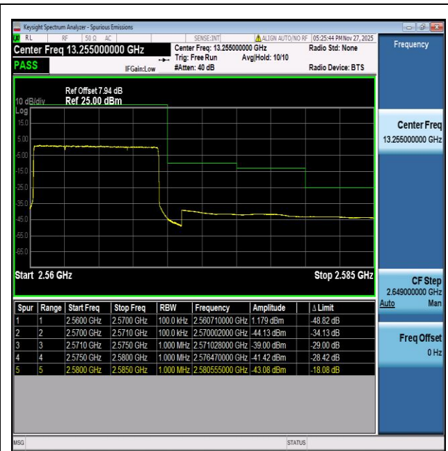
NTNV-n7-PC3-15-10-H-DFT-BPSK-Outer_Full-PASS
