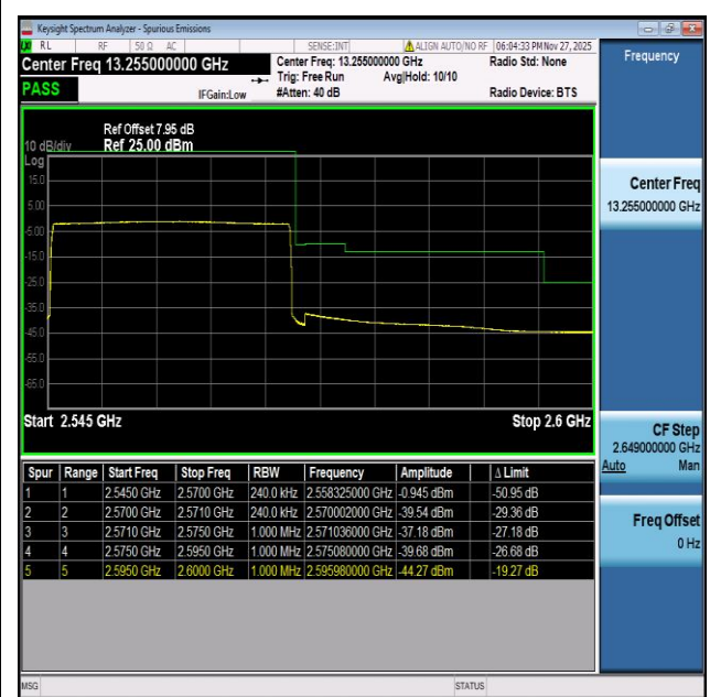
NTNV-n7-PC3-15-25-H-CP-QPSK-Outer_Full-PASS
