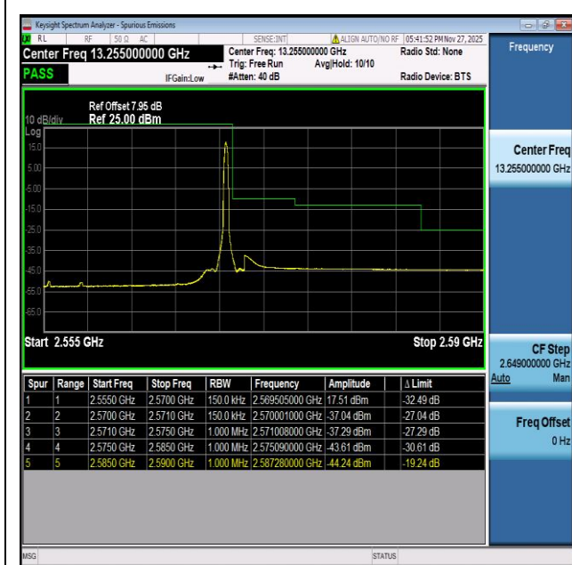
NTNV-n7-PC3-15-15-H-CP-QPSK-Edge_1RB_Right-PASS
