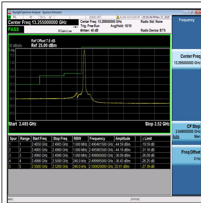
NTVN-n7-PC3-15-25-L-DFT-BPSK-Edge_1RB_Left-PASS
