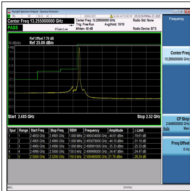
NTNV-n7-PC3-15-15-L-DFT-BPSK-Edge_1RB_Left-PASS
