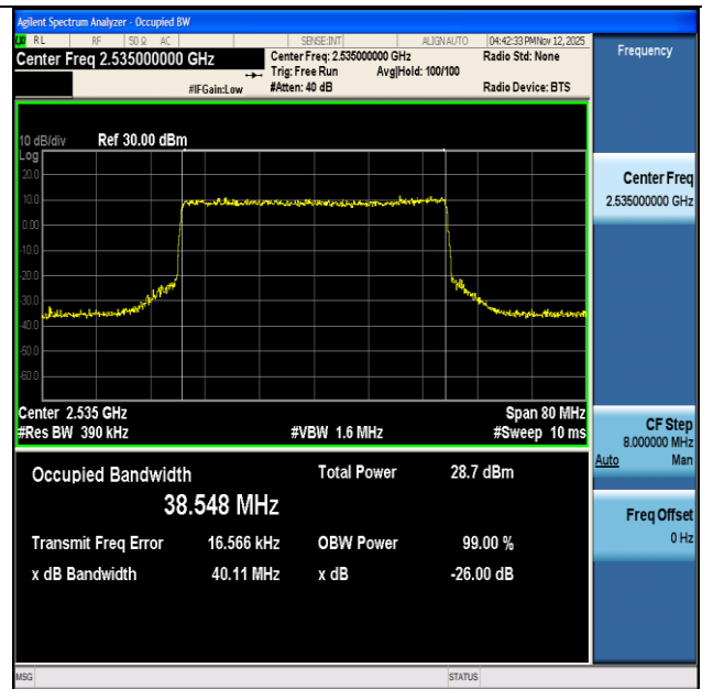
NTNV-n7-PC3-15-40-M-CP-16QAM-Outer_Full-Ant1-PASS
