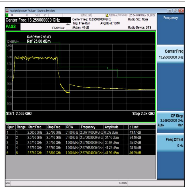
NTNV-n7-PC3-15-5-H-DFT-BPSK-Outer_Full-PASS
