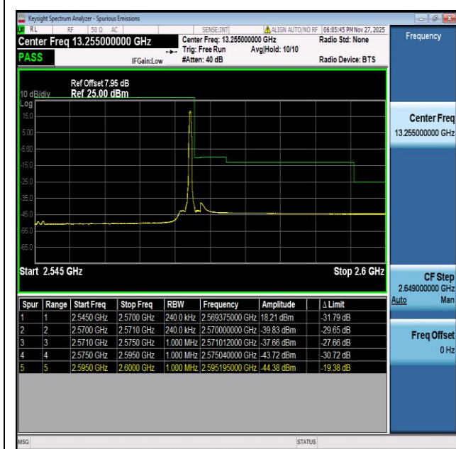
NTNV-n7-PC3-15-25-H-CP-QPSK-Edge_1RB_Right-PASS
