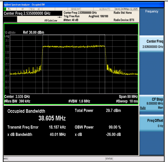
NTVN-n7-PC3-15-40-M-DFT-16QAM-Outer_Full-Ant1-PASS
