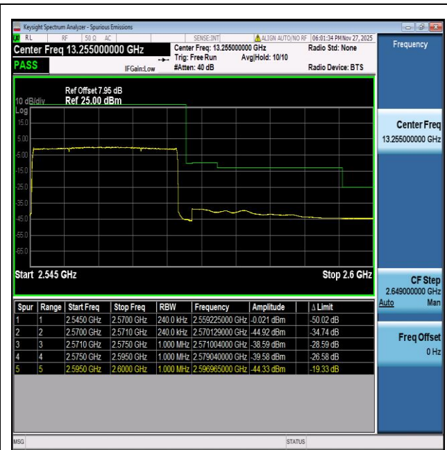
NTNV-n7-PC3-15-25-H-DFT-BPSK-Outer_Full-PASS
