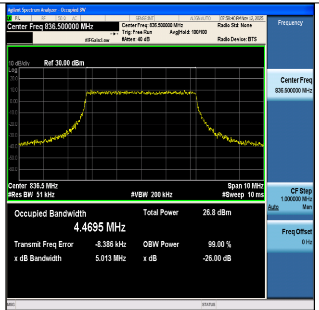
NTNV-n26(824-849)-PC3-15-5-M-CP-256QAM-Outer_Full-Ant1- PASS
