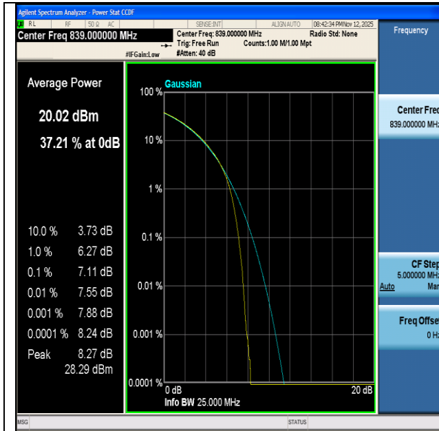
NTNV-n26(824-849)-PC3-15-20-H-CP-16QAM-Outer_Full-PASS
