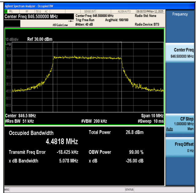
NTNV-n26(824-849)-PC3-15-5-H-CP-64QAM-Outer_Full-Ant1- PASS
