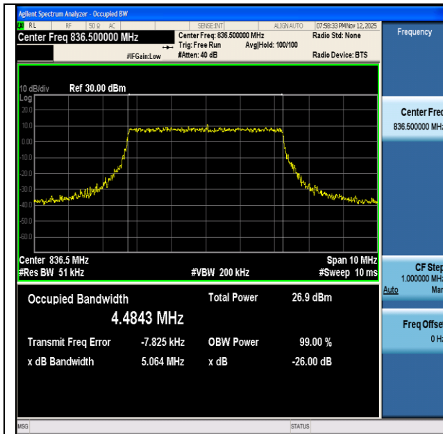
NTNV-n26(824-849)-PC3-15-5-M-CP-64QAM-Outer_Full-Ant1- PASS
