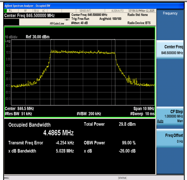
NTNV-n26(824-849)-PC3-15-5-H-DFT-QPSK-Outer_Full-Ant1- PASS
