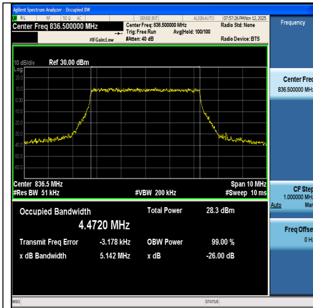
NTNV-n26(824-849)-PC3-15-5-M-DFT-64QAM-Outer_Full-Ant1- PASS
