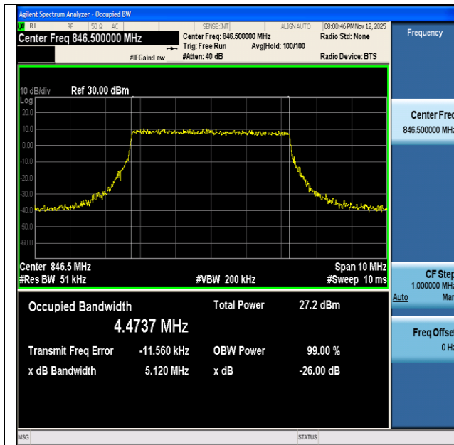
NTNV-n26(824-849)-PC3-15-5-H-CP-16QAM-Outer_Full-Ant1- PASS
