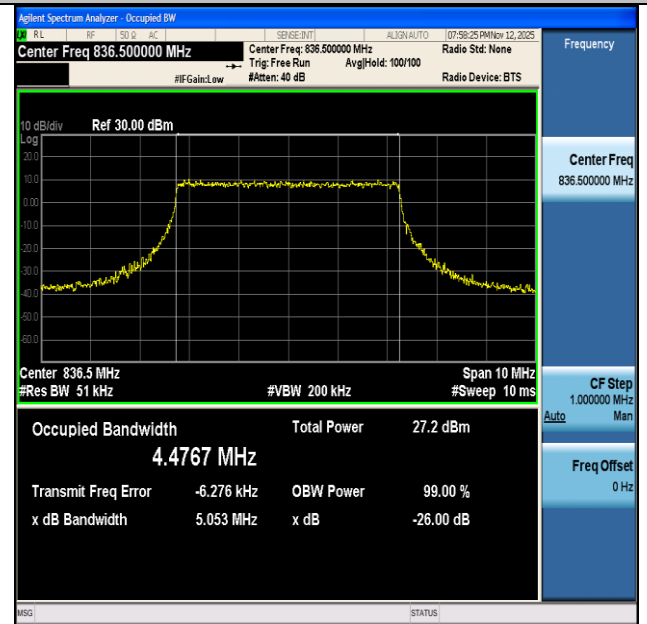
NTNV-n26(824-849)-PC3-15-5-M-CP-16QAM-Outer_Full-Ant1- PASS
