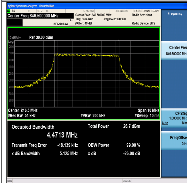
NTNV-n26(824-849)-PC3-15-5-H-CP-256QAM-Outer_Full-Ant1- PASS
