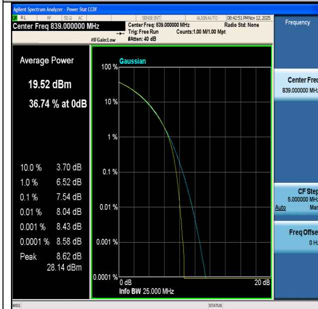
NTNV-n26(824-849)-PC3-15-20-H-CP-256QAM-Outer_Full-PASS
