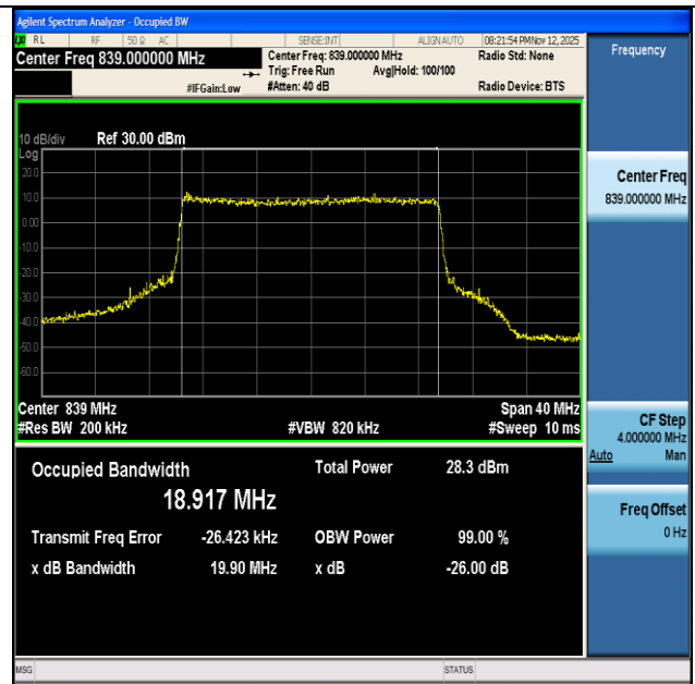
NTNV-n26(824-849)-PC3-15-20-H-CP-16QAM-Outer_Full-Ant1- PASS
