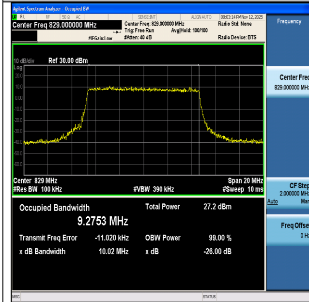
NTNV-n26(824-849)-PC3-15-10-L-CP-64QAM-Outer_Full-Ant1- PASS
