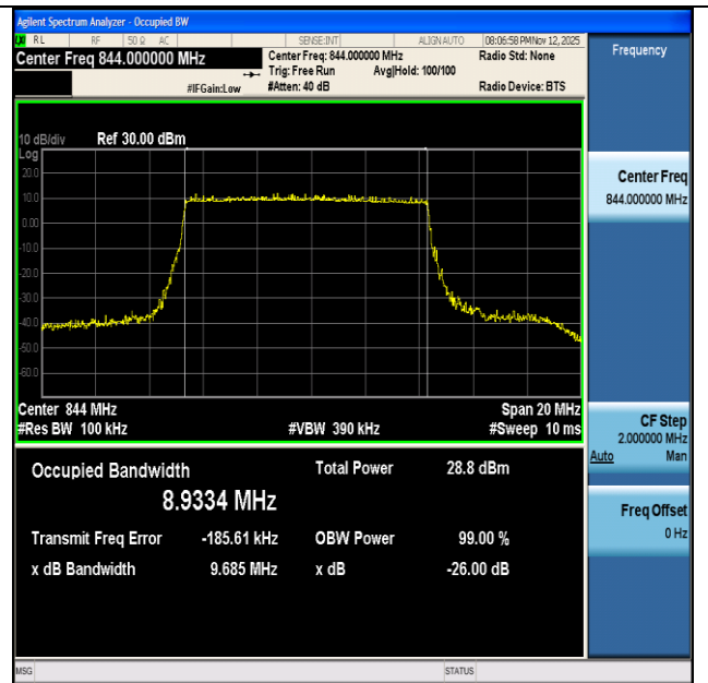
NTVN-n26(824-849)-PC3-15-10-H-DFT-256QAM-Outer_Full- Ant1-PASS
