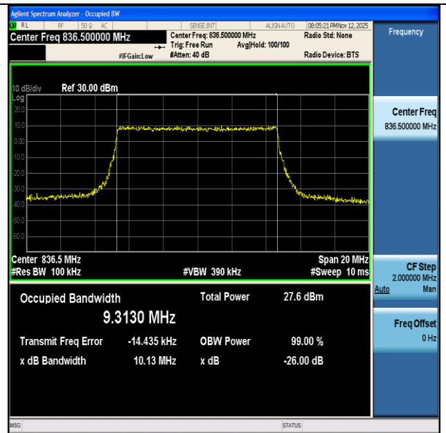
NTNV-n26(824-849)-PC3-15-10-M-CP-QPSK-Outer_Full-Ant1-PASS
