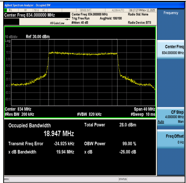
NTNV-n26(824-849)-PC3-15-20-L-CP-256QAM-Outer_Full-Ant1- PASS
