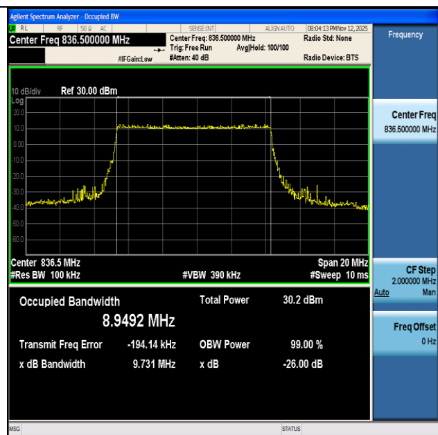
NTNV-n26(824-849)-PC3-15-10-M-DFT-QPSK-Outer_Full-Ant1- PASS
