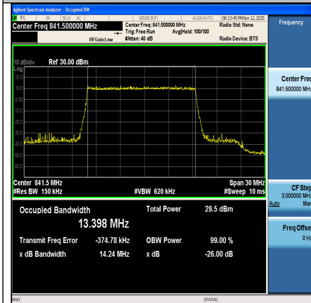
NTNV-n26(824-849)-PC3-15-15-H-DFT-16QAM-Outer_Full-Ant1- PASS
