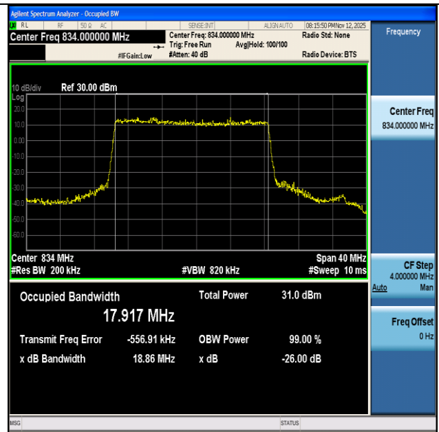
NTNV-n26(824-849)-PC3-15-20-L-DFT-BPSK-Outer_Full-Ant1- PASS
