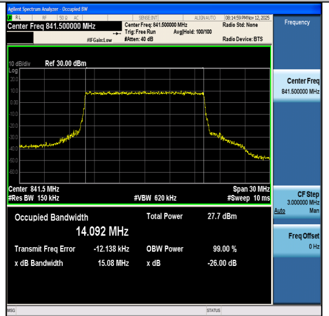
NTNV-n26(824-849)-PC3-15-15-H-CP-64QAM-Outer_Full-Ant1-PASS
