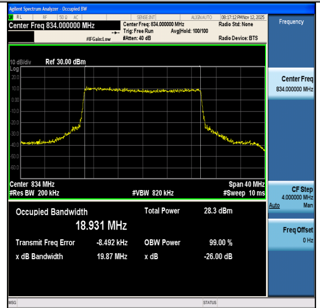
NTVN-n26(824-849)-PC3-15-20-L-CP-16QAM-Outer_Full-Ant1- PASS
