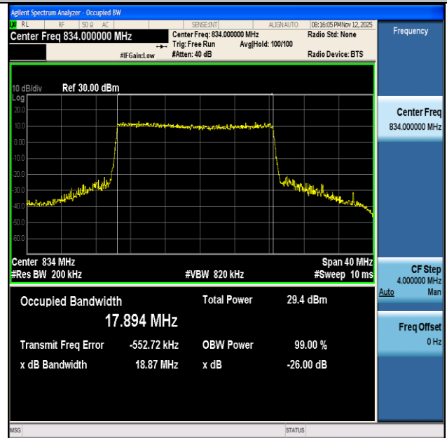
NTNV-n26(824-849)-PC3-15-20-L-DFT-16QAM-Outer_Full-Ant1- PASS
