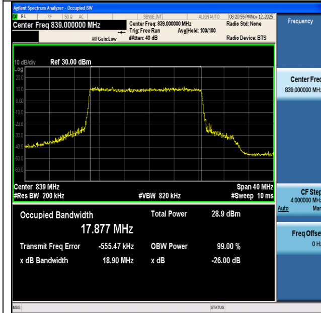
NTNV-n26(824-849)-PC3-15-20-H-DFT-64QAM-Outer_Full-Ant1- PASS
