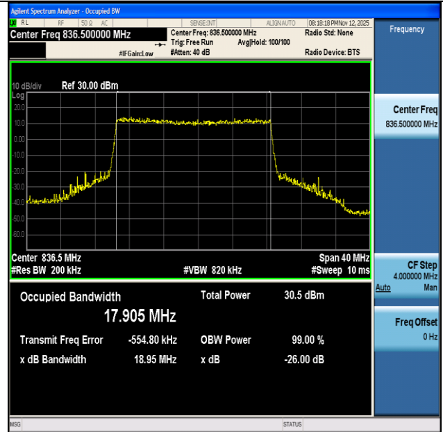
NTNV-n26(824-849)-PC3-15-20-M-DFT-QPSK-Outer_Full-Ant1- PASS
