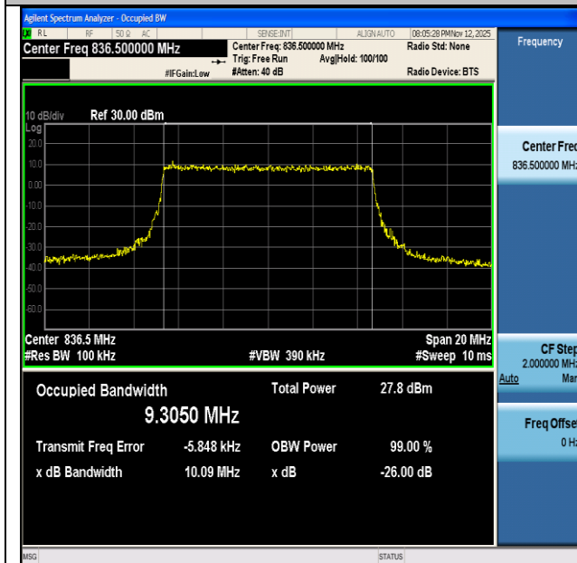
NTNV-n26(824-849)-PC3-15-10-M-CP-16QAM-Outer_Full-Ant1-PASS
