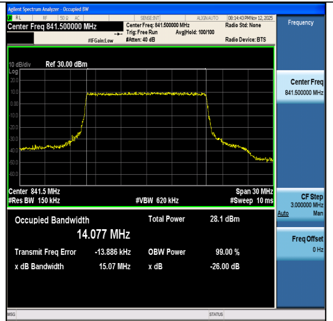
NTNV-n26(824-849)-PC3-15-15-H-CP-QPSK-Outer_Full-Ant1-PASS
