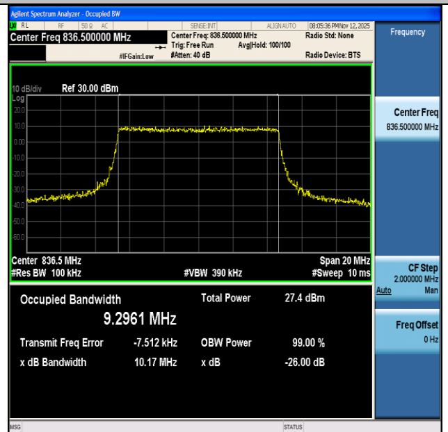
NTNV-n26(824-849)-PC3-15-10-M-CP-64QAM-Outer_Full-Ant1-PASS
