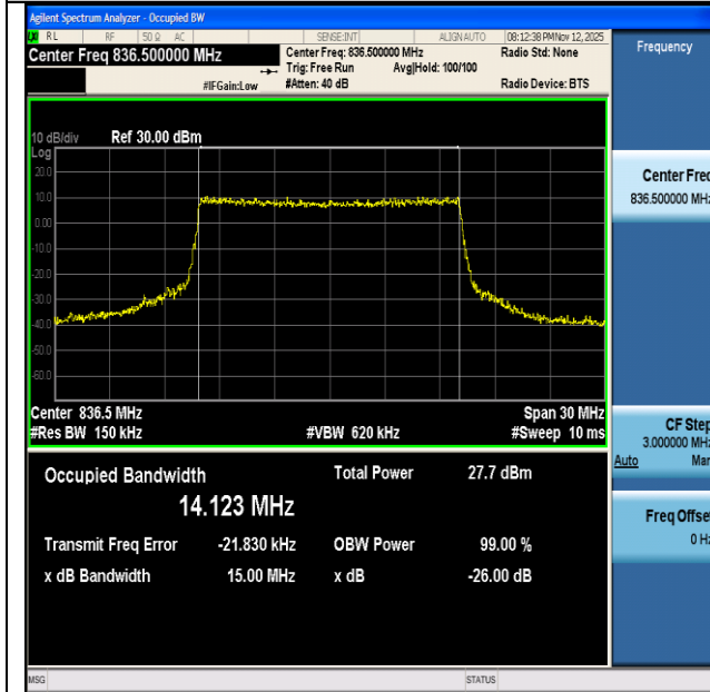
NTNV-n26(824-849)-PC3-15-15-M-CP-64QAM-Outer_Full-Ant1- PASS
