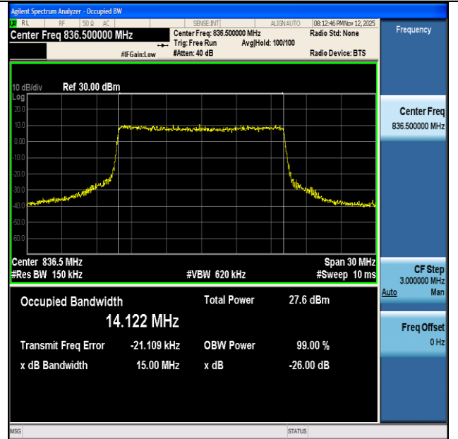
NTNV-n26(824-849)-PC3-15-15-M-CP-256QAM-Outer_Full-Ant1- PASS
