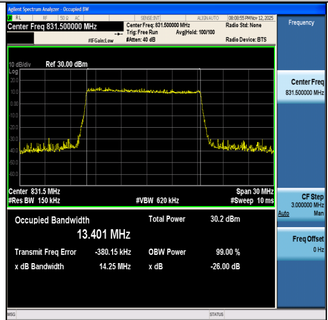
NTNV-n26(824-849)-PC3-15-15-L-DFT-QPSK-Outer_Full-Ant1- PASS
