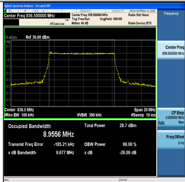
NTNV-n26(824-849)-PC3-15-10-M-DFT-64QAM-Outer_Full-Ant1- PASS
