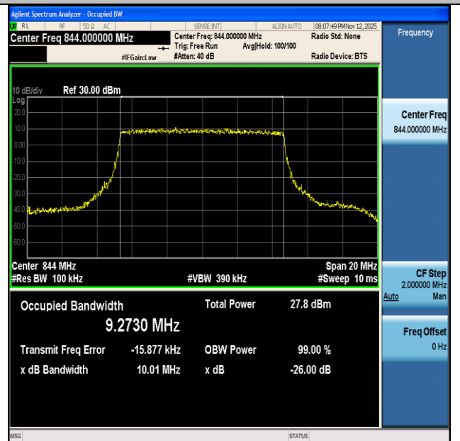
NTVN-n26(824-849)-PC3-15-10-H-CP-16QAM-Outer_Full-Ant1- PASS
