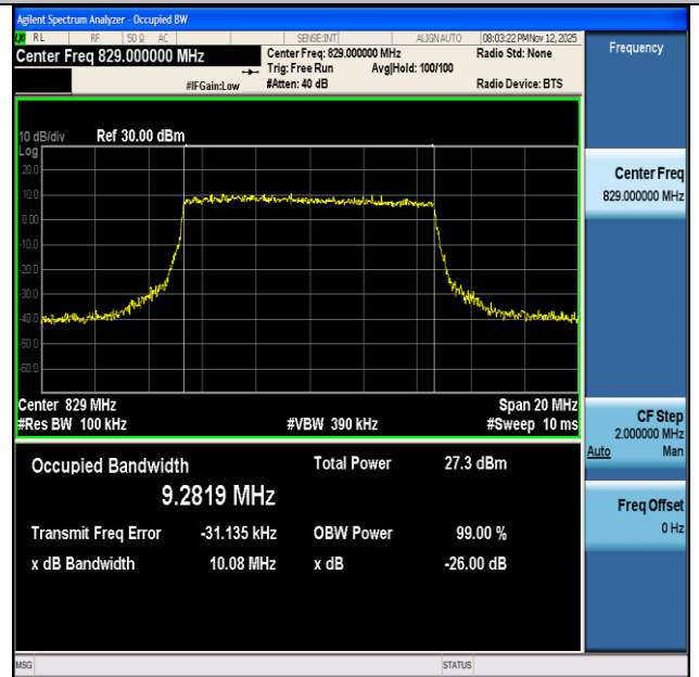
NTNV-n26(824-849)-PC3-15-10-L-CP-256QAM-Outer_Full-Ant1- PASS
