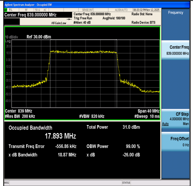
NTNV-n26(824-849)-PC3-15-20-H-DFT-BPSK-Outer_Full-Ant1- PASS
