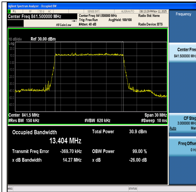
NTNV-n26(824-849)-PC3-15-15-H-DFT-BPSK-Outer_Full-Ant1- PASS
