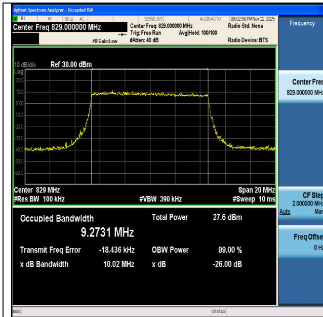
NTNV-n26(824-849)-PC3-15-10-L-CP-QPSK-Outer_Full-Ant1- PASS
