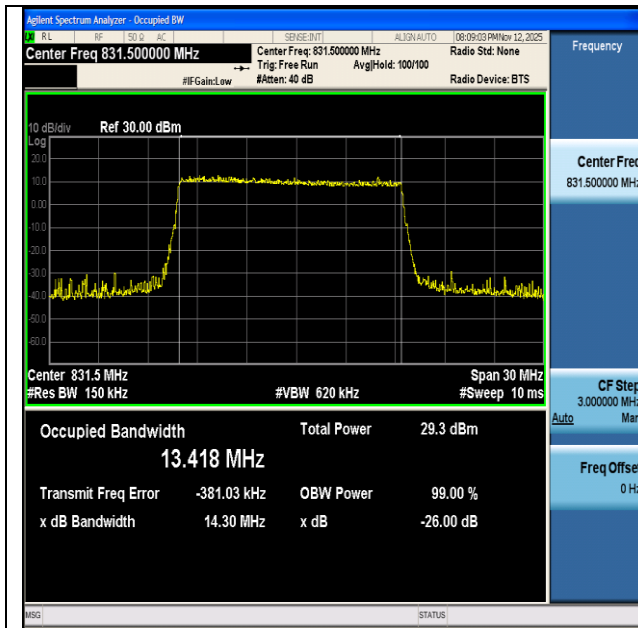
NTNV-n26(824-849)-PC3-15-15-L-DFT-16QAM-Outer_Full-Ant1- PASS
