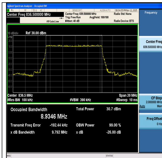
NTNV-n26(824-849)-PC3-15-10-M-DFT-BPSK-Outer_Full-Ant1- PASS
