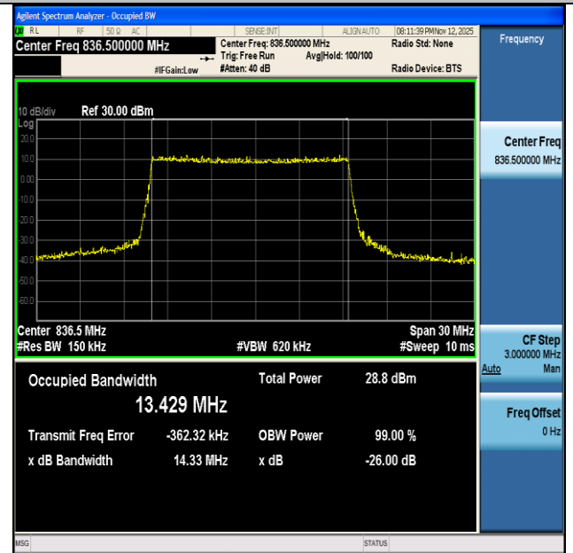
NTNV-n26(824-849)-PC3-15-15-M-DFT-256QAM-Outet_Full-Ant1-PASS
