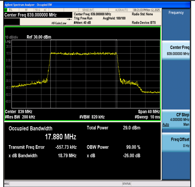
NTNV-n26(824-849)-PC3-15-20-H-DFT-256QAM-Outer_Full- Ant1-PASS
