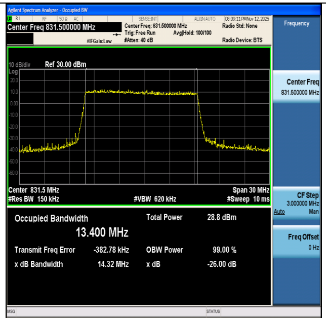
NTNV-n26(824-849)-PC3-15-15-L-DFT-64QAM-Outer_Full-Ant1- PASS
