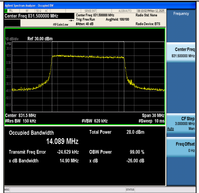
NTNV-n26(824-849)-PC3-15-15-L-CP-QPSK-Outer_Full-Ant1- PASS
