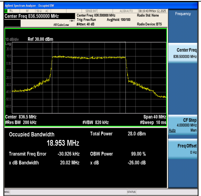
NTNV-n26(824-849)-PC3-15-20-M-CP-64QAM-Outer_Full-Ant1- PASS
