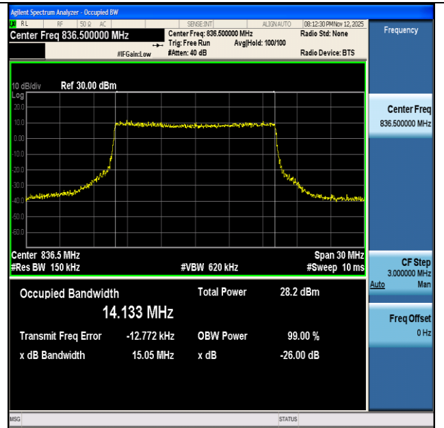
NTNV-n26(824-849)-PC3-15-15-M-CP-16QAM-Outer_Full-Ant1- PASS
