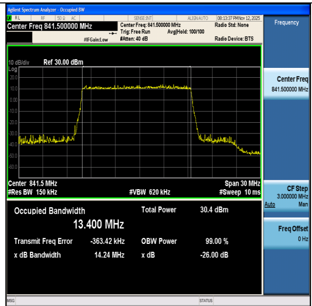
NTNV-n26(824-849)-PC3-15-15-H-DFT-QPSK-Outer_Full-Ant1- PASS
