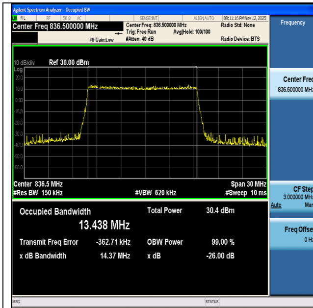
NTNV-n26(824-849)-PC3-15-15-M-DFT-QPSK-Outet_Full-Ant1- PASS
