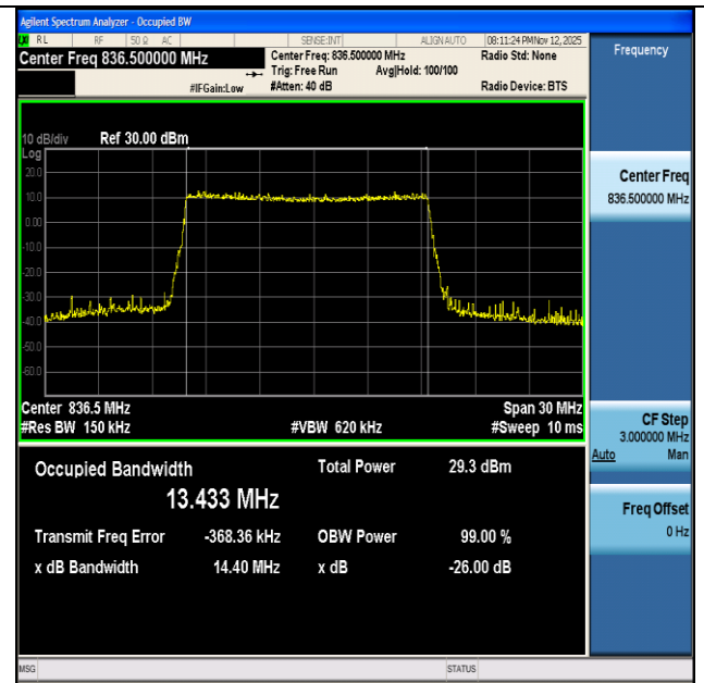
NTNV-n26(824-849)-PC3-15-15-M-DFT-16QAM-Outet_Full-Ant1- PASS
