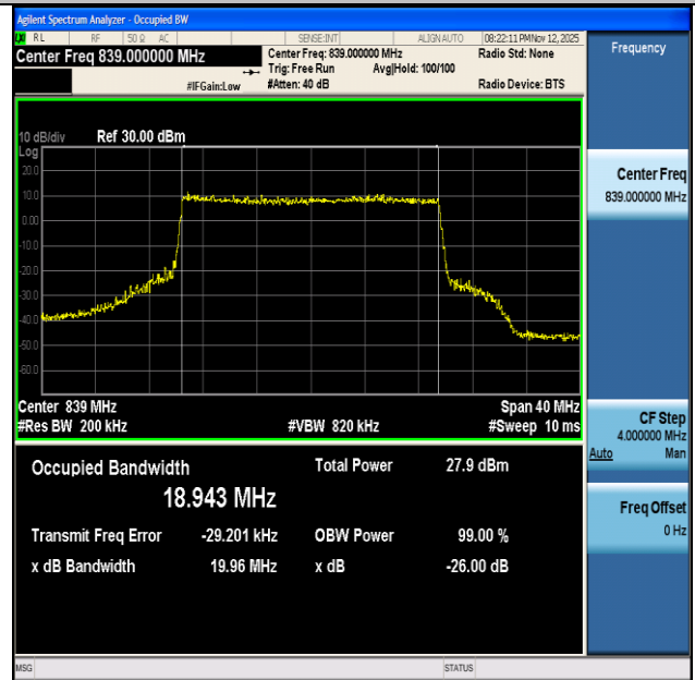
NTNV-n26(824-849)-PC3-15-20-H-CP-256QAM-Outer_Full-Ant1- PASS
