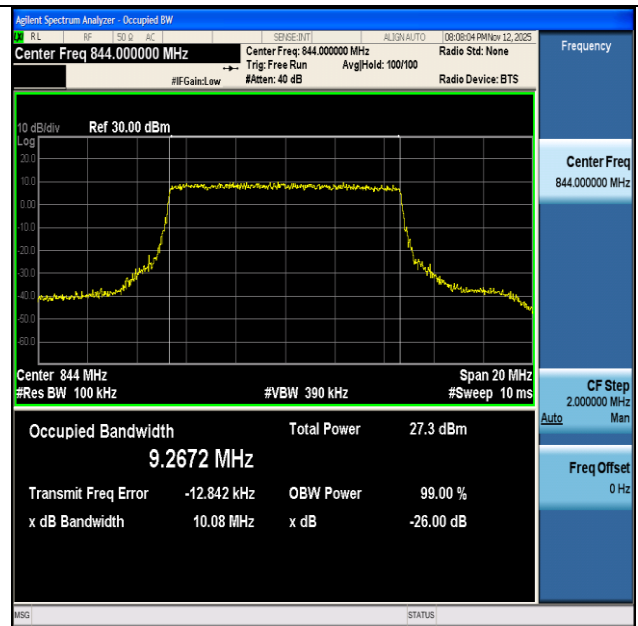
NTNV-n26(824-849)-PC3-15-10-H-CP-256QAM-Outer_Full-Ant1- PASS
