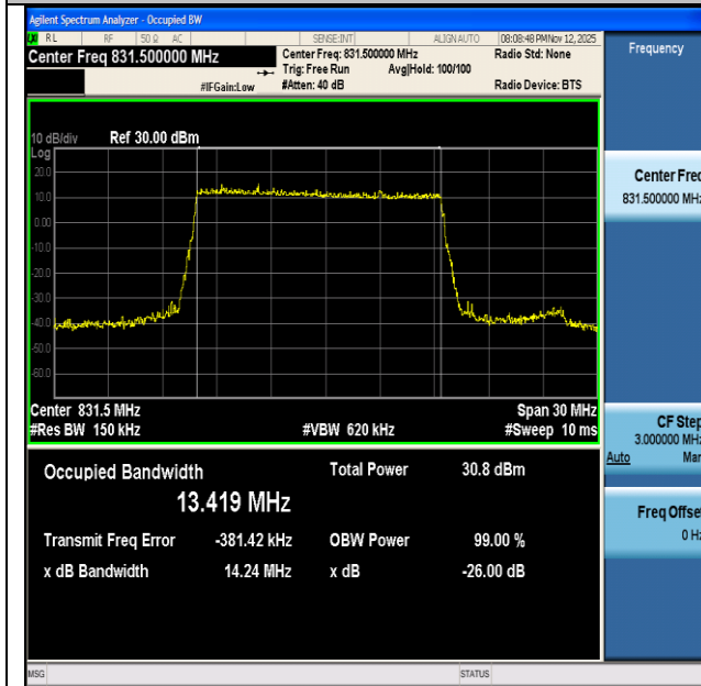
NTNV-n26(824-849)-PC3-15-15-L-DFT-BPSK-Outer_Full-Ant1- PASS
