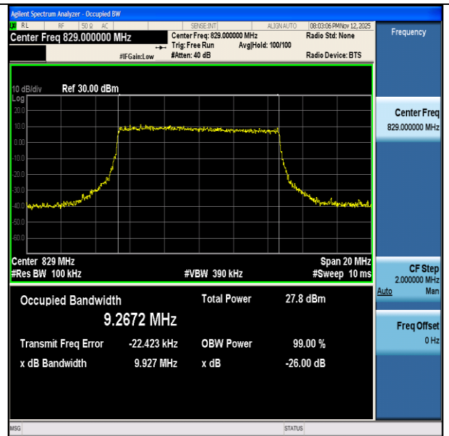
NTNV-n26(824-849)-PC3-15-10-L-CP-16QAM-Outer_Full-Ant1- PASS
