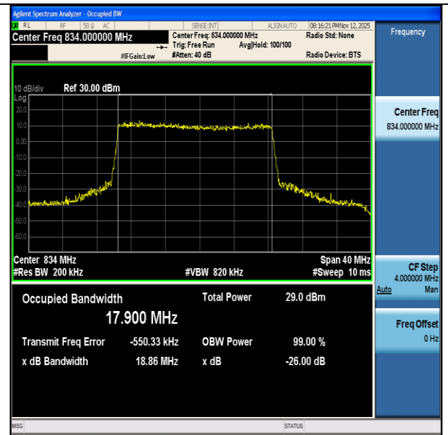
NTVN-n26(824-849)-PC3-15-20-L-DFT-256QAM-Outer_Full-Ant1- PASS
