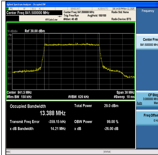
NTNV-n26(824-849)-PC3-15-15-H-DFT-256QAM-Outer_Full-Ant1-PASS
